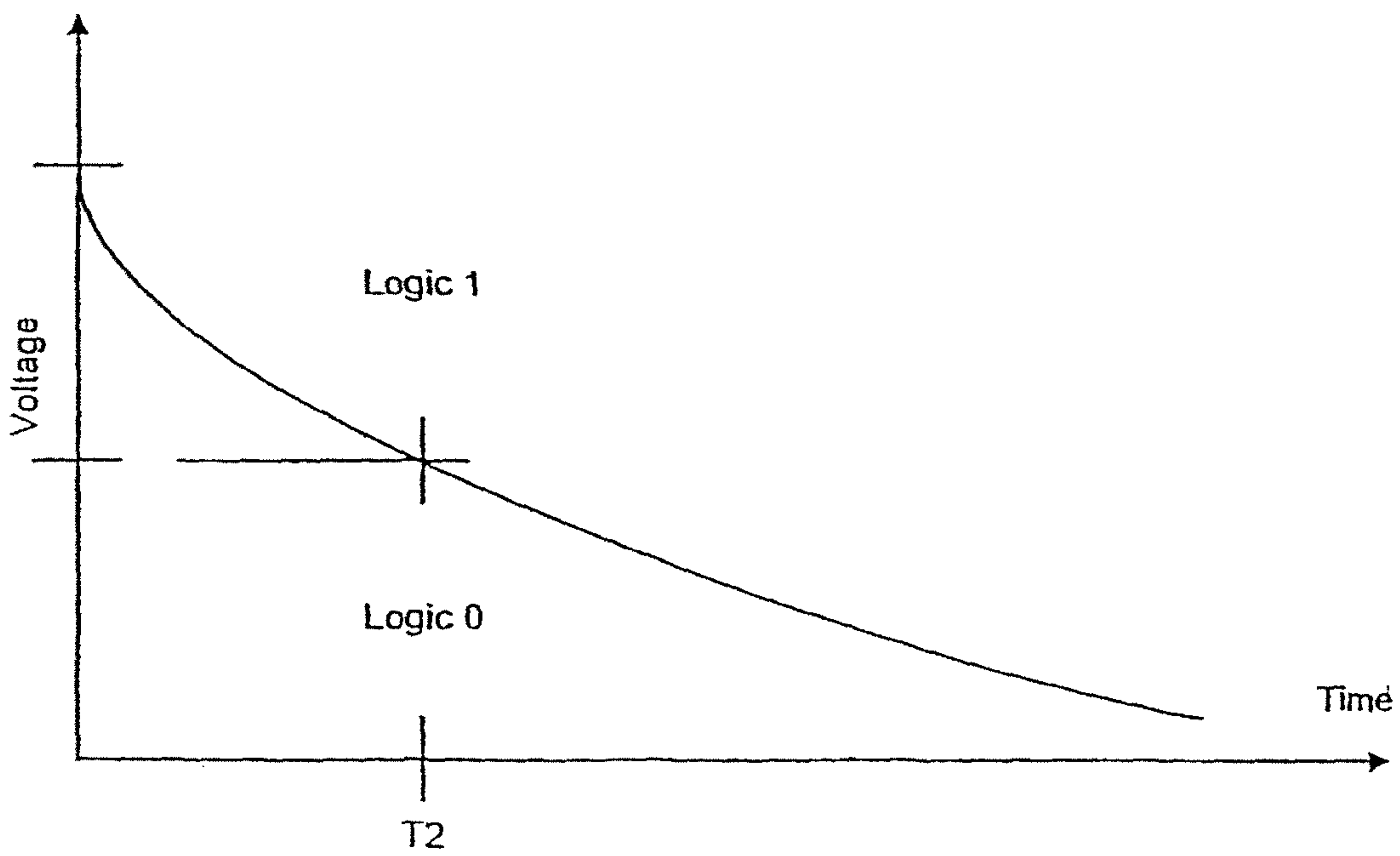
Figure 4(b) Discharge Waveform of Valid DRAM Bit
