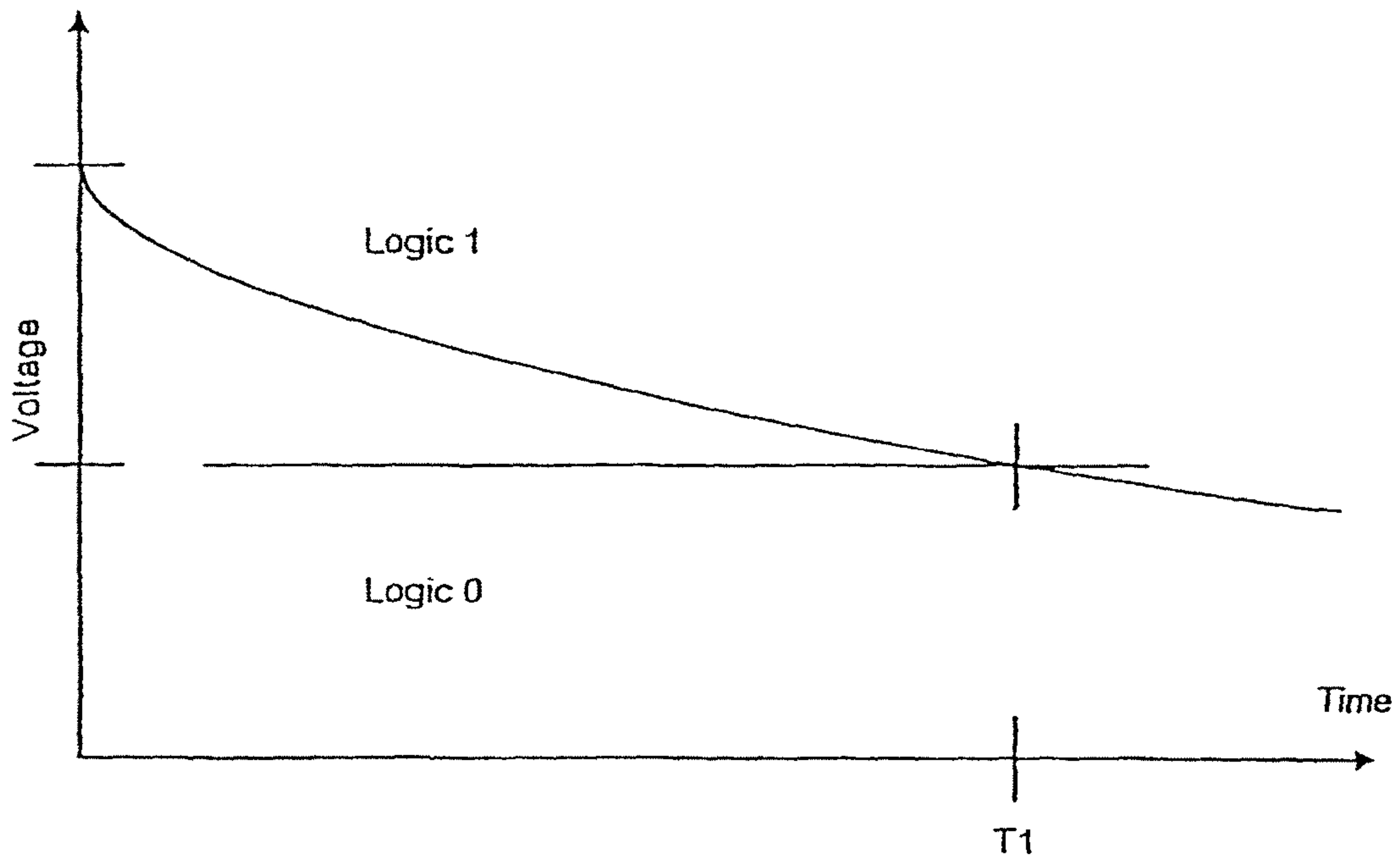
Figure 4(a): Discharge Waveform of Temporary Memory
