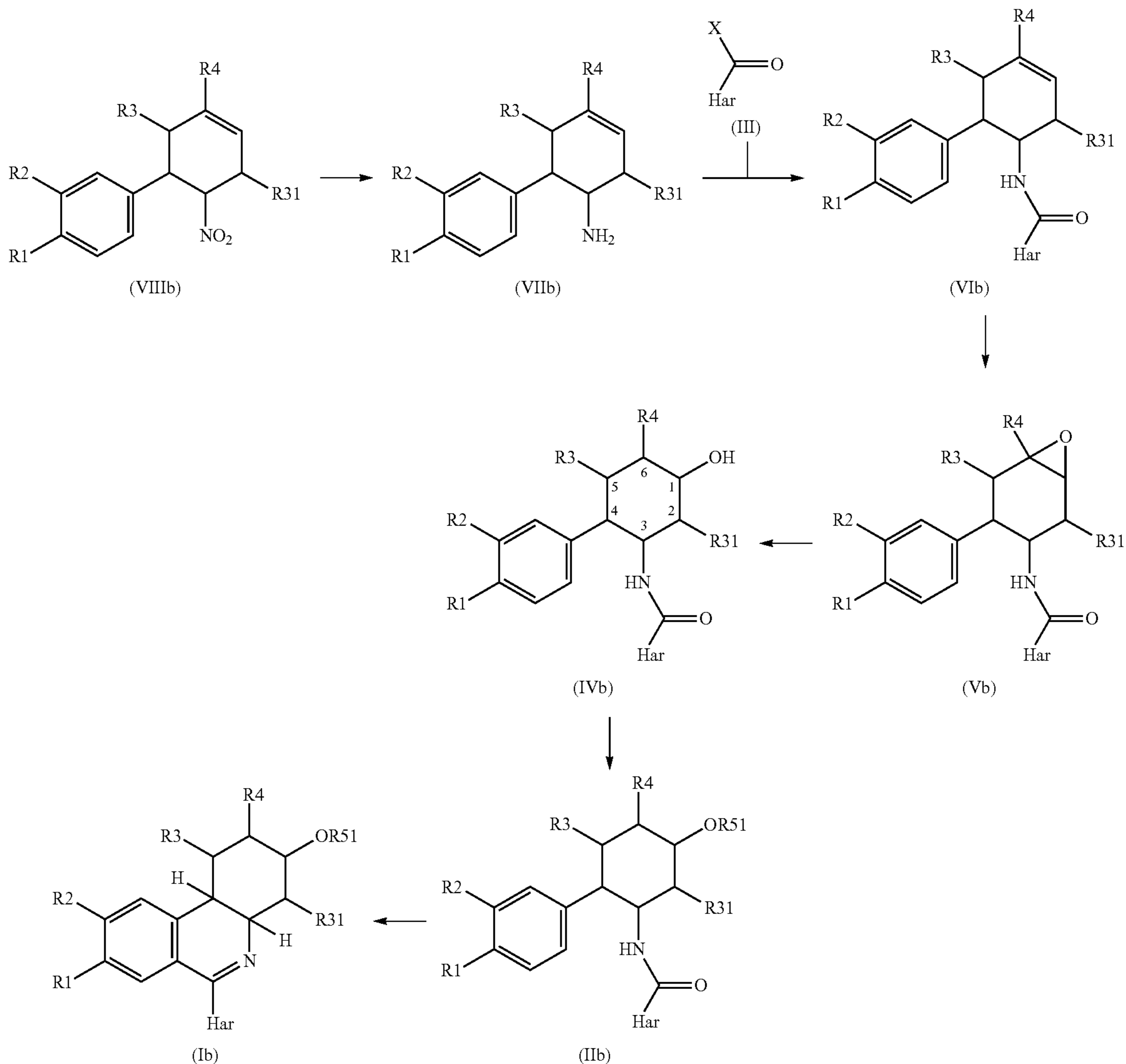
Reaction scheme 3:
