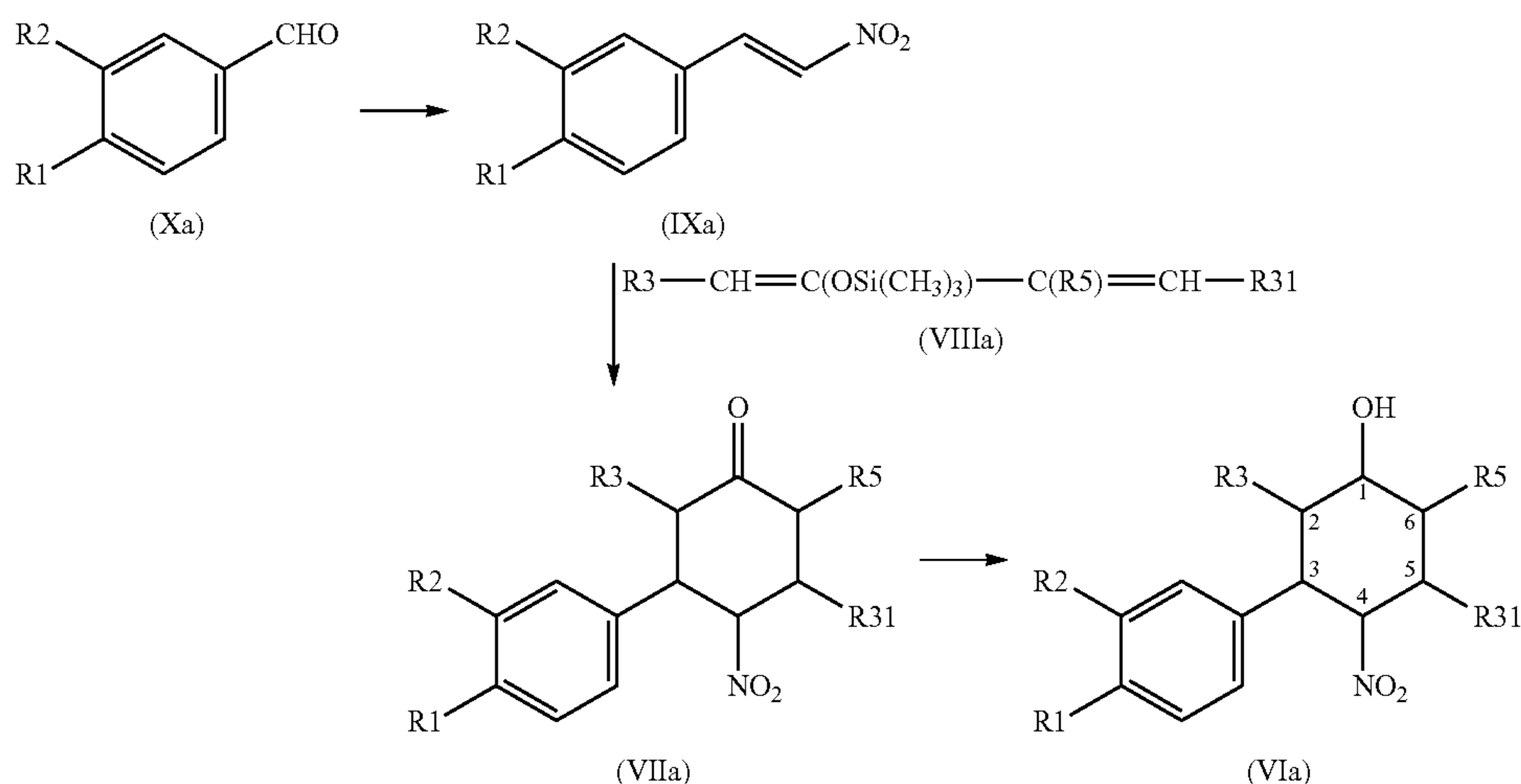
Reaction scheme 2:
