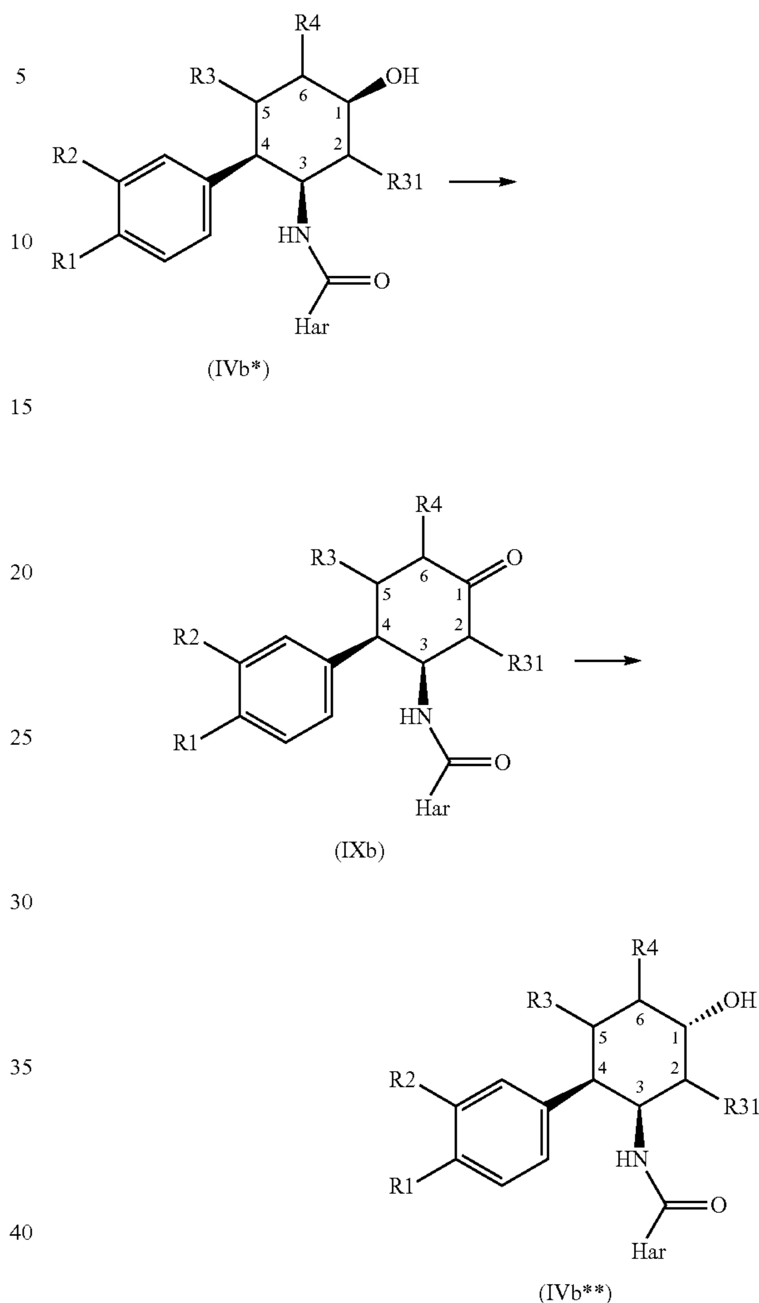
Reaction scheme 4:
