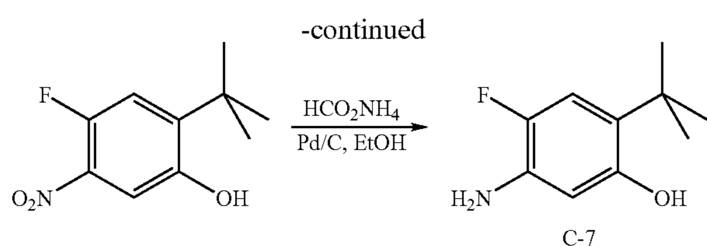
2-tert-Butyl-4-fluorophenol
