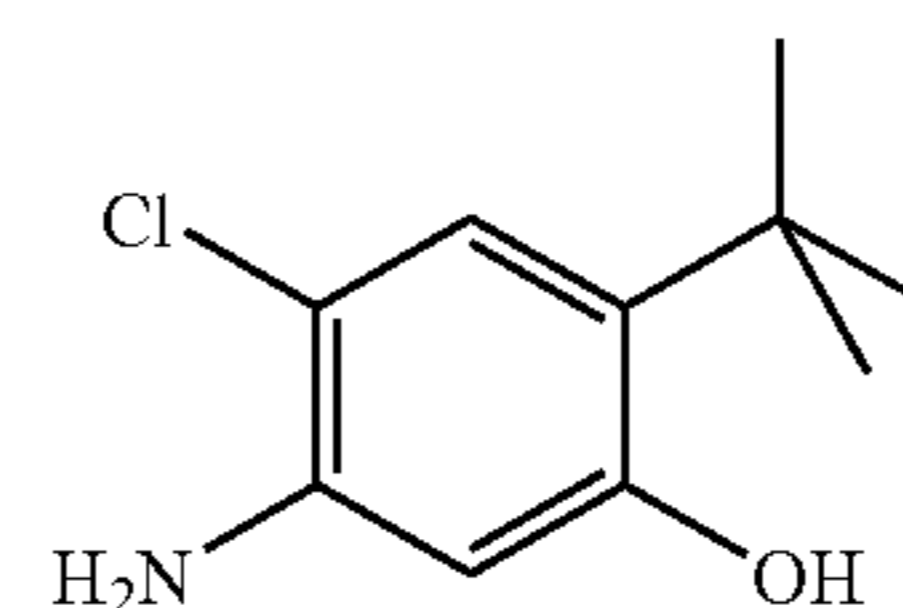
C-10; 2-tert-Butyl-5-amino-4-chlorophenol
