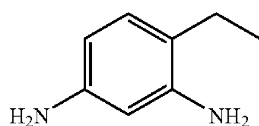
D-7; 4-Ethylbenzene-1,3-diamine
