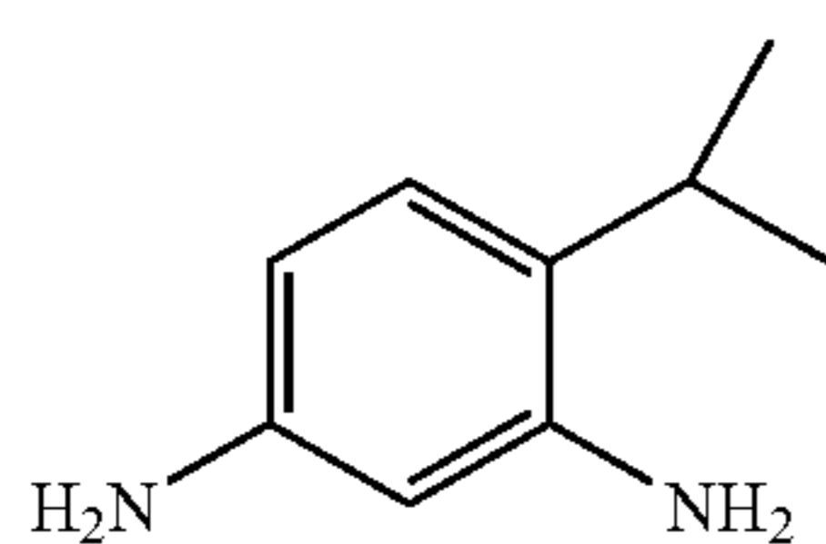
D-8; 4-Isopropylbenzene-1,3-diamine
