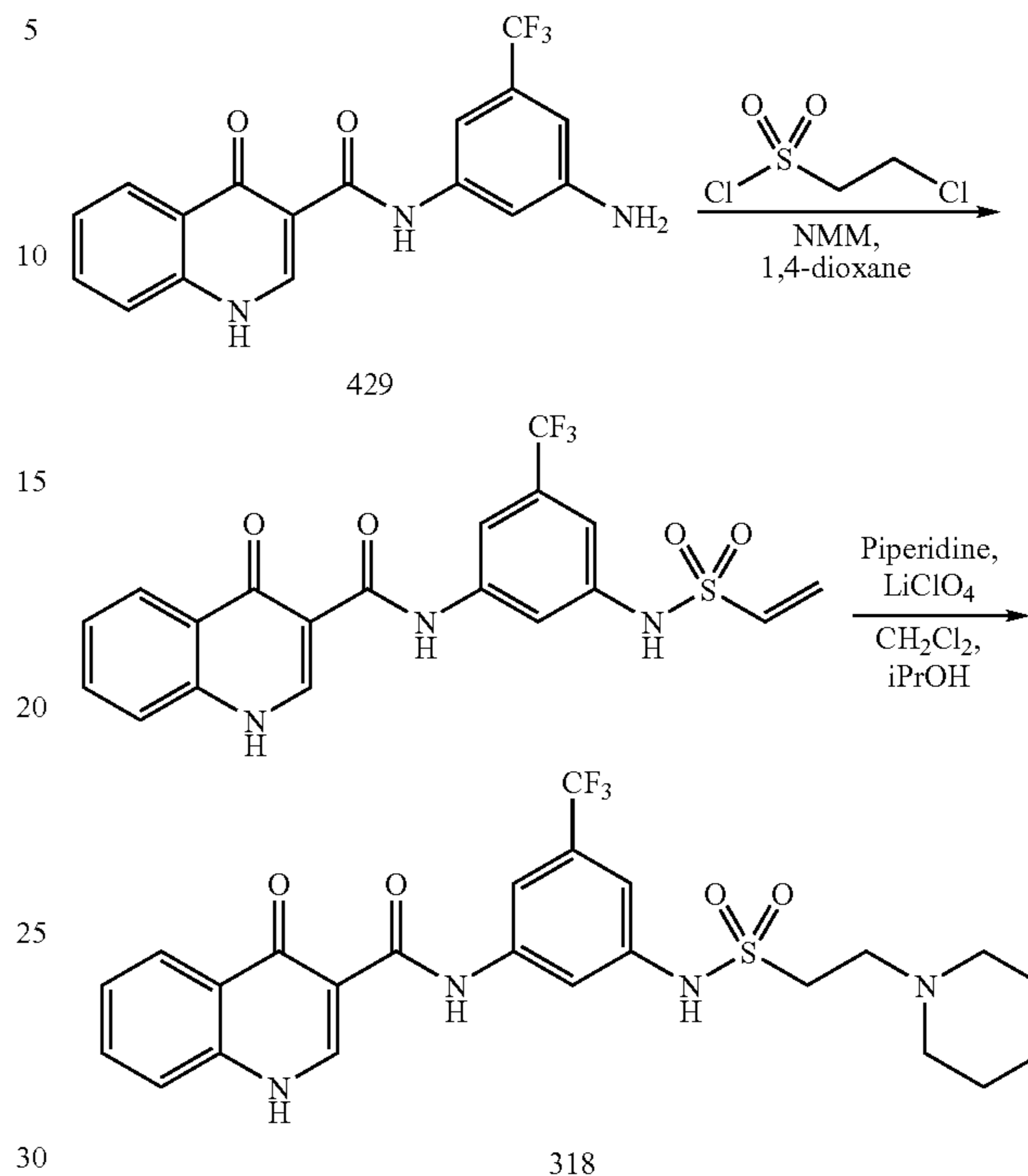
4-Oxo-N-[3-(trifluoromethyl)-5-(vinylsulfonylamino)]phenyl]-1,4-dihydroquinoline-3-carboxamide
