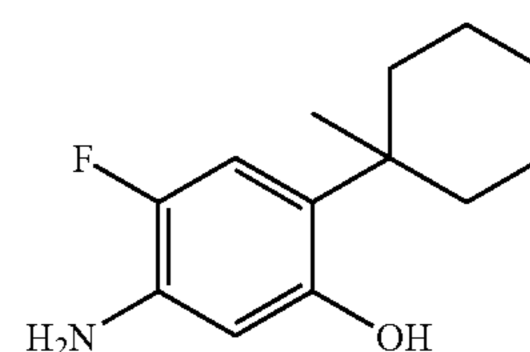
C-13; 5-Amino-4-fluoro-2-(1-methylcyclohexyl)phenol
