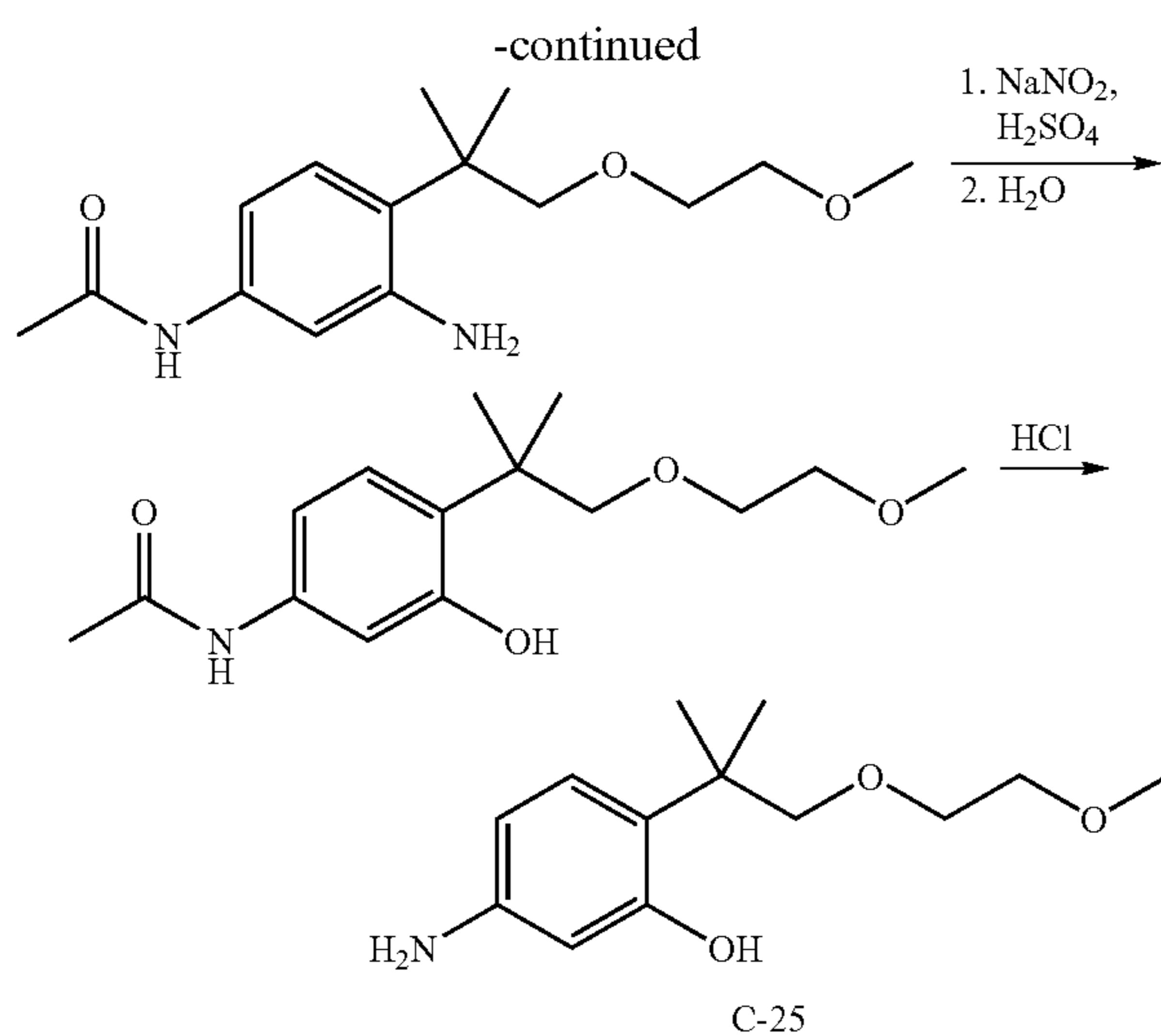
2-Methyl-2-phenyl-propan-1-ol
