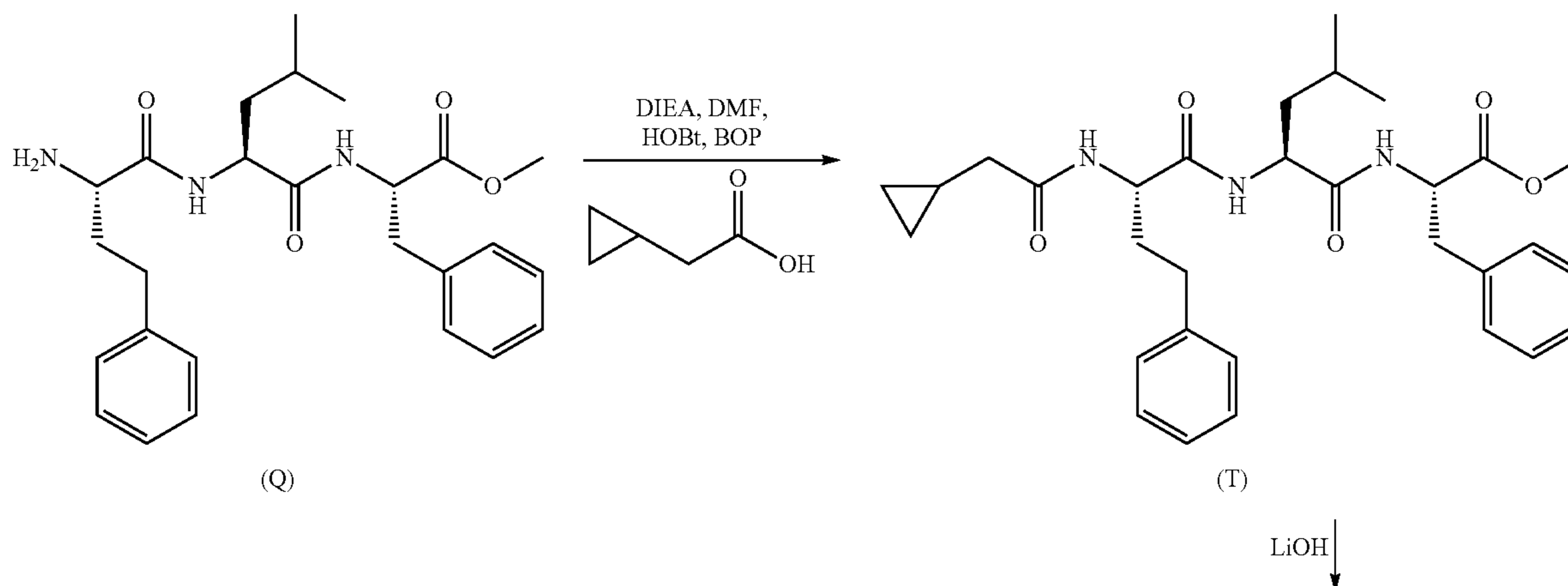
Scheme 5: Synthesis of Example 5
