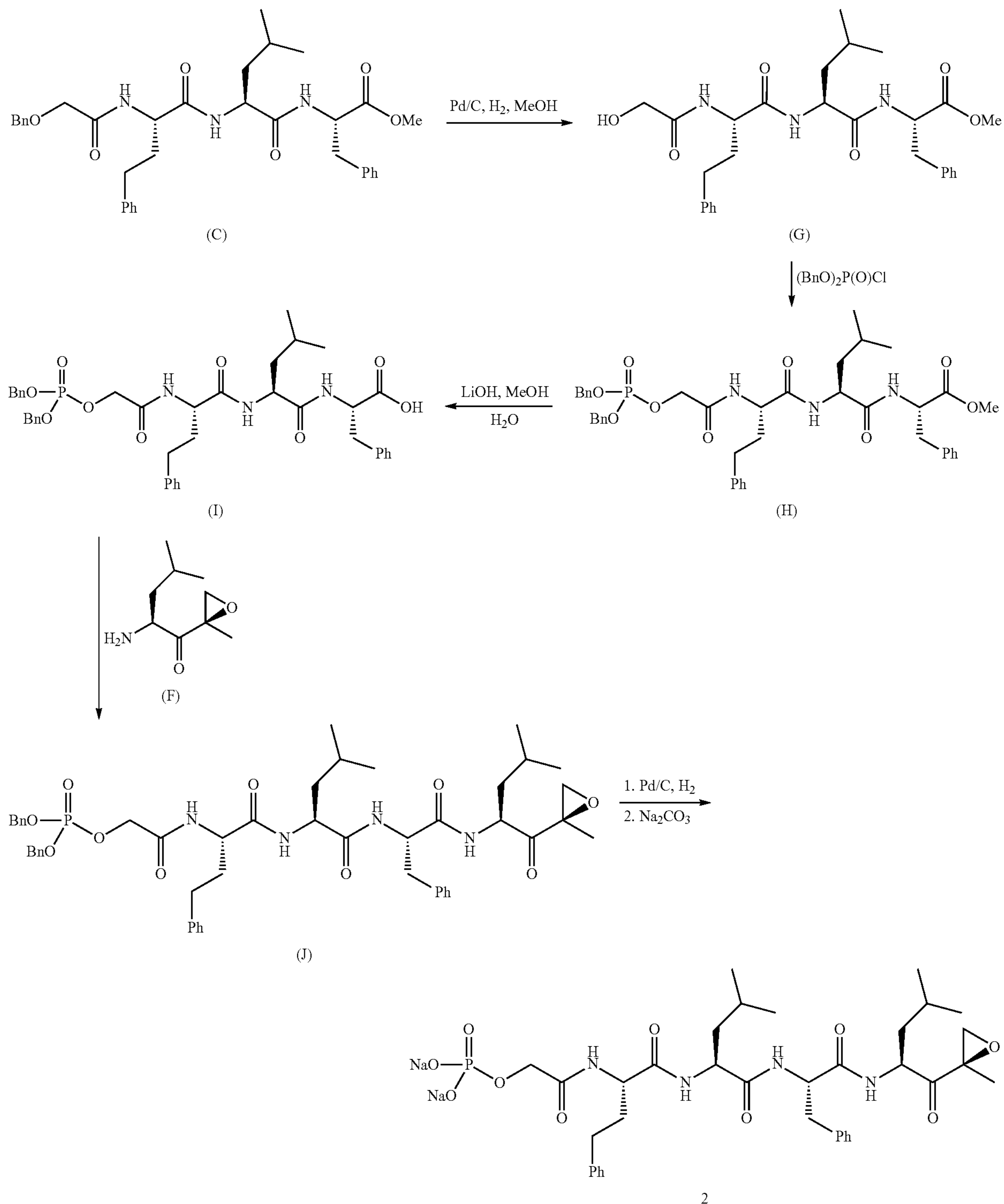
Scheme 2: Synthesis of Example 2
