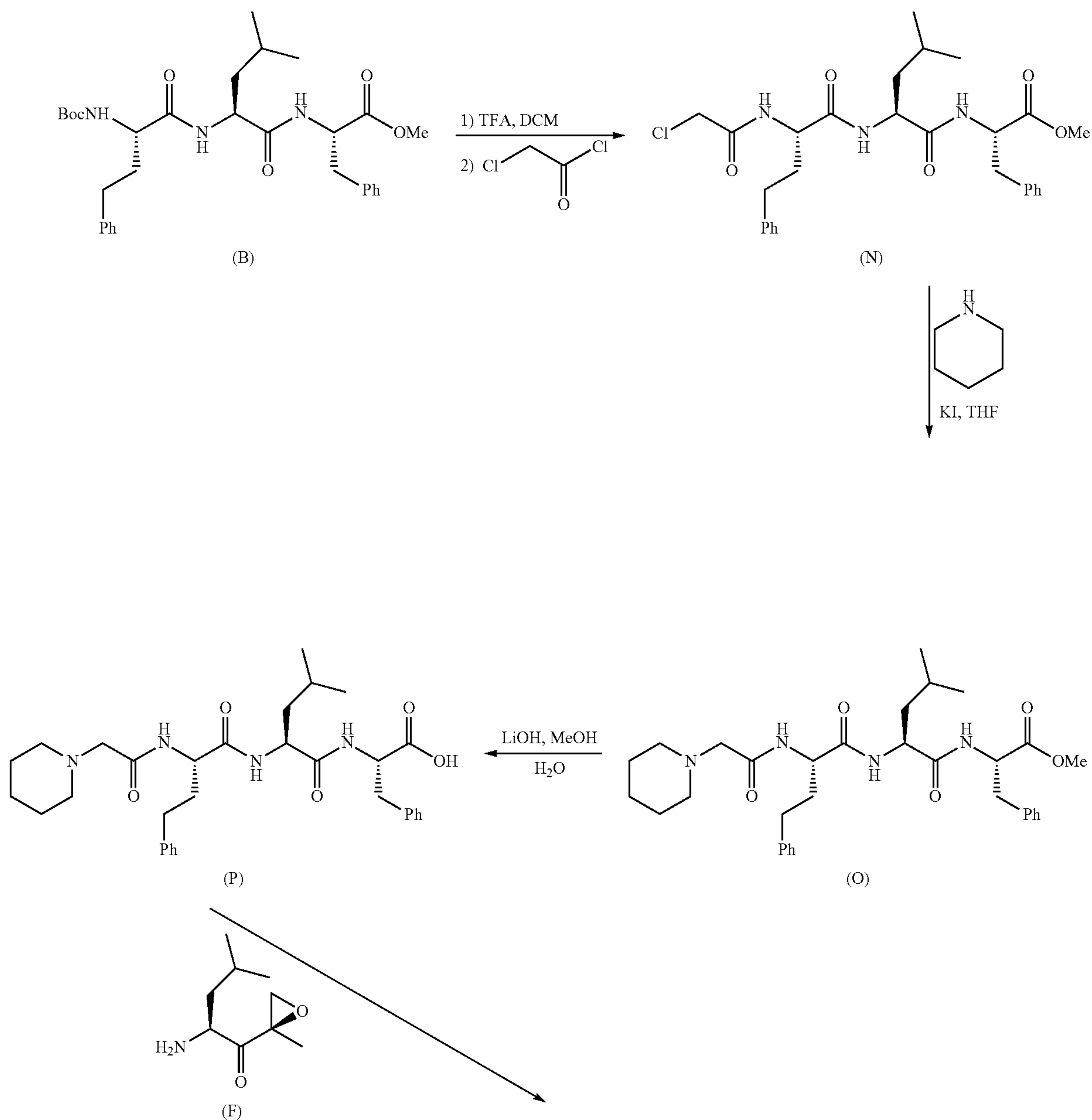
Scheme 4: Synthesis of Example 4
