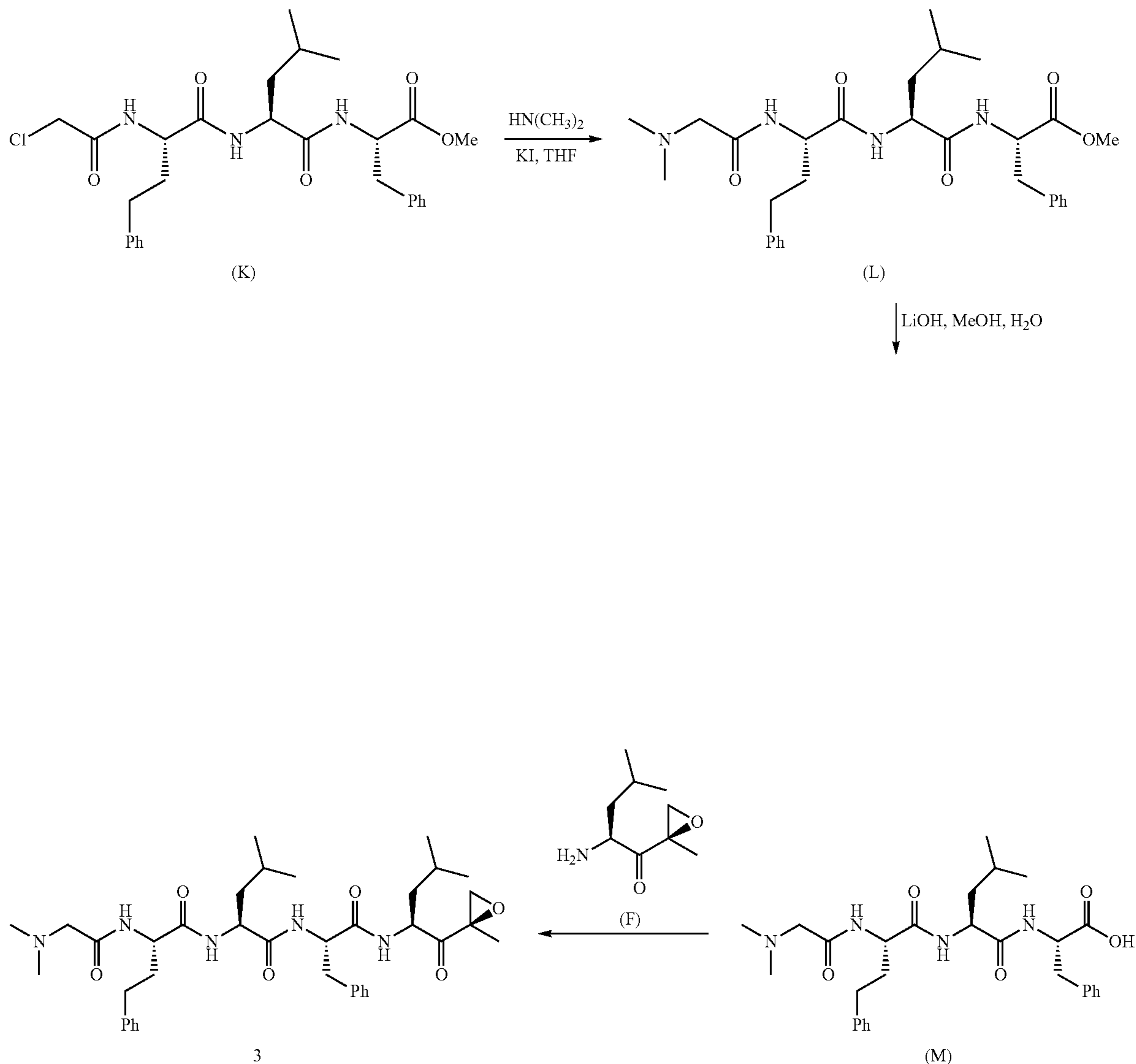
Scheme 3: Synthesis of Example 3
