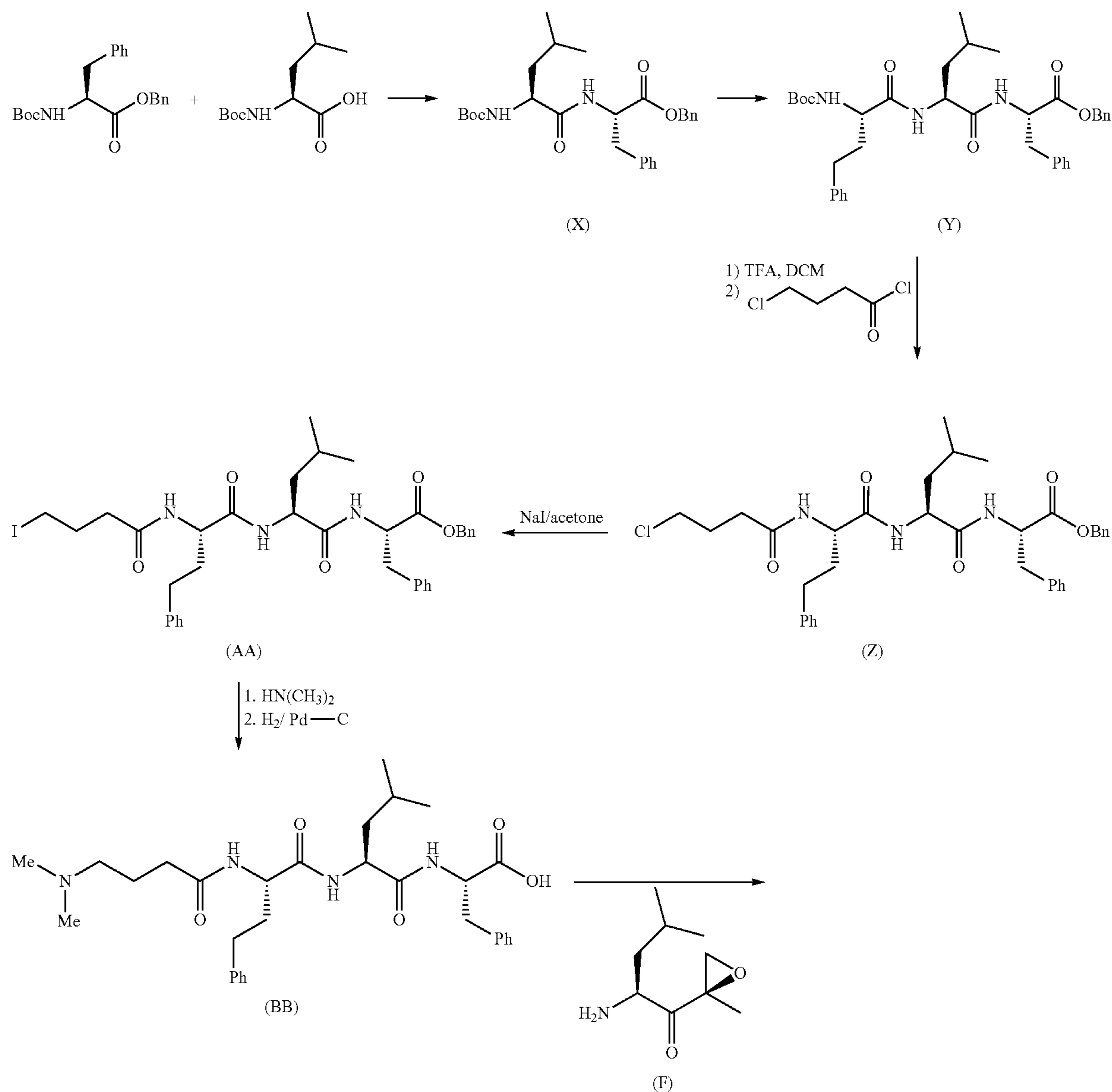
Scheme 7: Synthesis of Example 7
