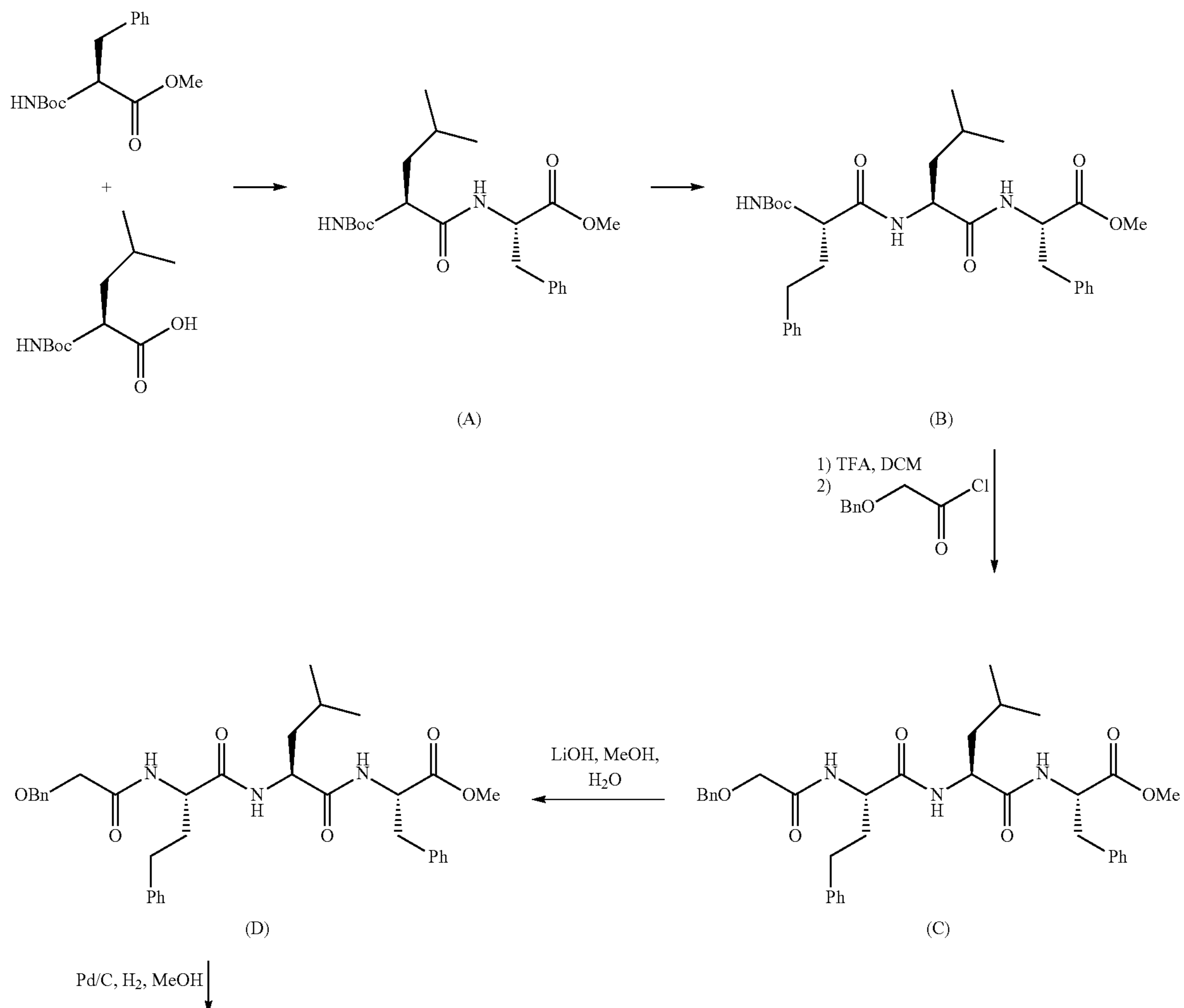
Scheme 1: Synthesis of Example 1
