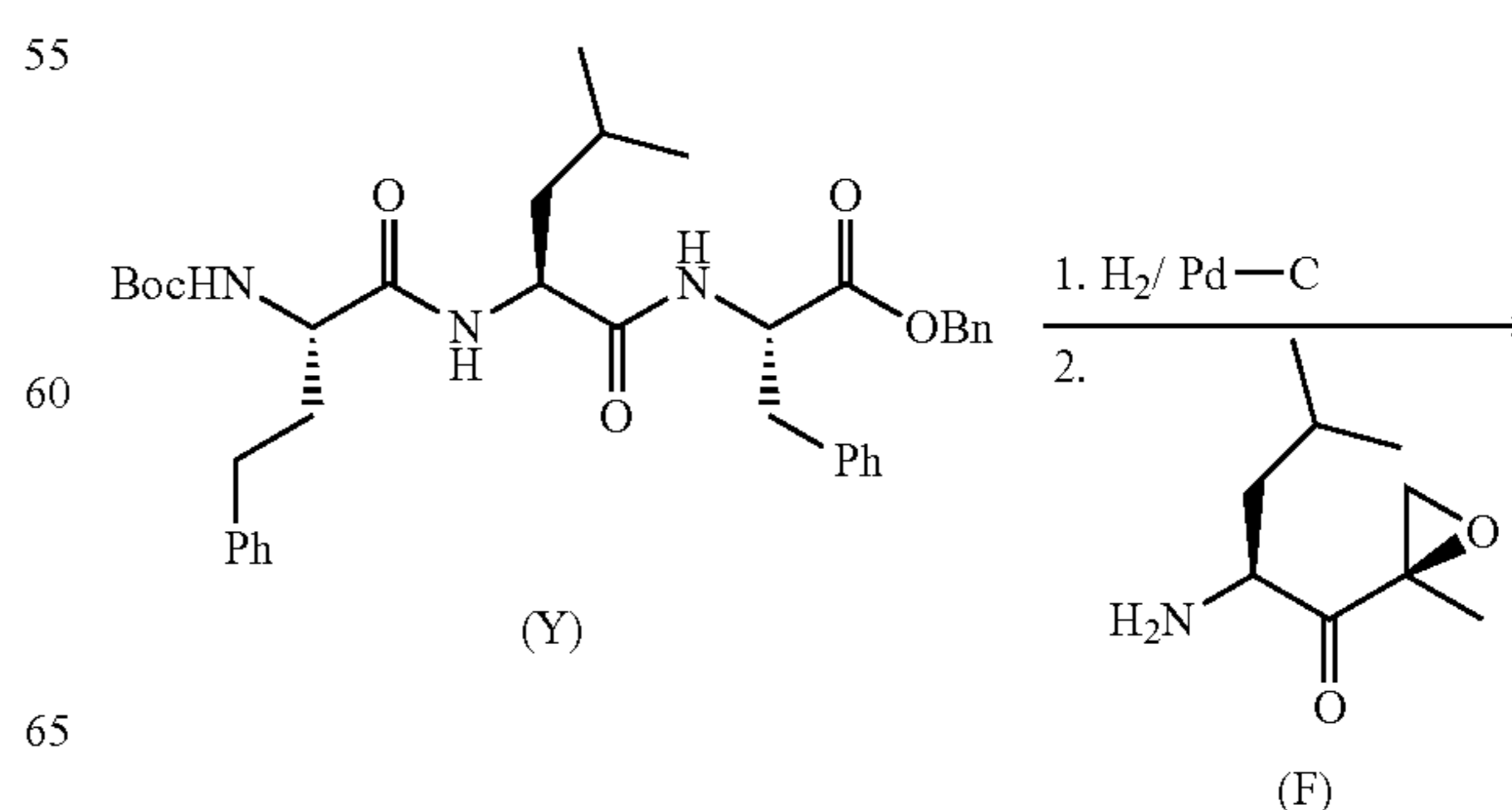
Scheme 8: Synthesis of Example 8
