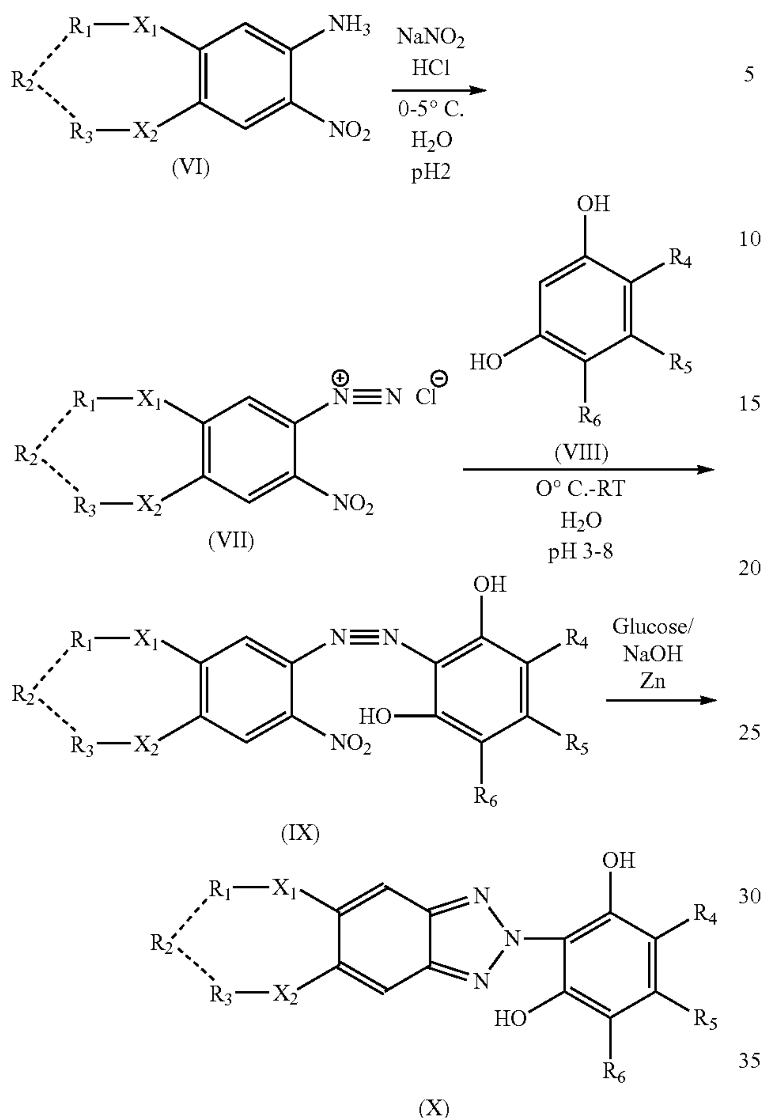
Scheme 1. Generic 2, 6-dihydroxyphenyl-2H-benzotriazole synthesis
