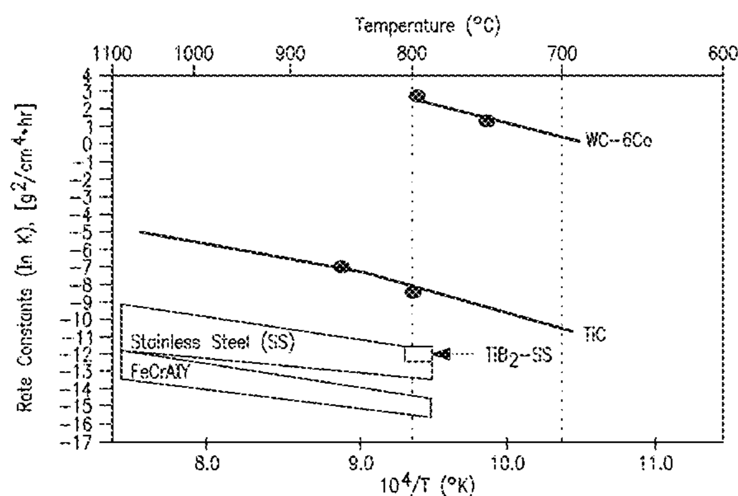
Corrosion Resistance Versus Temperature of Prior Art TiC, FeCrAlY, Stainless Steel (SS) and WC-6Co In Comparison to TiB 2 -SS Cermet of Present Invention (a) and SEM Images of Corrosion Layer Formed on WC-Co Cermet and TiB 2 -SS Cermet (b)
