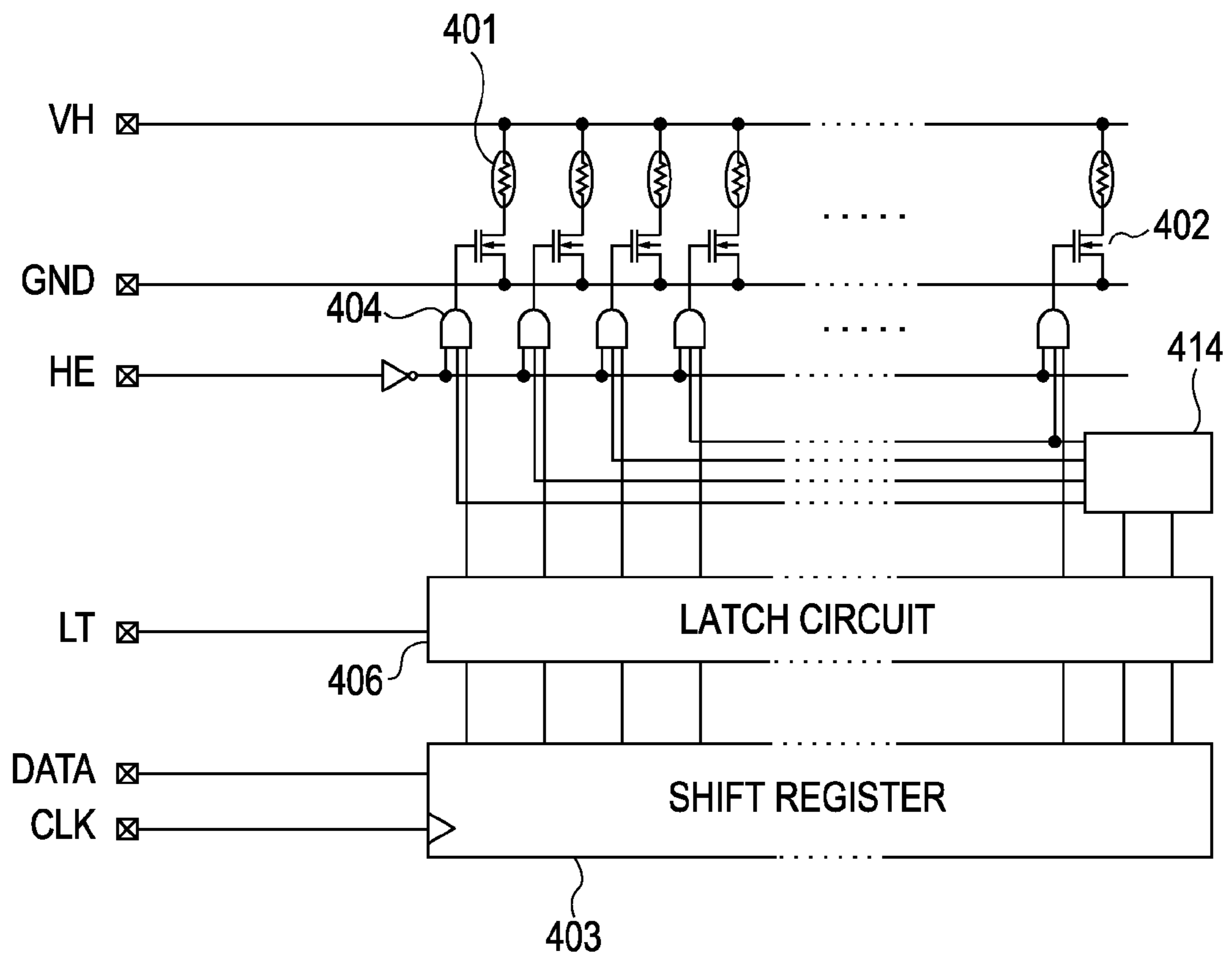
FIG. 9 PRIOR ART
