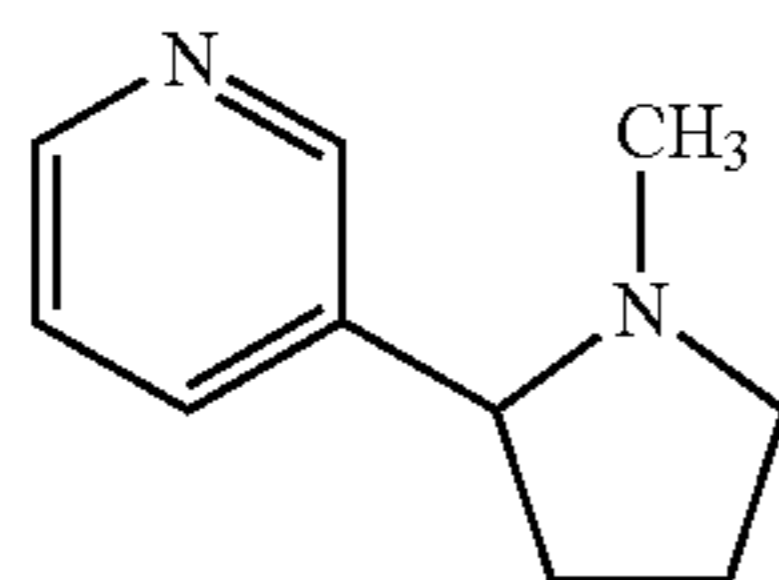
3-(1-methylpyrrolidin-2-yl)pyridine C_{10}H_{14}N_2 Mol. Wt.: 162.23 pK_{a1}=7.84 , pK_{a2}=3.04 at 15^\circ C .
