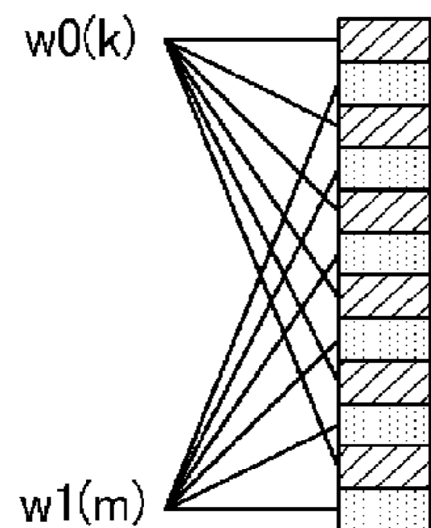
Secondary synchronization channel of slot 0
