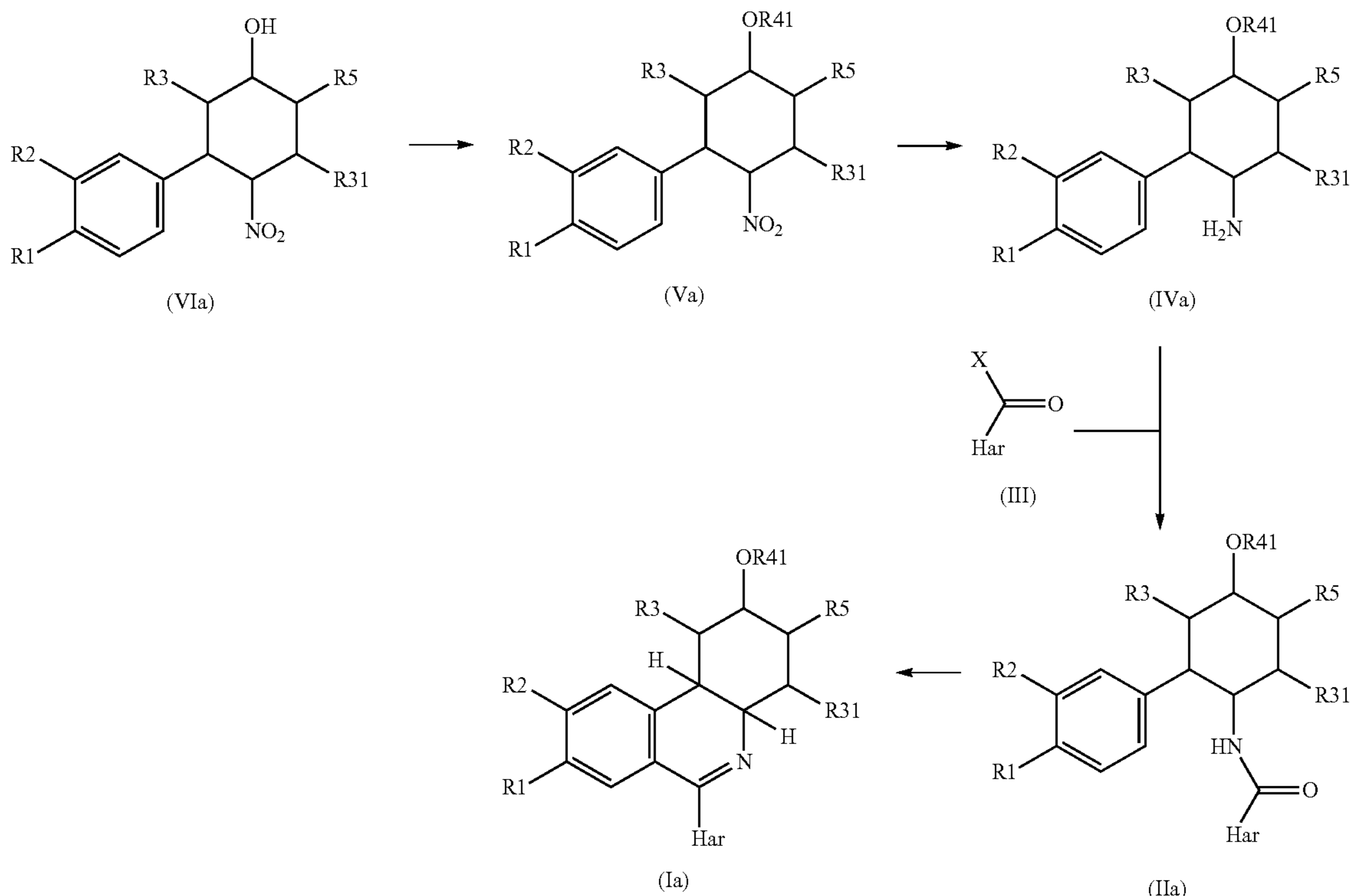
Reaction scheme 1:
