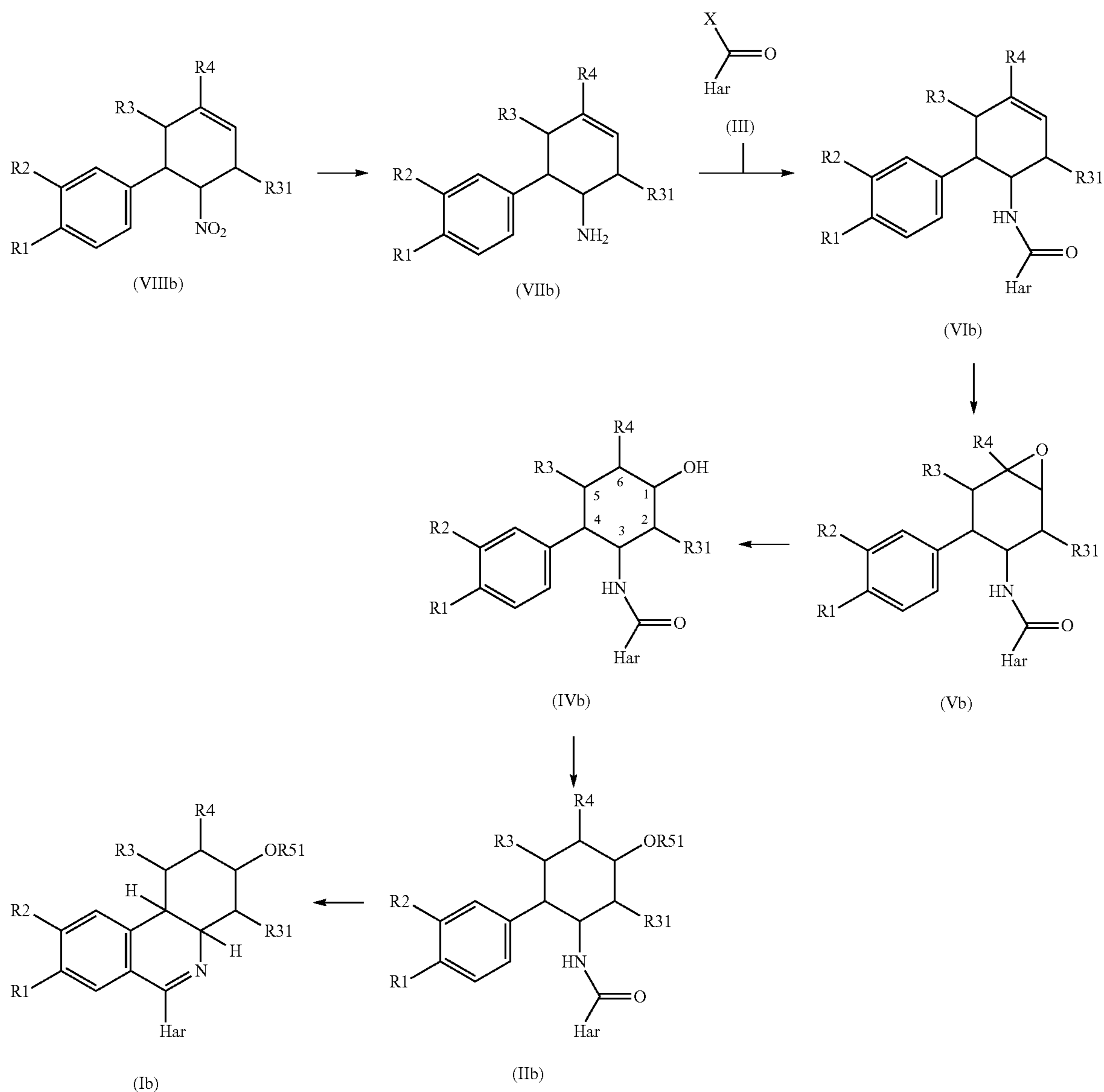
Reaction scheme 3:
