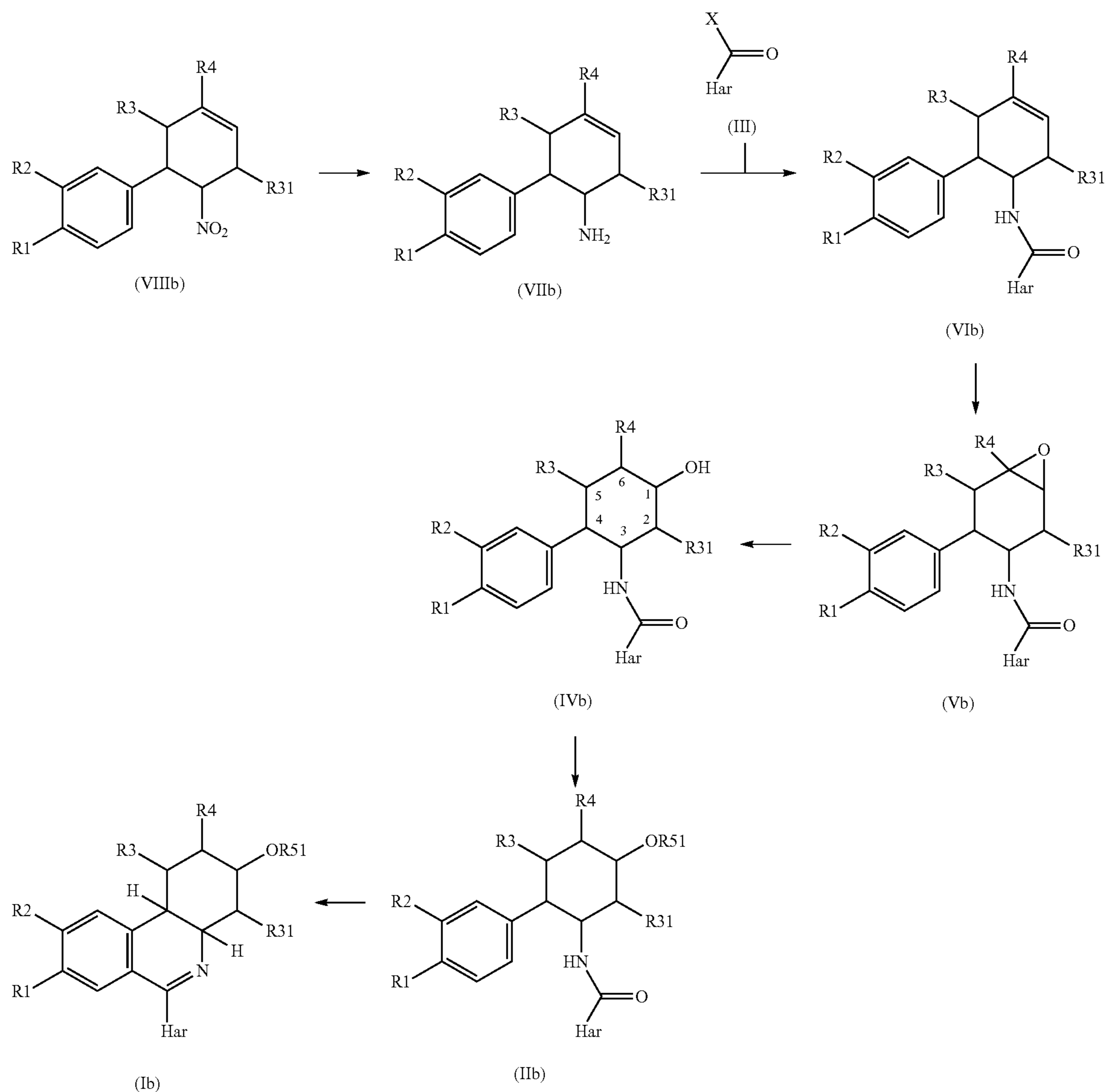
Reaction scheme 3:
