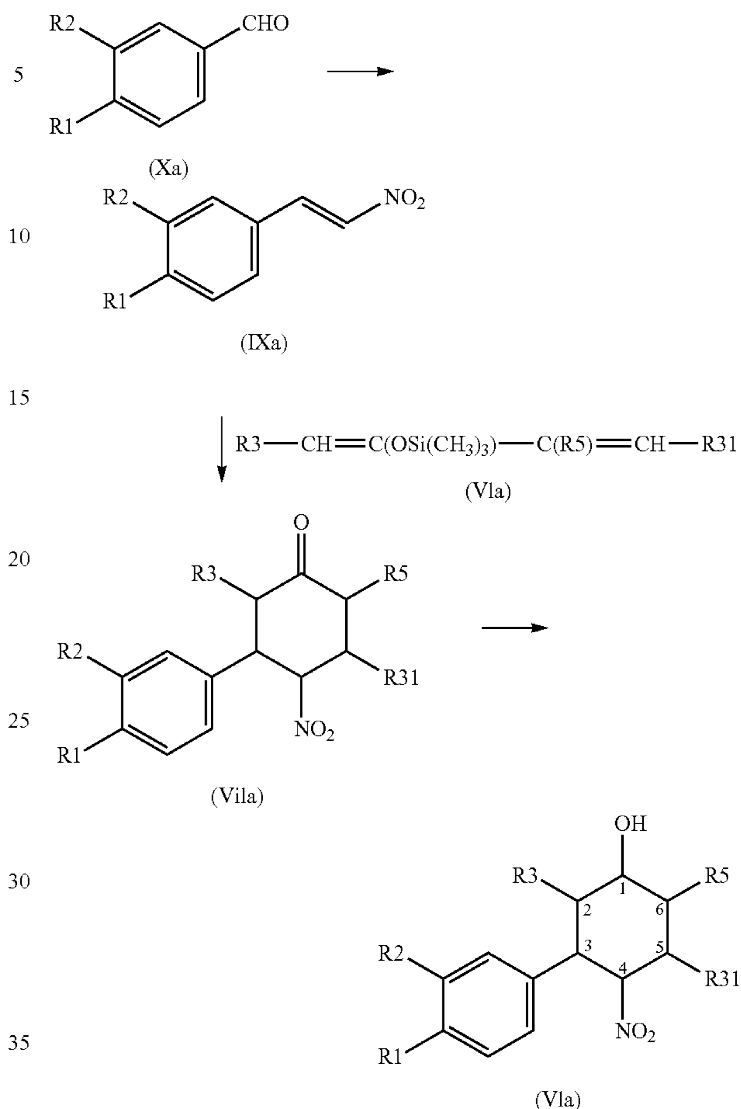
Reaction scheme 2:
