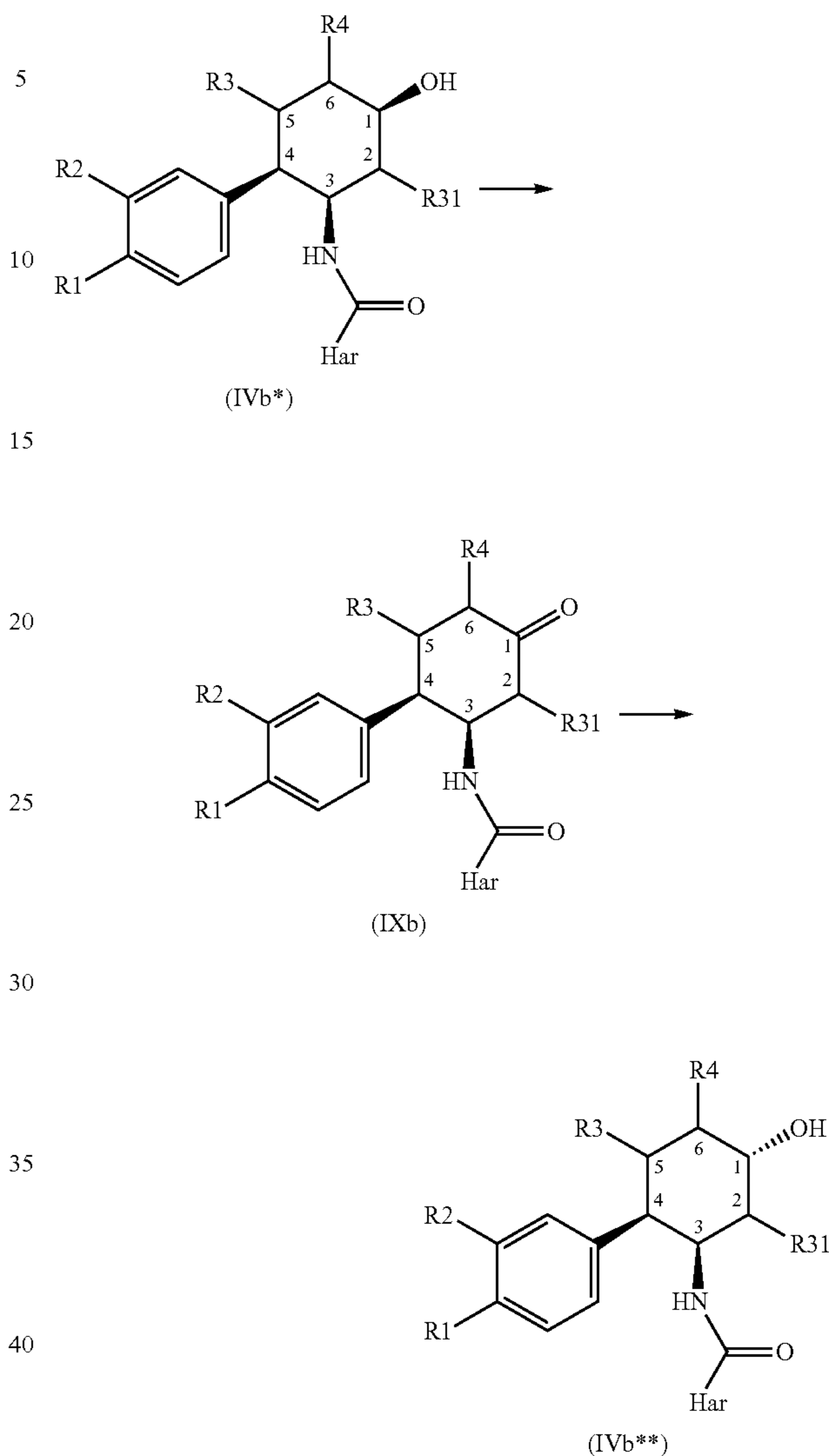
Reaction scheme 4:
