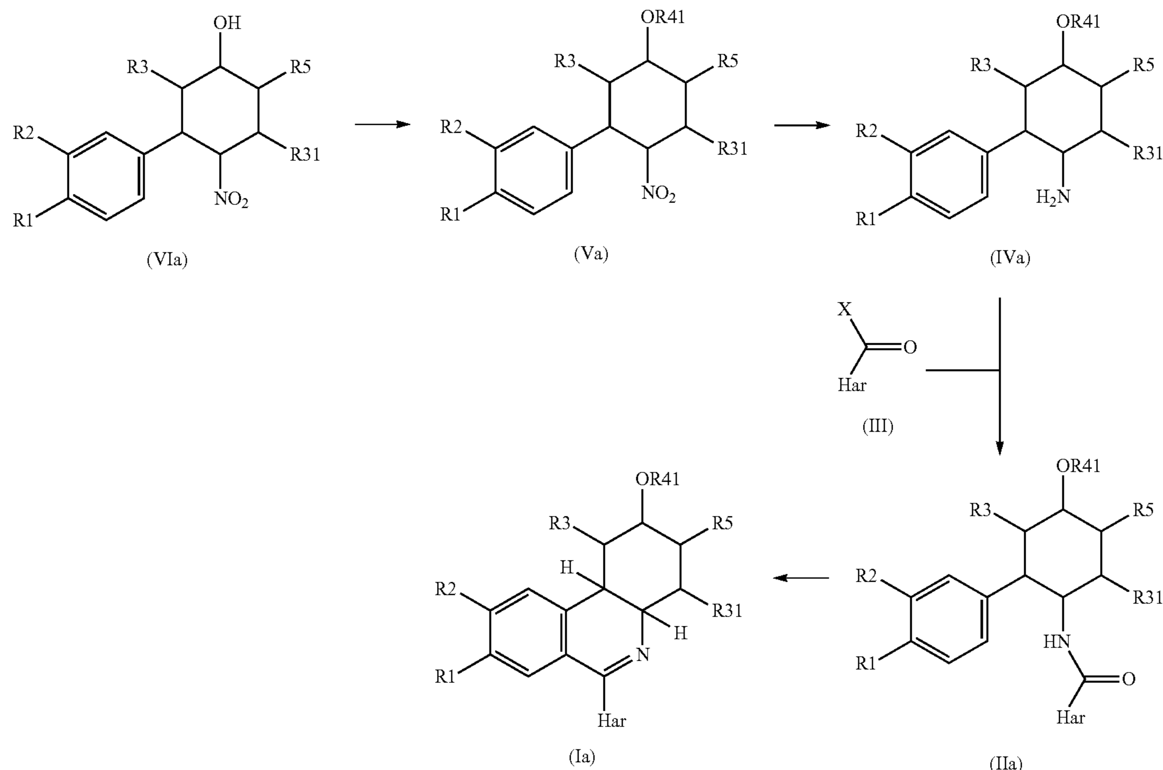
Reaction scheme 1:
