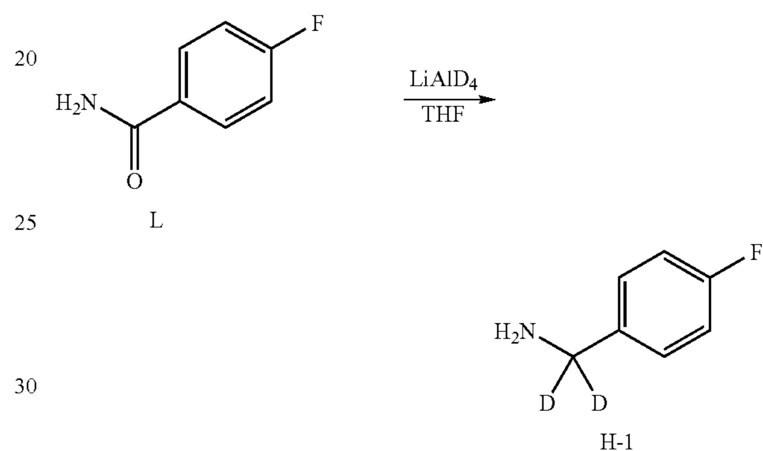
Scheme 2a. Synthesis of Compound H-2
