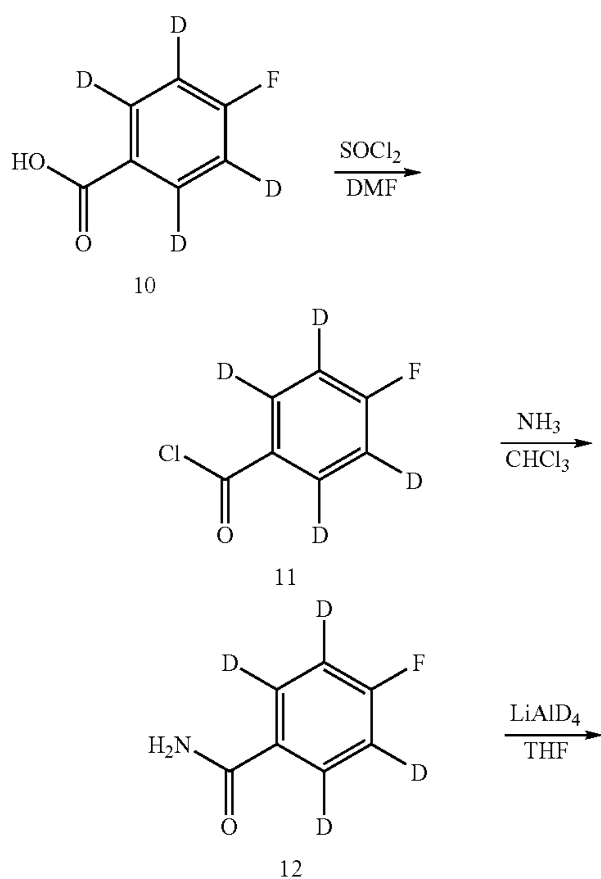
Scheme 4.
