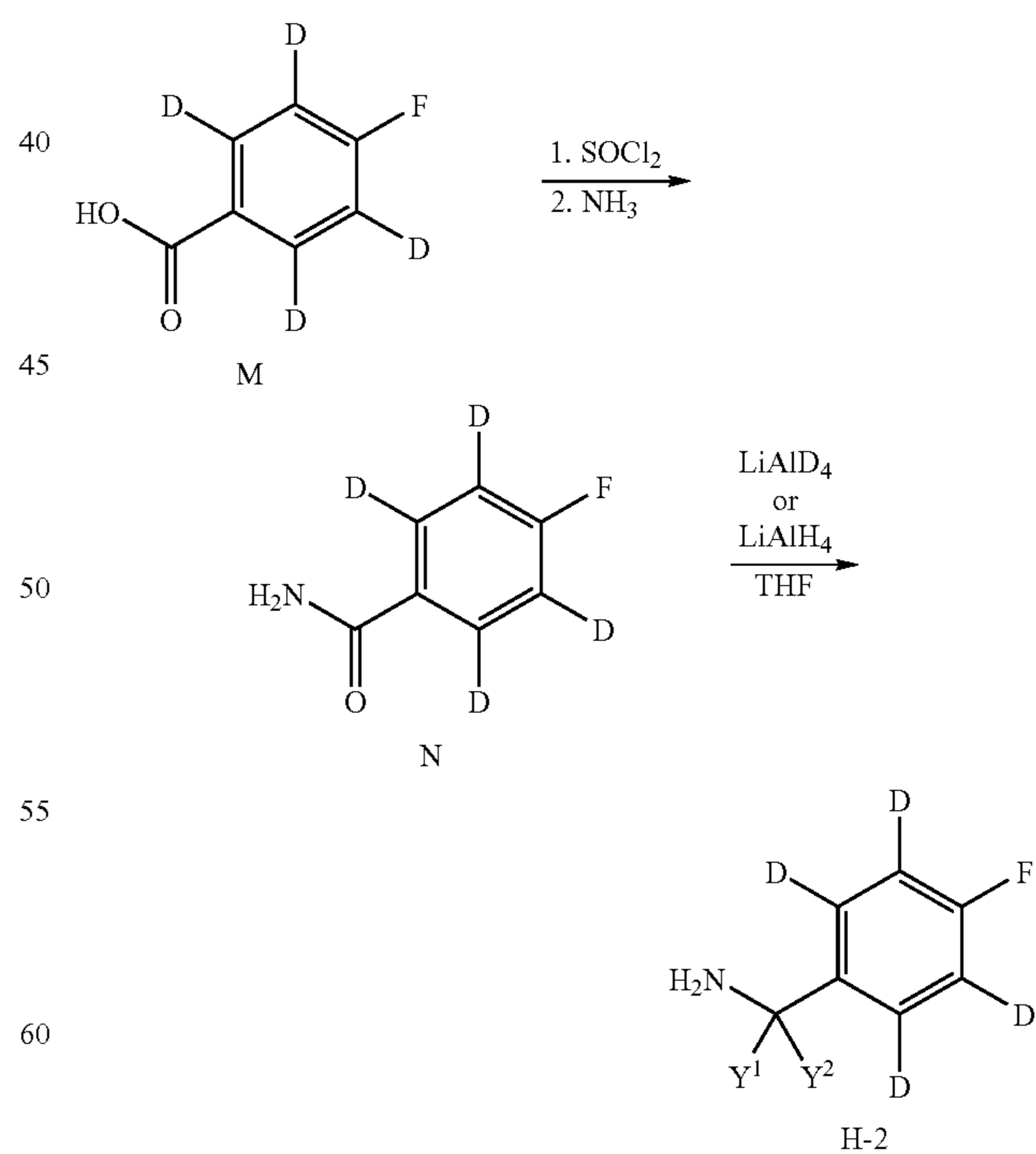
Scheme 2b. Synthesis of Compound H-2.
