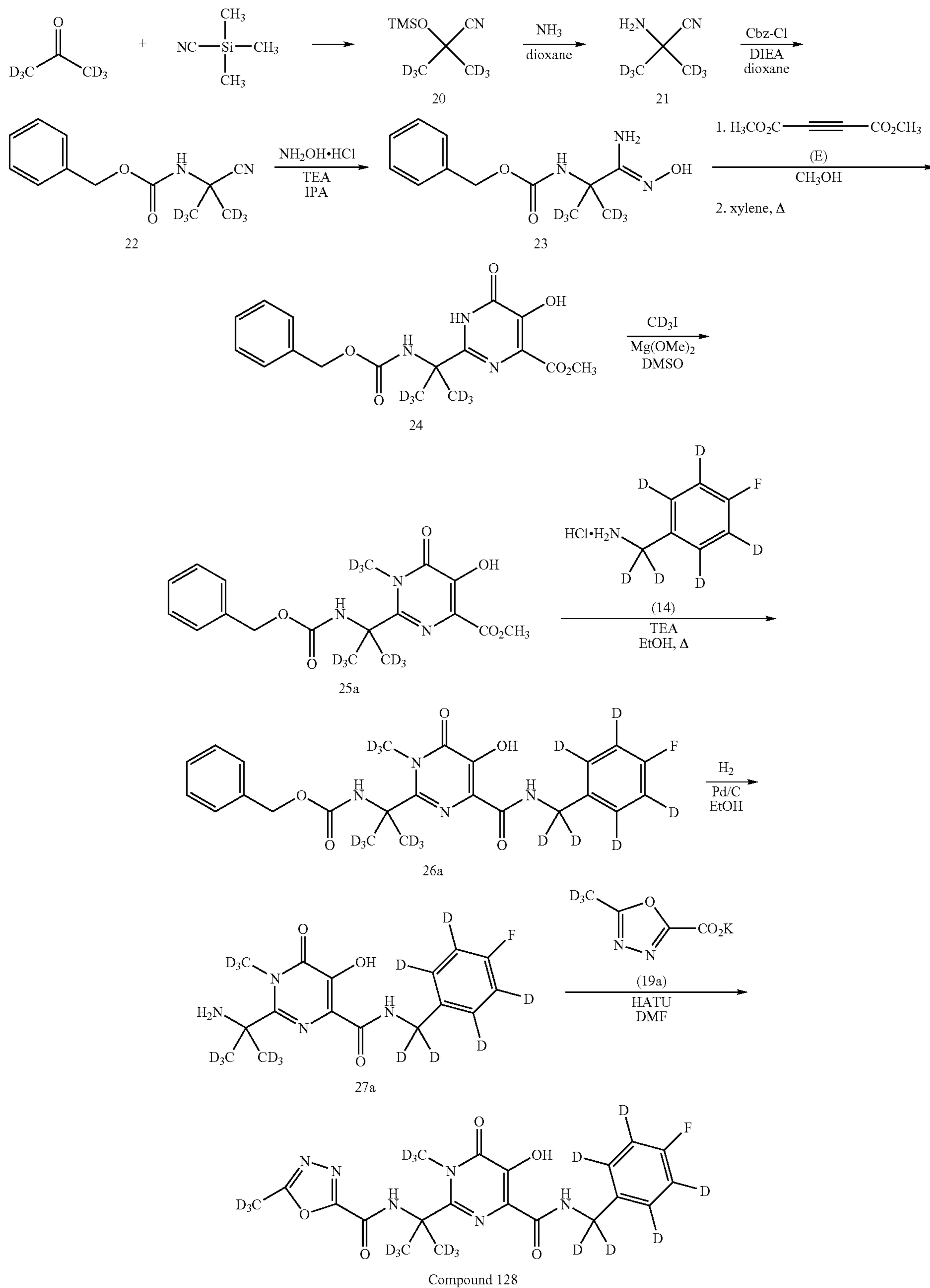
Scheme 6.
