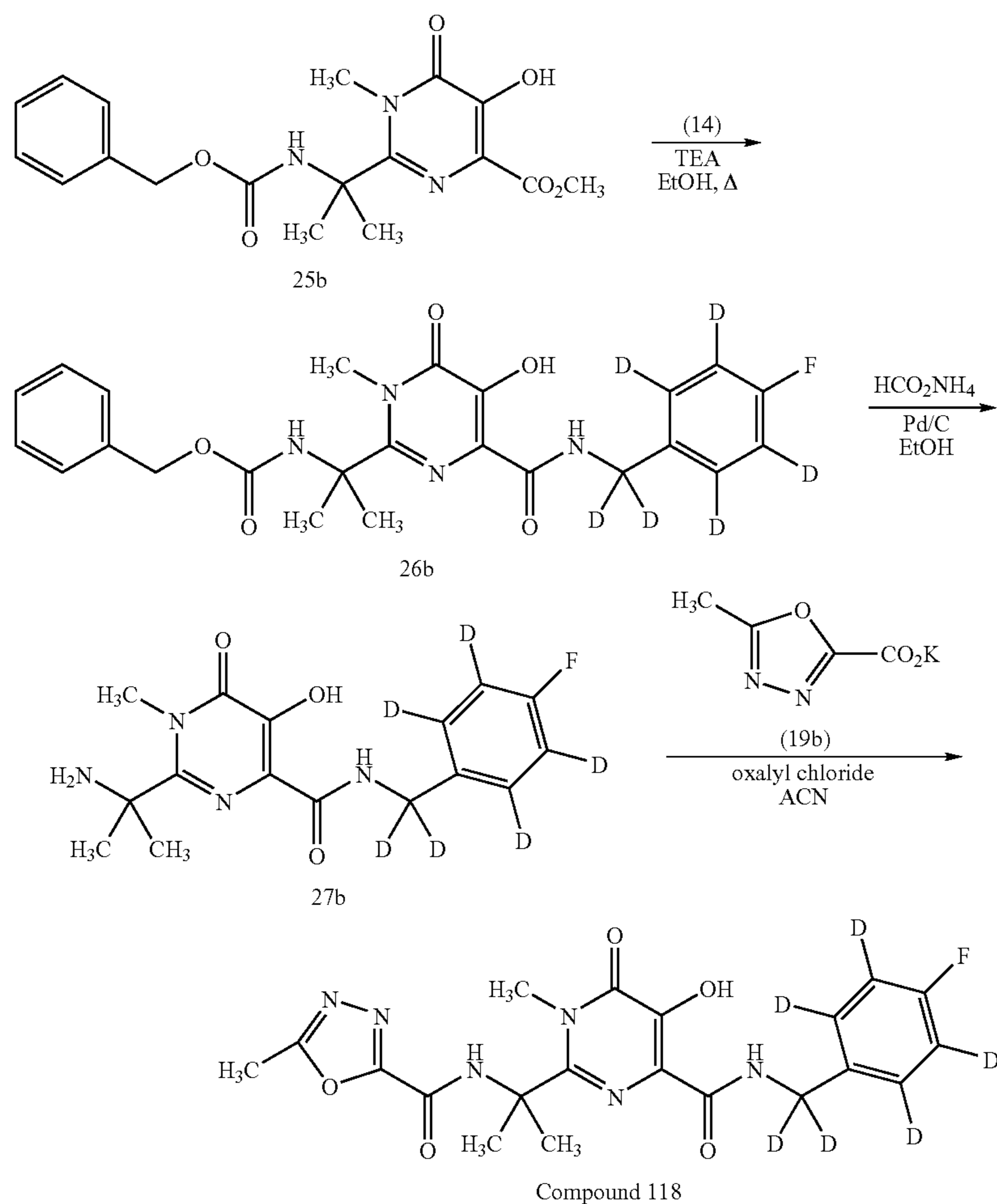
Scheme 7
