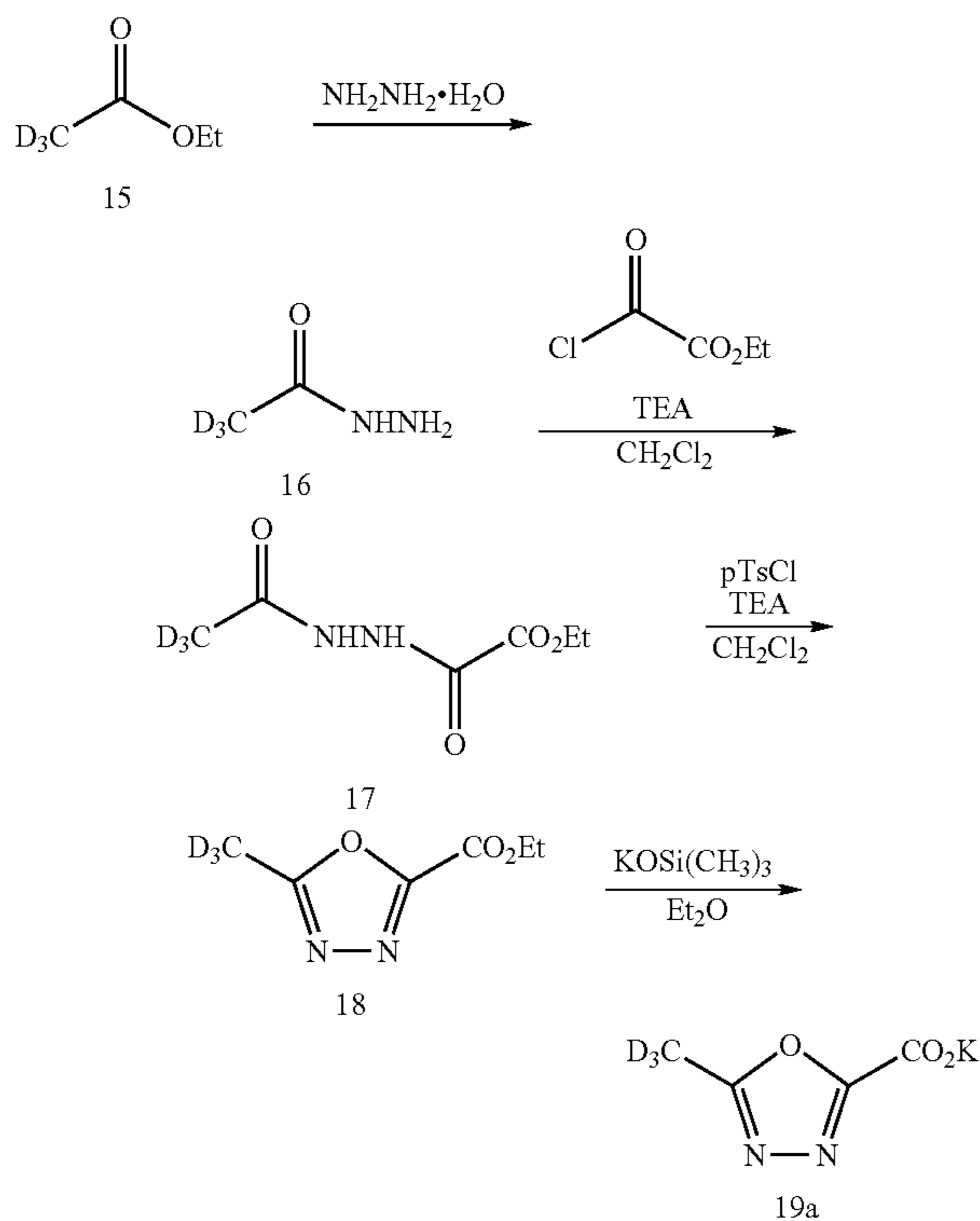
Scheme 5.
