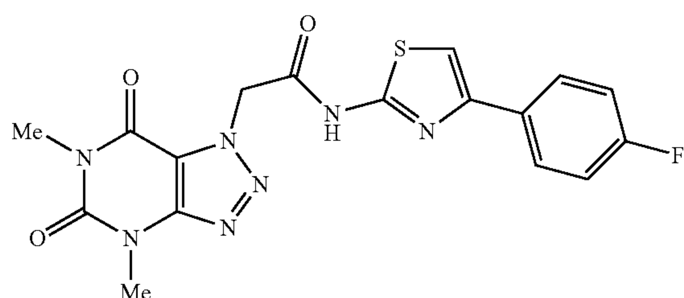
2-(4,6-dimethyl-5,7-dioxo-4,5,6,7-tetrahydro-1H-[1,2,3]triazolo[4,5-d]pyrimidin-1-yl)-N-(4-(4-fluorophenyl)thiazol-2-yl)acetamide
