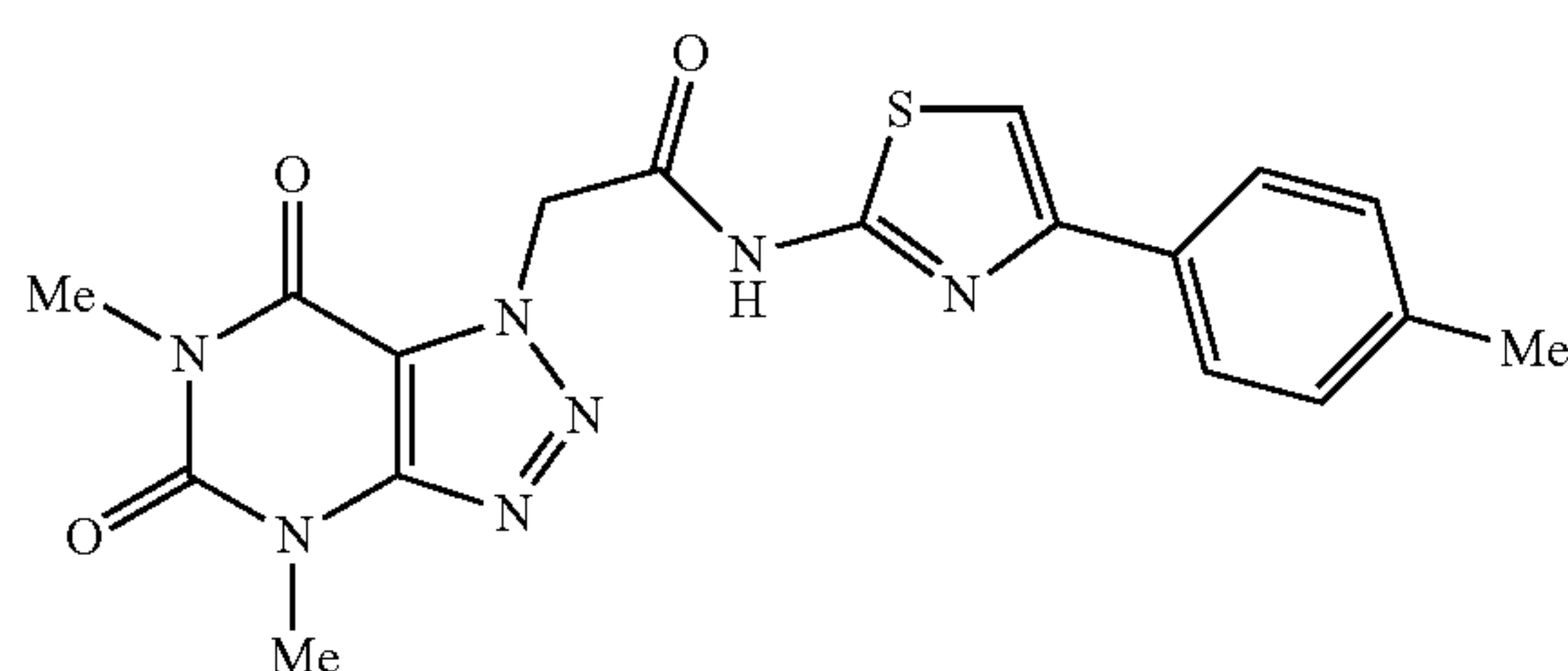
2-(4,6-dimethyl-5,7-dioxo-4,5,6,7-tetrahydro-1H-[1,2,3]triazolo[4,5-d]pyrimidin-1-yl)-N-(4-p-tolylthiazol-2-yl)acetamide
