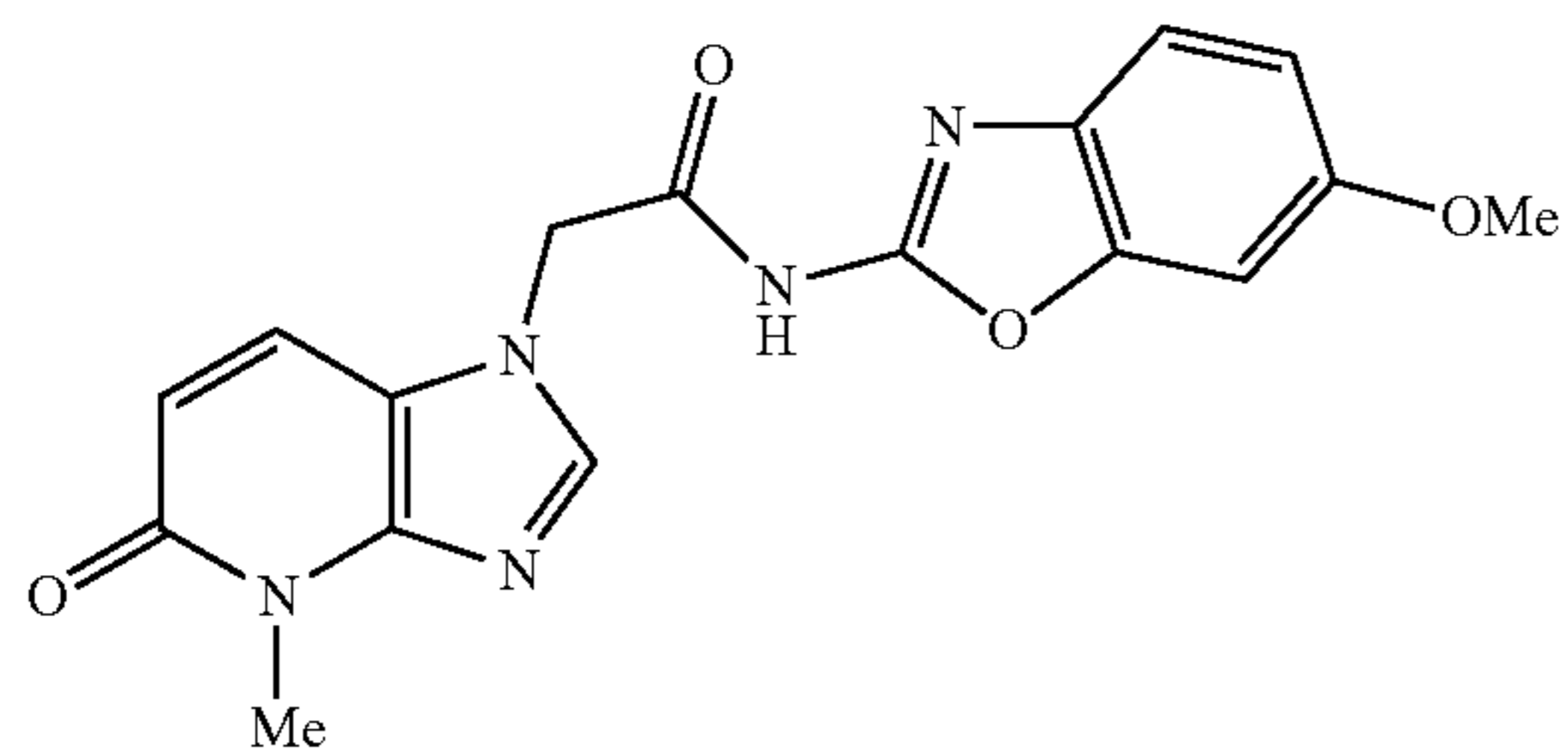
N-(6-methoxybenzo[d]oxazol-2-yl)-2-(4-methyl-5-oxo-4,5-dihydro-1H-imidazo[4,5-b]pyridin-1-yl)acetamide
