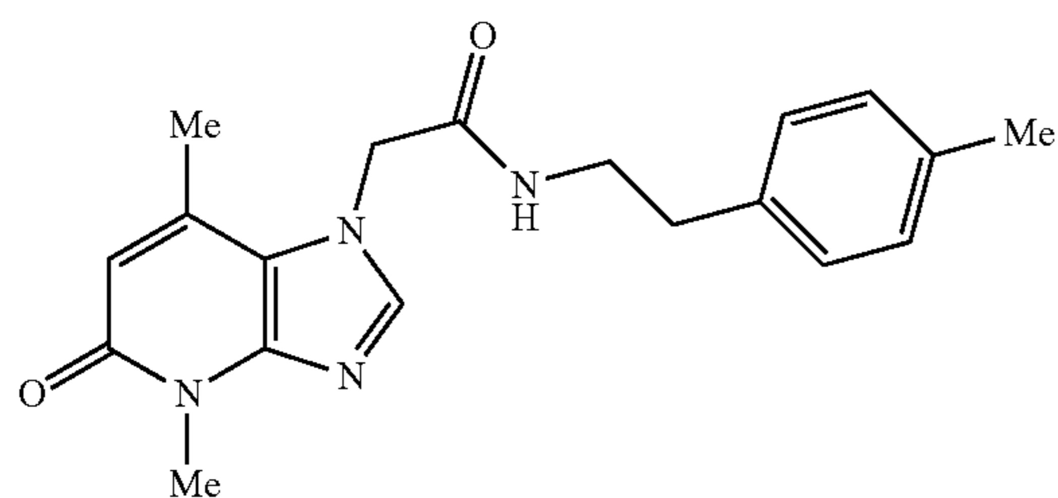
2-(4,7-dimethyl-5-oxo-4,5-dihydro-1H-imidazo[4,5-b]pyridin-1-yl)-N-(4-methylphenethyl)acetamide
