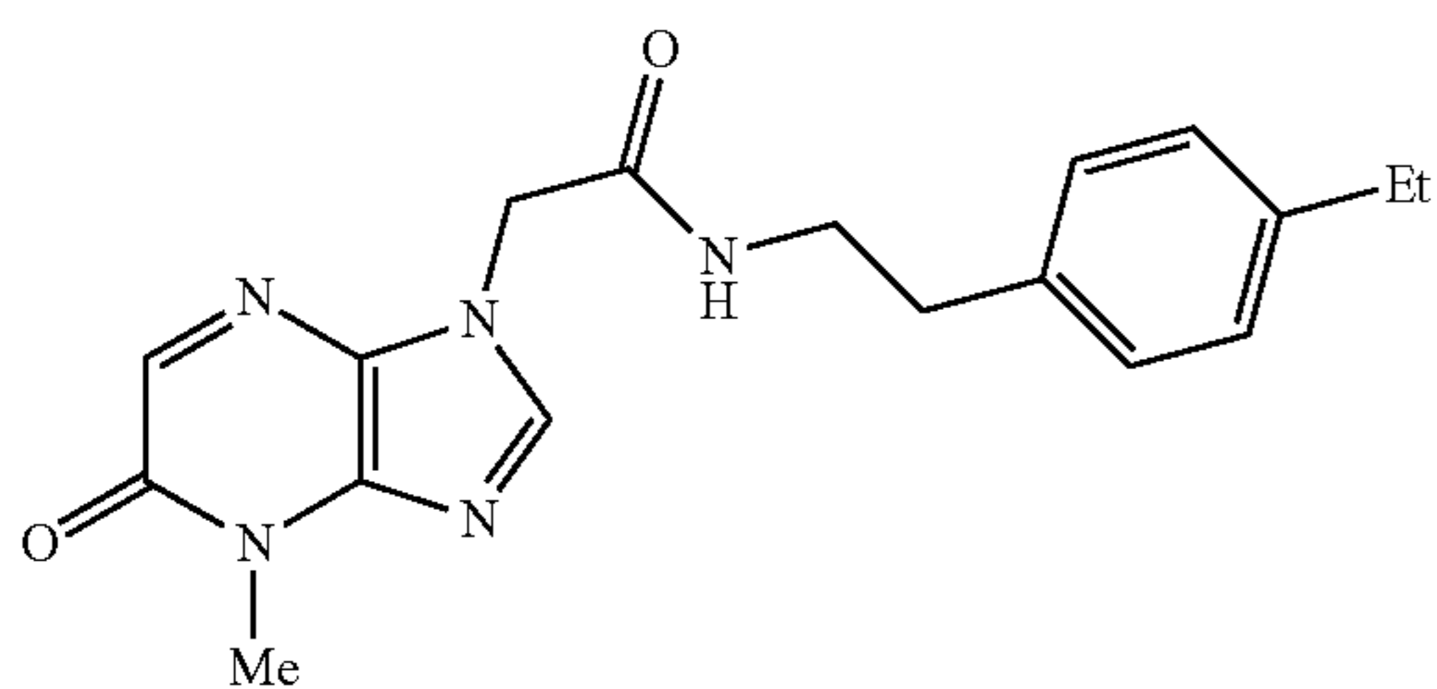
N-(4-ethylphenethyl)-2-(4-methyl-5-oxo-4,5-dihydro-1H-imidazo[4,5-b]pyrazin-1-yl)acetamide
