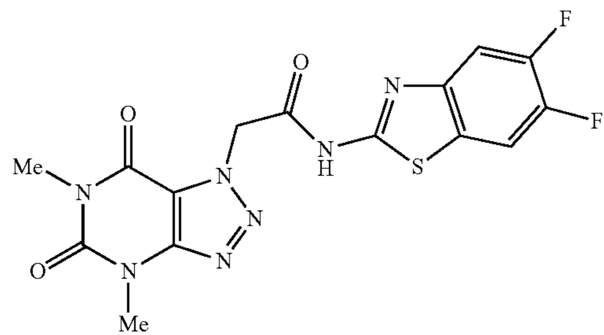
N-(5,6-difluorobenzo[d]thiazol-2-yl)-2-(4,6-dimethyl-5,7-dioxo-4,5,6,7-tetrahydro-1H-[1,2,3]triazolo[4,5-d]pyrimidin-1-yl)acetamide
