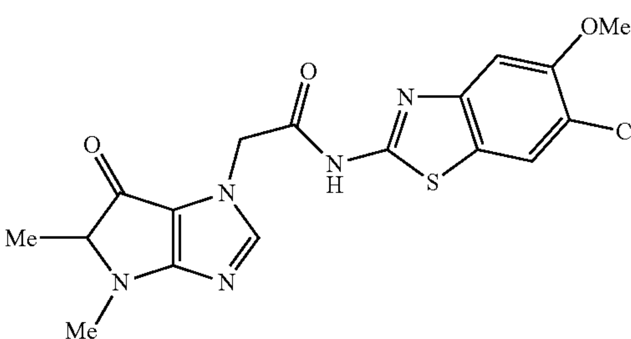
N-(6-chloro-5-methoxybenzo[d]thiazol-2-yl)-2-(4,5-dimethyl-6-oxo-5,6-dihydropyrrolo[3,2-d]imidazol-1(4H)-yl)acetamide
