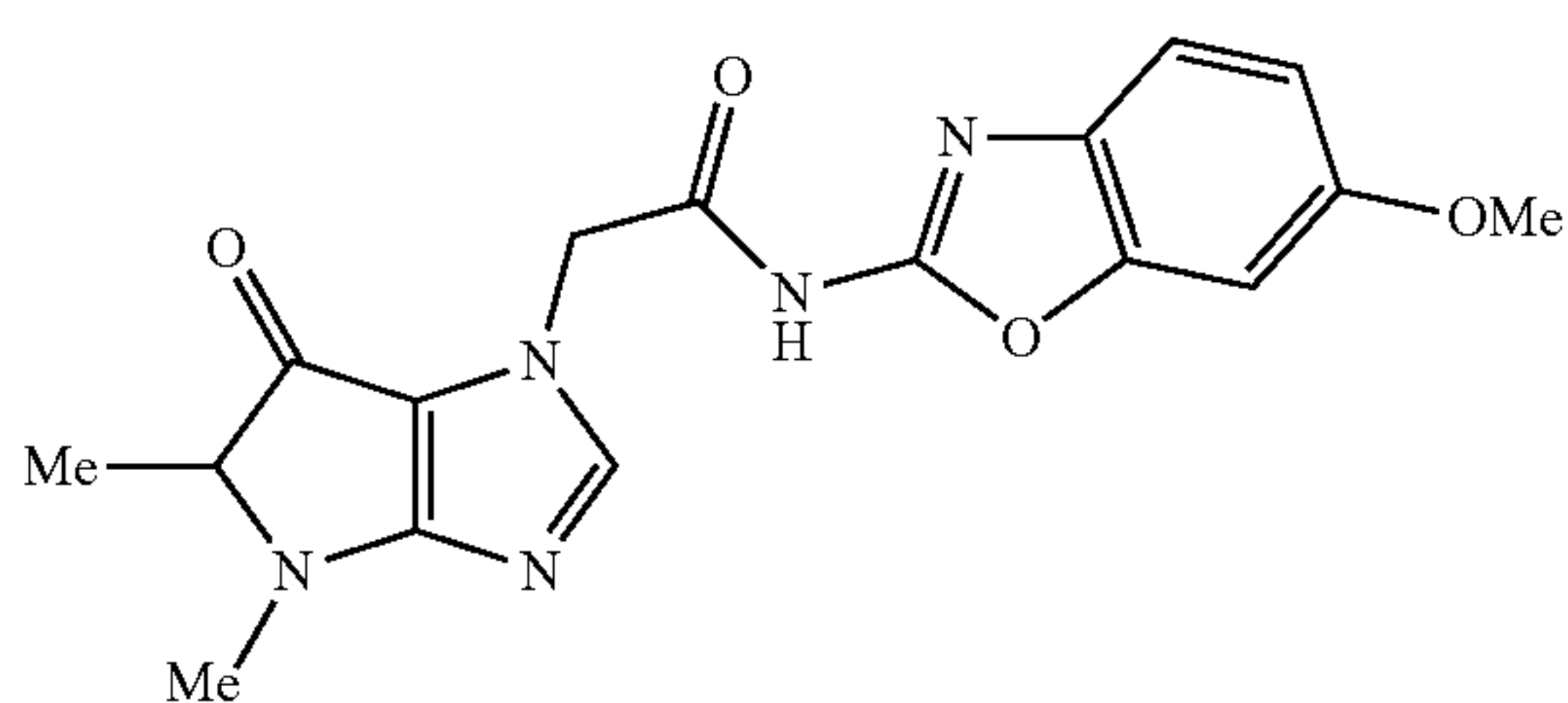
2-(4,5-dimethyl-6-oxo-5,6-dihydropyrrolo[3,2-d]imidazol-1(4H)-yl)-N-(6-methoxybenzo[d]oxazol-2-yl)acetamide
