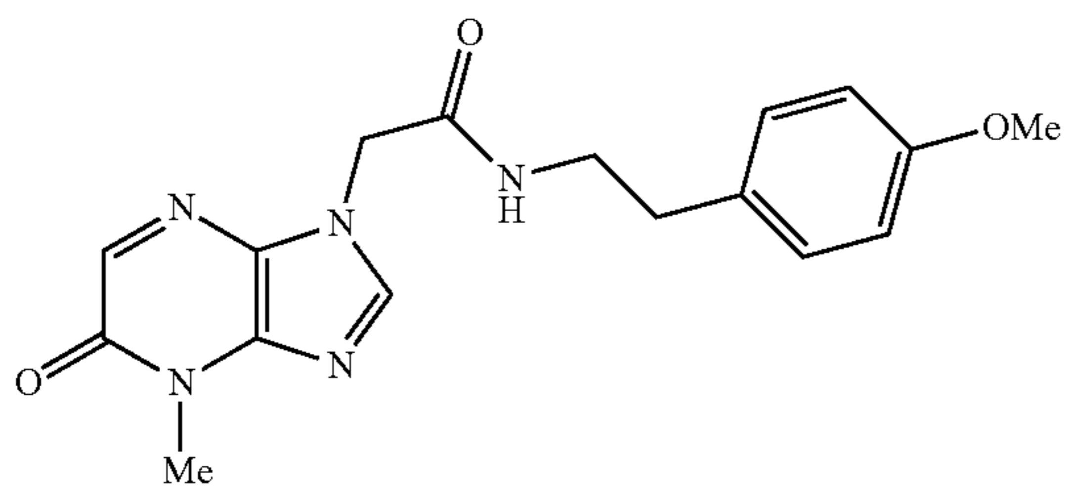
N-(4-methoxyphenethyl)-2-(4-methyl-5-oxo-4,5-dihydro-1H-imidazo[4,5-b]pyrazin-1-yl)acetamide
