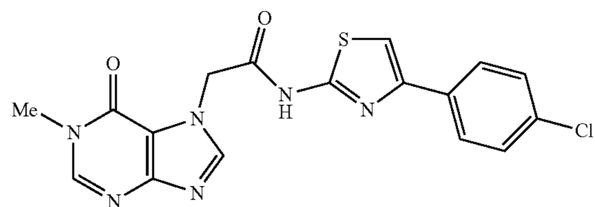
N-(4-(4-chlorophenyl)thiazol-2-yl)-2-(1-methyl-6-oxo-1H-purin-7(6H)-yl)acetamide
