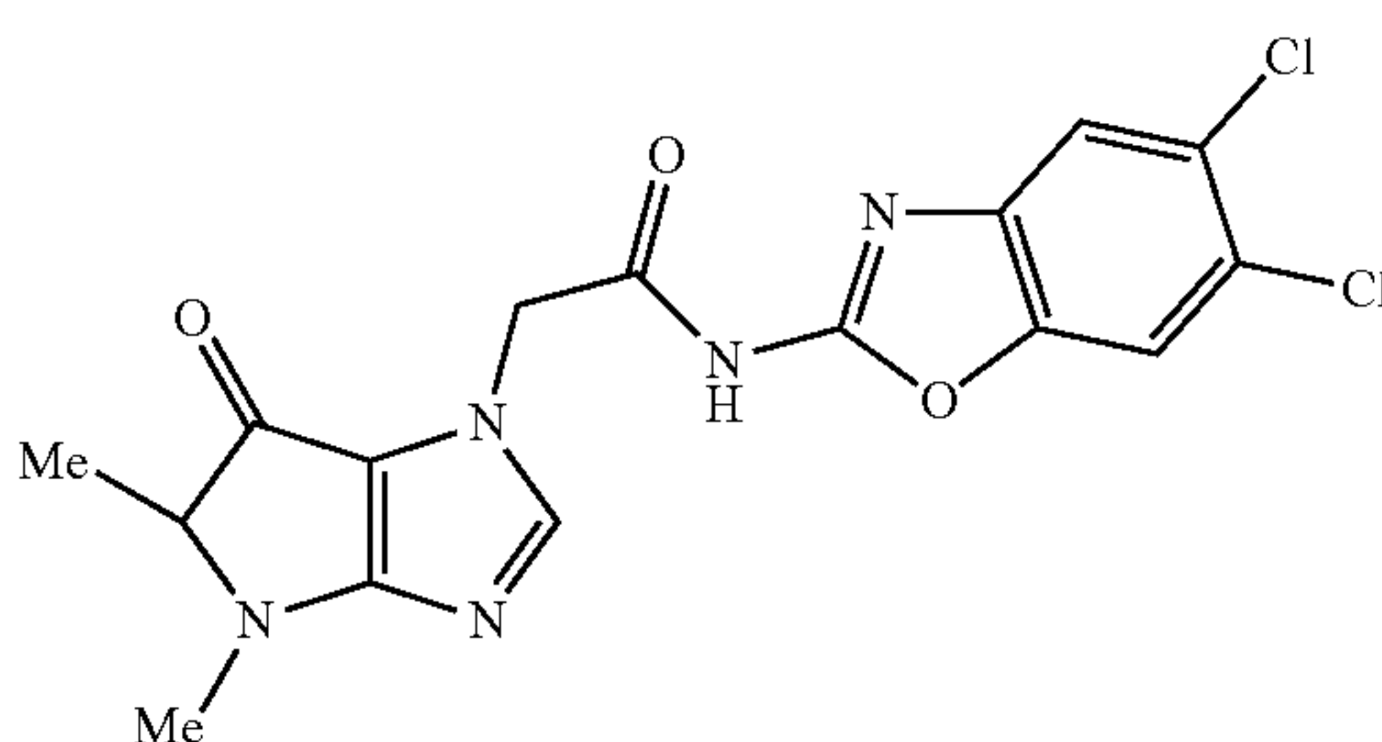
N-(5,6-dichlorobenzo[d]oxazol-2-yl)-2-(4,5-dimethyl-6-oxo-5,6-dihydropyrrolo[3,2-d]imidazol-1(4H)-yl)acetamide
