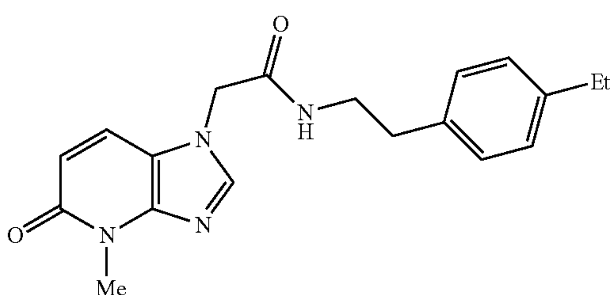
N-(4-ethylphenethyl)-2-(4-methyl-5-oxo-4,5-dihydro-1H-imidazo[4,5-b]pyridin-1-yl)acetamide
