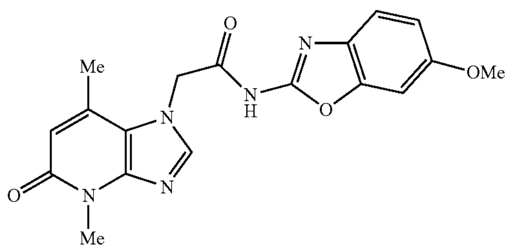
2-(4,7-dimethyl-5-oxo-4,5-dihydro-1H-imidazo[4,5-b]pyridin-1-yl)-N-(6-methoxybenzo[d]oxazol-2-yl)acetamide
