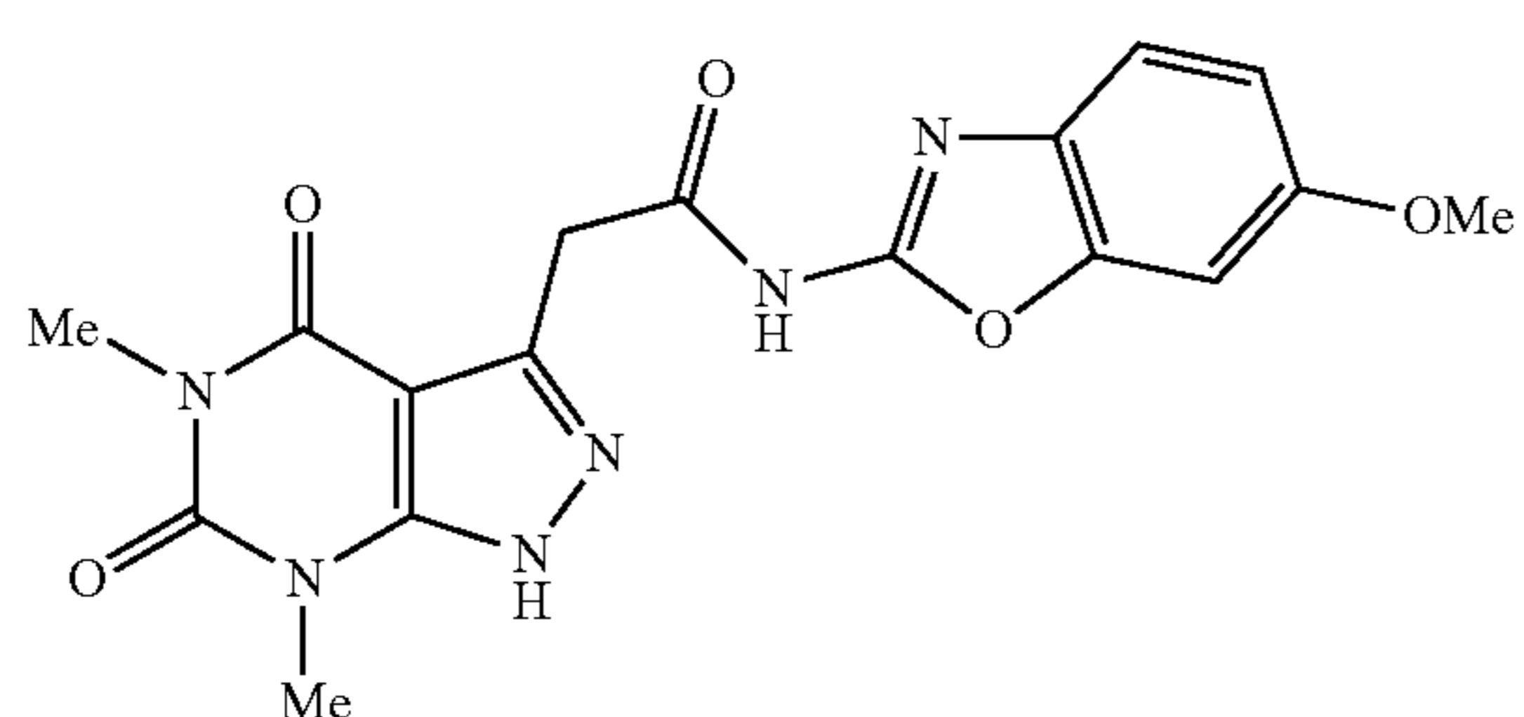
2-(5,7-dimethyl-4,6-dioxo-4,5,6,7-tetrahydro-1H-pyrazolo[3,4-d]pyrimidin-3-yl)-N-(6-methoxybenzo[d]oxazol-2-yl)acetamide
