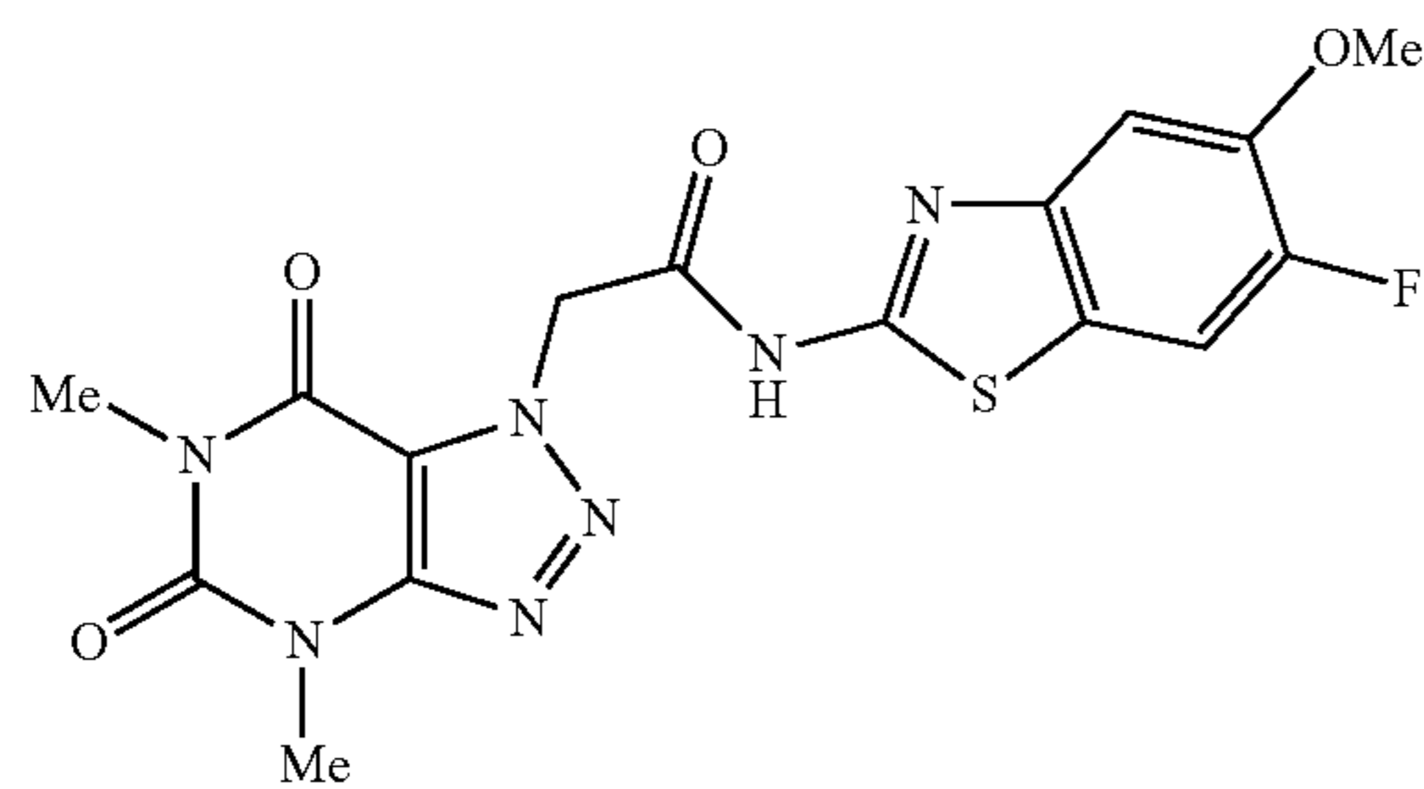
2-(4,6-dimethyl-5,7-dioxo-4,5,6,7-tetrahydro-1H-[1,2,3]triazolo[4,5-d]pyrimidin-1-yl)-N-(6-fluoro-5-methoxybenzo[d]thiazol-2-yl)acetamide
