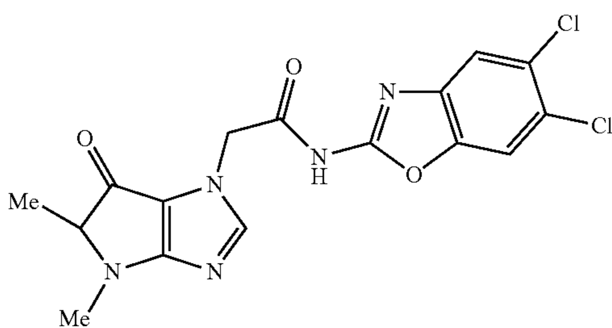
N-(5,6-dichlorobenzo[d]oxazol-2-yl)-2-(4,5-dimethyl-6-oxo-5,6-dihydropyrrolo[3,2-d]imidazol-1(4H)-yl)acetamide
