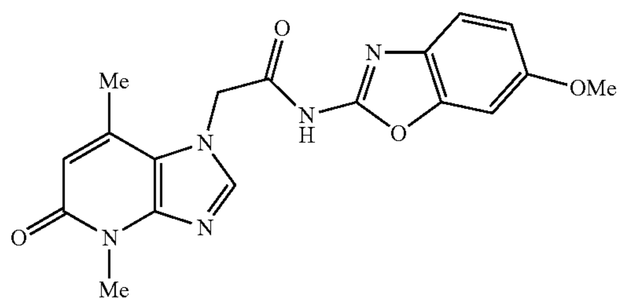
2-(4,7-dimethyl-5-oxo-4,5-dihydro-1H-imidazo[4,5-b]pyridin-1-yl)-N-(6-methoxybenzo[d]oxazol-2-yl)acetamide
