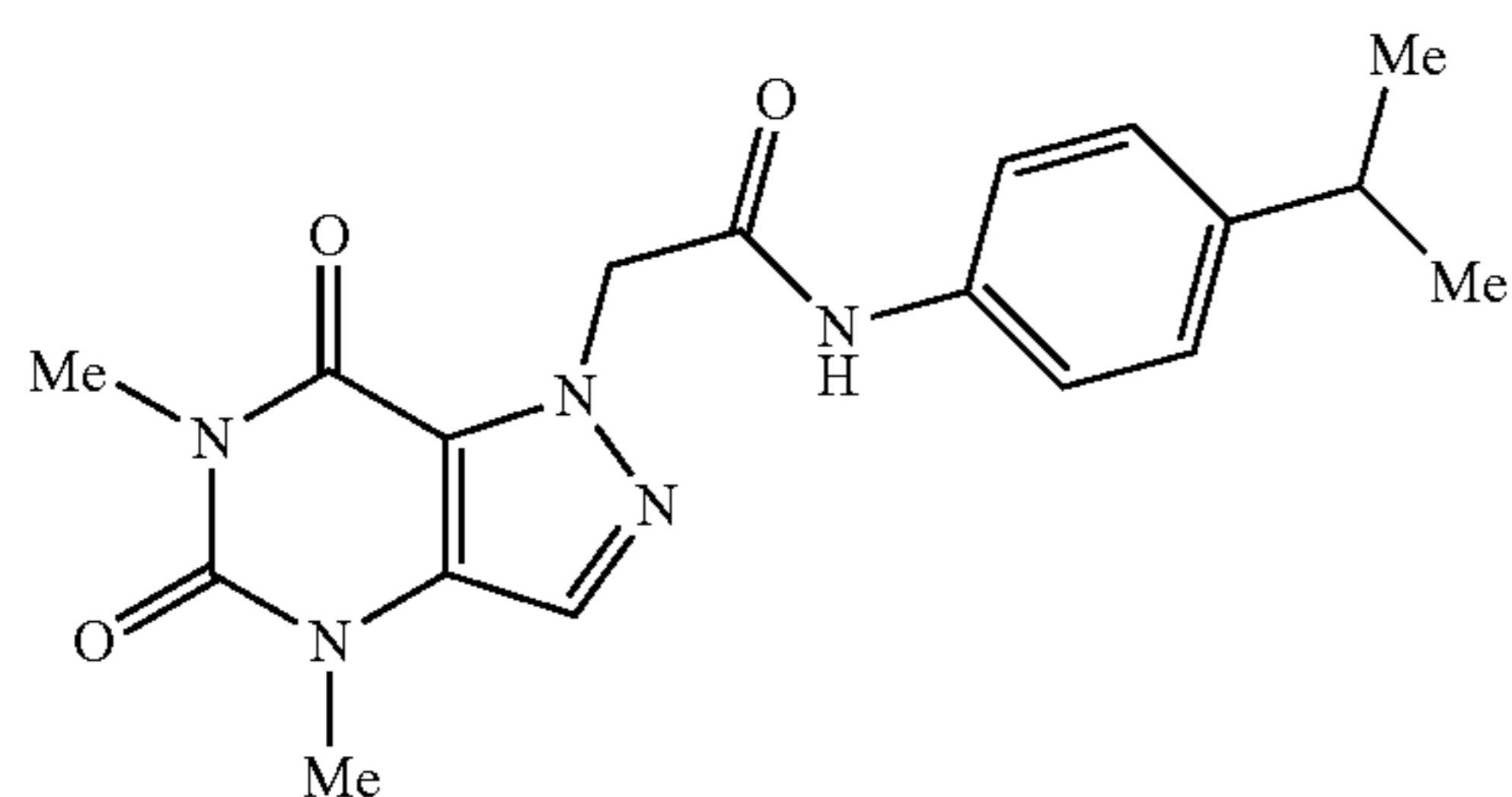
2-(4,6-dimethyl-5,7-dioxo-4,5,6,7-tetrahydro-1H-pyrazolo[4,3-d]pyrimidin-1-yl)-N-(4-isopropylphenyl)acetamide
