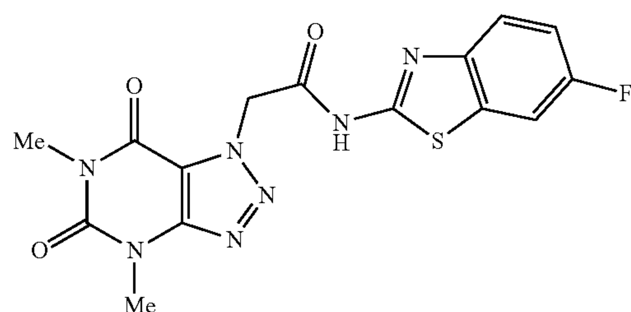
2-(4,6-dimethyl-5,7-dioxo-4,5,6,7-tetrahydro-1H-[1,2,3]triazolo[4,5-d]pyrimidin-1-yl)-N-(6-fluorobenzo[d]thiazol-2-yl)acetamide
