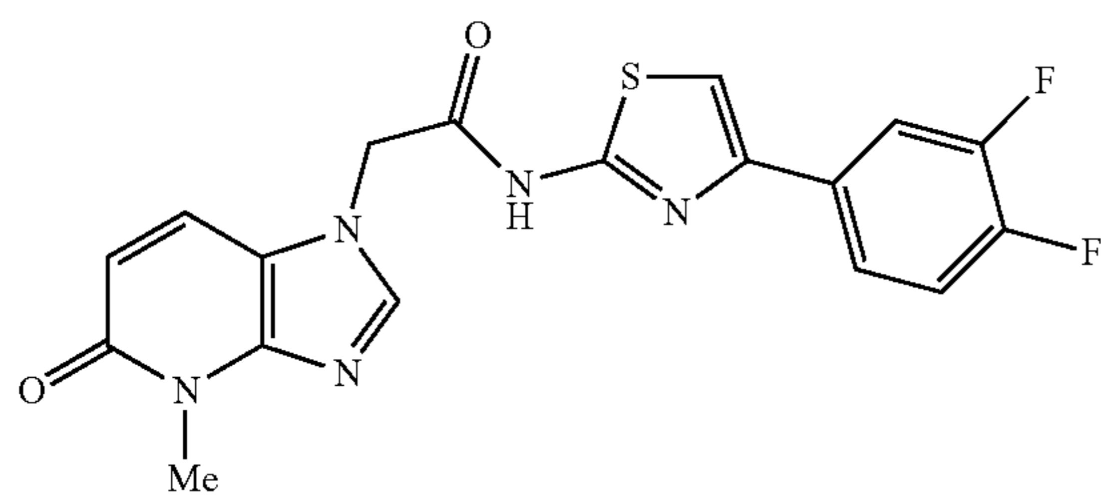
N-(4-(3,4-difluorophenyl)thiazol-2-yl)-2-(4-methyl-5-oxo-4,5-dihydro-1H-imidazo[4,5-b]pyridin-1-yl)acetamide
