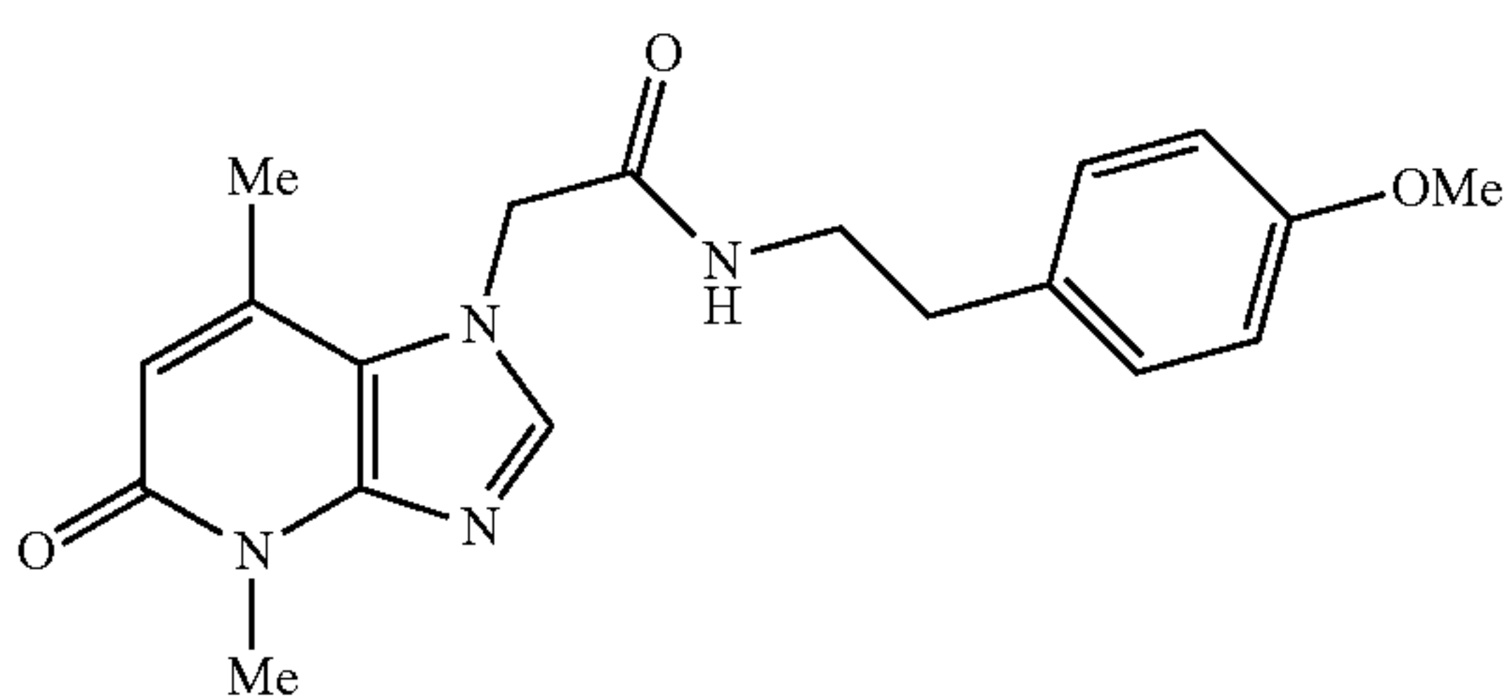
2-(4,7-dimethyl-5-oxo-4,5-dihydro-1H-imidazo[4,5-b]pyridin-1-yl)-N-(4-methoxyphenethyl)acetamide
