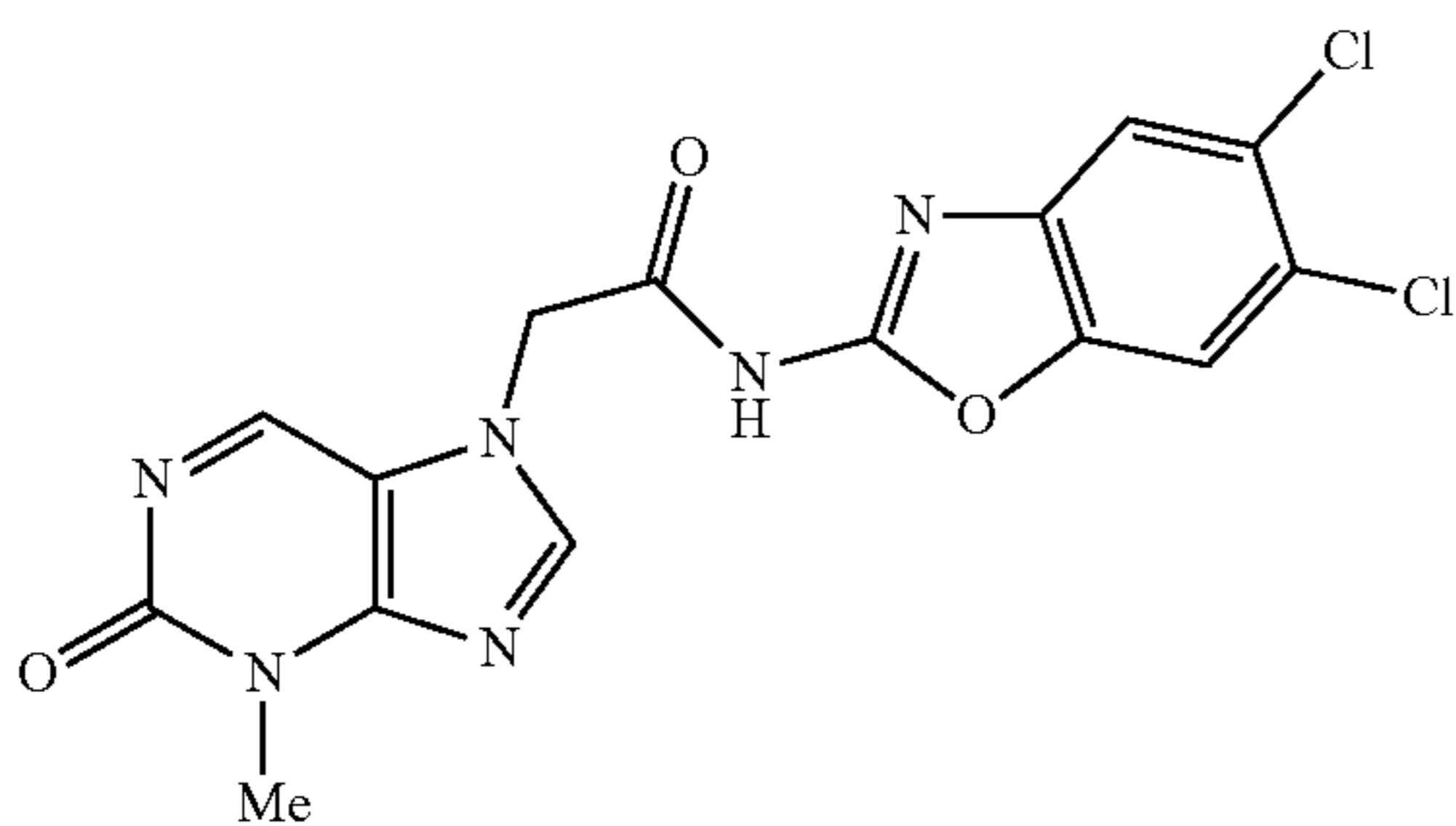
N-(5,6-dichlorobenzo[d]oxazol-2-yl)-2-(3-methyl-2-oxo-2,3-dihydropurin-7-yl)acetamide
