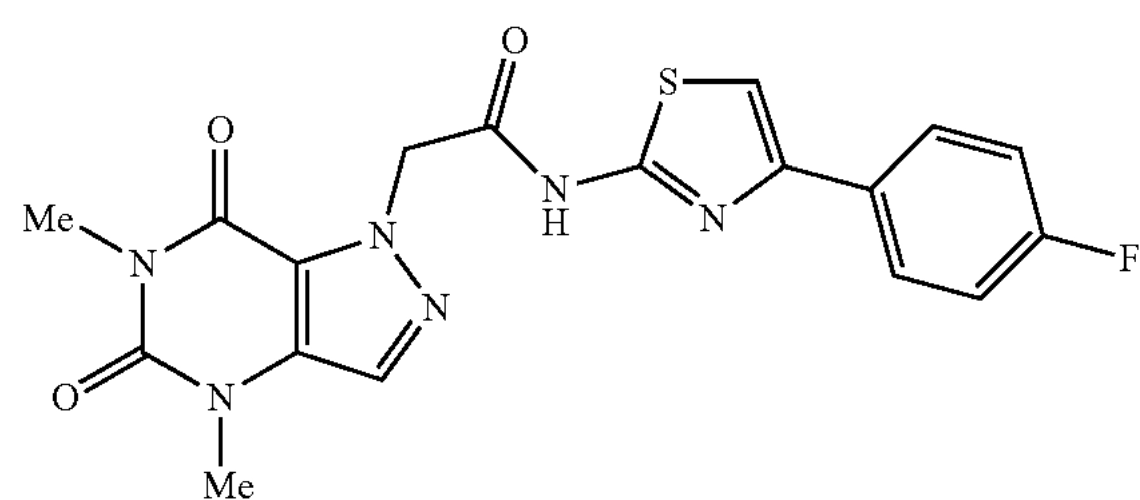
2-(4,6-dimethyl-5,7-dioxo-4,5,6,7-tetrahydro-1H-pyrazolo[4,3-d]pyrimidin-1-yl)-N-(4-(4-fluorophenyl)thiazol-2-yl)acetamide
