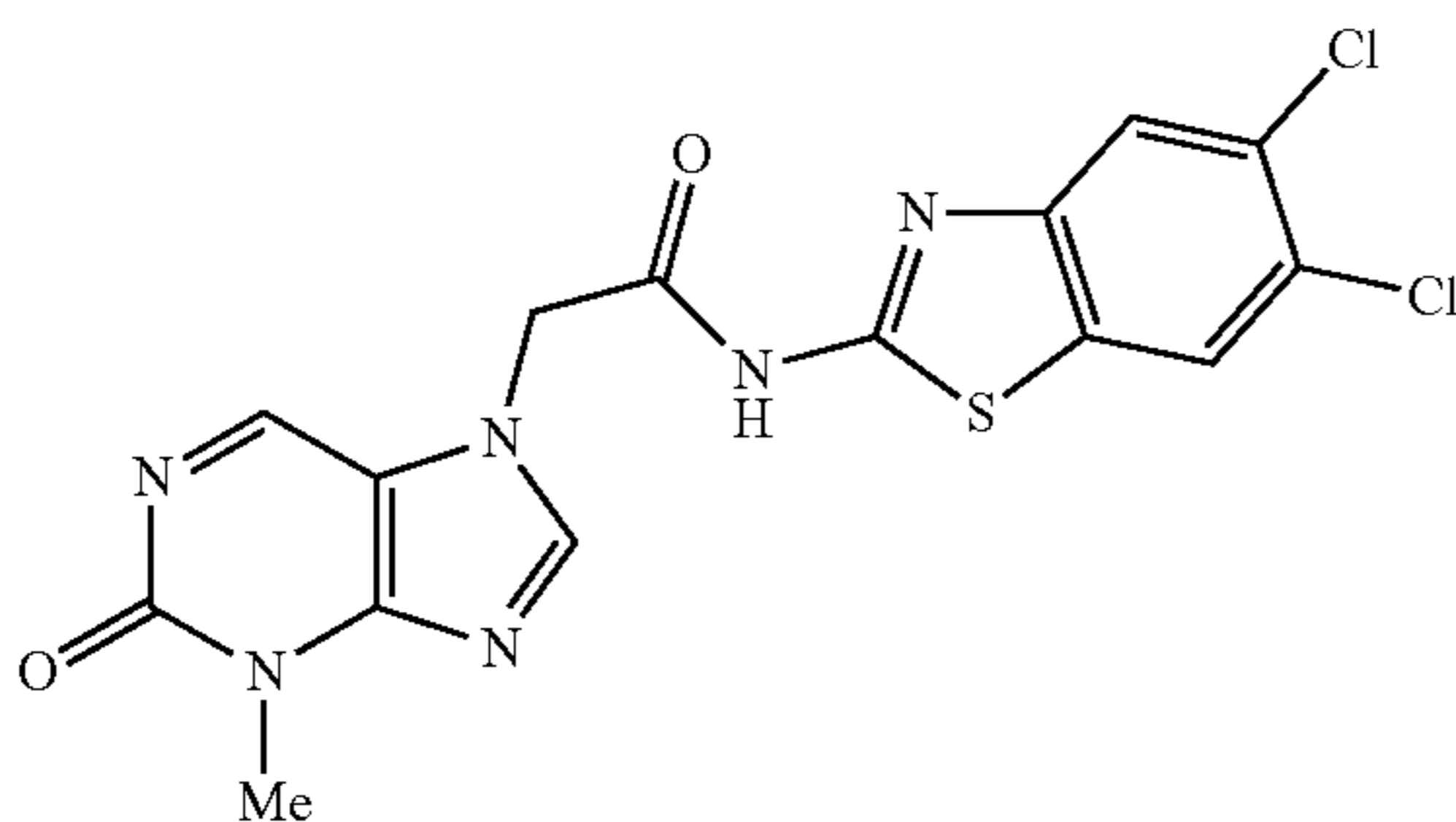
N-(5,6-dichlorobenzo[d]thiazol-2-yl)-2-(3-methyl-2-oxo-2,3-dihydropurin-7-yl)acetamide
