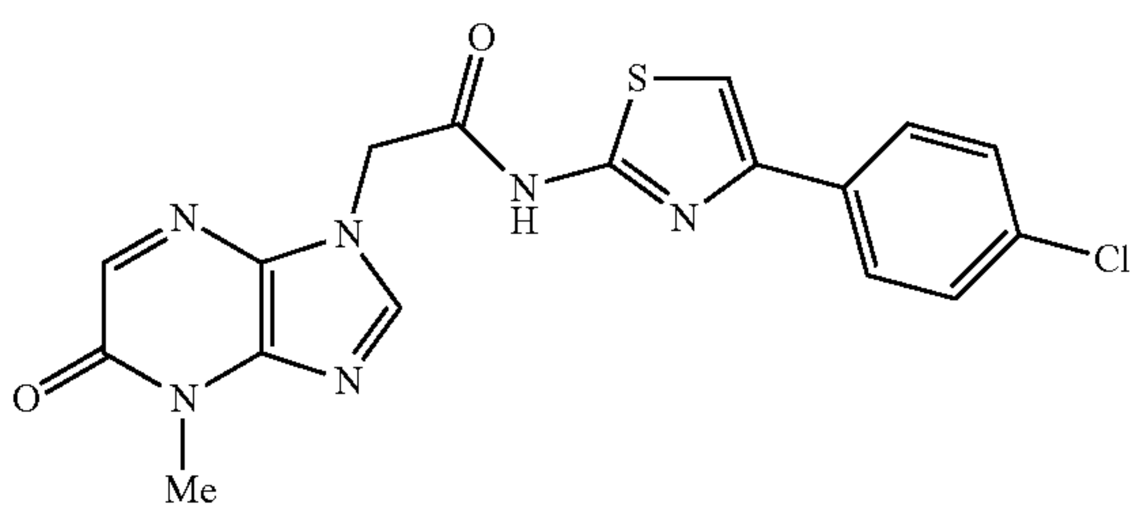
N-(4-(4-chlorophenyl)thiazol-2-yl)-2-(4-methyl-5-oxo-4,5-dihydro-1H-imidazo[4,5-b]pyrazin-1-yl)acetamide
