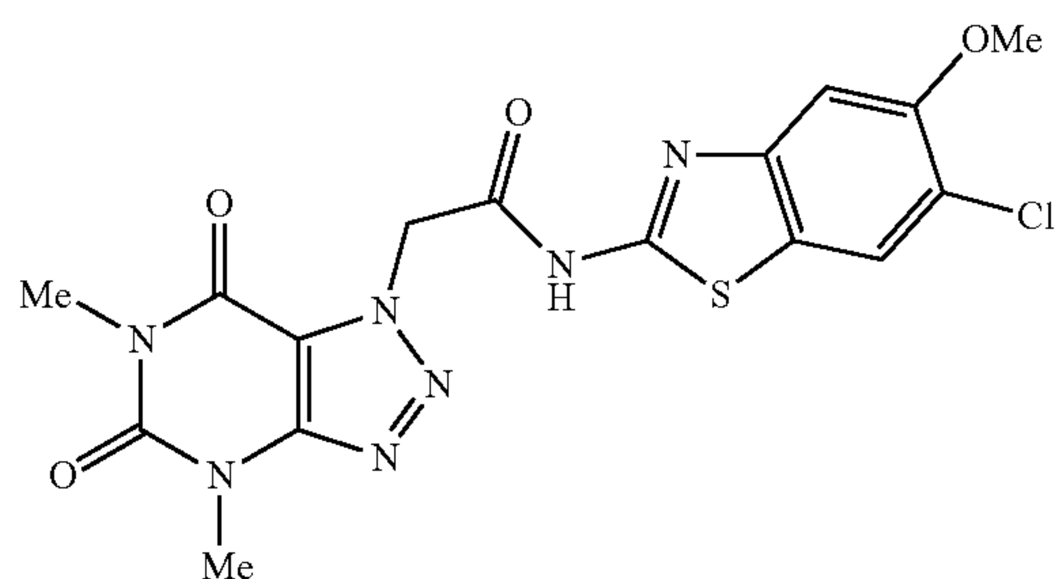
N-(6-chloro-5-methoxybenzo[d]thiazol-2-yl)-2-(4,6-dimethyl-5,7-dioxo-4,5,6,7-tetrahydro-1H-[1,2,3]triazolo[4,5-d]pyrimidin-1-yl)acetamide
