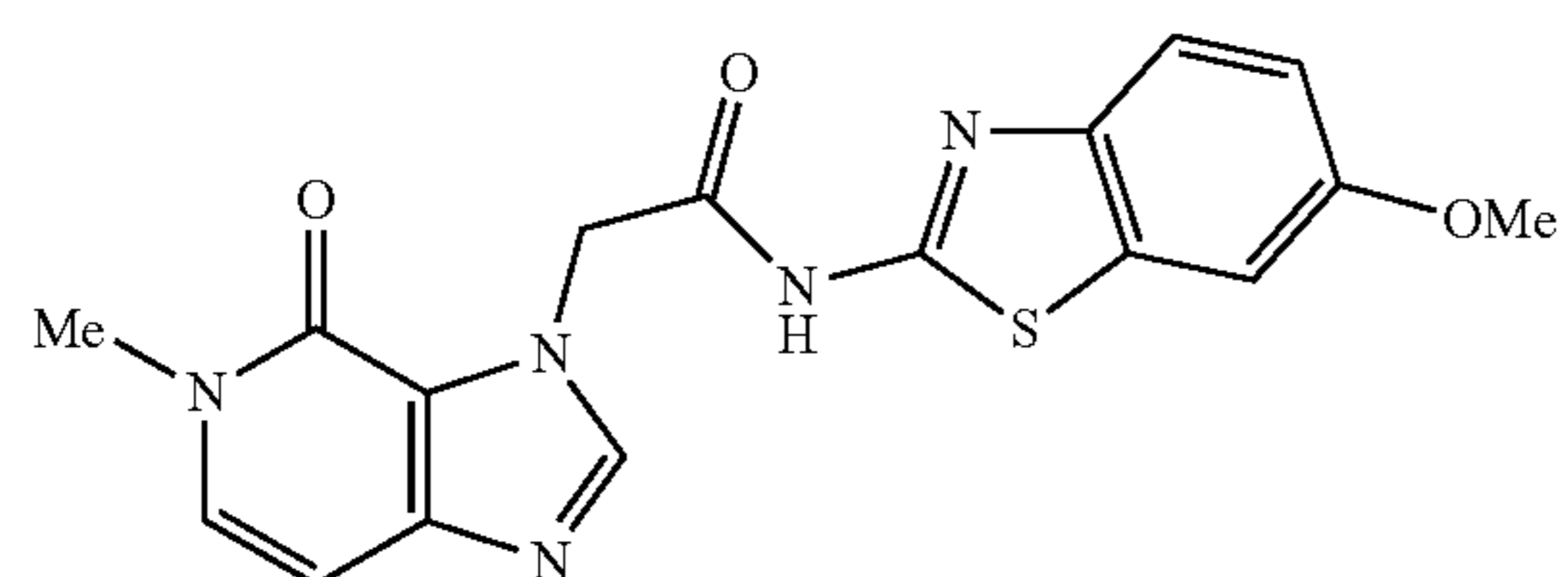
N-(6-methoxybenzo[d]thiazol-2-yl)-2-(5-methyl-4-oxo-4,5-dihydro-3H-imidazo[4,5-c]pyridin-3-yl)acetamide
