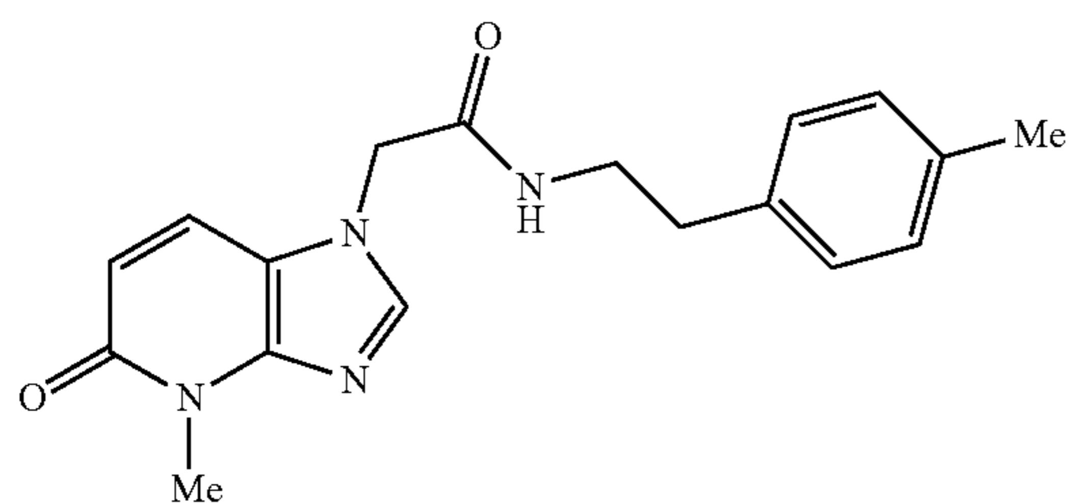
2-(4-methyl-5-oxo-4,5-dihydro-1H-imidazo[4,5-b]pyridin-1-yl)-N-(4-methylphenethyl)acetamide
