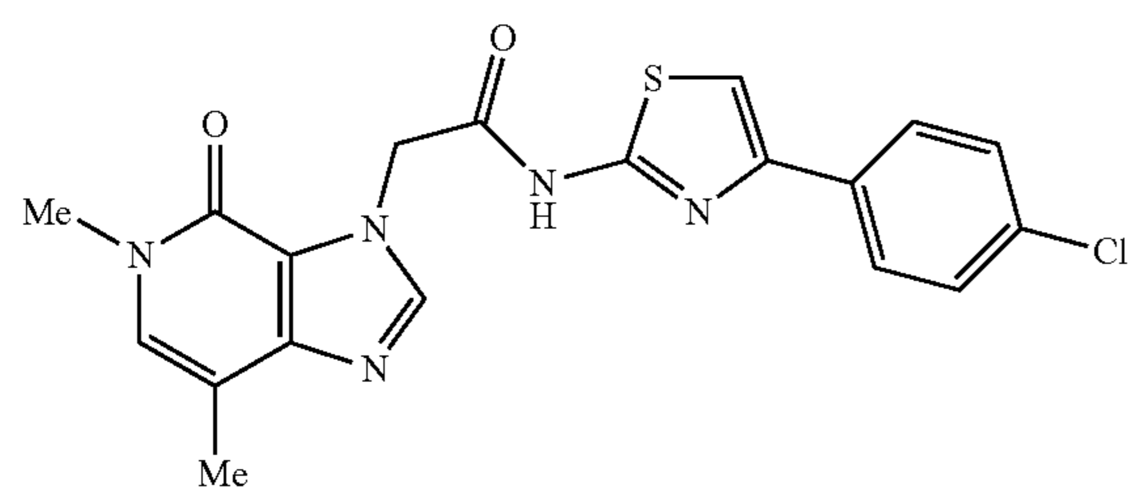
N-(4-(4-chlorophenyl)thiazol-2-yl)-2-(5,7-dimethyl-4-oxo-4,5-dihydro-3H-imidazo[4,5-c]pyridin-3-yl)acetamide
