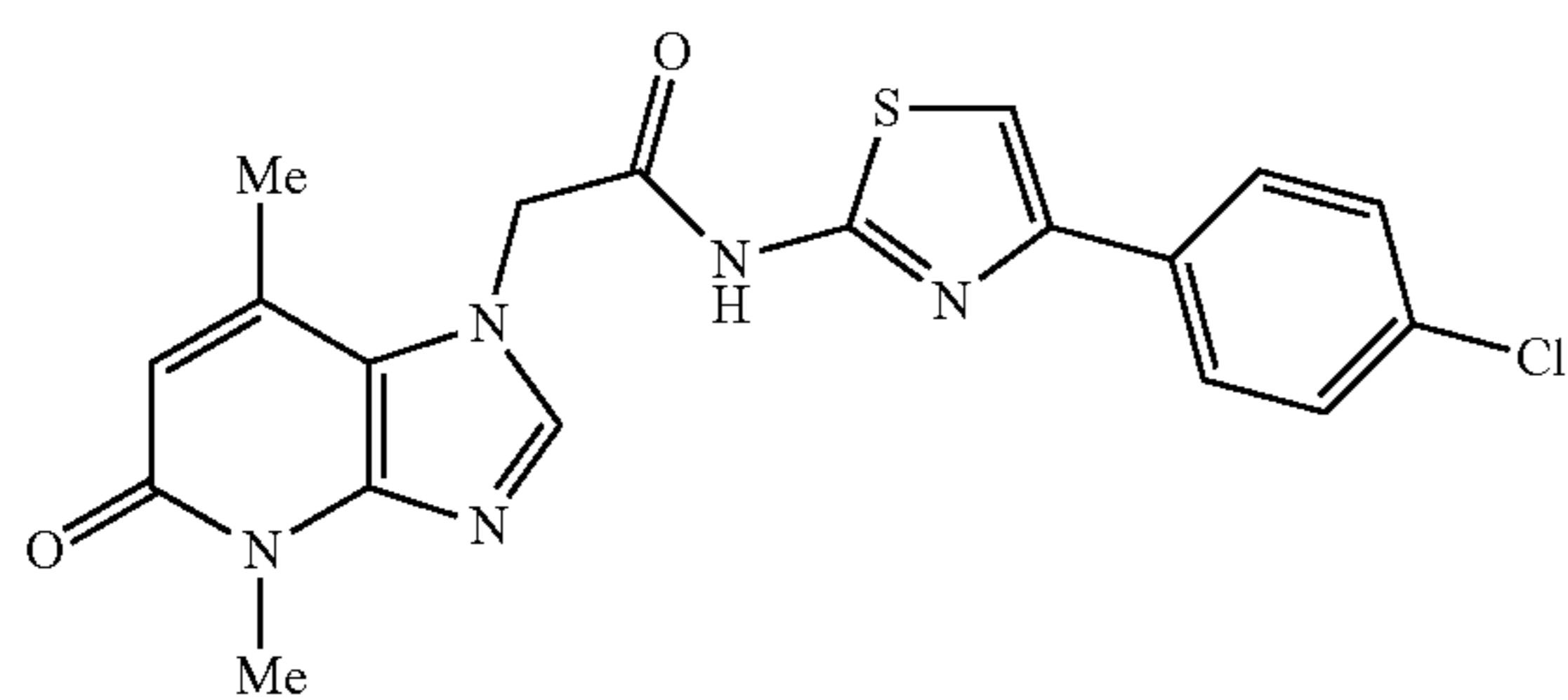
N-(4-(4-chlorophenyl)thiazol-2-yl)-2-(4,7-dimethyl-5-oxo-4,5-dihydro-1H-imidazo[4,5-b]pyridin-1-yl)acetamide
