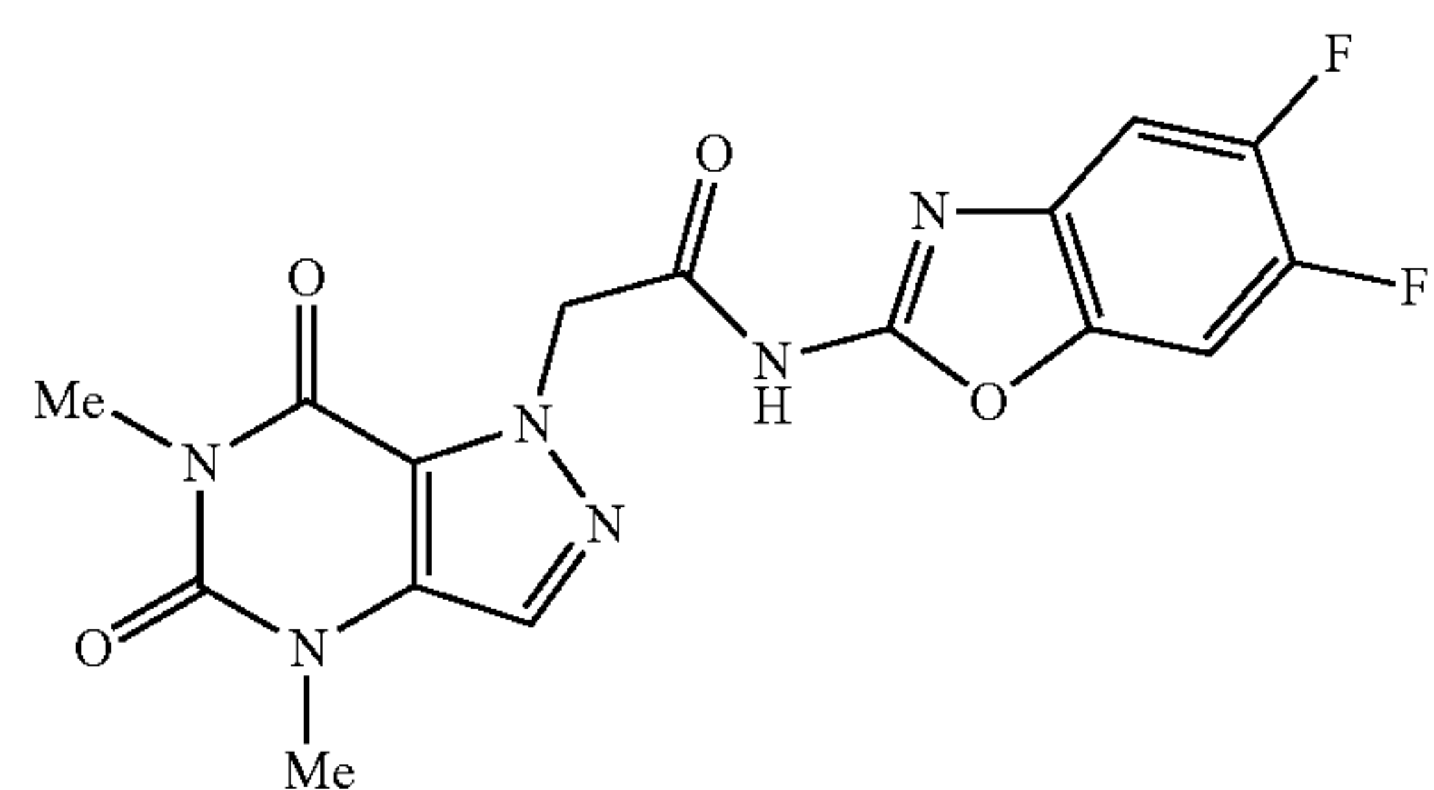
N-(5,6-difluorobenzo[d]oxazol-2-yl)-2-(4,6-dimethyl-5,7-dioxo-4,5,6,7-tetrahydro-1H-pyrazolo[4,3-d]pyrimidin-1-yl)acetamide
