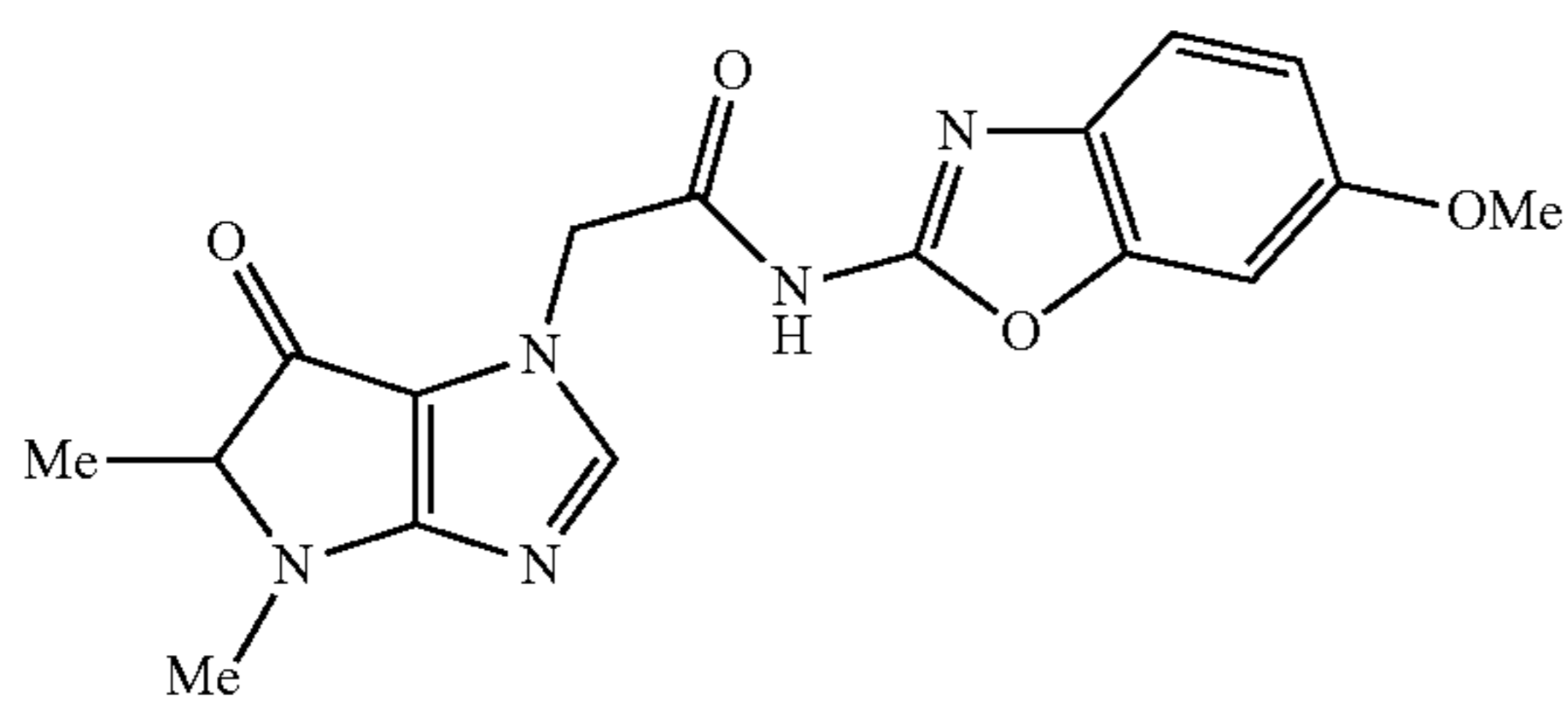
2-(4,5-dimethyl-6-oxo-5,6-dihydropyrrolo[3,2-d]imidazol-1(4H)-yl)-N-(6-methoxybenzo[d]oxazol-2-yl)acetamide
