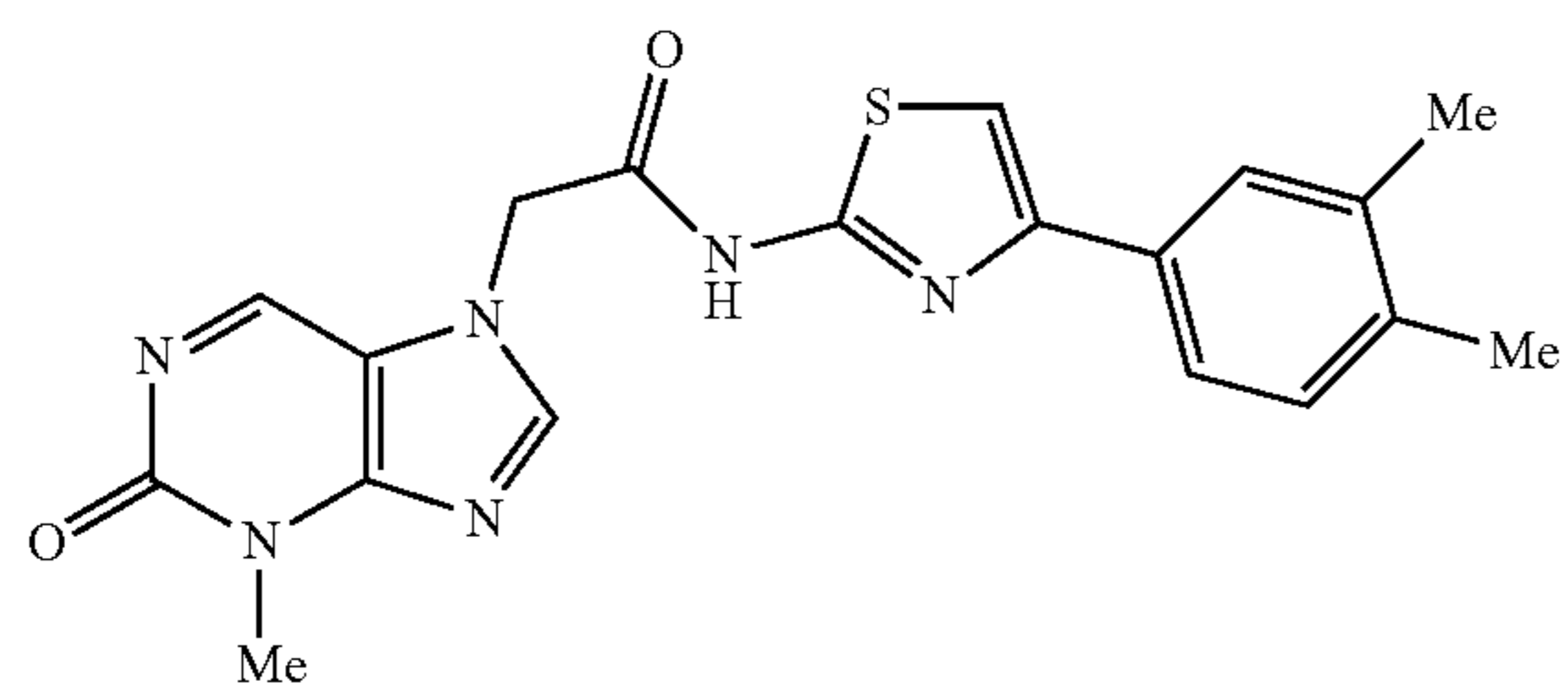
N-(4-(3,4-dimethylphenyl)thiazol-2-yl)-2-(3-methyl-2-oxo-2,3-dihydropurin-7-yl)acetamide
