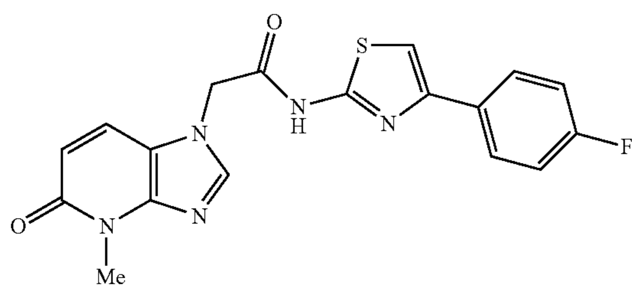
N-(4-(4-fluorophenyl)thiazol-2-yl)-2-(4-methyl-5-oxo-4,5-dihydro-1H-imidazo[4,5-b]pyridin-1-yl)acetamide
