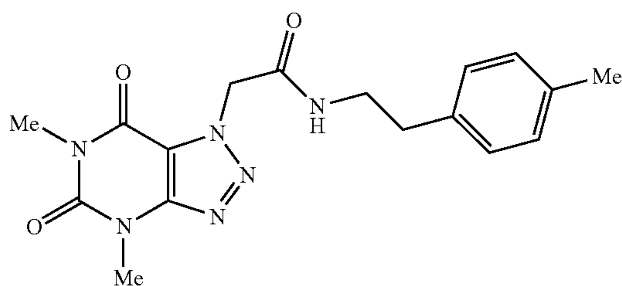
2-(4,6-dimethyl-5,7-dioxo-4,5,6,7-tetrahydro-1H-[1,2,3]triazolo[4,5-d]pyrimidin-1-yl)-N-(4-methylphenethyl)acetamide
