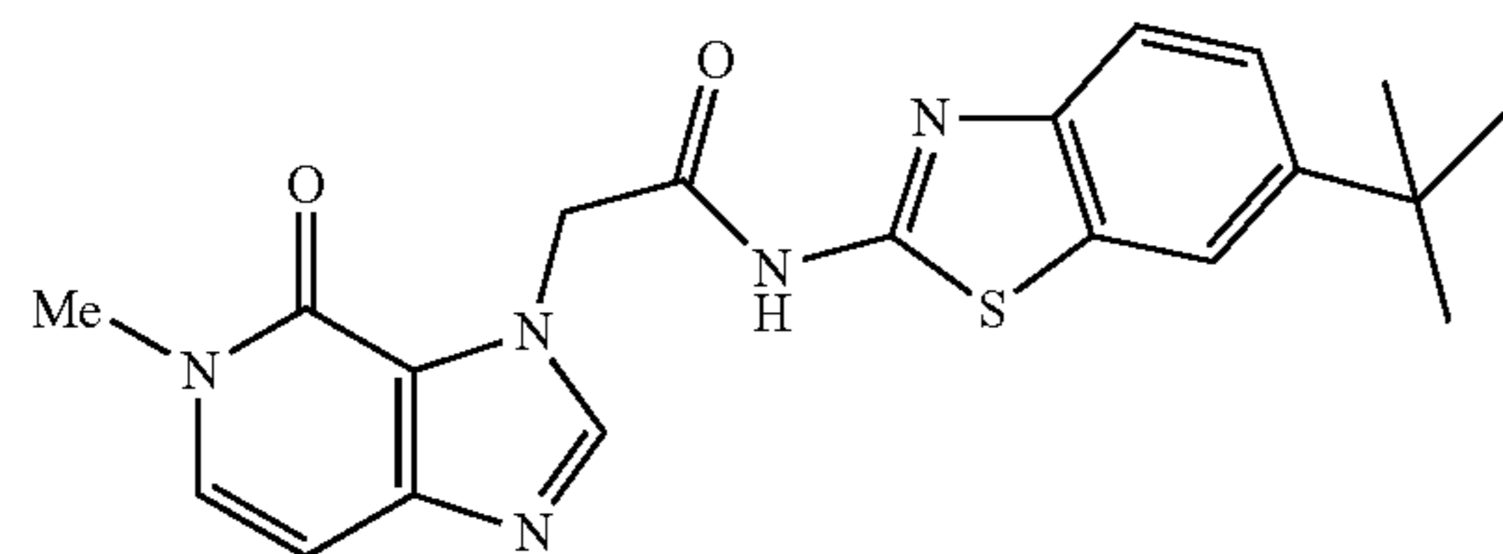
N-(6-tert-butylbenzo[d]thiazol-2-yl)-2-(5-methyl-4-oxo-4,5-dihydro-3H-imidazo[4,5-c]pyridin-3-yl)acetamide
