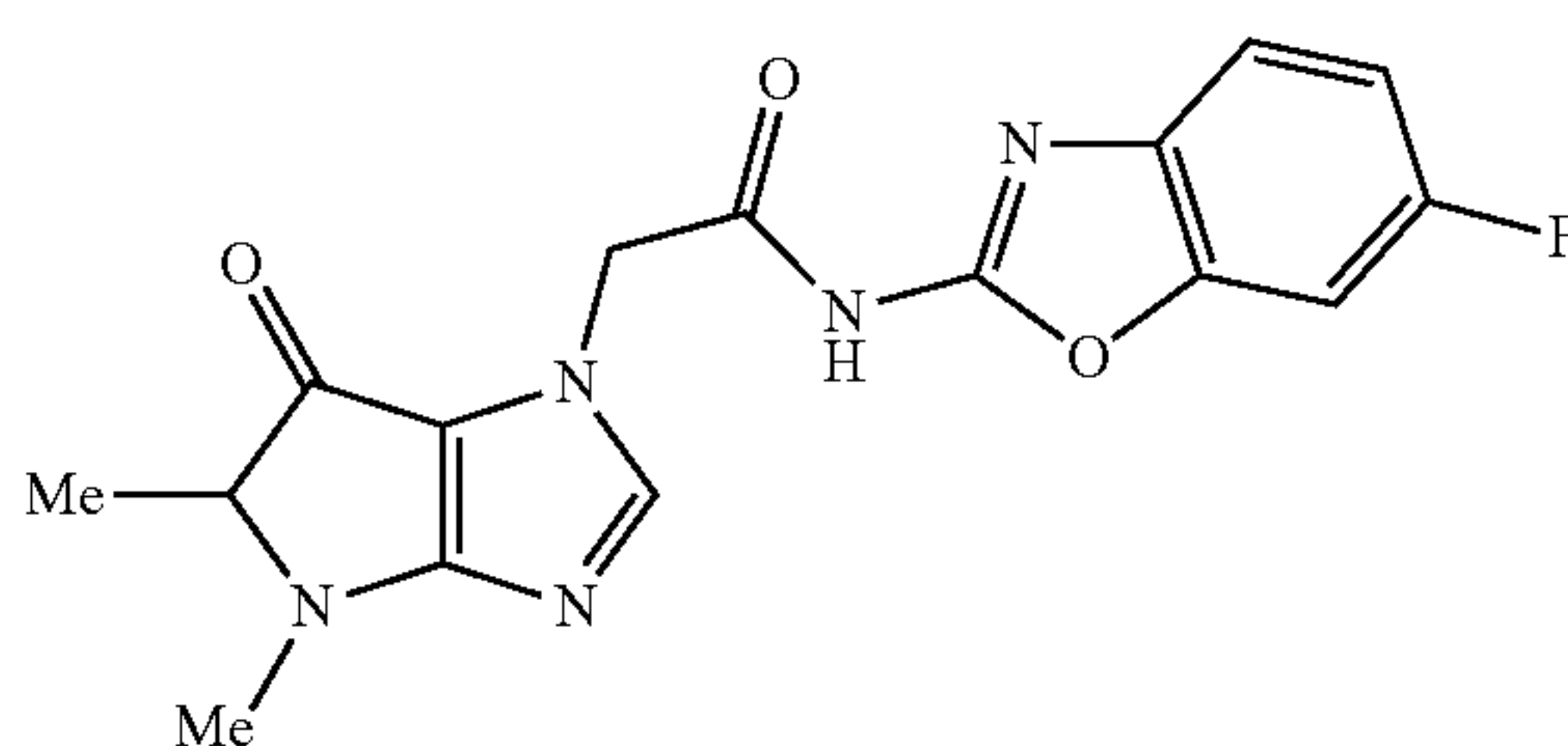
2-(4,5-dimethyl-6-oxo-5,6-dihydropyrrolo[3,2-d]imidazol-1(4H)-yl)-N-(6-fluorobenzo[d]oxazol-2-yl)acetamide
