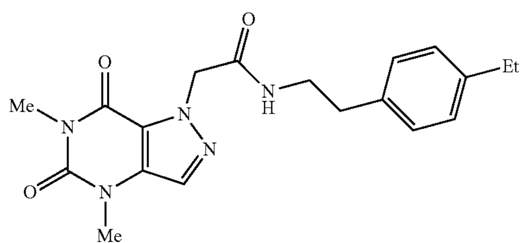
2-(4,6-dimethyl-5,7-dioxo-4,5,6,7-tetrahydro-1H-pyrazolo[4,3-d]pyrimidin-1-yl)-N-(4-ethylphenethyl)acetamide
