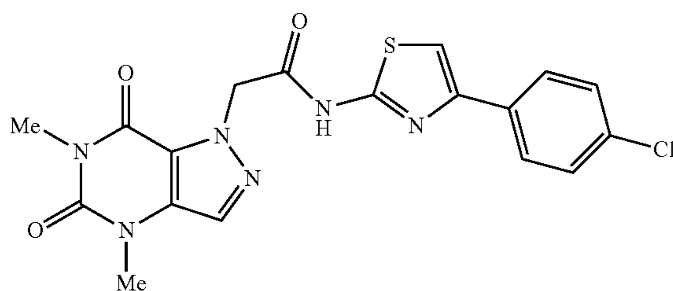
N-(4-(4-chlorophenyl)thiazol-2-yl)-2-(4,6-dimethyl-5,7-dioxo-4,5,6,7-tetrahydro-1H-pyrazolo[4,3-d]pyrimidin-1-yl)acetamide
