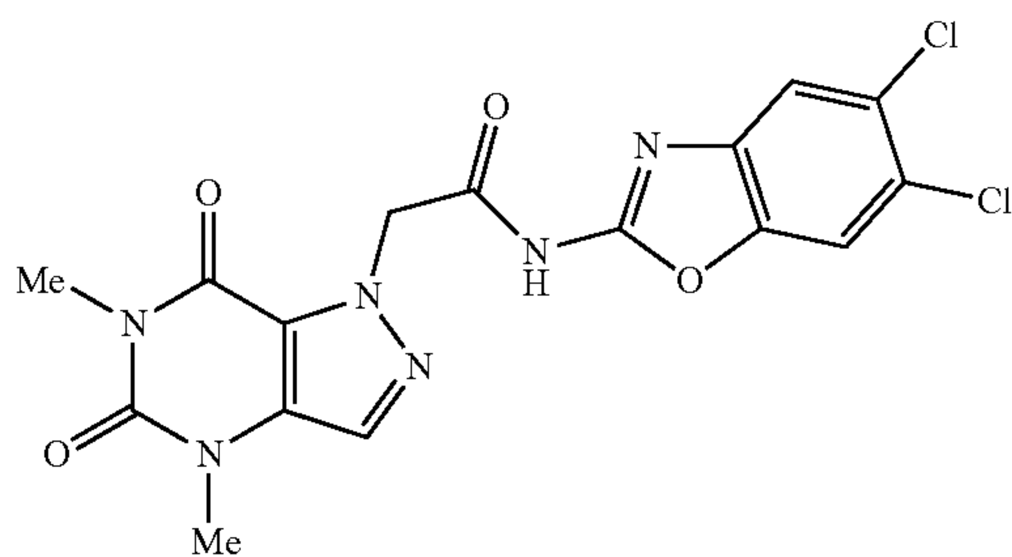
N-(5,6-dichlorobenzo[d]oxazol-2-yl)-2-(4,6-dimethyl-5,7-dioxo-4,5,6,7-tetrahydro-1H-pyrazolo[4,3-d]pyrimidin-1-yl)acetamide
