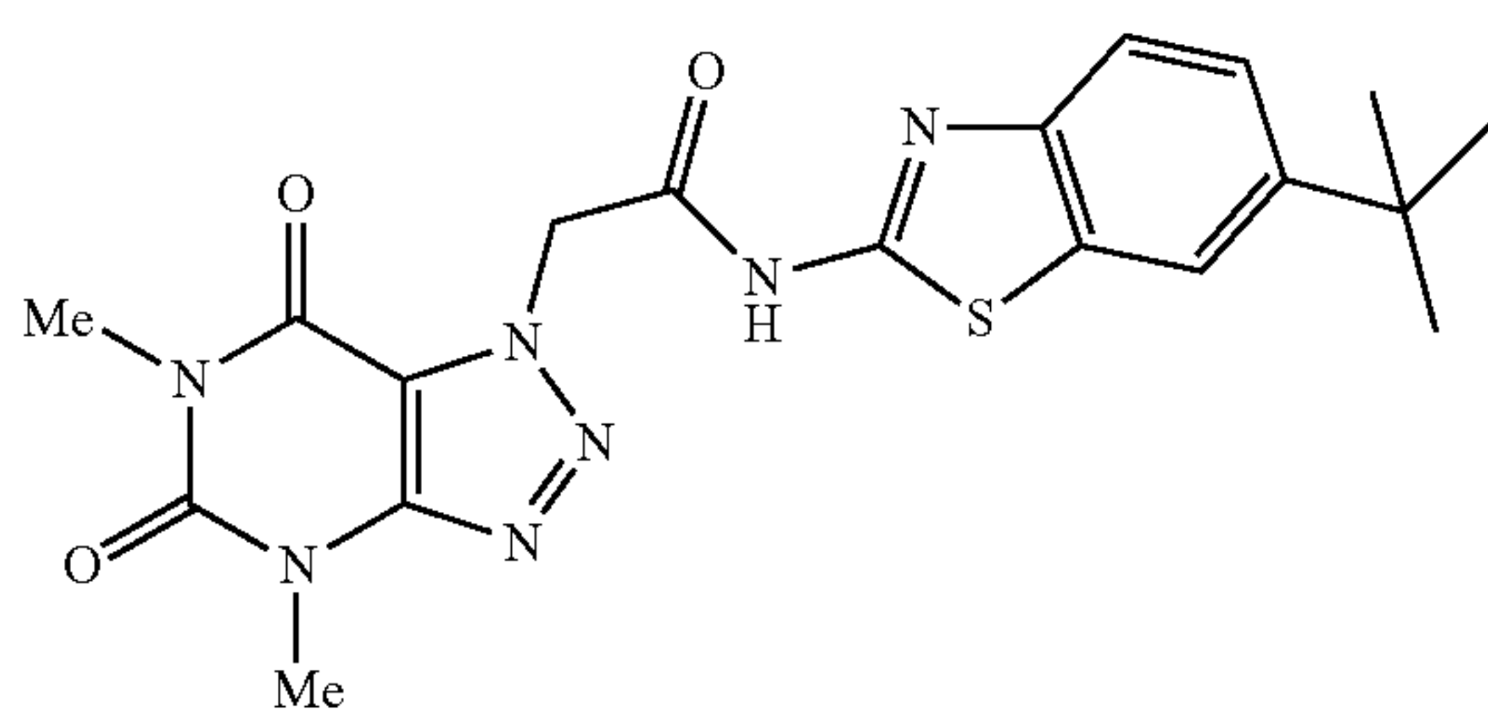
N-(6-tert-butylbenzo[d]thiazol-2-yl)-2-(4,6-dimethyl-5,7-dioxo-4,5,6,7-tetrahydro-1H-[1,2,3]triazolo[4,5-d]pyrimidin-1-yl)acetamide
