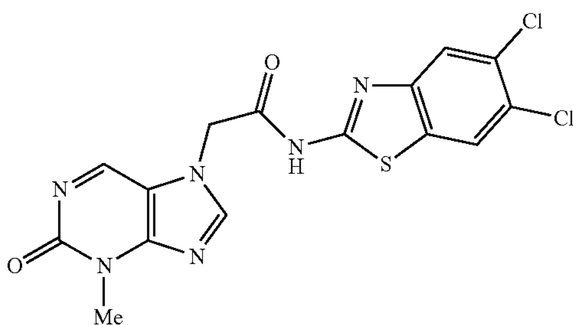
N-(5,6-dichlorobenzo[d]thiazol-2-yl)-2-(3-methyl-2-oxo-2,3-dihydropurin-7-yl)acetamide
