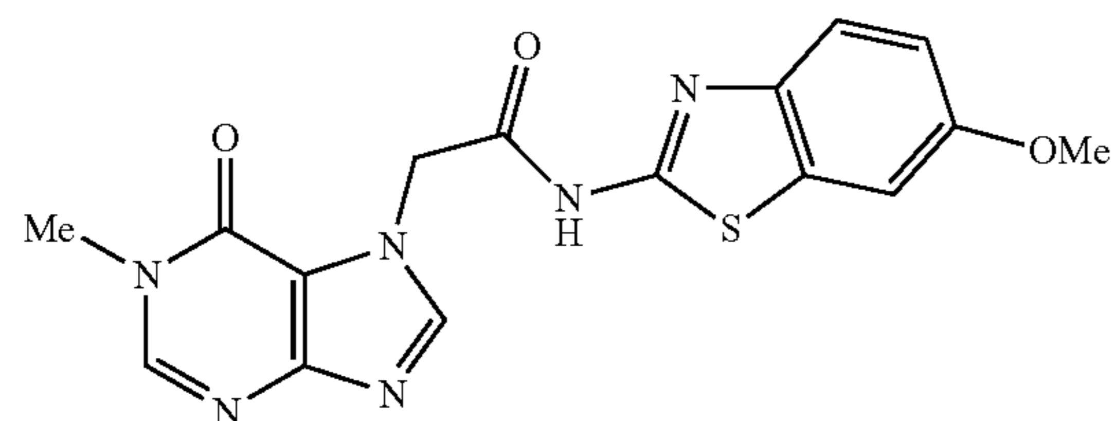
N-(6-methoxybenzo[d]thiazol-2-yl)-2-(1-methyl-6-oxo-1H-purin-7(6H)-yl)acetamide
