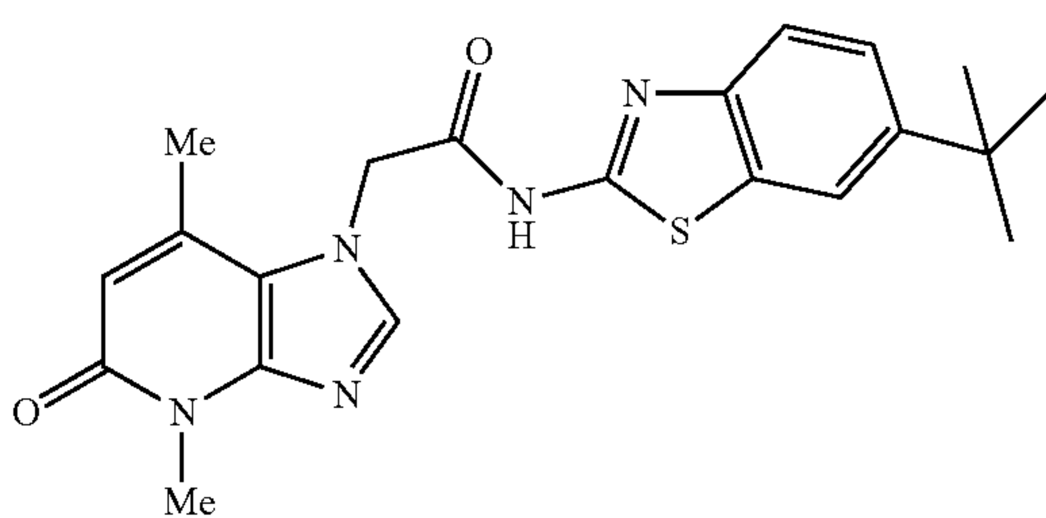
N-(6-tert-butylbenzo[d]thiazol-2-yl)-2-(4,7-dimethyl-5-oxo-4,5-dihydro-1H-imidazo[4,5-b]pyridin-1-yl)acetamide
