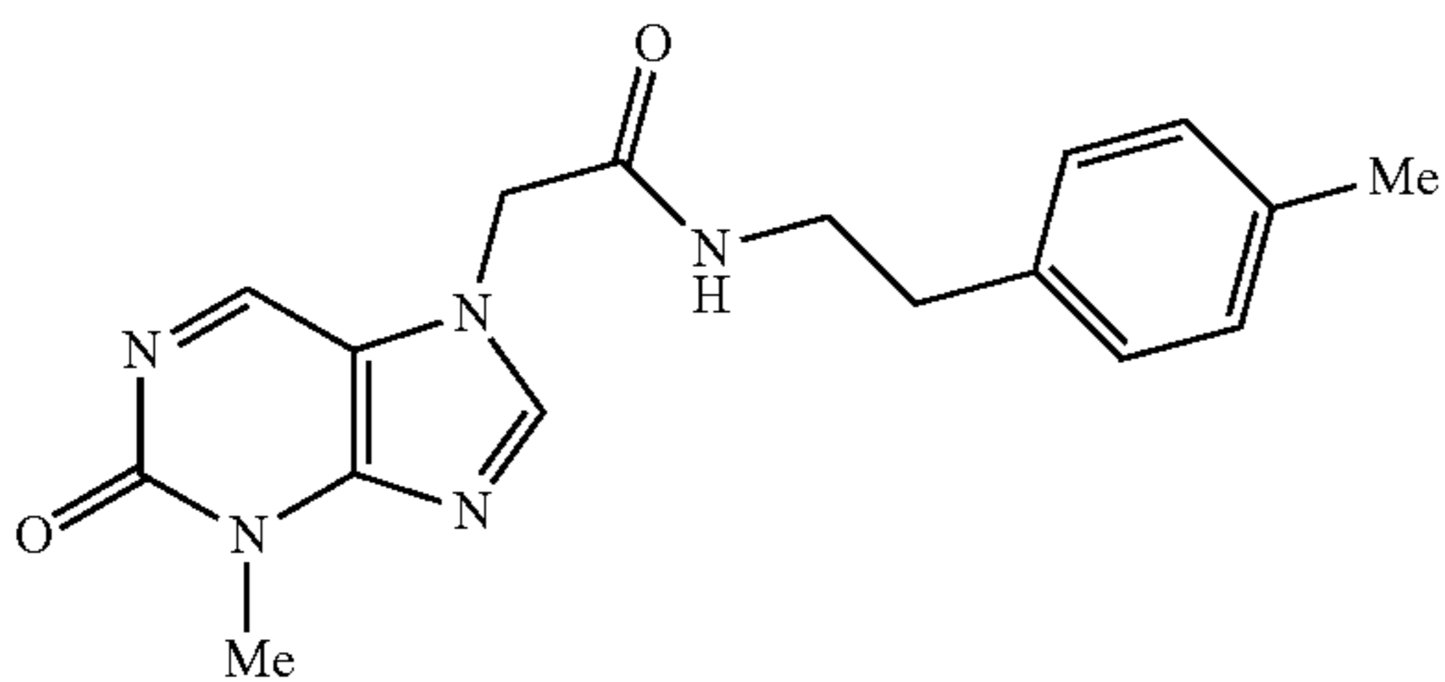
N-(4-methylphenethyl)-2-(3-methyl-2-oxo-2,3-dihydropurin-7-yl)acetamide
