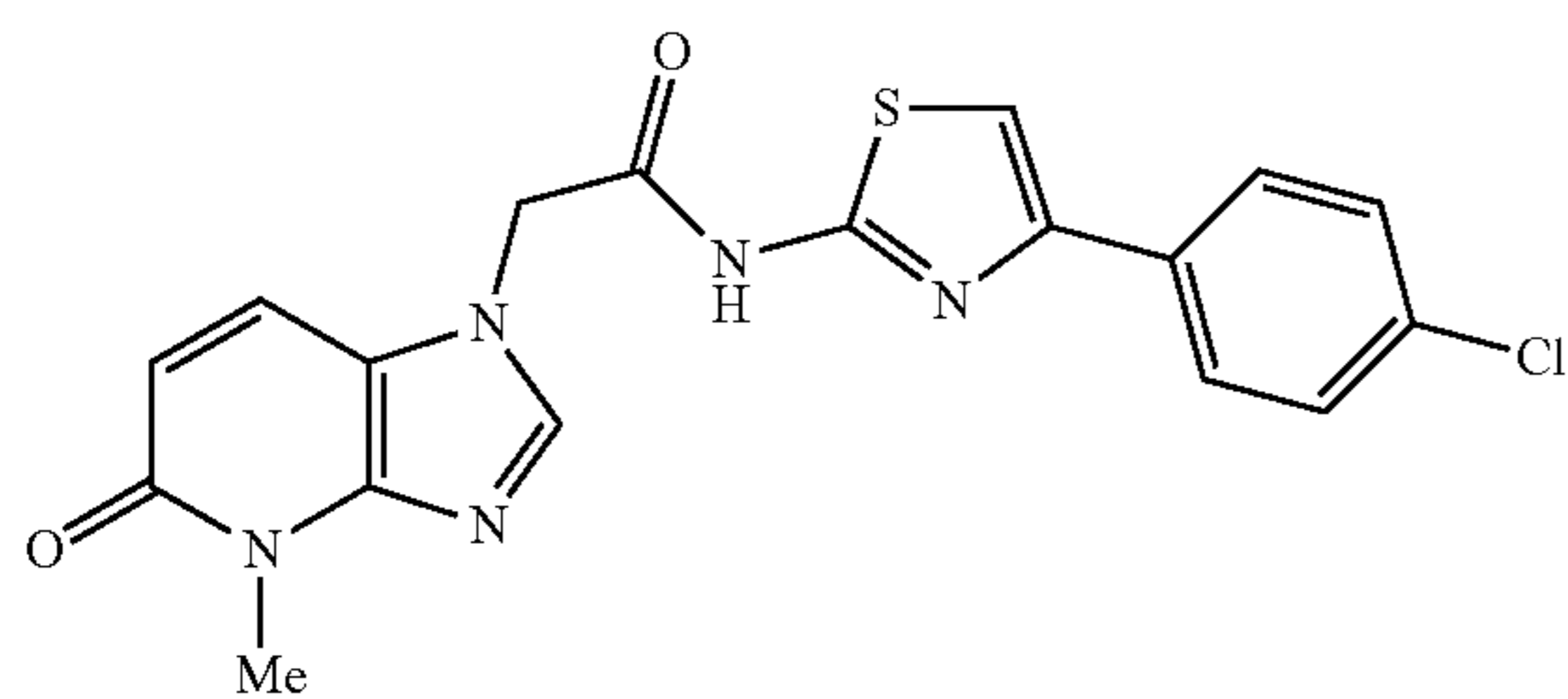
N-(4-(4-chlorophenyl)thiazol-2-yl)-2-(4-methyl-5-oxo-4,5-dihydro-1H-imidazo[4,5-b]pyridin-1-yl)acetamide
