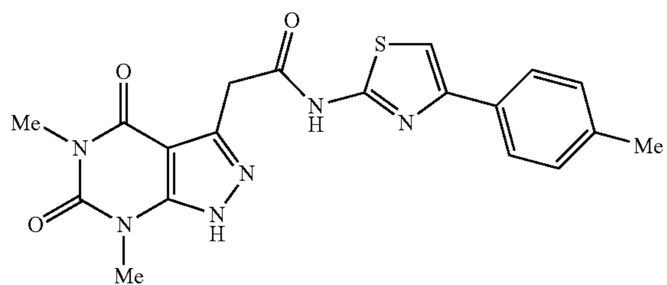
2-(5,7-dimethyl-4,6-dioxo-4,5,6,7-tetrahydro-1H-pyrazolo[3,4-d]pyrimidin-3-yl)-N-(4-p-tolylthiazol-2-yl)acetamide
