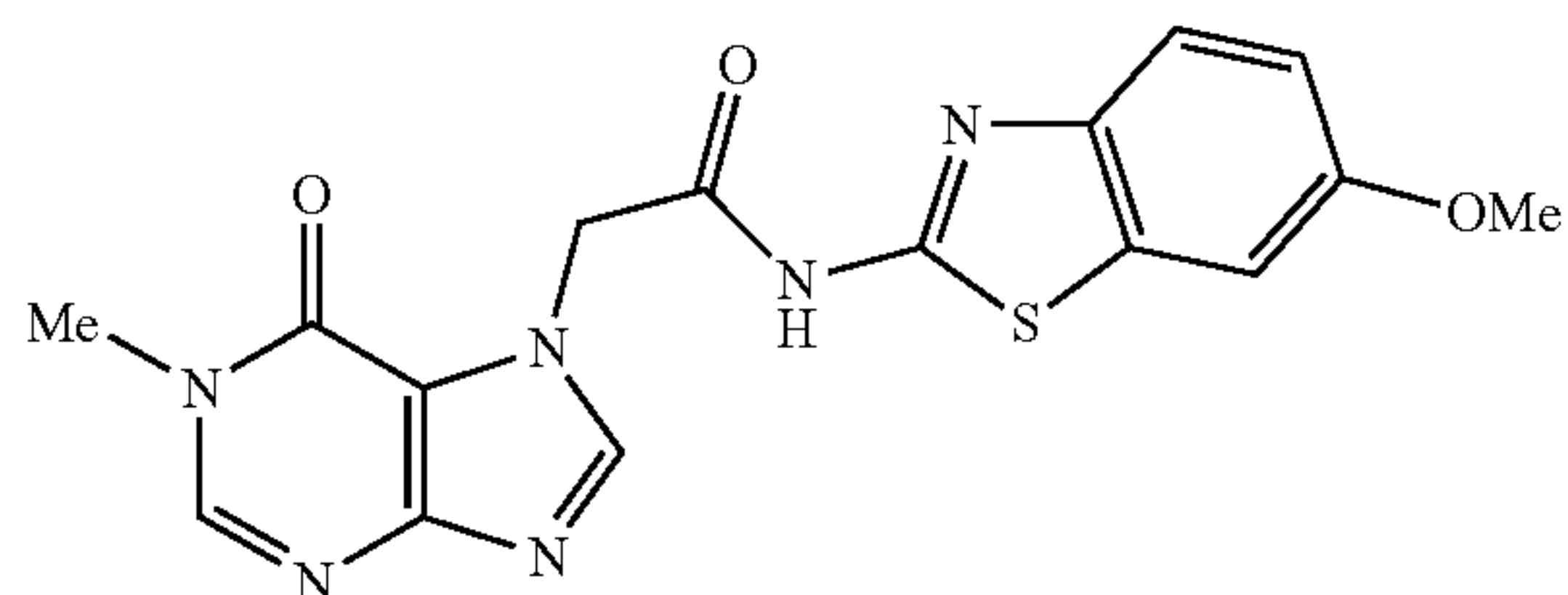
N-(6-methoxybenzo[d]thiazol-2-yl)-2-(1-methyl-6-oxo-1H-purin-7(6H)-yl)acetamide
