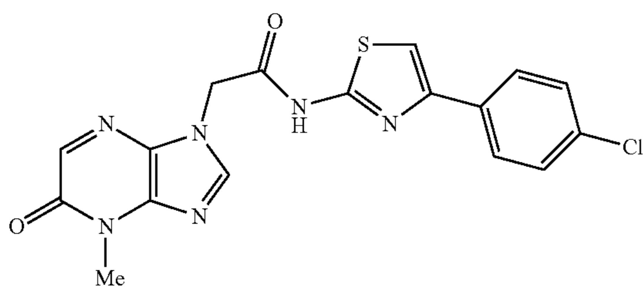
N-(4-(4-chlorophenyl)thiazol-2-yl)-2-(4-methyl-5-oxo-4,5-dihydro-1H-imidazo[4,5-b]pyrazin-1-yl)acetamide
