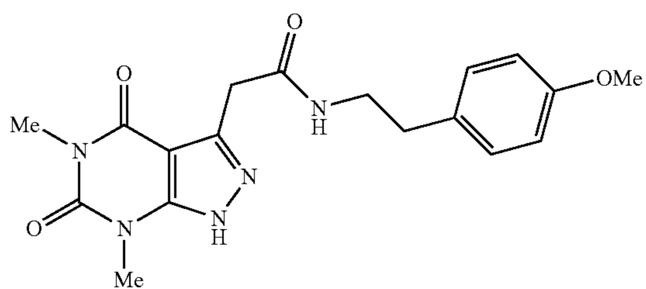
2-(5,7-dimethyl-4,6-dioxo-4,5,6,7-tetrahydro-1H-pyrazolo[3,4-d]pyrimidin-3-yl)-N-(4-methoxyphenethyl)acetamide
