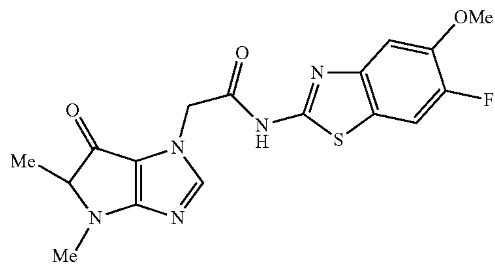
2-(4,5-dimethyl-6-oxo-5,6-dihydropyrrolo[3,2-d]imidazol-1(4H)-yl)-N-(6-fluoro-5-methoxybenzo[d]thiazol-2-yl)acetamide
