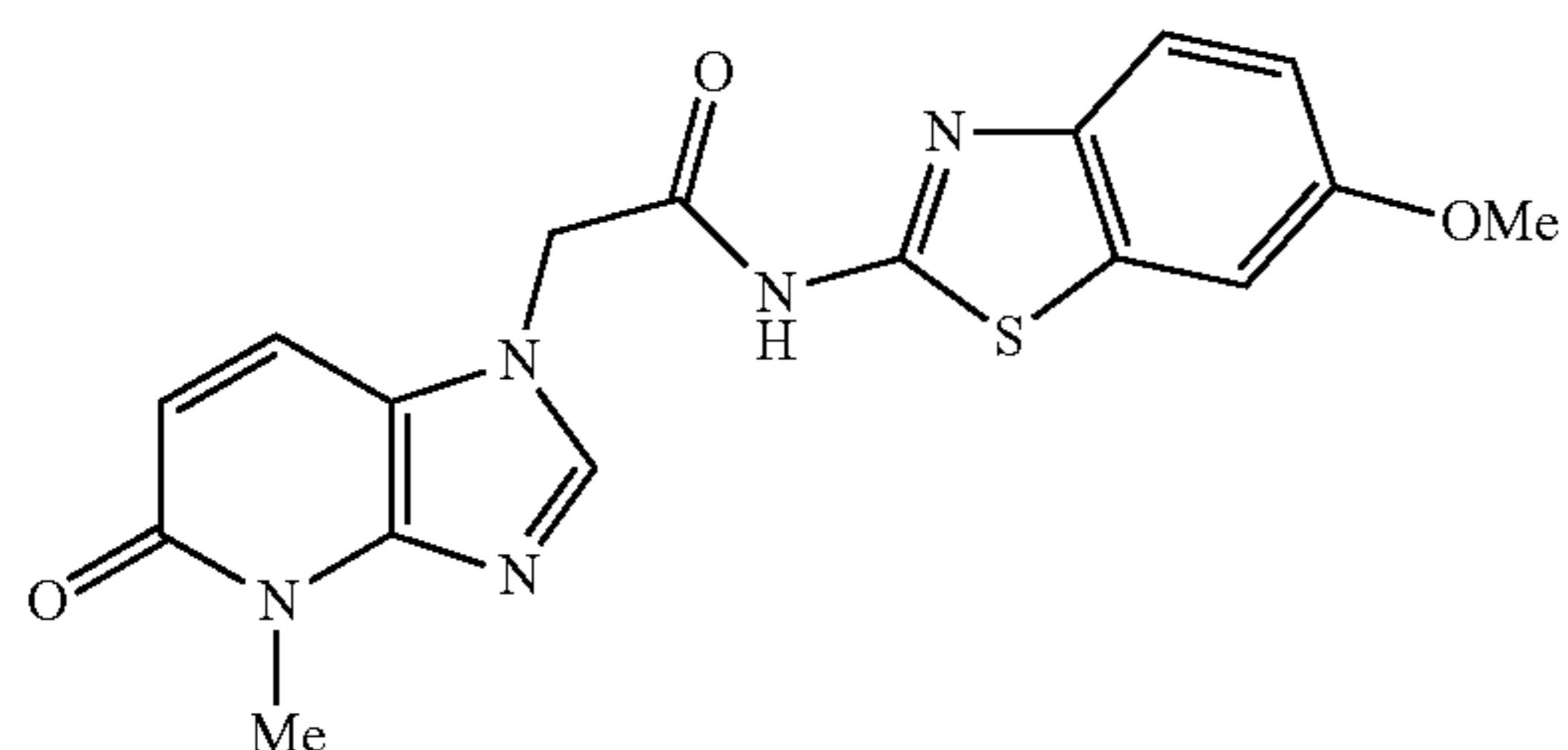
N-(6-methoxybenzo[d]thiazol-2-yl)-2-(4-methyl-5-oxo-4,5-dihydro-1H-imidazo[4,5-b]pyridin-1-yl)acetamide
