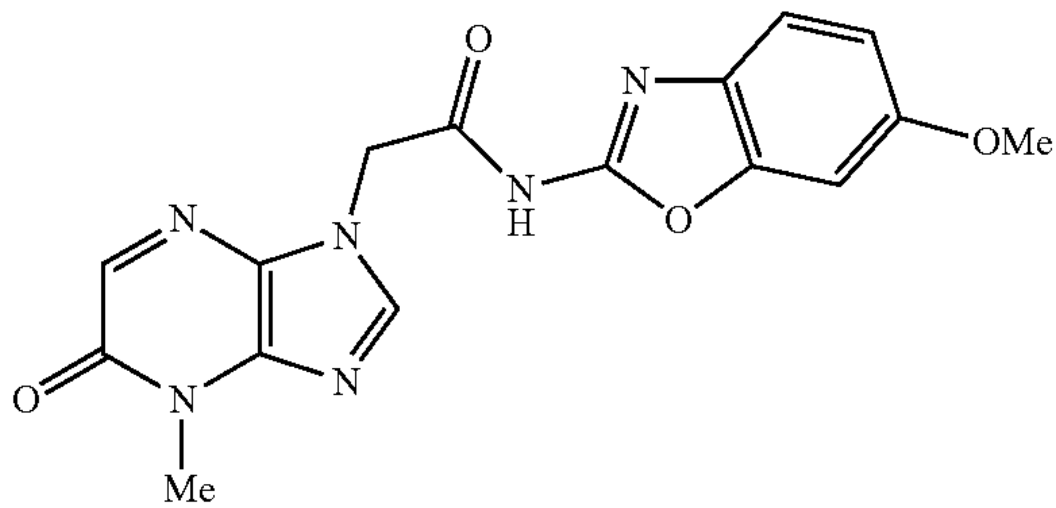
N-(6-methoxybenzo[d]oxazol-2-yl)-2-(4-methyl-5-oxo-4,5-dihydro-1H-imidazo[4,5-b]pyridin-1-yl)acetamide
