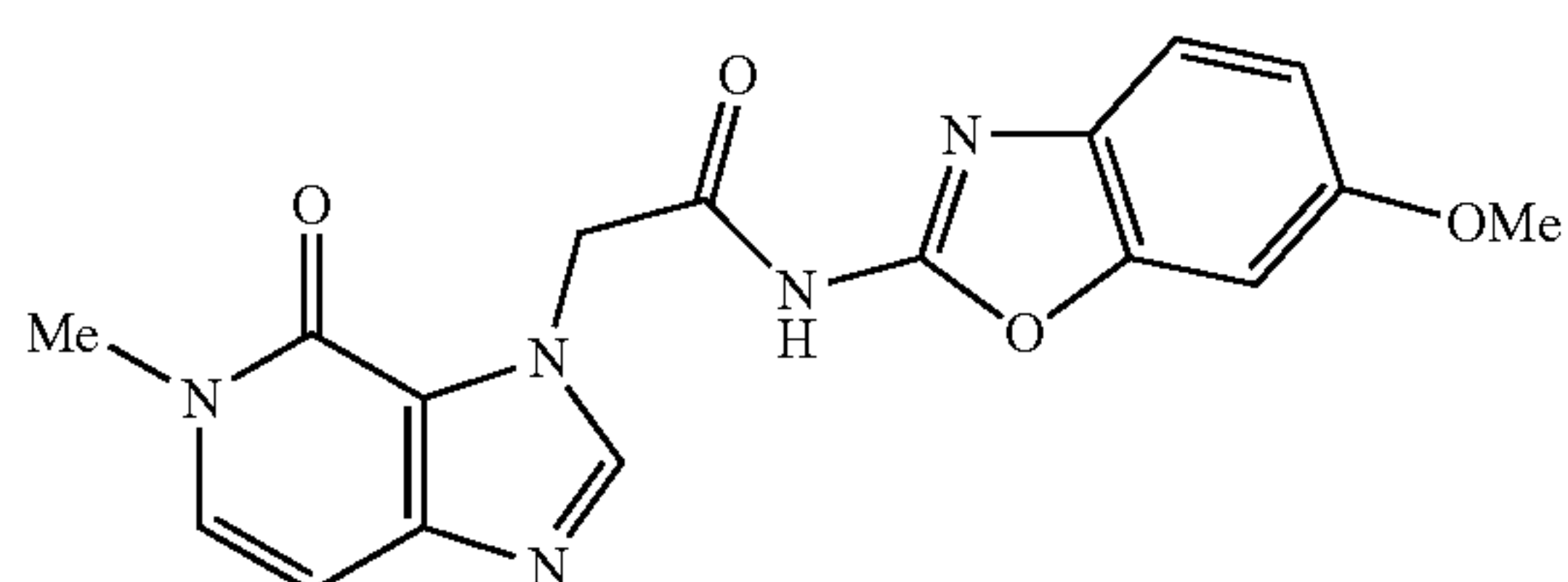
N-(6-methoxybenzo[d]oxazol-2-yl)-2-(5-methyl-4-oxo-4,5-dihydro-3H-imidazo[4,5-c]pyridin-3-yl)acetamide
