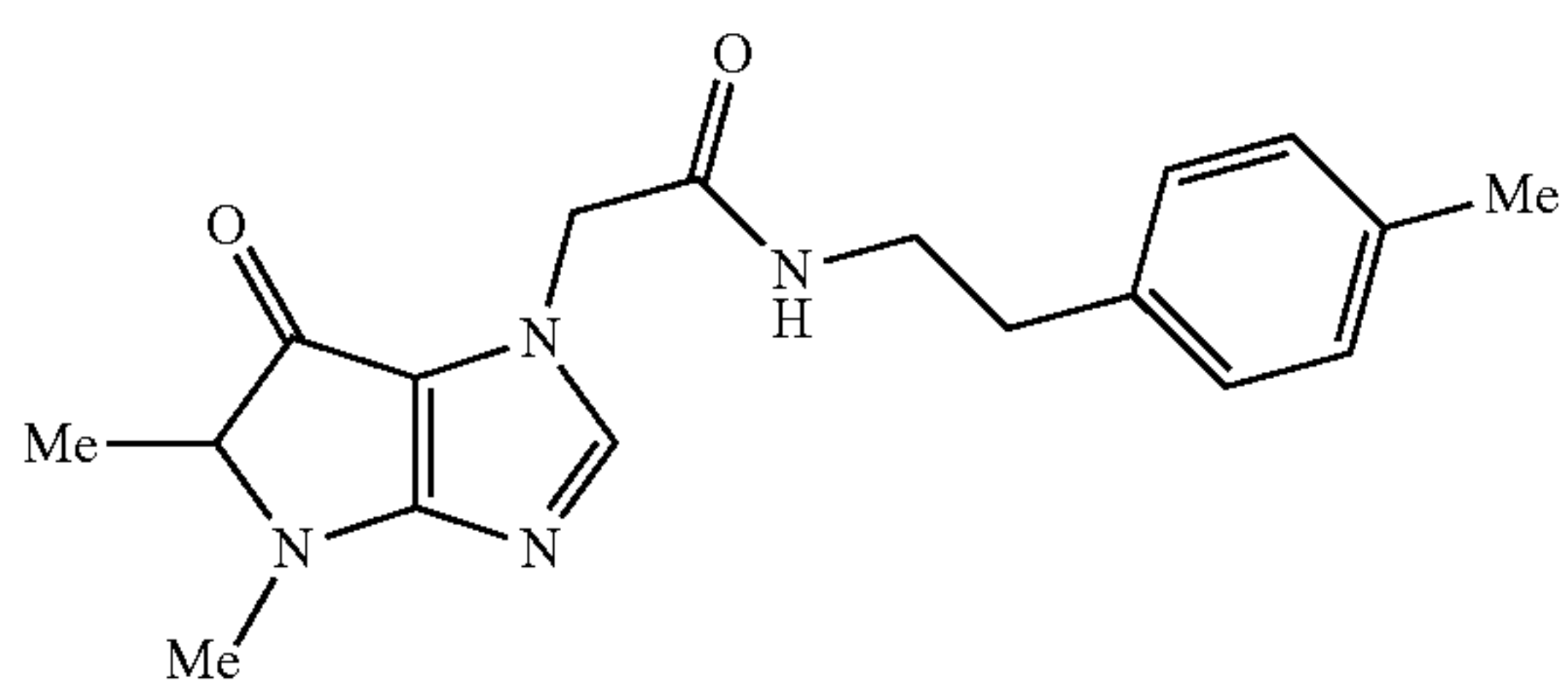
2-(4,5-dimethyl-6-oxo-5,6-dihydropyrrolo[3,2-d]imidazol-1(4H)-yl)-N-(4-methylphenethyl)acetamide
