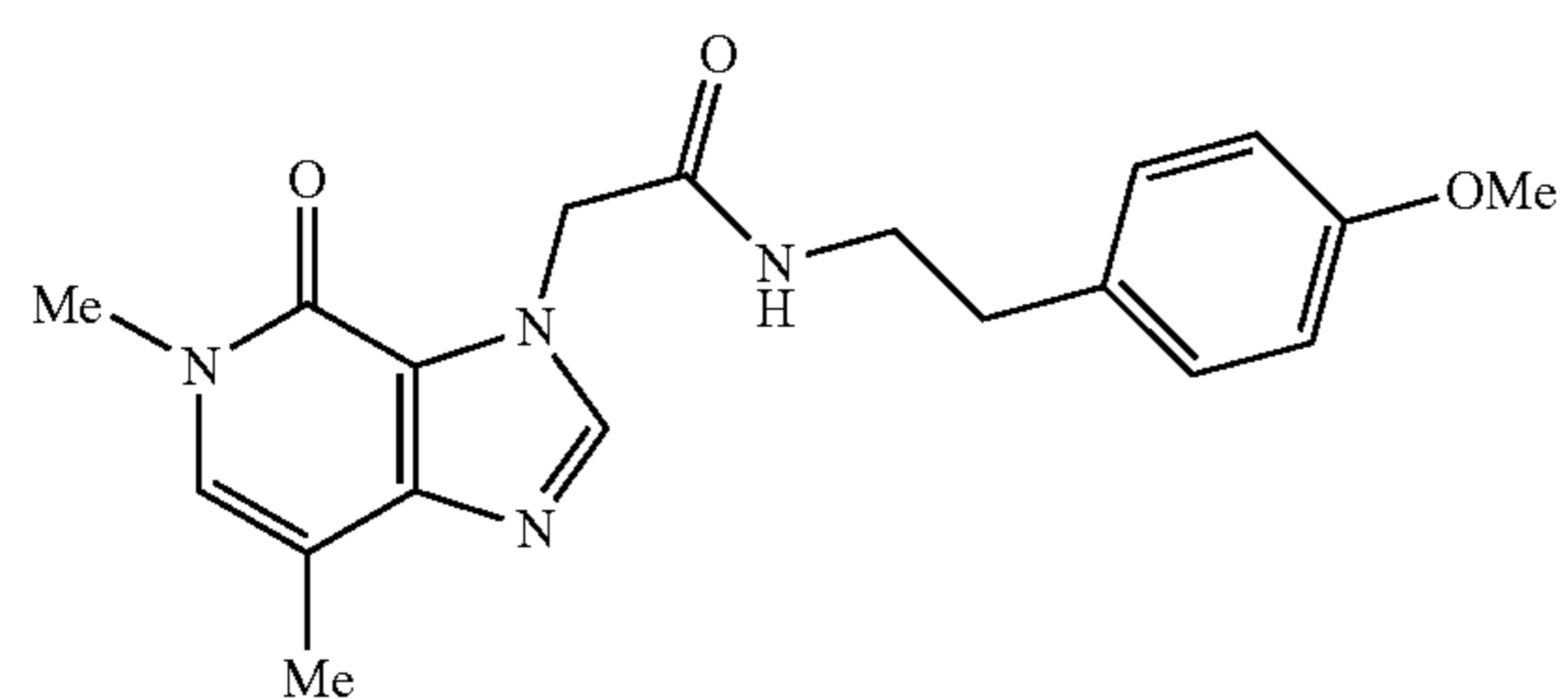
2-(5,7-dimethyl-4-oxo-4,5-dihydro-3H-imidazo[4,5-c]pyridin-3-yl)-N-(4-methoxyphenethyl)acetamide
