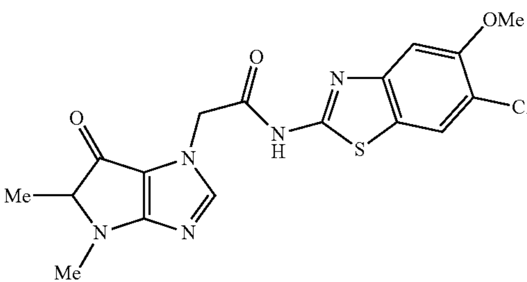
N-(6-chloro-5-methoxybenzo[d]thiazol-2-yl)-2-(4,5-dimethyl-6-oxo-5,6-dihydropyrrolo[3,2-d]imidazol-1(4H)-yl)acetamide
