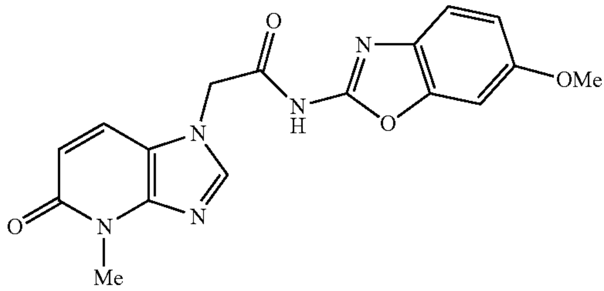
N-(6-methoxybenzo[d]oxazol-2-yl)-2-(4-methyl-5-oxo-4,5-dihydro-1H-imidazo[4,5-b]pyridin-1-yl)acetamide
