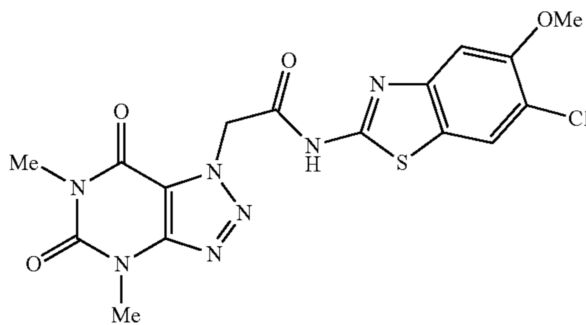
N-(6-chloro-5-methoxybenzo[d]thiazol-2-yl)-2-(4,6-dimethyl-5,7-dioxo-4,5,6,7-tetrahydro-1H-[1,2,3]triazolo[4,5-d]pyrimidin-1-yl)acetamide
