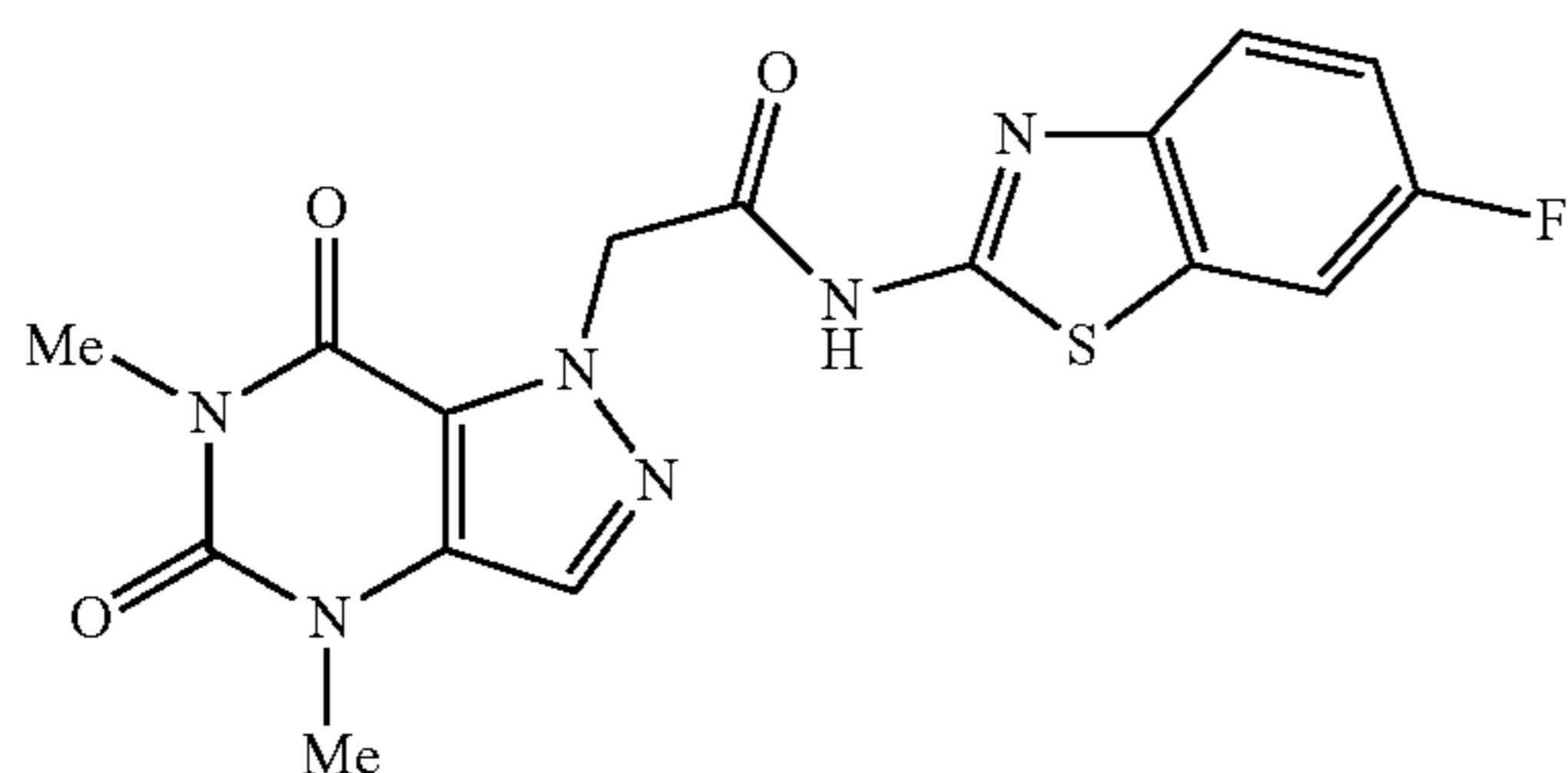
2-(4,6-dimethyl-5,7-dioxo-4,5,6,7-tetrahydro-1H-pyrazolo[4,3-d]pyrimidin-1-yl)-N-(6-fluorobenzo[d]thiazol-2-yl)acetamide
