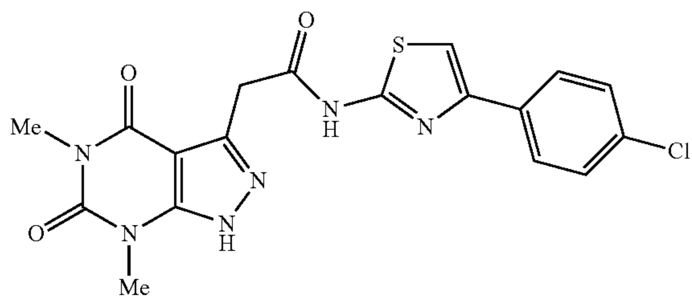
N-(4-(4-chlorophenyl)thiazol-2-yl)-2-(5,7-dimethyl-4,6-dioxo-4,5,6,7-tetrahydro-1H-pyrazolo[3,4-d]pyrimidin-3-yl)acetamide
