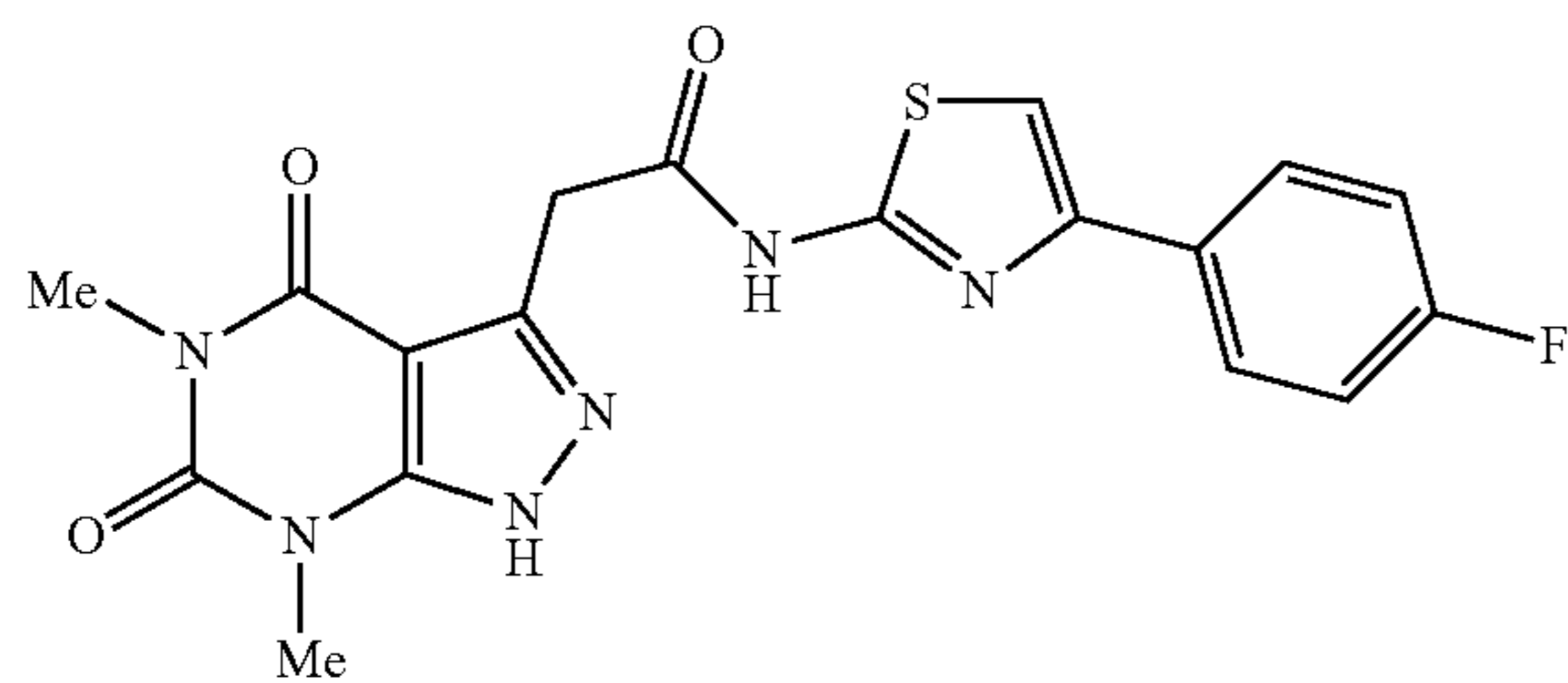
2-(5,7-dimethyl-4,6-dioxo-4,5,6,7-tetrahydro-1H-pyrazolo[3,4-d]pyrimidin-3-yl)-N-(4-(4-fluorophenyl)thiazol-2-yl)acetamide
