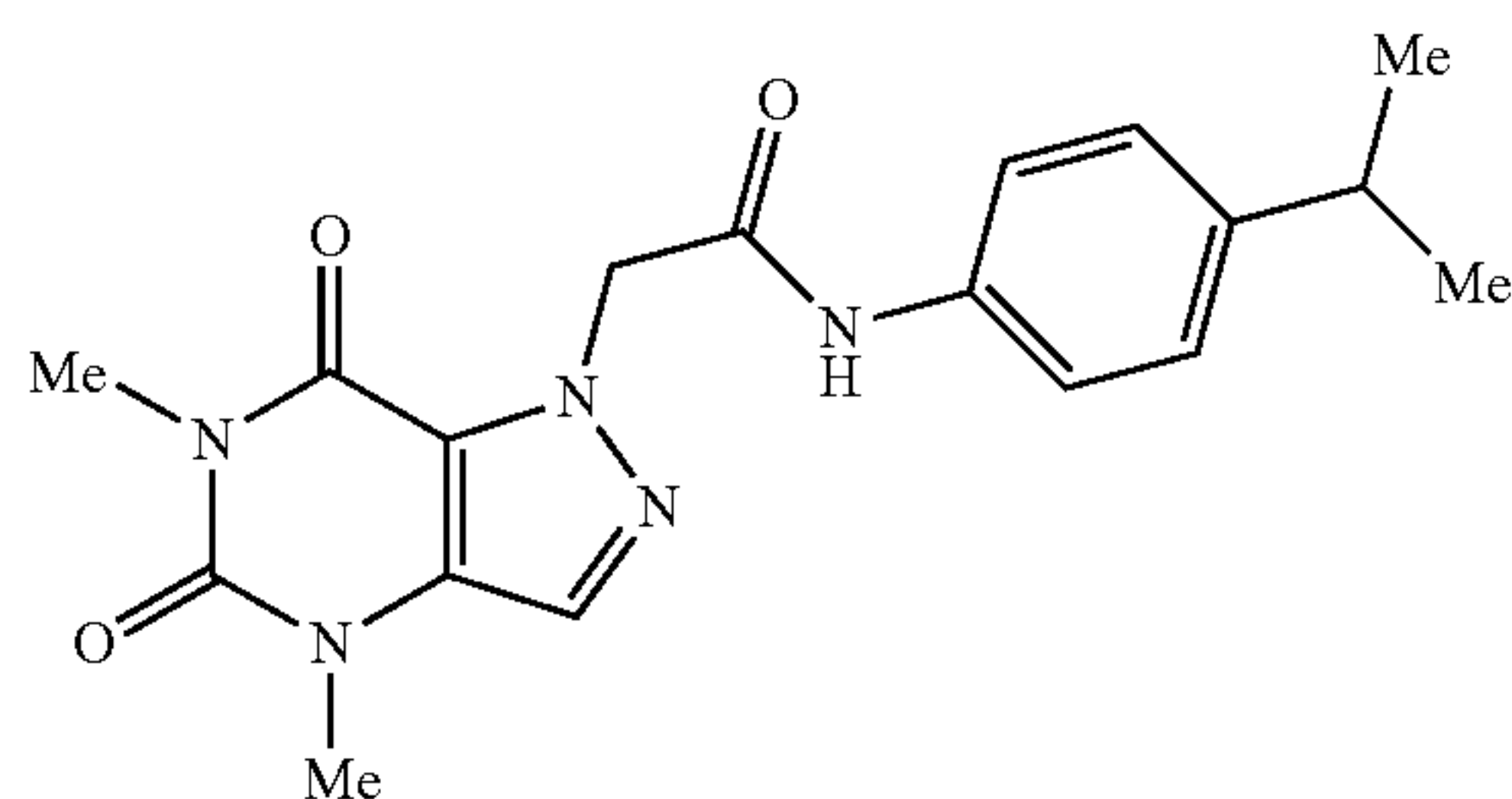
2-(4,6-dimethyl-5,7-dioxo-4,5,6,7-tetrahydro-1H-pyrazolo[4,3-d]pyrimidin-1-yl)-N-(4-isopropylphenyl)acetamide
