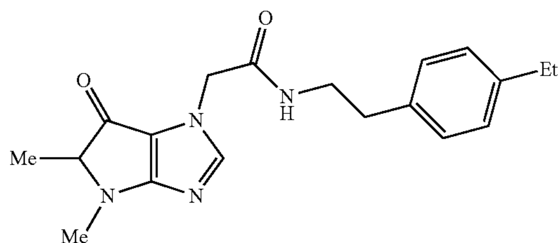
2-(4,5-dimethyl-6-oxo-5,6-dihydropyrrolo[3,2-d]imidazol-1(4H)-yl)-N-(4-ethylphenethyl)acetamide
