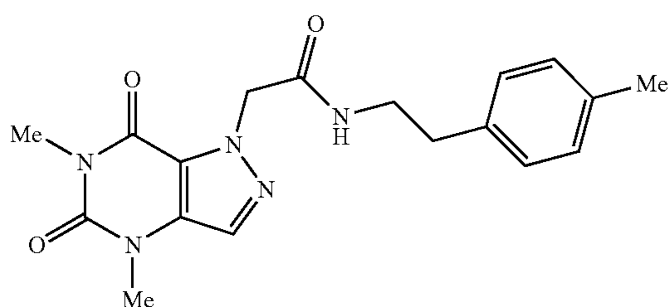
2-(4,6-dimethyl-5,7-dioxo-4,5,6,7-tetrahydro-1H-pyrazolo[4,3-d]pyrimidin-1-yl)-N-(4-methylphenethyl)acetamide
