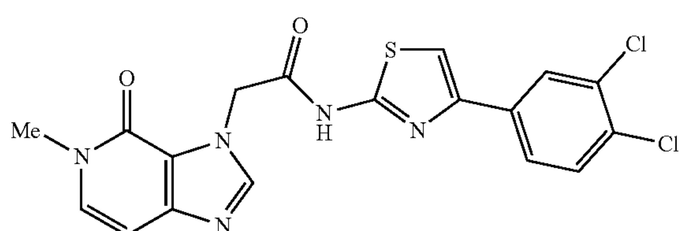
N-(4-(3,4-dichlorophenyl)thiazol-2-yl)-2-(5-methyl-4-oxo-4,5-dihydro-3H-imidazo[4,5-c]pyridin-3-yl)acetamide
