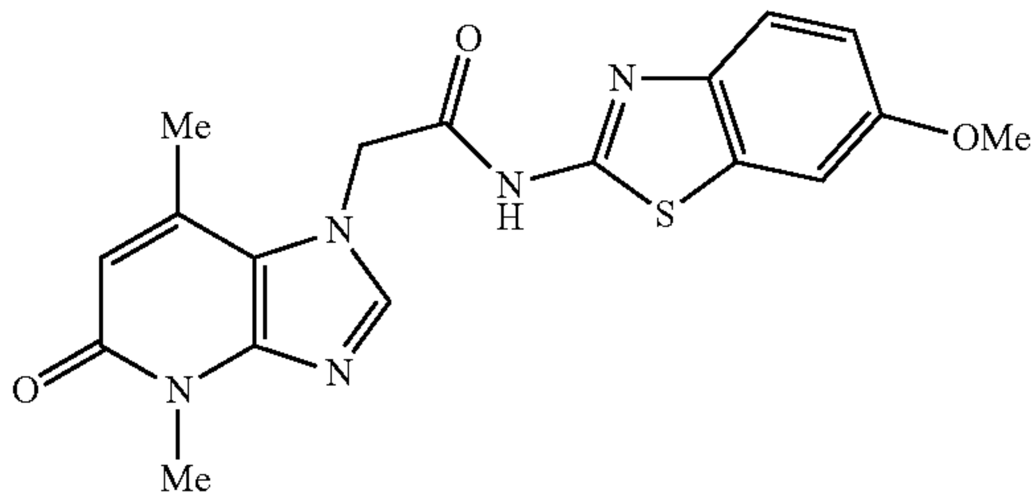
2-(4,7-dimethyl-5-oxo-4,5-dihydro-1H-imidazo[4,5-b]pyridin-1-yl)-N-(6-methoxybenzo[d]thiazol-2-yl)acetamide
