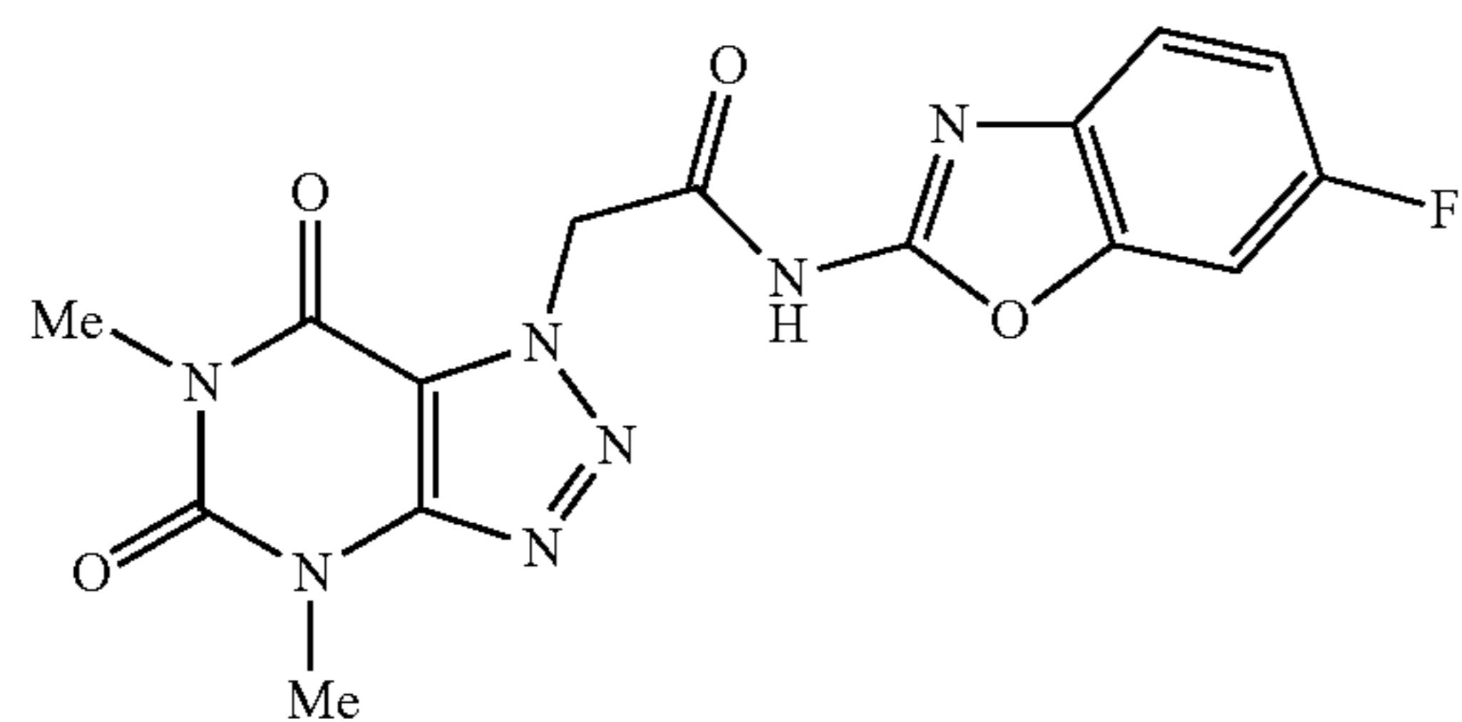
2-(4,6-dimethyl-5,7-dioxo-4,5,6,7-tetrahydro-1H-[1,2,3]triazolo[4,5-d]pyrimidin-1-yl)-N-(6-fluorobenzo[d]oxazol-2-yl)acetamide
