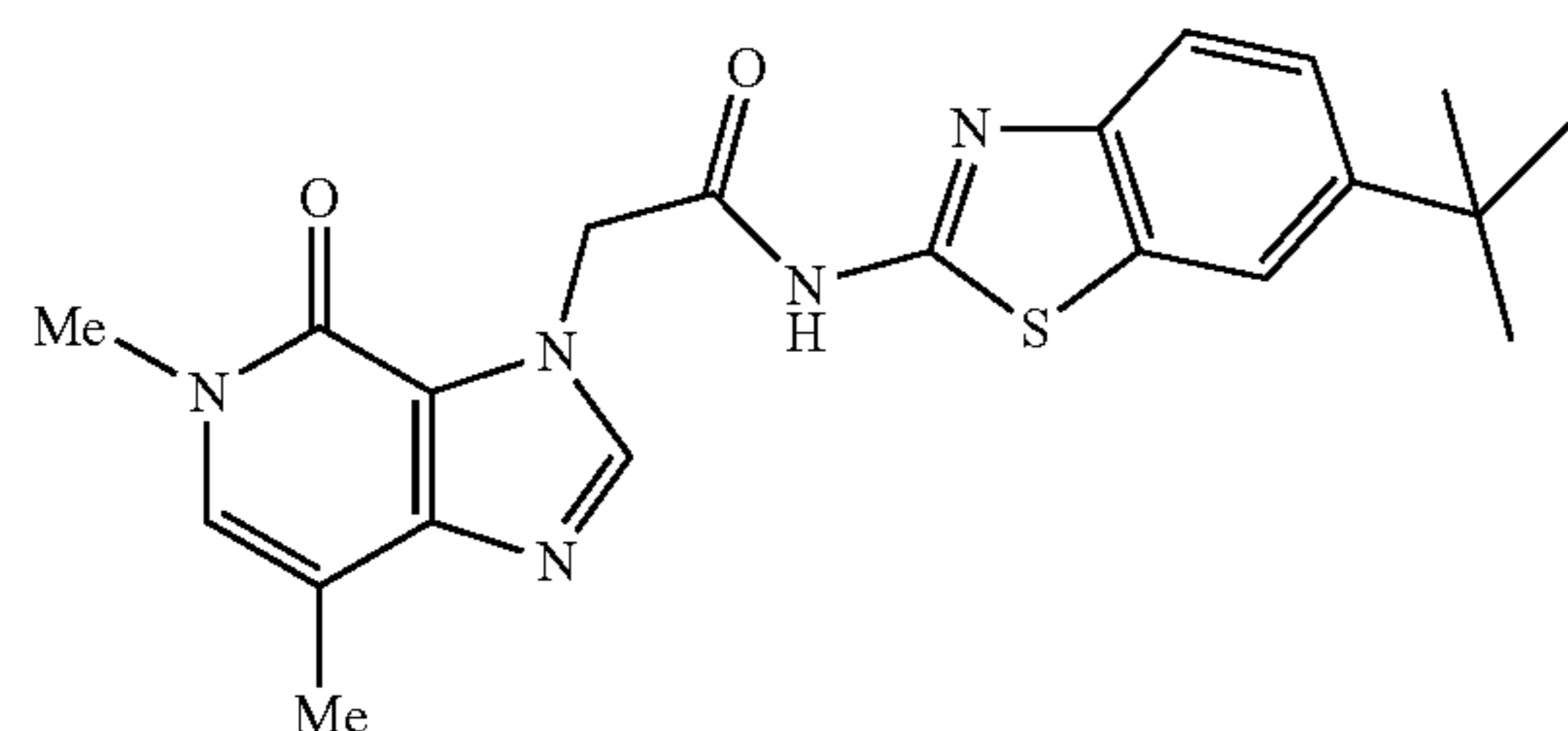
N-(6-tert-butylbenzo[d]thiazol-2-yl)-2-(5,7-dimethyl-4-oxo-4,5-dihydro-3H-imidazo[4,5-c]pyridin-3-yl)acetamide
