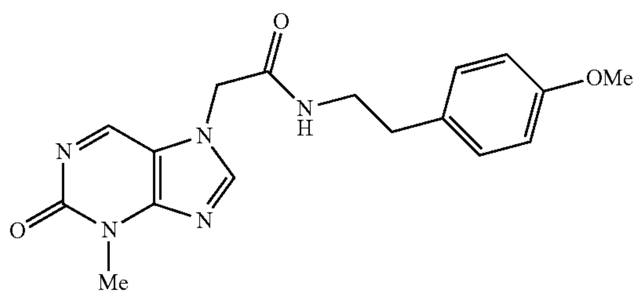
N-(4-methoxyphenethyl)-2-(3-methyl-2-oxo-2,3-dihydropurin-7-yl)acetamide
