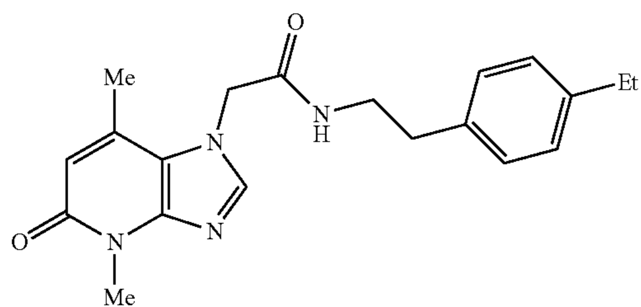
2-(4,7-dimethyl-5-oxo-4,5-dihydro-1H-imidazo[4,5-b]pyridin-1-yl)-N-(4-ethylphenethyl)acetamide
