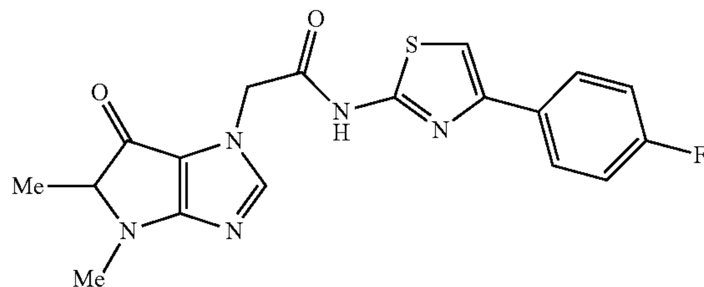
2-(4,5-dimethyl-6-oxo-5,6-dihydropyrrolo[3,2-d]imidazol-1(4H)-yl)-N-(4-(4-fluorophenyl)thiazol-2-yl)acetamide
