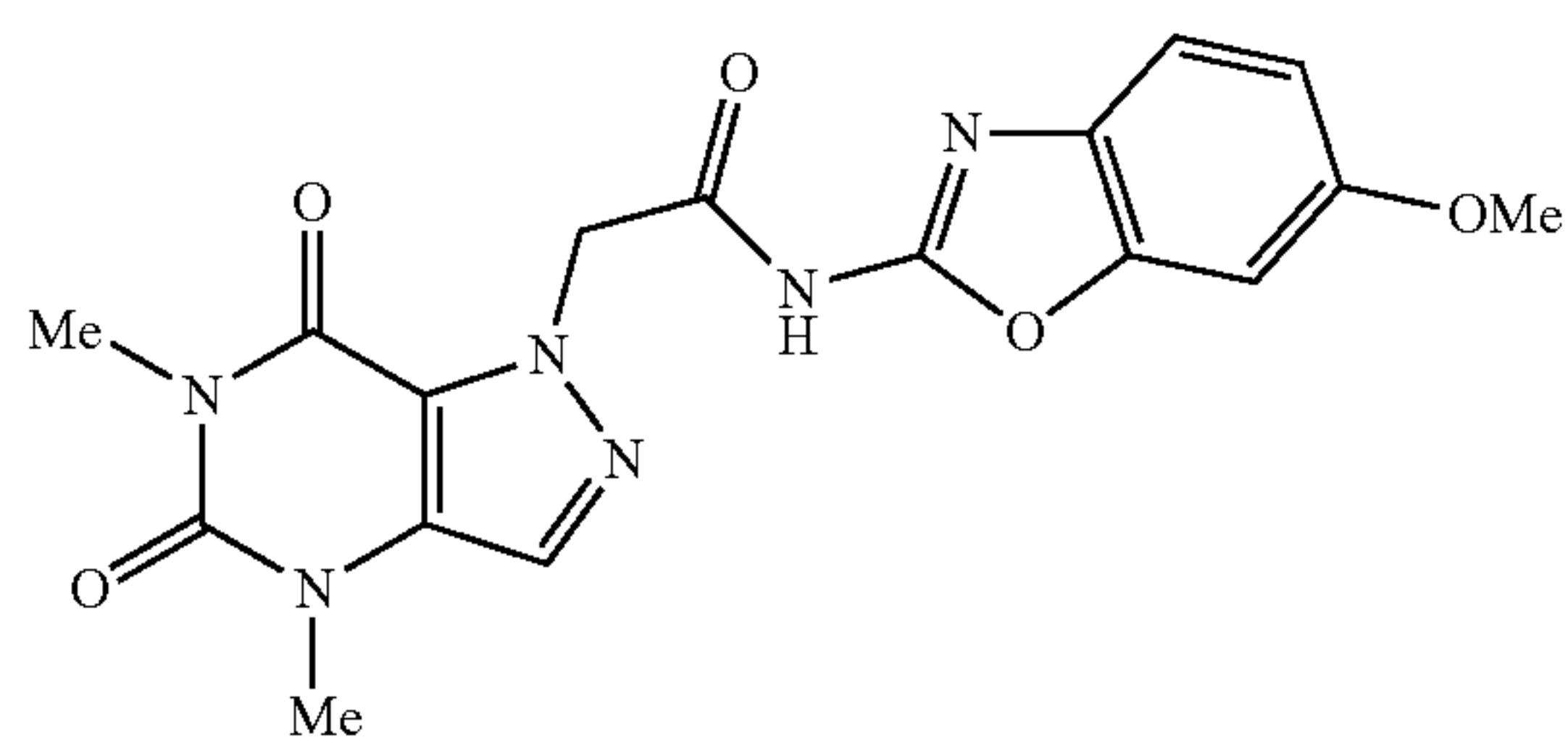
2-(4,6-dimethyl-5,7-dioxo-4,5,6,7-tetrahydro-1H-pyrazolo[4,3-d]pyrimidin-1-yl)-N-(6-methoxybenzo[d]oxazol-2-yl)acetamide
