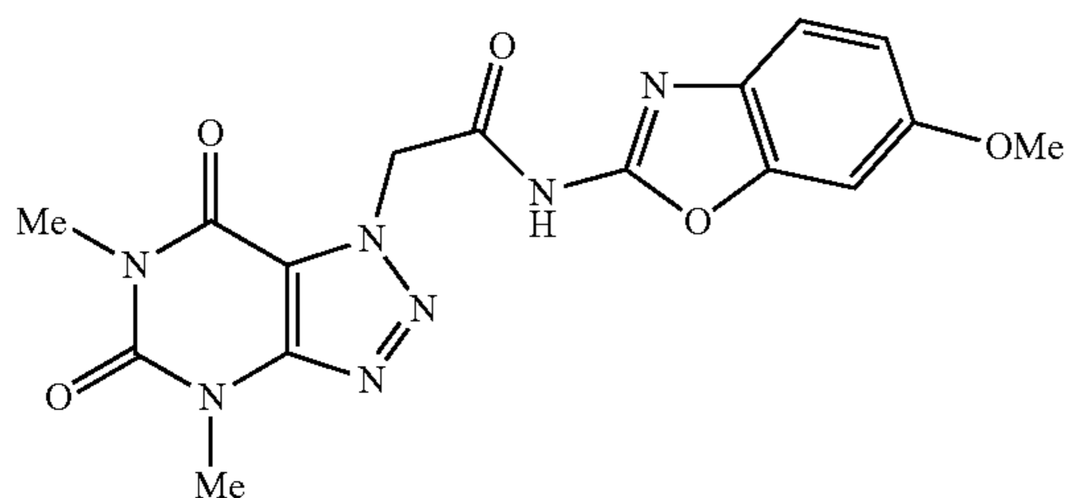
2-(4,6-dimethyl-5,7-dioxo-4,5,6,7-tetrahydro-1H-[1,2,3]triazolo[4,5-d]pyrimidin-1-yl)-N-(6-methoxybenzo[d]oxazol-2-yl)acetamide
