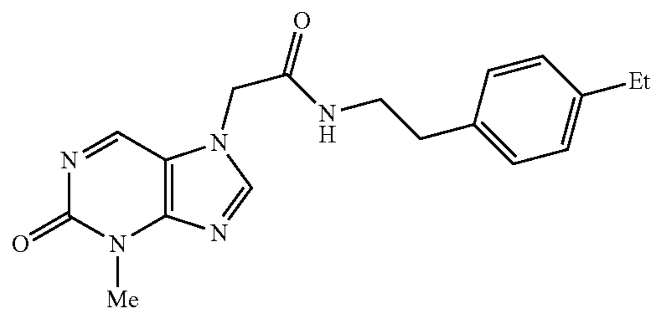
N-(4-ethylphenethyl)-2-(3-methyl-2-oxo-2,3-dihydropurin-7-yl)acetamide
