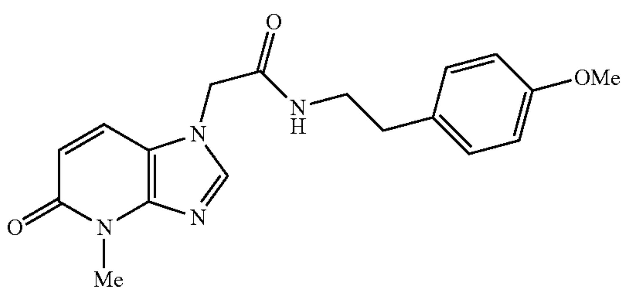
N-(4-methoxyphenethyl)-2-(4-methyl-5-oxo-4,5-dihydro-1H-imidazo[4,5-b]pyridin-1-yl)acetamide
