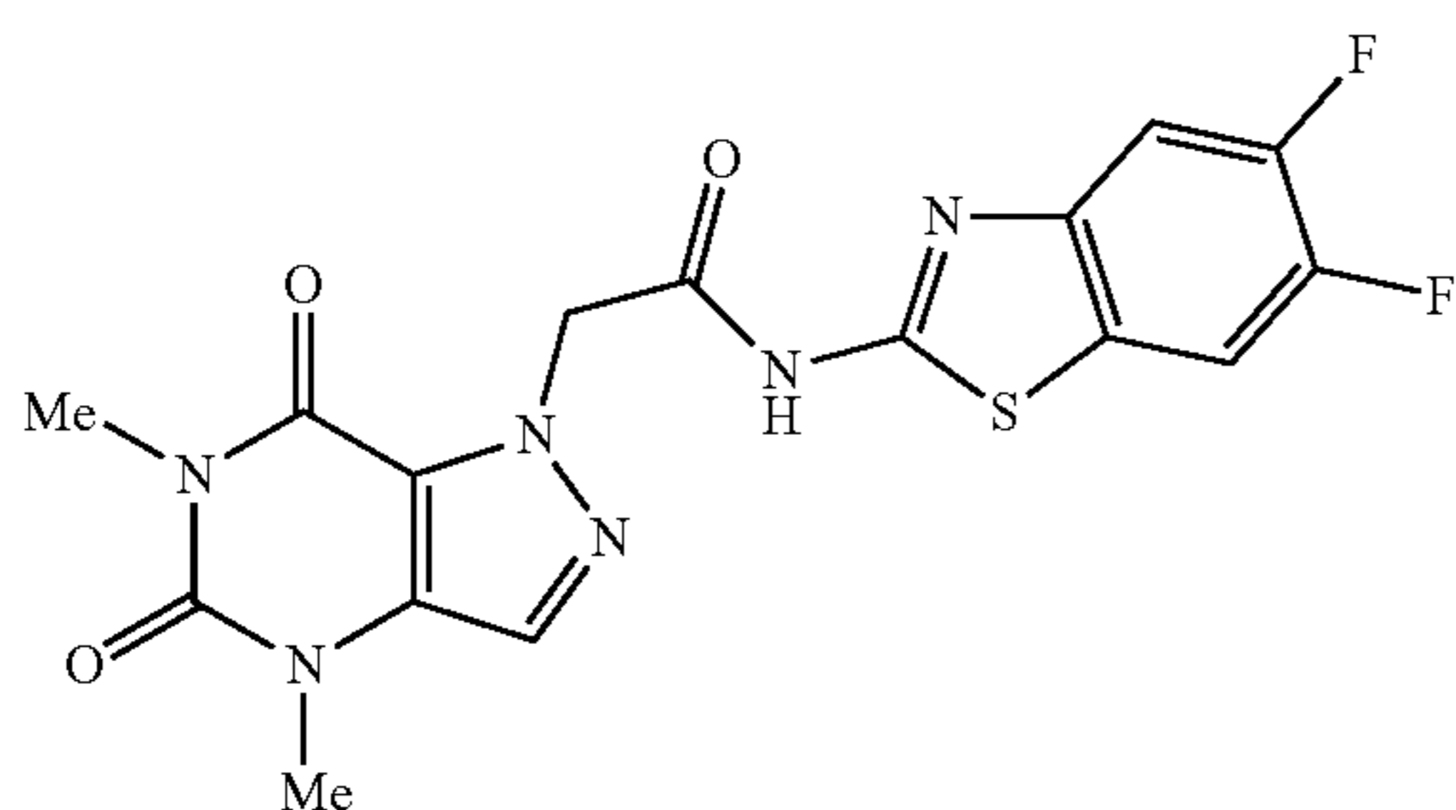
N-(5,6-difluorobenzo[d]thiazol-2-yl)-2-(4,6-dimethyl-5,7-dioxo-4,5,6,7-tetrahydro-1H-pyrazolo[4,3-d]pyrimidin-1-yl)acetamide
