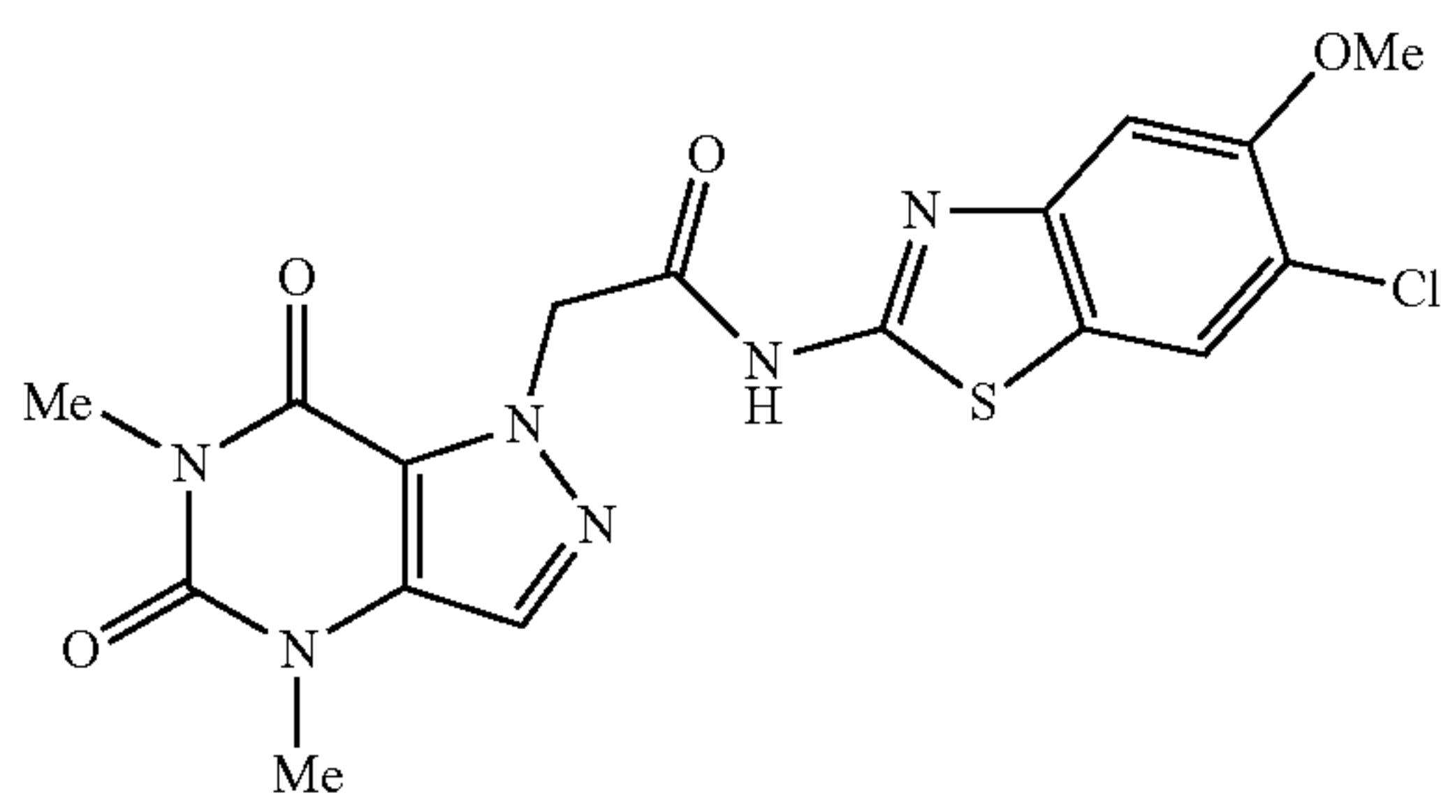
N-(6-chloro-5-methoxybenzo[d]thiazol-2-yl)-2-(4,6-dimethyl-5,7-dioxo-4,5,6,7-tetrahydro-1H-pyrazolo[4,3-d]pyrimidin-1-yl)acetamide
