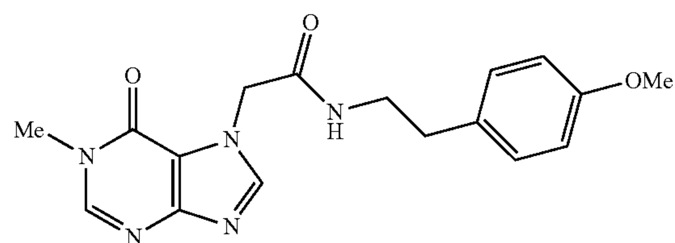
N-(4-methoxyphenethyl)-2-(1-methyl-6-oxo-1H-purin-7(6H)-yl)acetamide
