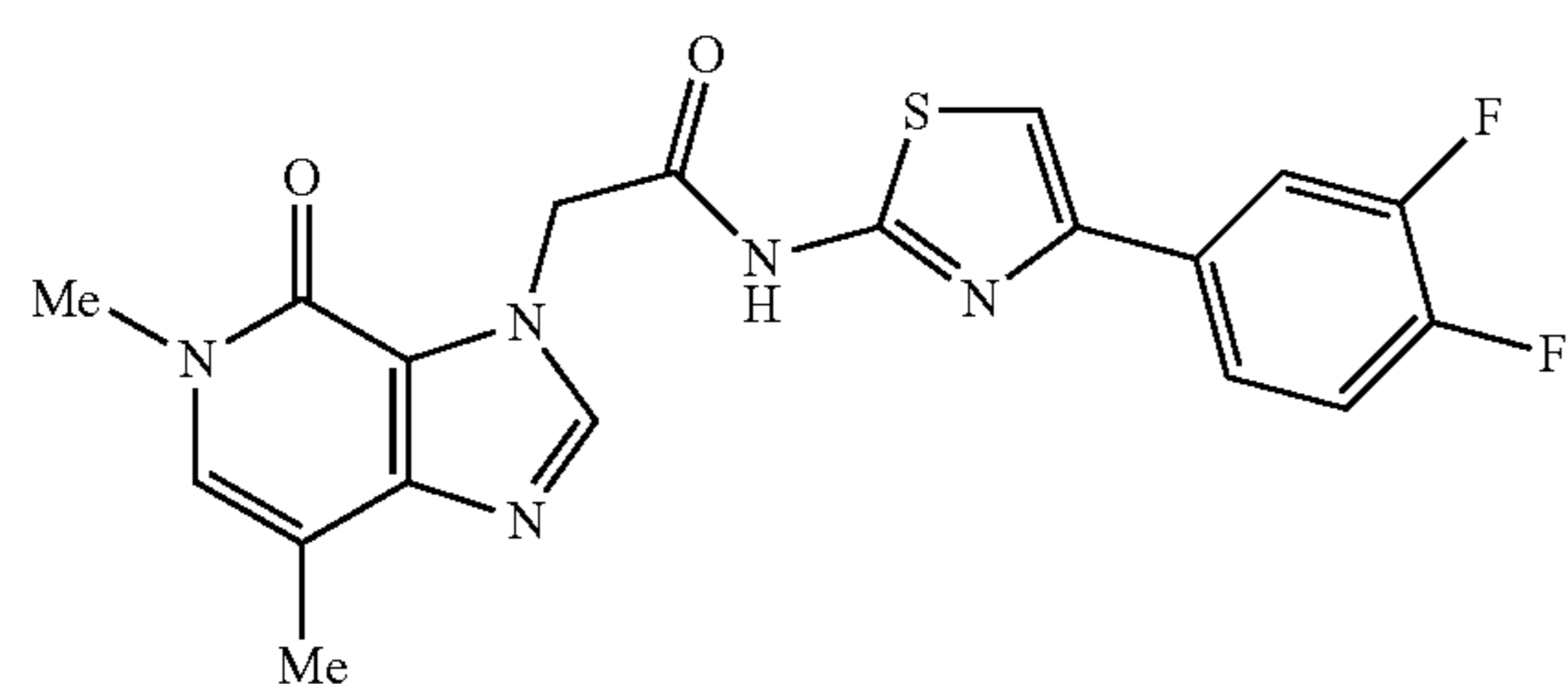
N-(4-(3,4-difluorophenyl)thiazol-2-yl)-2-(5,7-dimethyl-4-oxo-4,5-dihydro-3H-imidazo[4,5-c]pyridin-3-yl)acetamide
