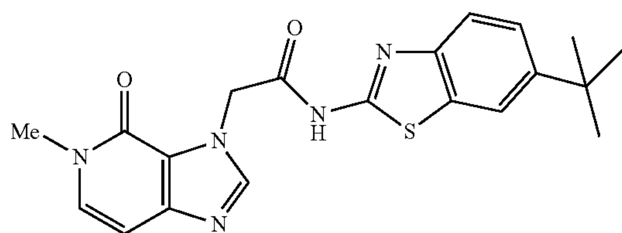
N-(6-tert-butylbenzo[d]thiazol-2-yl)-2-(5-methyl-4-oxo-4,5-dihydro-3H-imidazol[4,5-c]pyridin-3-yl)acetamide
