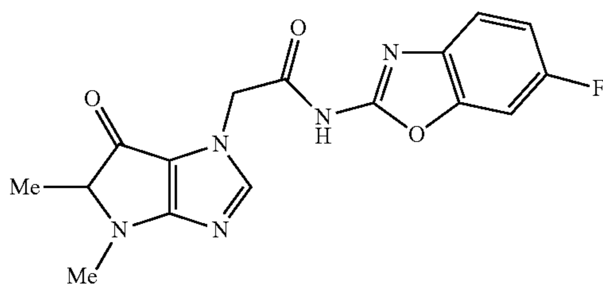
2-(4,5-dimethyl-6-oxo-5,6-dihydropyrrolo[3,2-d]imidazol-1(4H)-yl)-N-(6-fluorobenzo[d]oxazol-2-yl)acetamide
