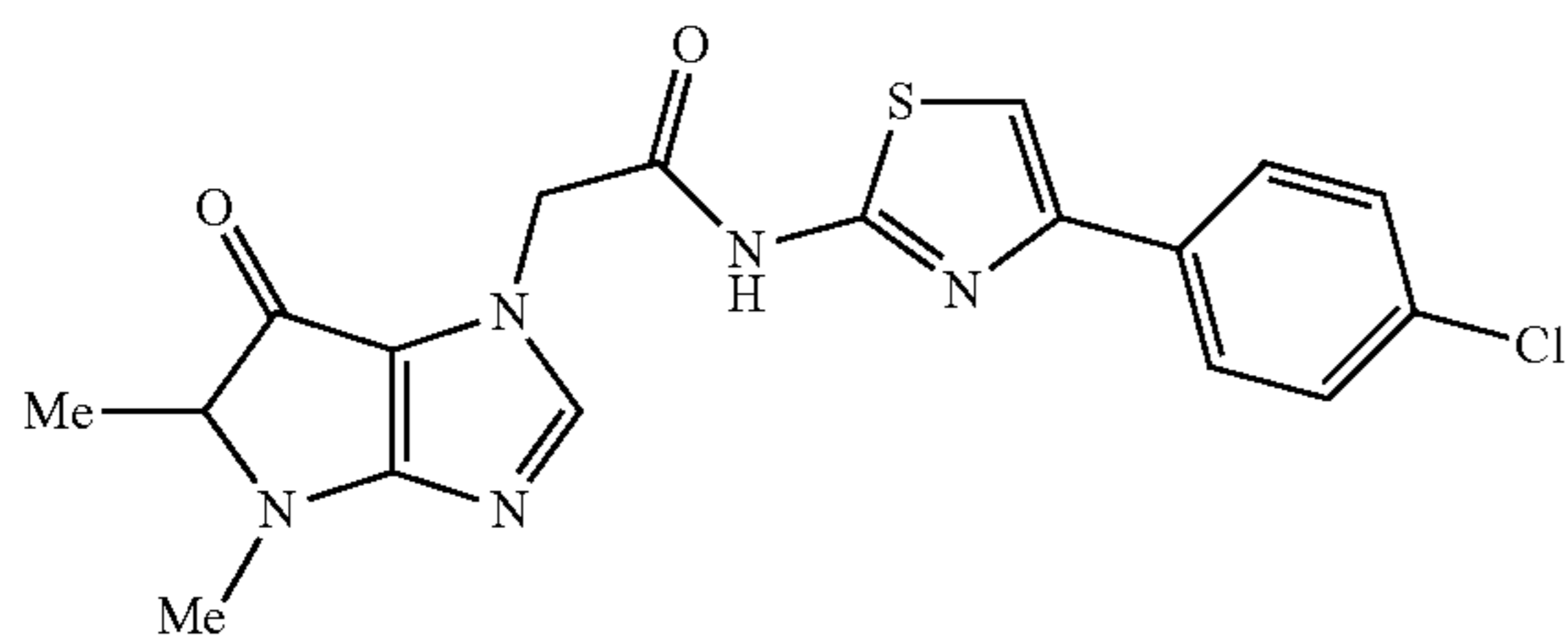
N-(4-(4-chlorophenyl)thiazol-2-yl)-2-(4,5-dimethyl-6-oxo-5,6-dihydropyrrolo[3,2-d]imidazol-1(4H)-yl)acetamide
