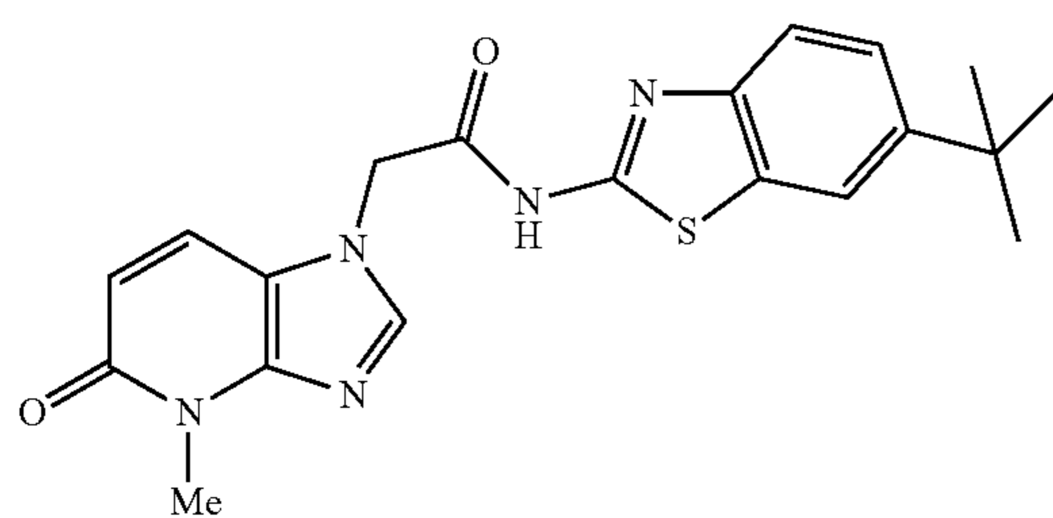
N-(6-tert-butylbenzo[d]thiazol-2-yl)-2-(4-methyl-5-oxo-4,5-dihydro-1H-imidazo[4,5-b]pyridin-1-yl)acetamide
