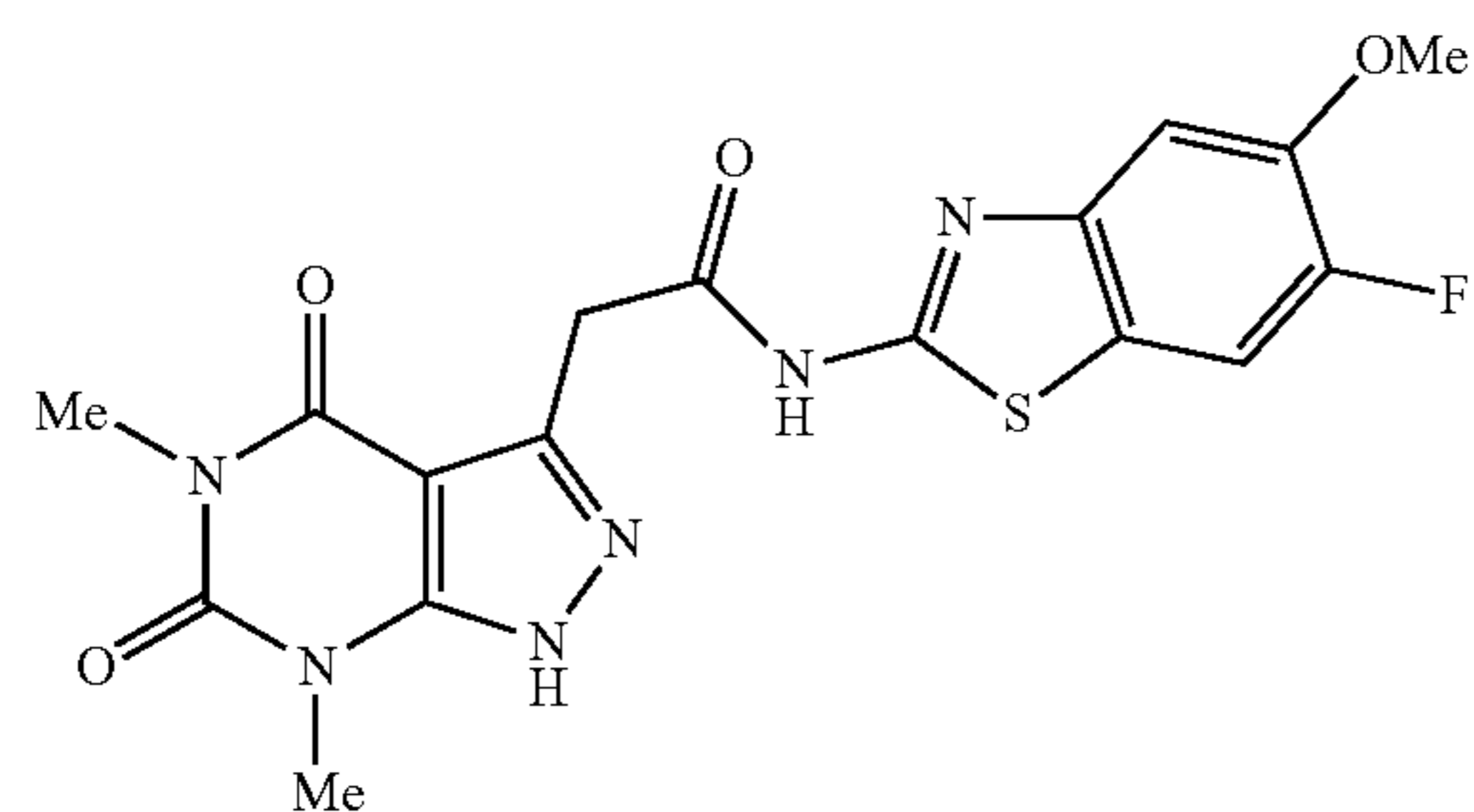
2-(5,7-dimethyl-4,6-dioxo-4,5,6,7-tetrahydro-1H-pyrazolo[3,4-d]pyrimidin-3-yl)-N-(6-fluoro-5-methoxybenzo[d]thiazol-2-yl)acetamide
