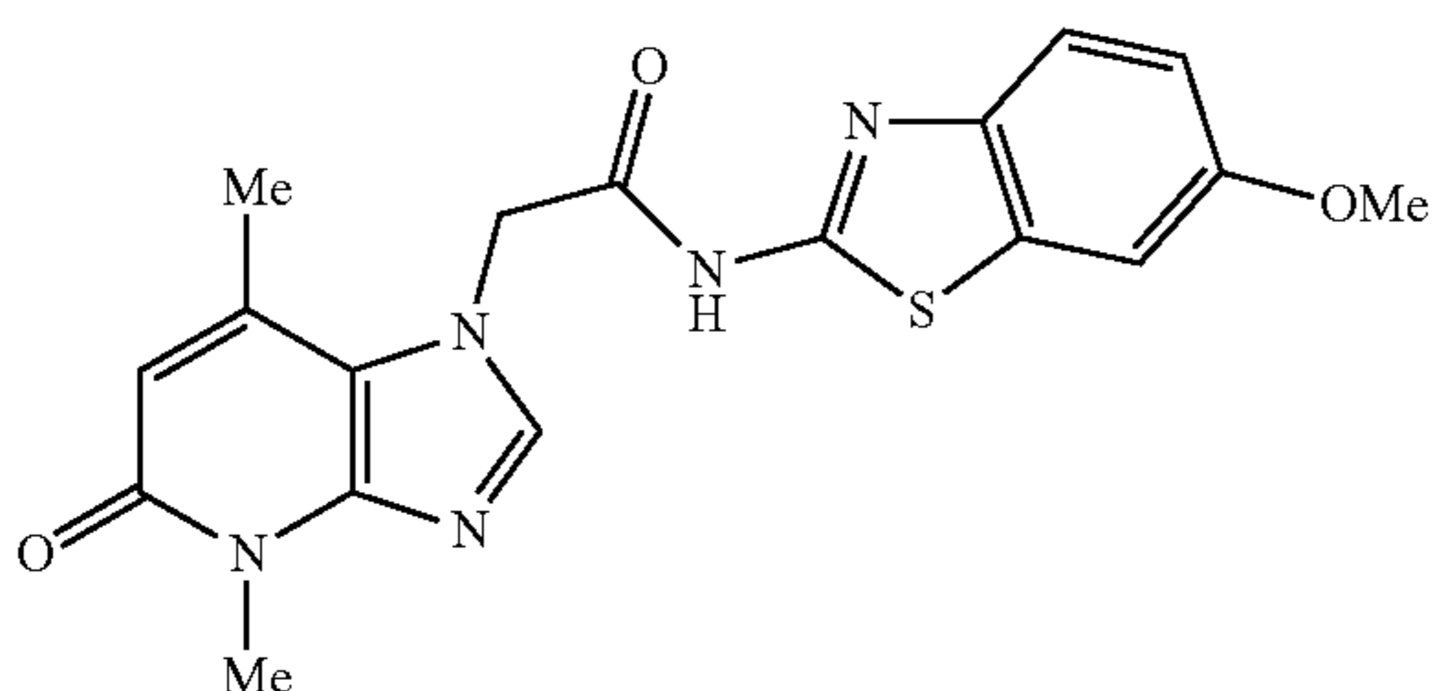
2-(4,7-dimethyl-5-oxo-4,5-dihydro-1H-imidazo[4,5-b]pyridin-1-yl)-N-(6-methoxybenzo[d]thiazol-2-yl)acetamide
