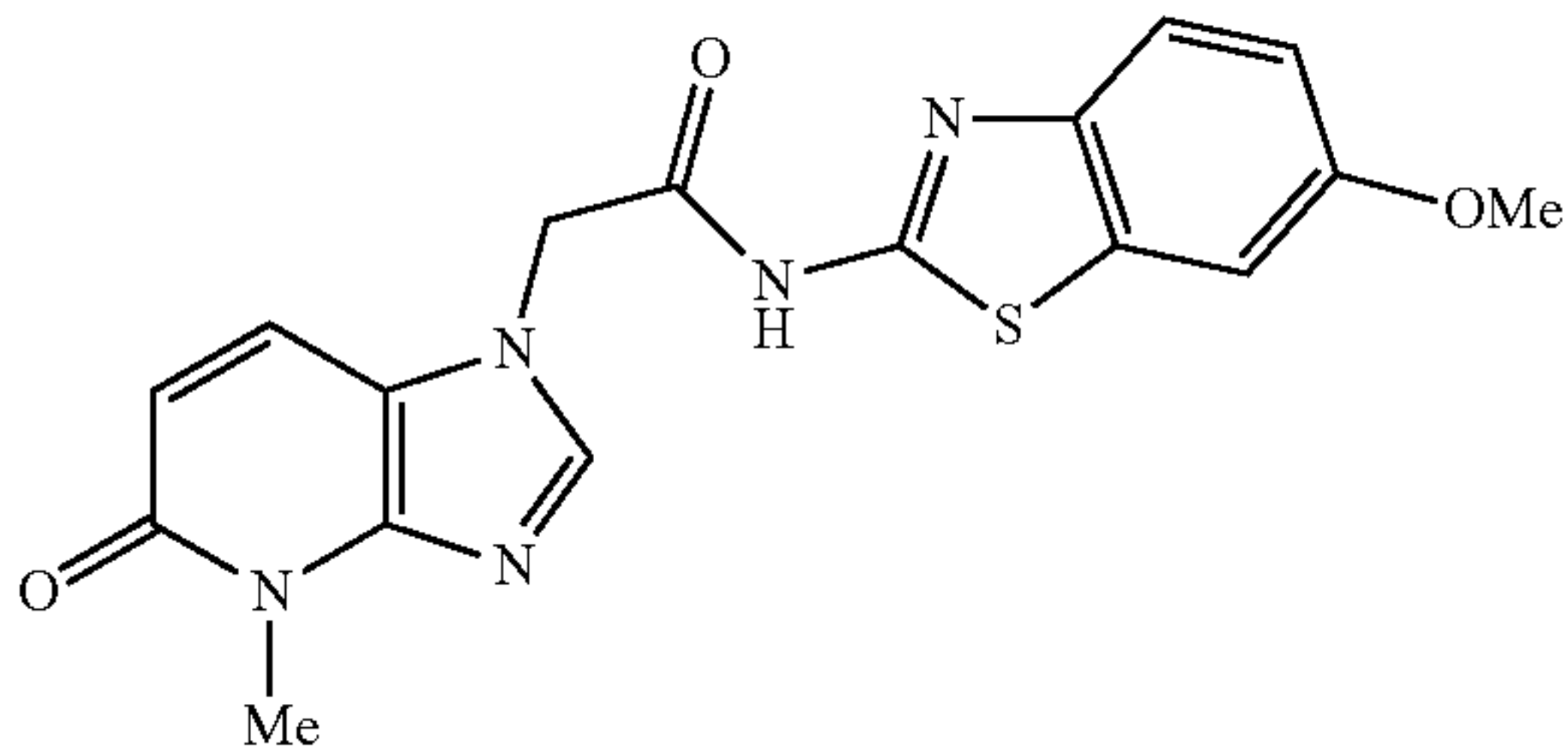
N-(6-methoxybenzo[d]thiazol-2-yl)-2-(4-methyl-5-oxo-4,5-dihydro-1H-imidazo[4,5-b]pyridin-1-yl)acetamide
