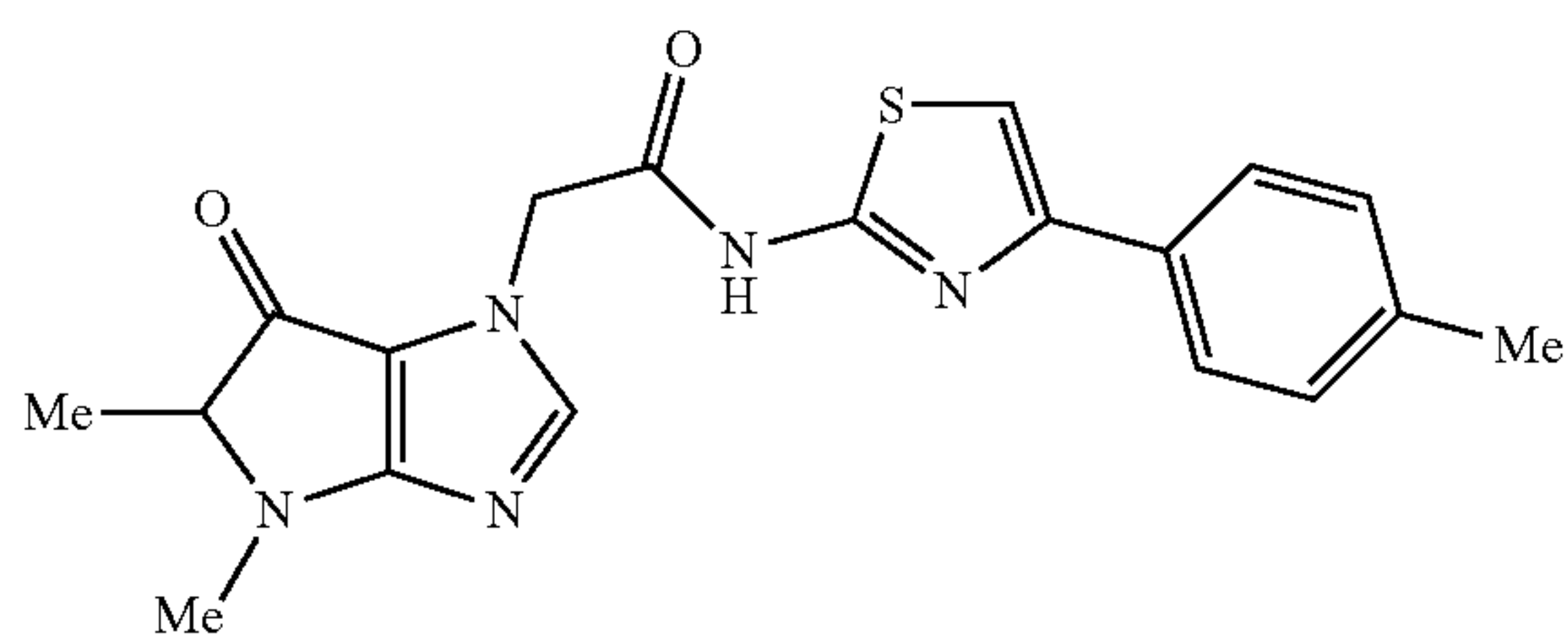
2-(4,5-dimethyl-6-oxo-5,6-dihydropyrrolo[3,2-d]imidazol-1(4H)-yl)-N-(4-p-tolylthiazol-2-yl)acetamide
