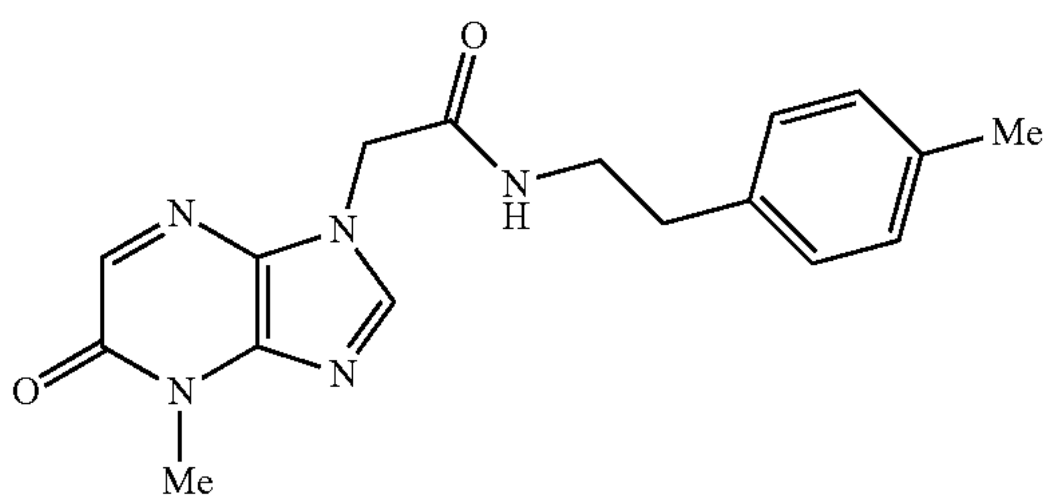
2-(4-methyl-5-oxo-4,5-dihydro-1H-imidazo[4,5-b]pyrazin-1-yl)-N-(4-methylphenethyl)acetamide
