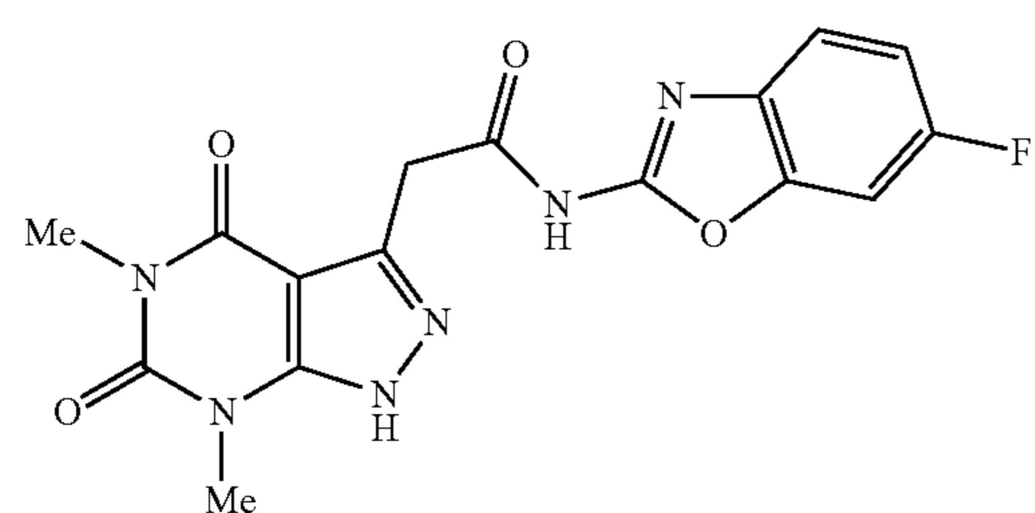
2-(5,7-dimethyl-4,6-dioxo-4,5,6,7-tetrahydro-1H-pyrazolo[3,4-d]pyrimidin-3-yl)-N-(6-fluorobenzo[d]oxazol-2-yl)acetamide
