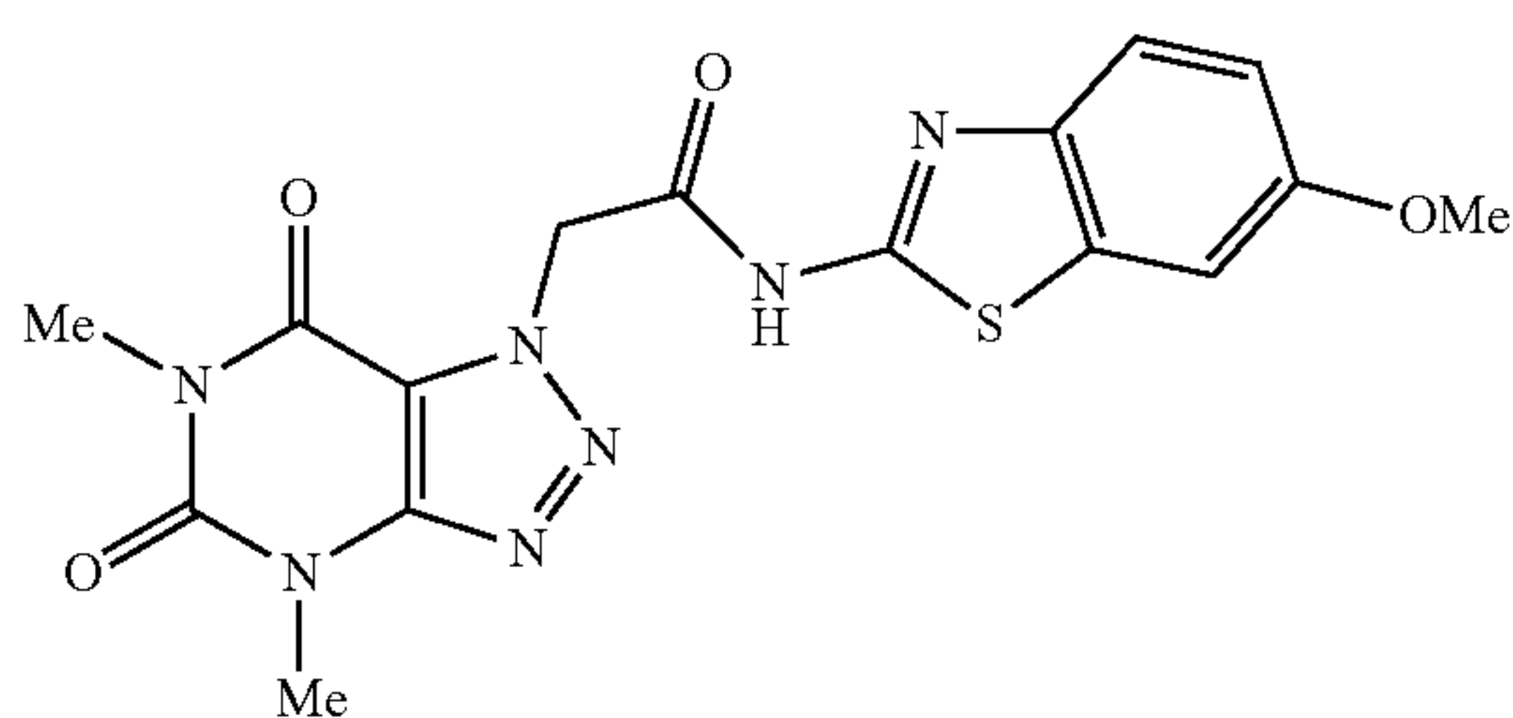
2-(4,6-dimethyl-5,7-dioxo-4,5,6,7-tetrahydro-1H-[1,2,3]triazolo[4,5-d]pyrimidin-1-yl)-N-(6-methoxybenzo[d]thiazol-2-yl)acetamide
