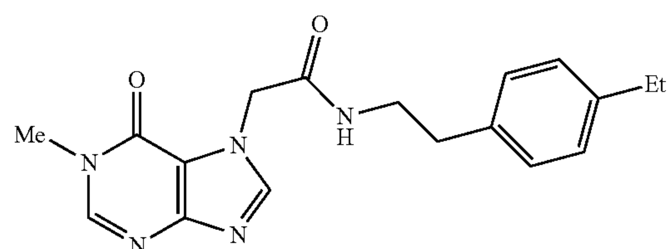
N-(4-ethylphenethyl)-2-(1-methyl-6-oxo-1H-purin-7(6H)-yl)acetamide
