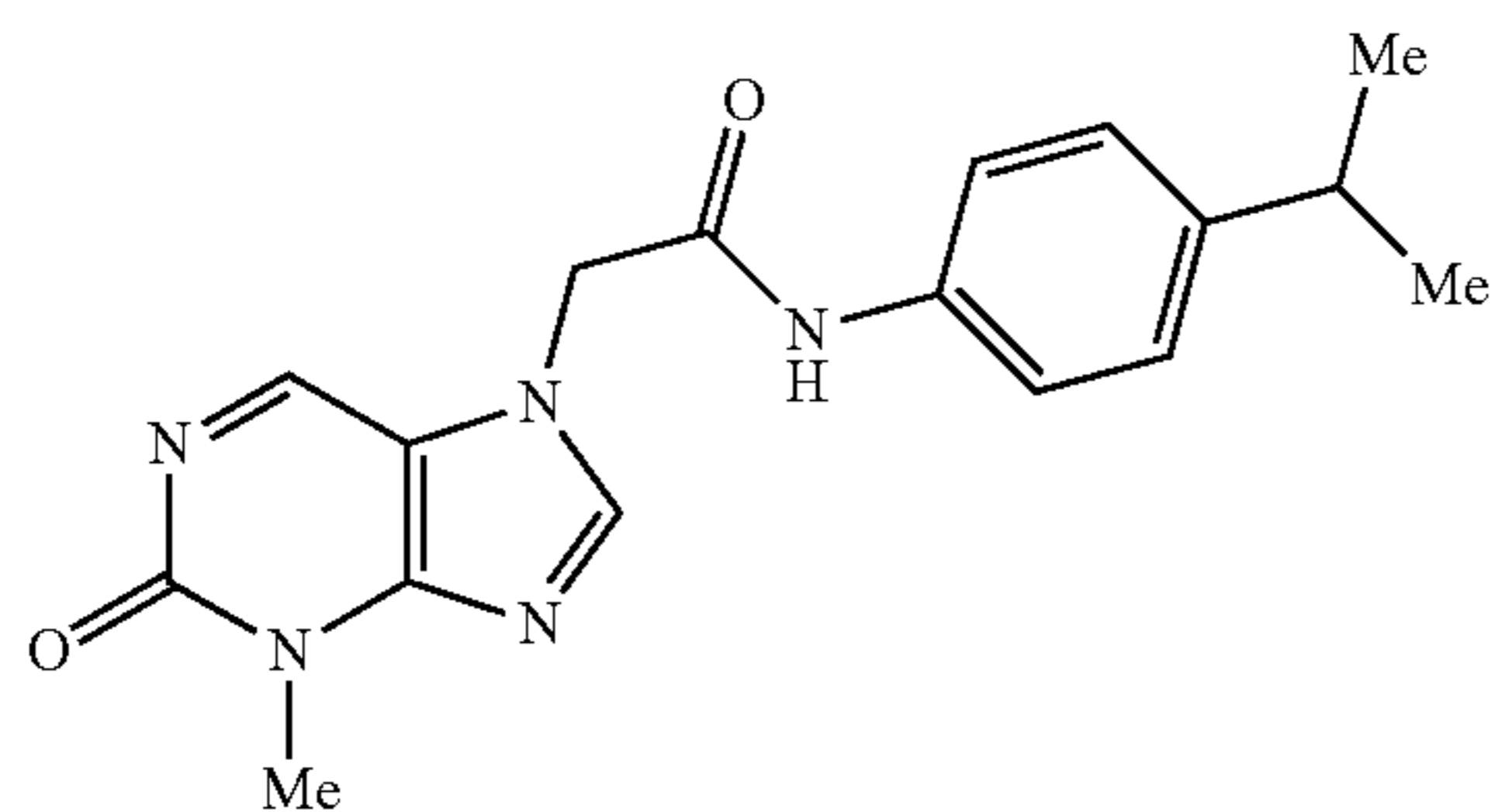
N-(4-isopropylphenyl)-2-(3-methyl-2-oxo-2,3-dihydropurin-7-yl)acetamide
