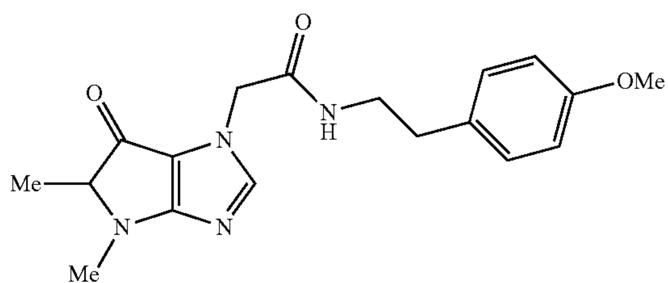
2-(4,5-dimethyl-6-oxo-5,6-dihydropyrrolo[3,2-d]imidazol-1(4H)-yl)-N-(4-methoxyphenethyl)acetamide
