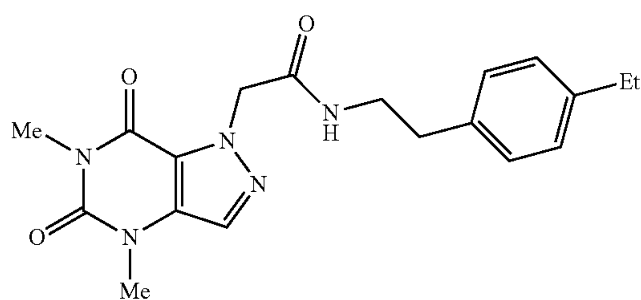
2-(4,6-dimethyl-5,7-dioxo-4,5,6,7-tetrahydro-1H-pyrazolo[4,3-d]pyrimidin-1-yl)-N-(4-ethylphenethyl)acetamide
