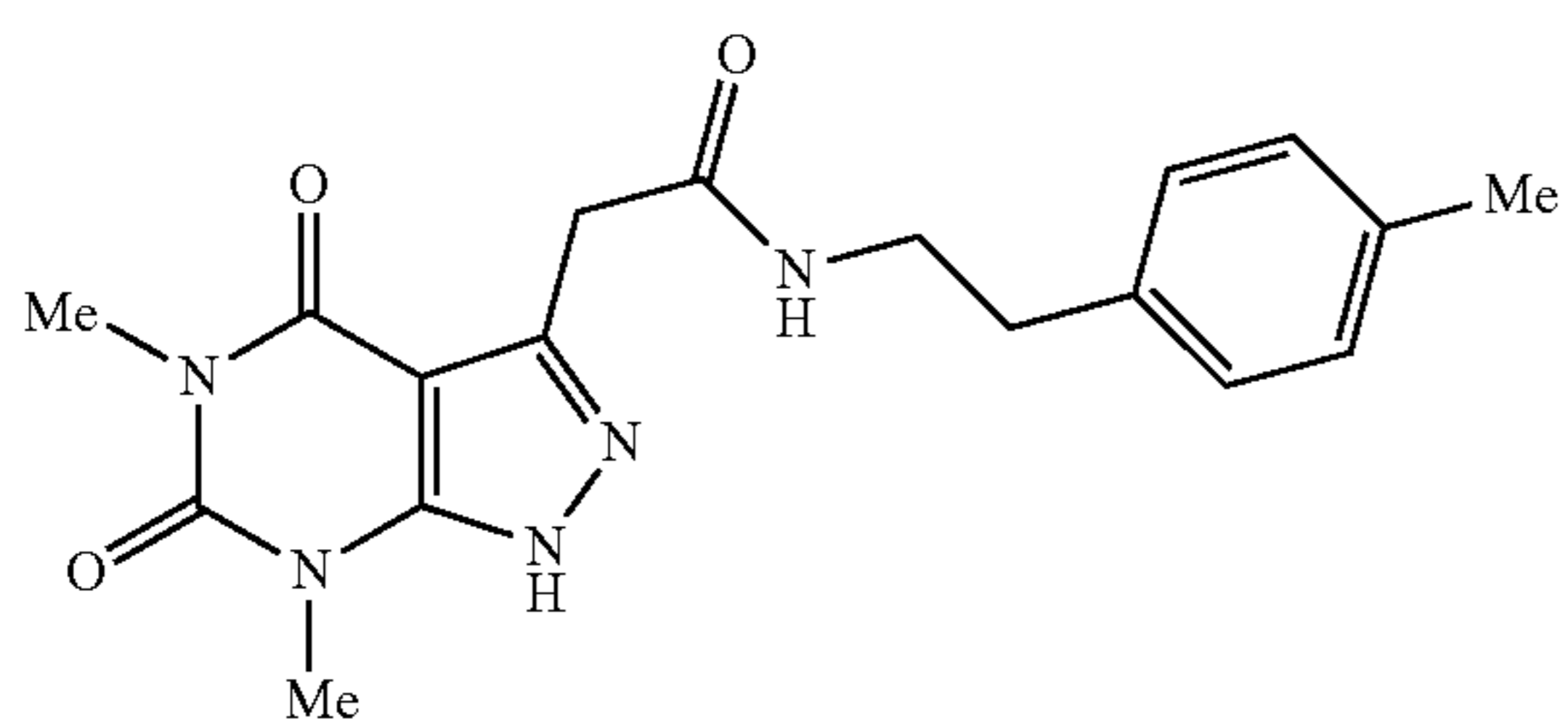
2-(5,7-dimethyl-4,6-dioxo-4,5,6,7-tetrahydro-1H-pyrazolo[3,4-d]pyrimidin-3-yl)-N-(4-methylphenethyl)acetamide
