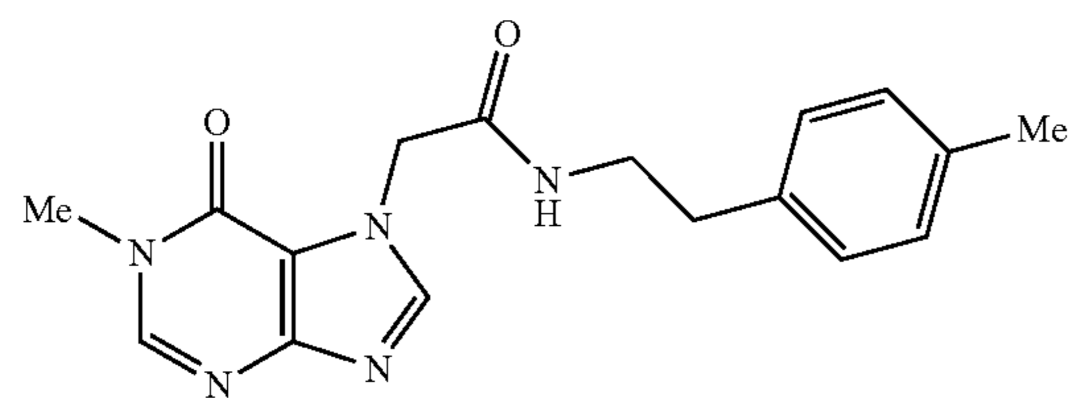
2-(1-methyl-6-oxo-1H-purin-7(6H)-yl)-N-(4-methylphenethyl)acetamide
