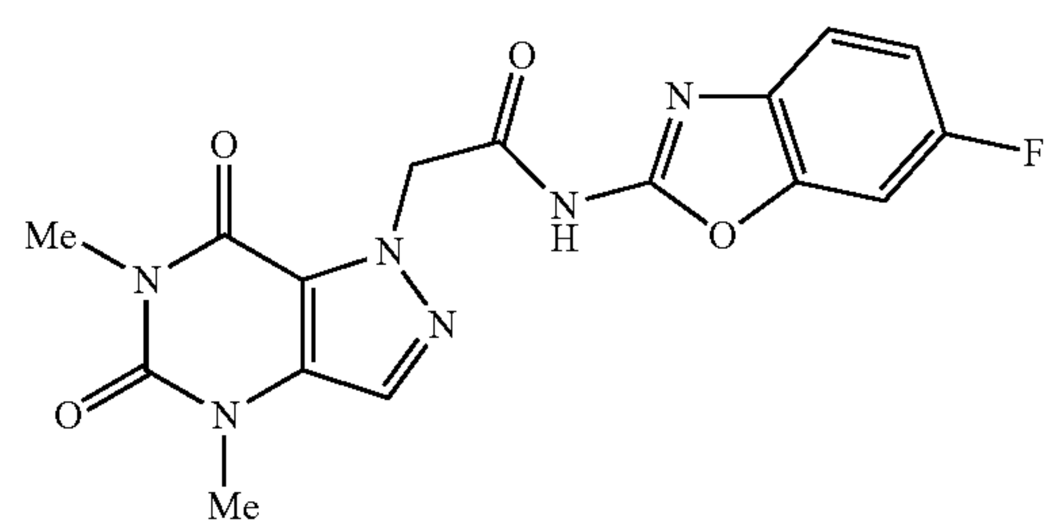
2-(4,6-dimethyl-5,7-dioxo-4,5,6,7-tetrahydro-1H-pyrazolo[4,3-d]pyrimidin-1-yl)-N-(6-fluorobenzo[d]oxazol-2-yl)acetamide
