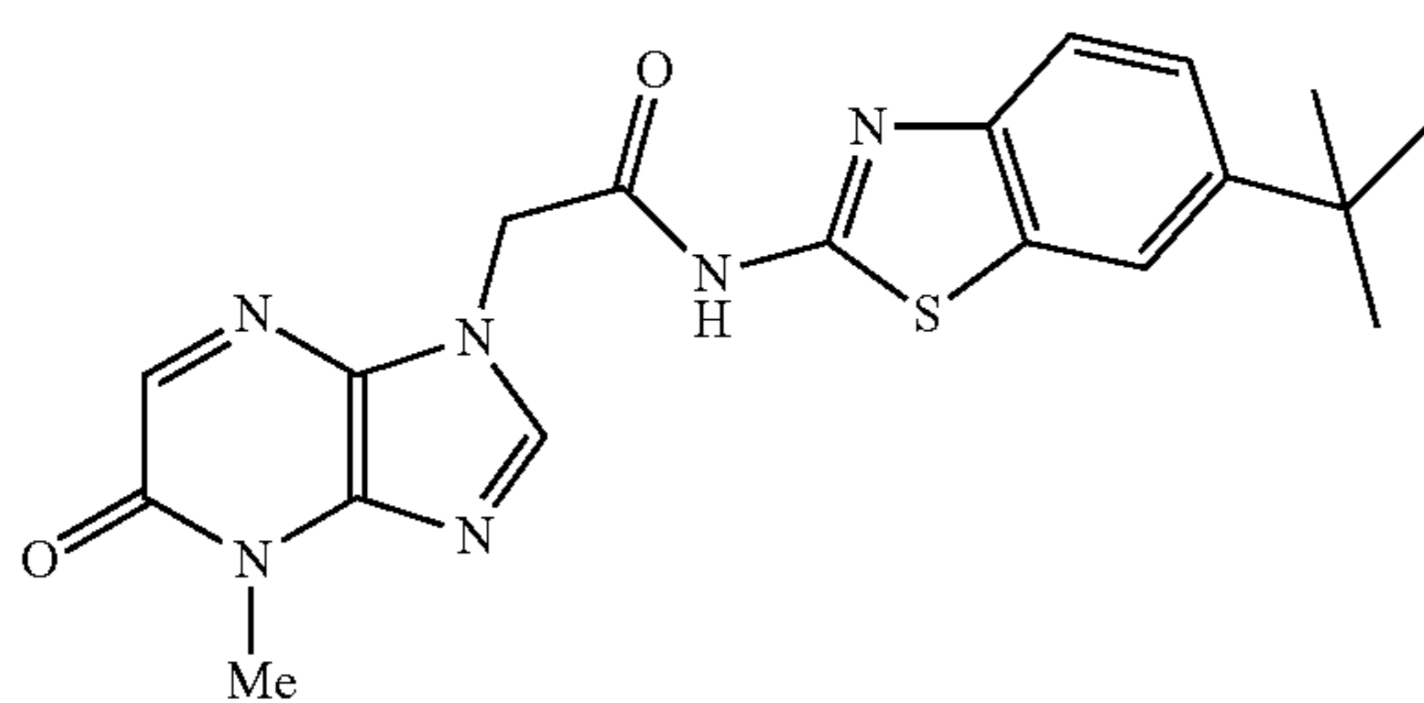
N-(6-tert-butylbenzo[d]thiazol-2-yl)-2-(4-methyl-5-oxo-4,5-dihydro-1H-imidazo[4,5-b]pyrazin-1-yl)acetamide
