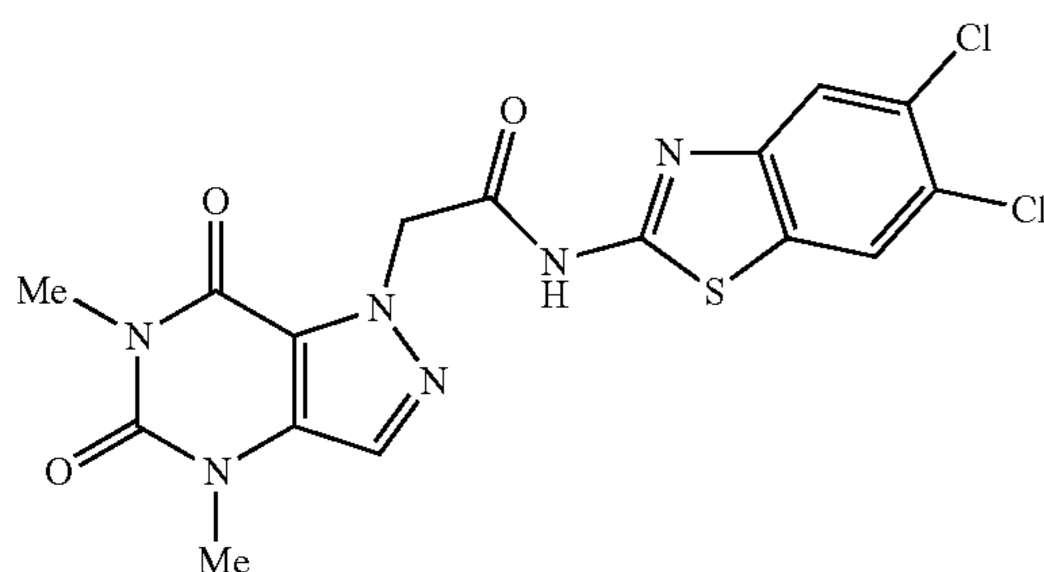
N-(5,6-dichlorobenzo[d]thiazol-2-yl)-2-(4,6-dimethyl-5,7-dioxo-4,5,6,7-tetrahydro-1H-pyrazolo[4,3-d]pyrimidin-1-yl)acetamide
