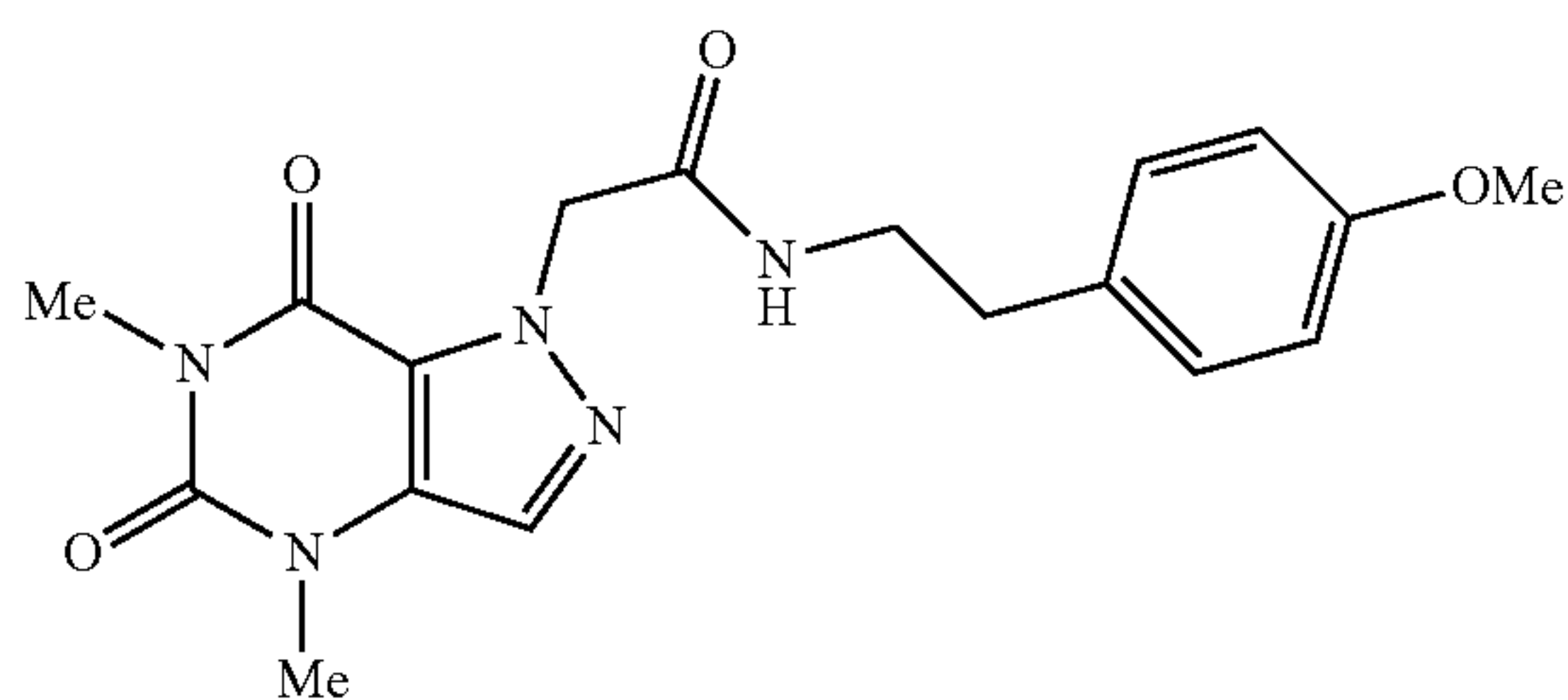
2-(4,6-dimethyl-5,7-dioxo-4,5,6,7-tetrahydro-1H-pyrazolo[4,3-d]pyrimidin-1-yl)-N-(4-methoxyphenethyl)acetamide
