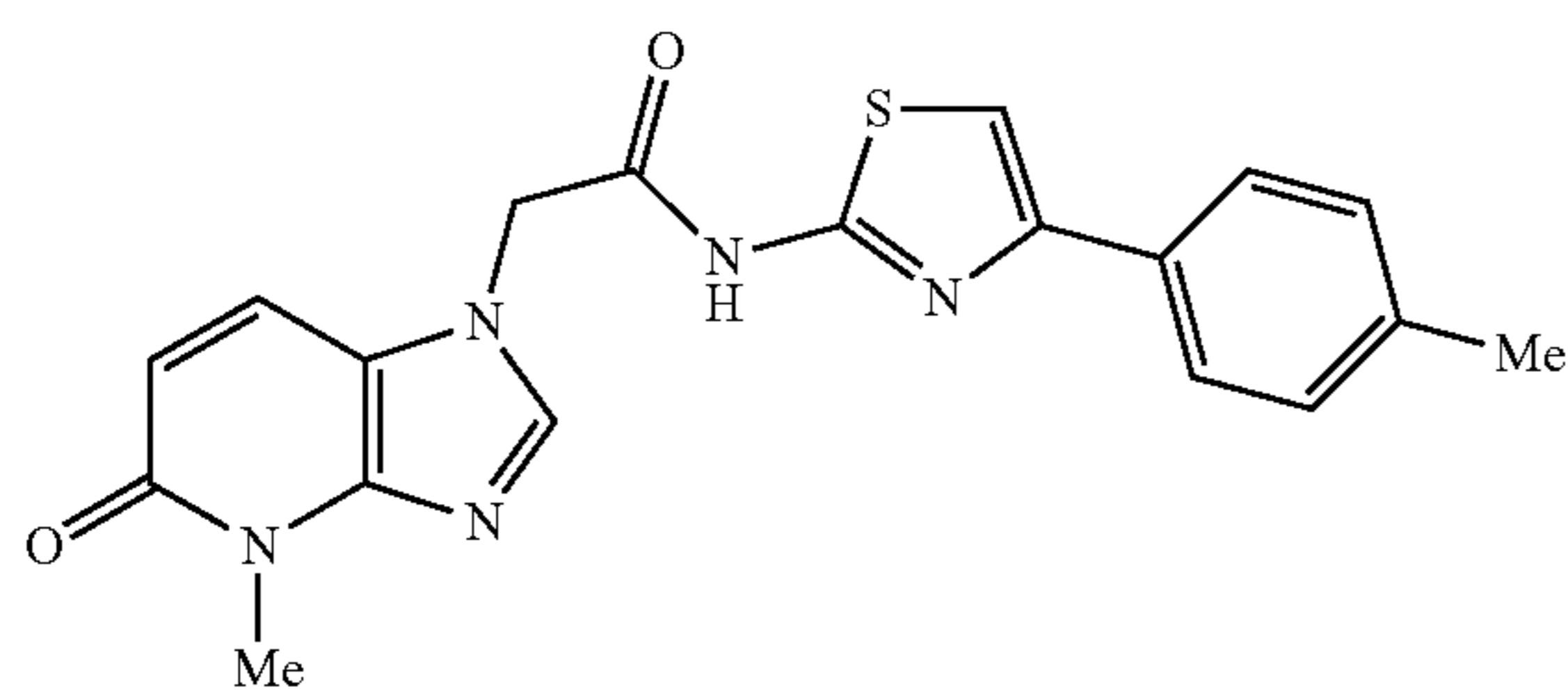
2-(4-methyl-5-oxo-4,5-dihydro-1H-imidazo[4,5-b]pyridin-1-yl)-N-(4-p-tolylthiazol-2-yl)acetamide
