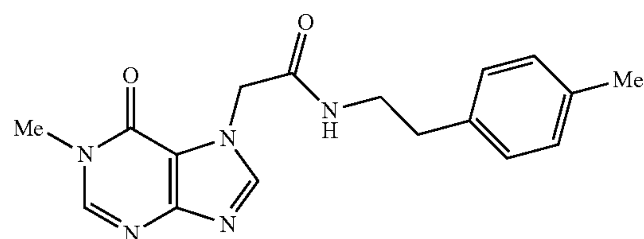
2-(1-methyl-6-oxo-1H-purin-7(6H)-yl)-N-(4-methylphenethyl)acetamide
