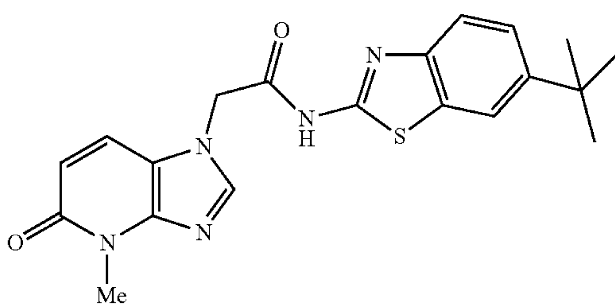
N-(6-tert-butylbenzo[d]thiazol-2-yl)-2-(4-methyl-5-oxo-4,5-dihydro-1H-imidazo[4,5-b]pyridin-1-yl)acetamide
