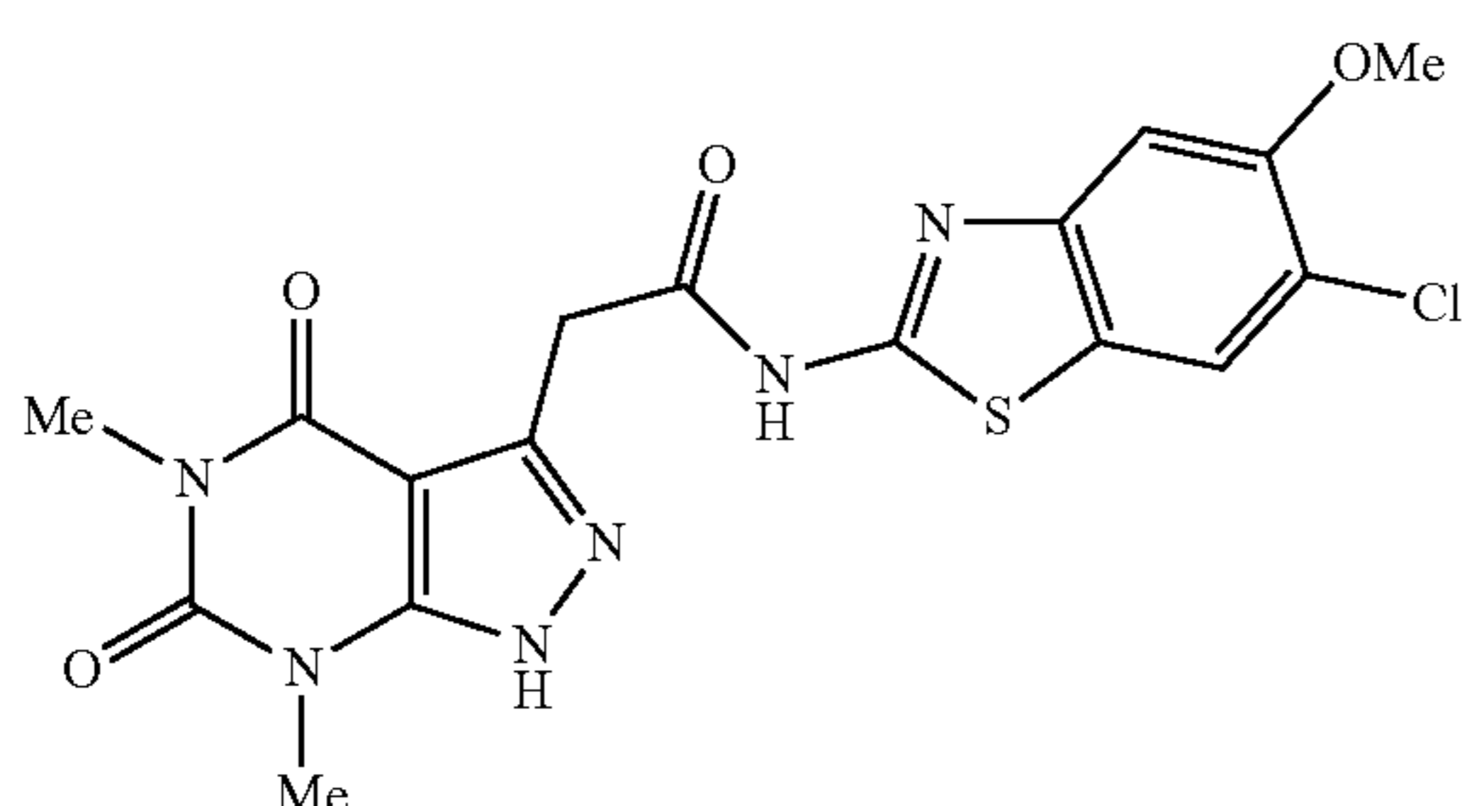
N-(6-chloro-5-methoxybenzo[d]thiazol-2-yl)-2-(5,7-dimethyl-4,6-dioxo-4,5,6,7-tetrahydro-1H-pyrazolo[3,4-d]pyrimidin-3-yl)acetamide
