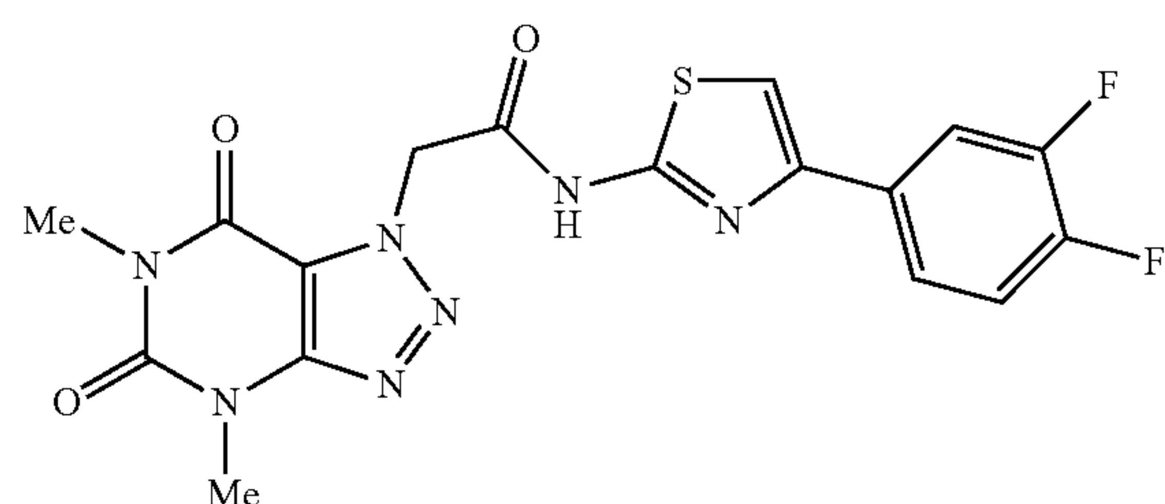
N-(4-(3,4-difluorophenyl)thiazol-2-yl)-2-(4,6-dimethyl-5,7-dioxo-4,5,6,7-tetrahydro-1H-[1,2,3]triazolo[4,5-d]pyrimidin-1-yl)acetamide
