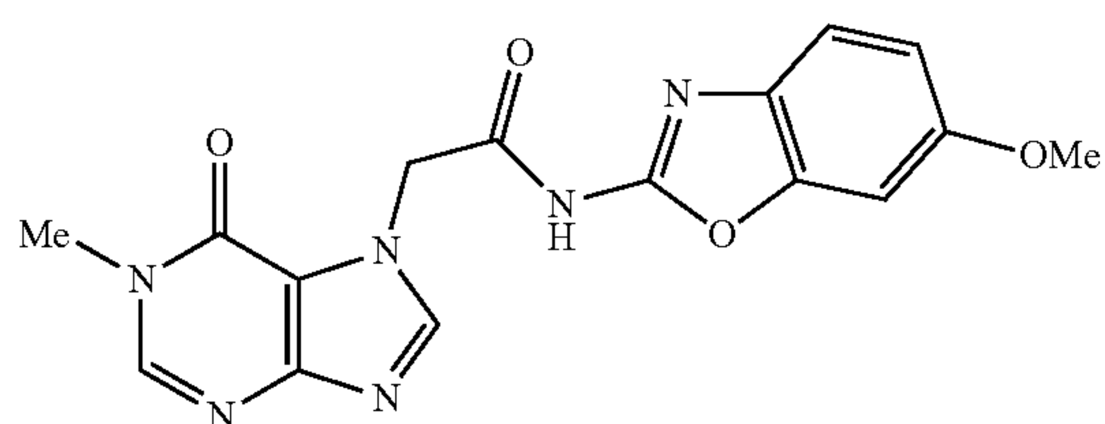
N-(6-methoxybenzo[d]oxazol-2-yl)-2-(1-methyl-6-oxo-1H-purin-7(6H)-yl)acetamide
