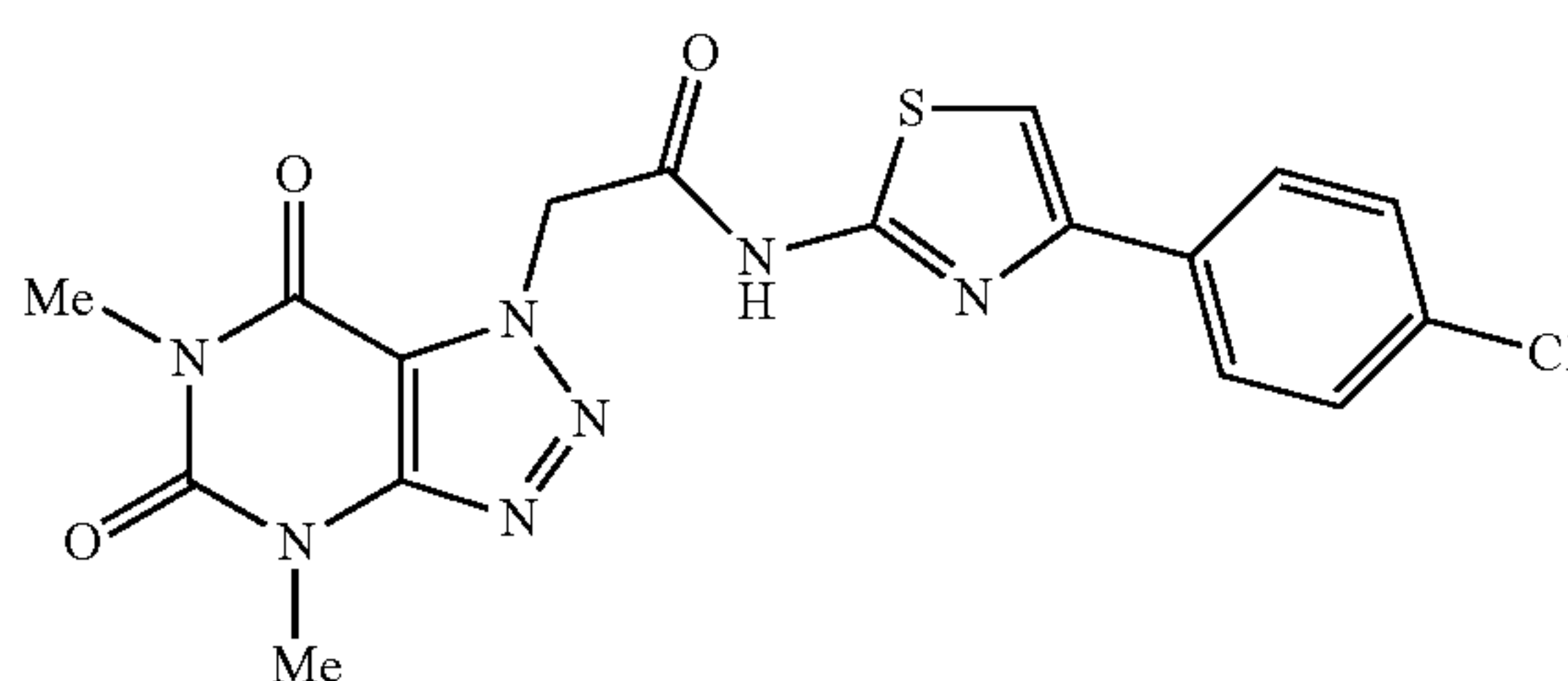
N-(4-(4-chlorophenyl)thiazol-2-yl)-2-(4,6-dimethyl-5,7-dioxo-4,5,6,7-tetrahydro-1H-[1,2,3]triazolo[4,5-d]pyrimidin-1-yl)acetamide
