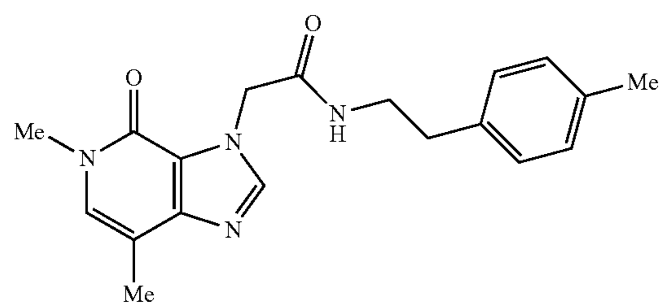
2-(5,7-dimethyl-4-oxo-4,5-dihydro-3H-imidazo[4,5-c]pyridin-3-yl)-N-(4-methylphenethyl)acetamide
