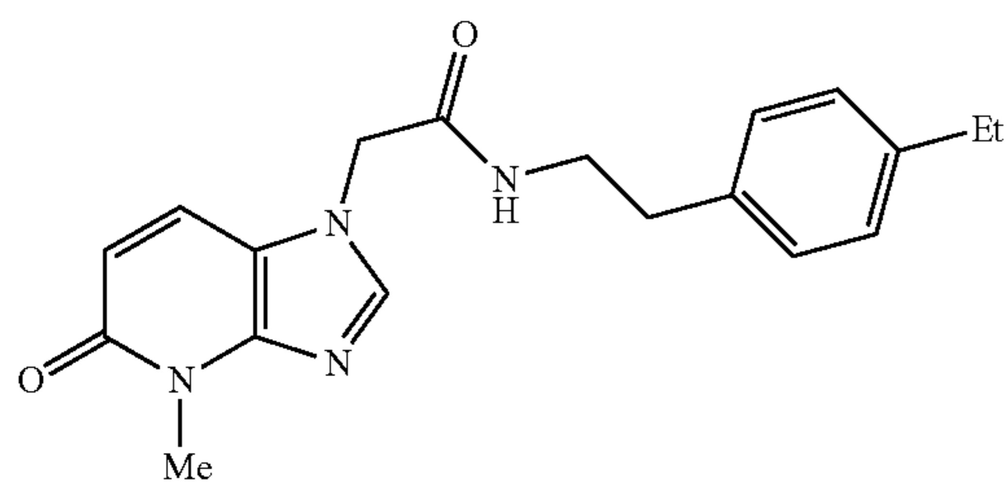
N-(4-ethylphenethyl)-2-(4-methyl-5-oxo-4,5-dihydro-1H-imidazo[4,5-b]pyridin-1-yl)acetamide
