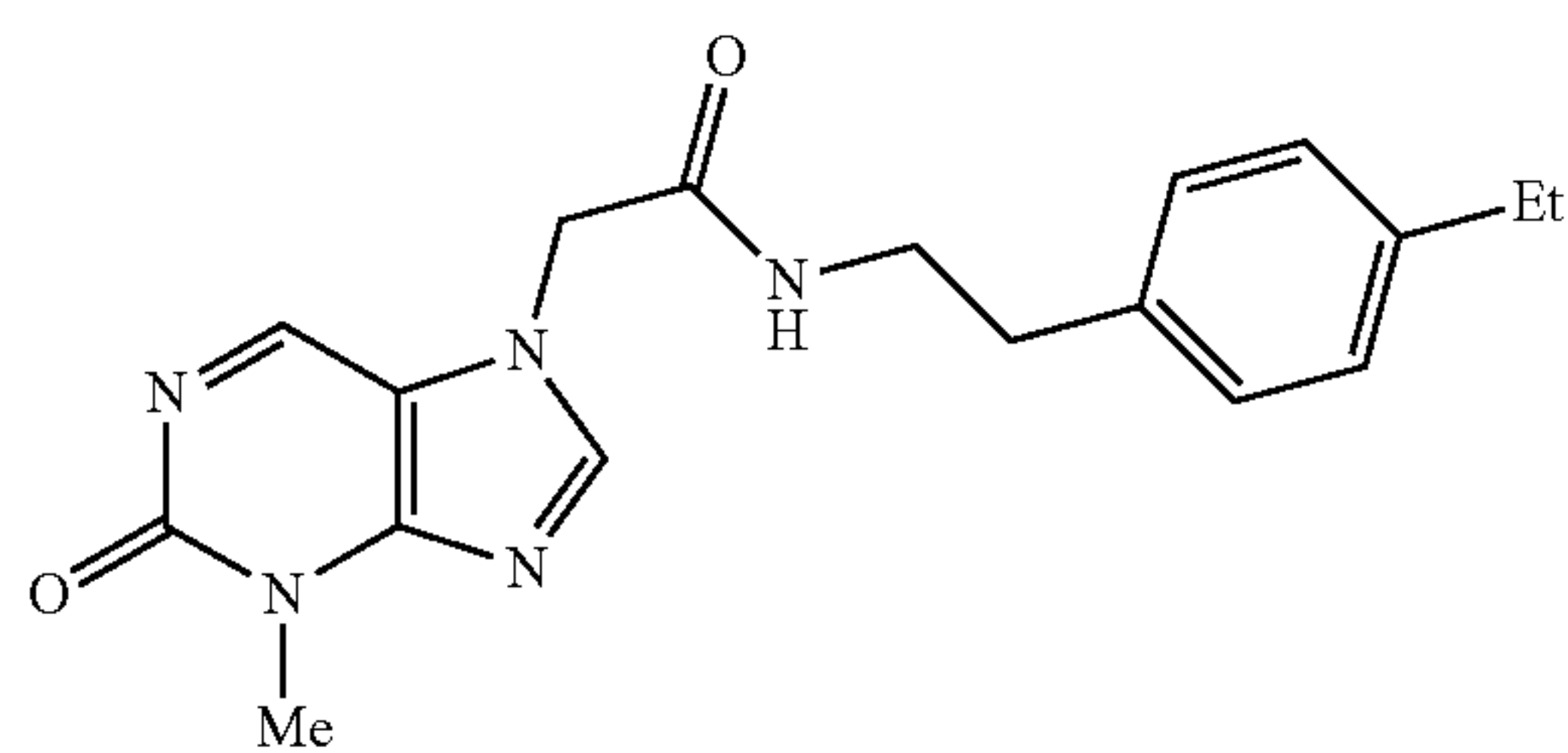
N-(4-ethylphenethyl)-2-(3-methyl-2-oxo-2,3-dihydropurin-7-yl)acetamide
