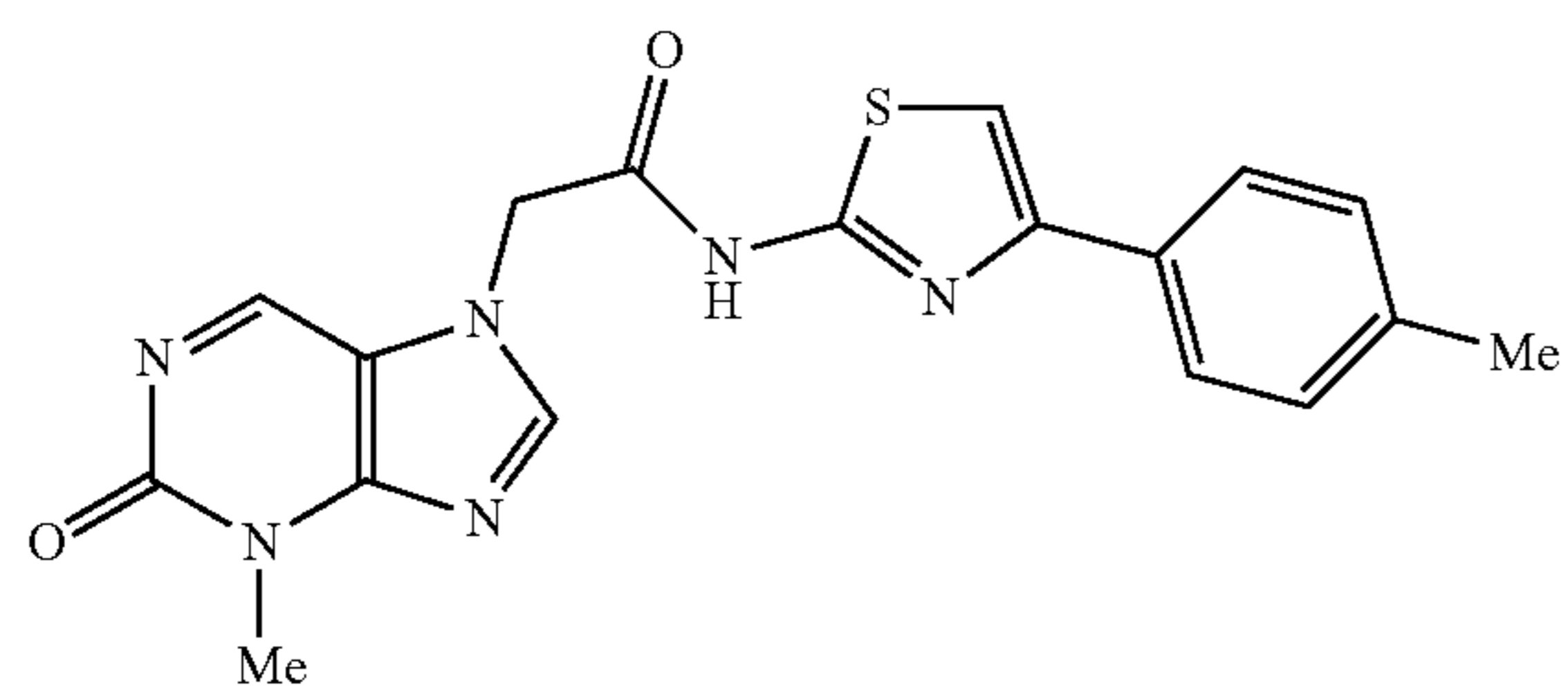
2-(3-methyl-2-oxo-2,3-dihydropurin-7-yl)-N-(4-p-tolylthiazol-2-yl)acetamide
