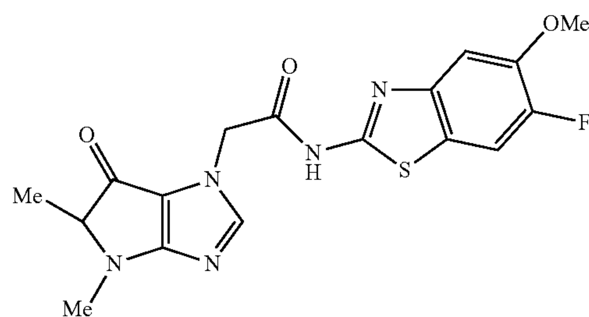
2-(4,5-dimethyl-6-oxo-5,6-dihydropyrrolo[3,2-d]imidazol-1(4H)-yl)-N-(6-fluoro-5-methoxybenzo[d]thiazol-2-yl)acetamide
