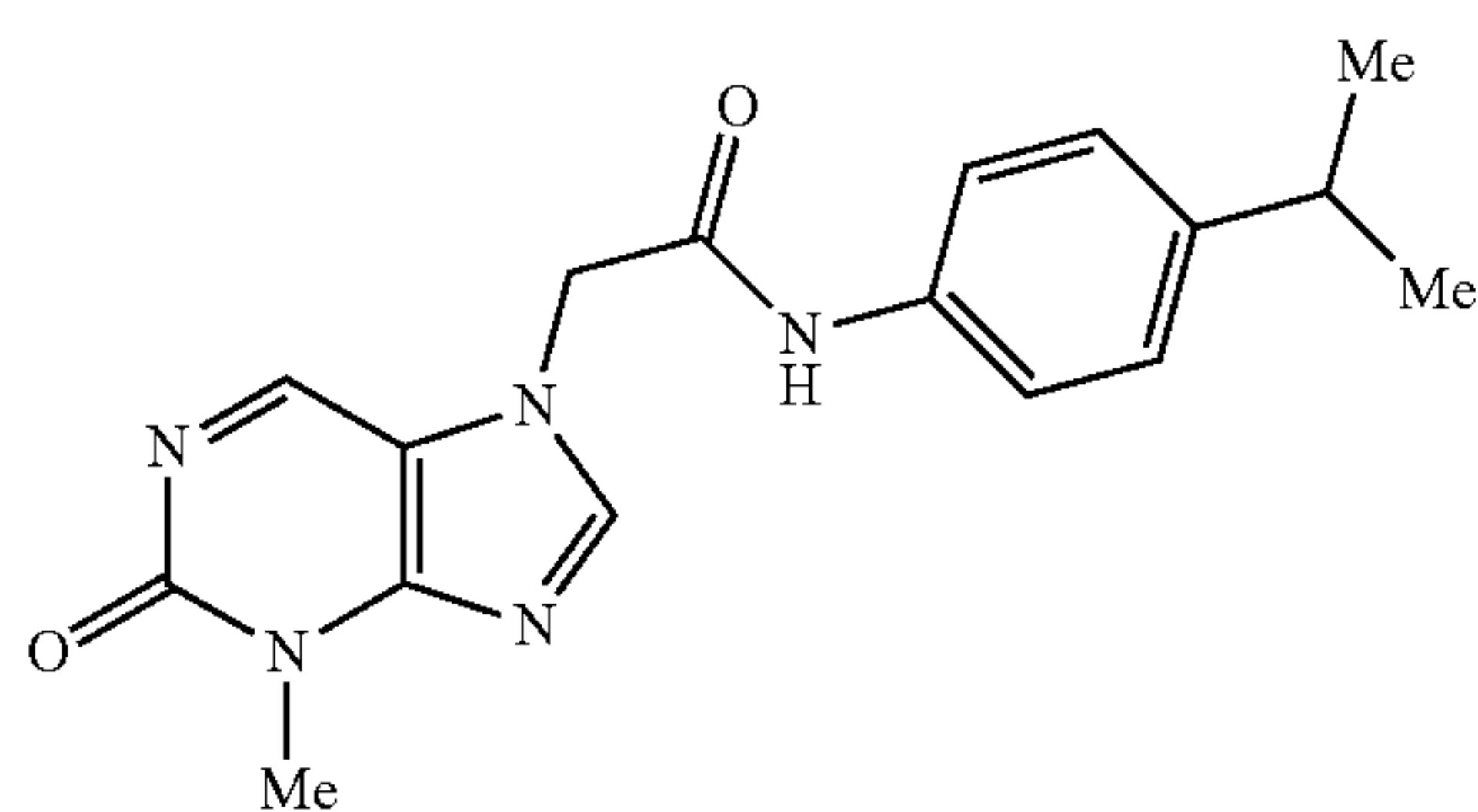
N-(4-isopropylphenyl)-2-(3-methyl-2-oxo-2,3-dihydropurin-7-yl)acetamide
