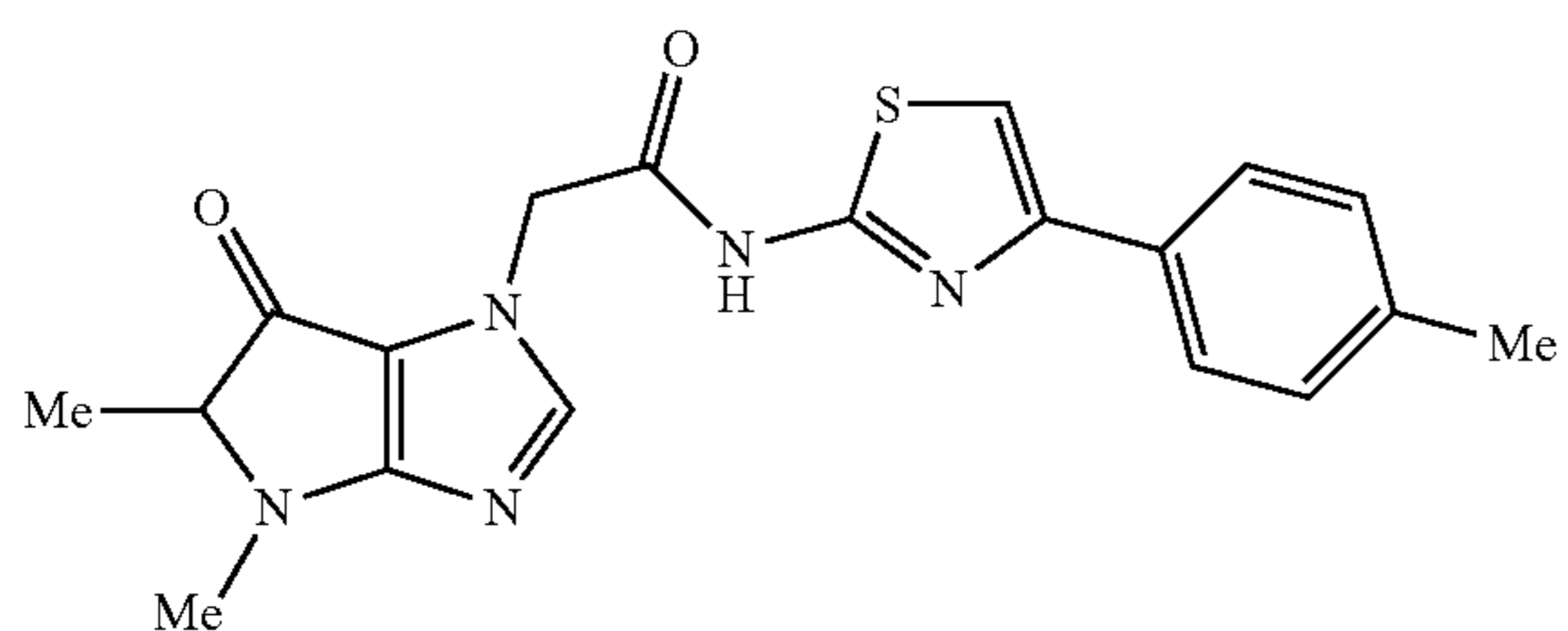
2-(4,5-dimethyl-6-oxo-5,6-dihydropyrrolo[3,2-d]imidazol-1(4H)-yl)-N-(4-p-tolylthiazol-2-yl)acetamide
