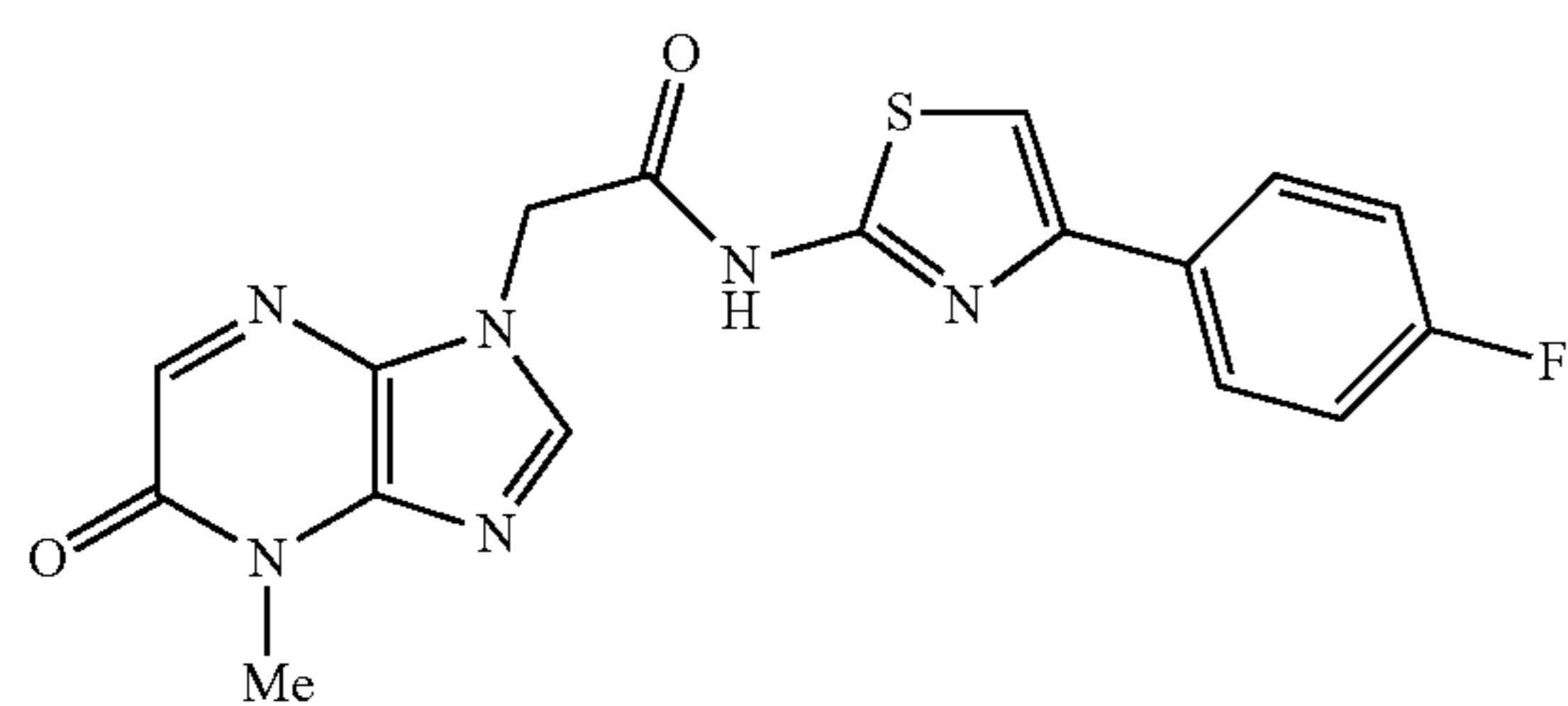
N-(4-(4-fluorophenyl)thiazol-2-yl)-2-(4-methyl-5-oxo-4,5-dihydroimidazo[4,5-b]pyrazin-1-yl)acetamide
