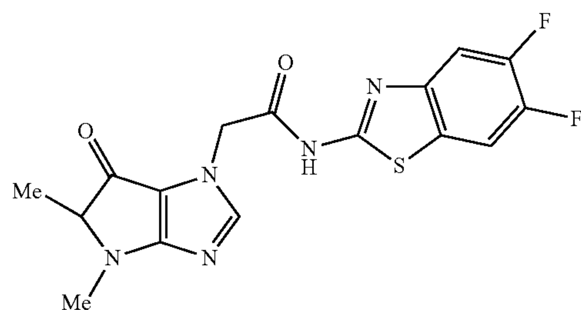
N-(5,6-difluorobenzo[d]thiazol-2-yl)-2-(4,5-dimethyl-6-oxo-5,6-dihydropyrrolo[3,2-d]imidazol-1(4H)-yl)acetamide
