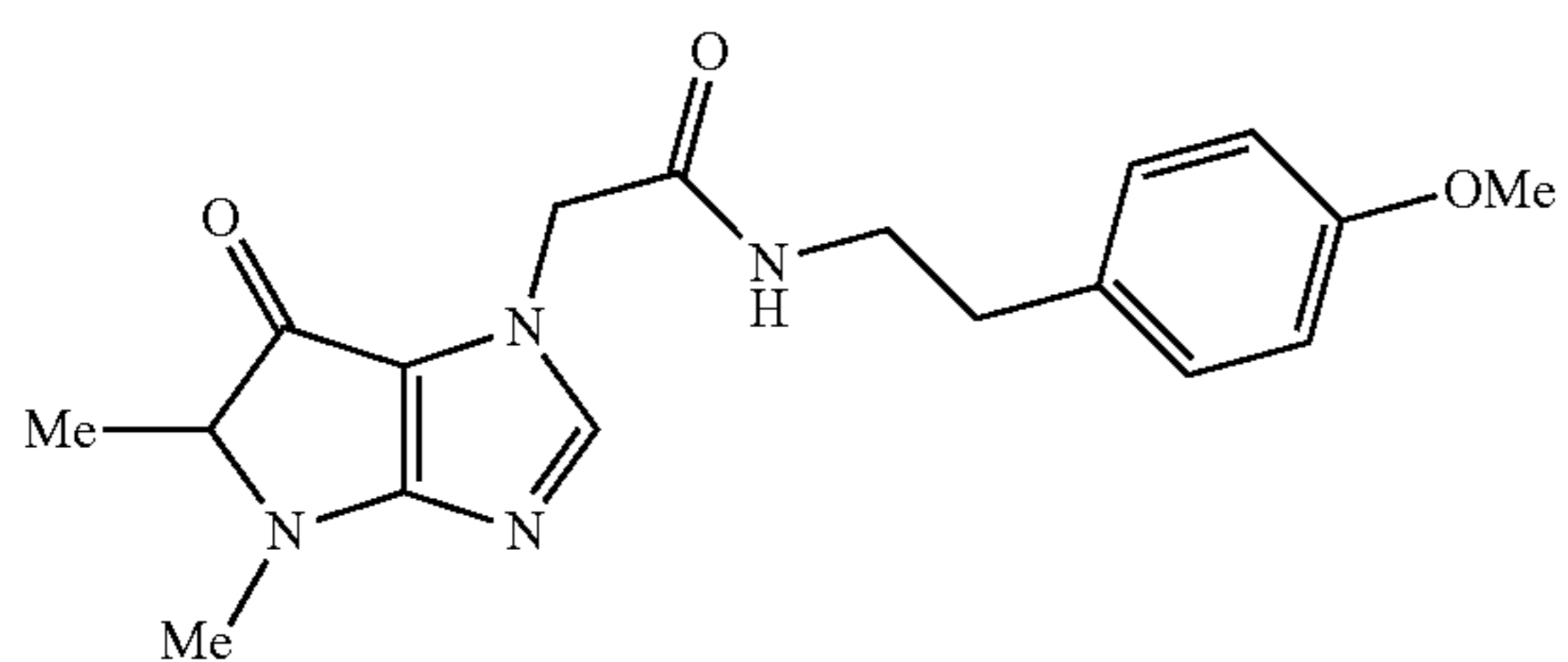
2-(4,5-dimethyl-6-oxo-5,6-dihydropyrrolo[3,2-d]imidazol-1(4H)-yl)-N-(4-methoxyphenethyl)acetamide
