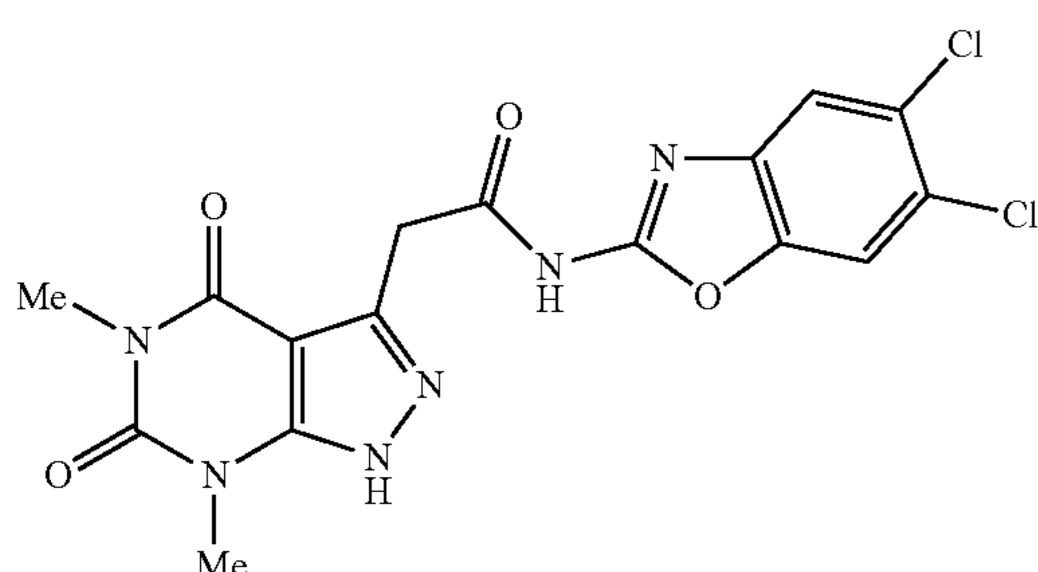
N-(5,6-dichlorobenzo[d]oxazol-2-yl)-2-(5,7-dimethyl-4,6-dioxo-4,5,6,7-tetrahydro-1H-pyrazolo[3,4-d]pyrimidin-3-yl)acetamide
