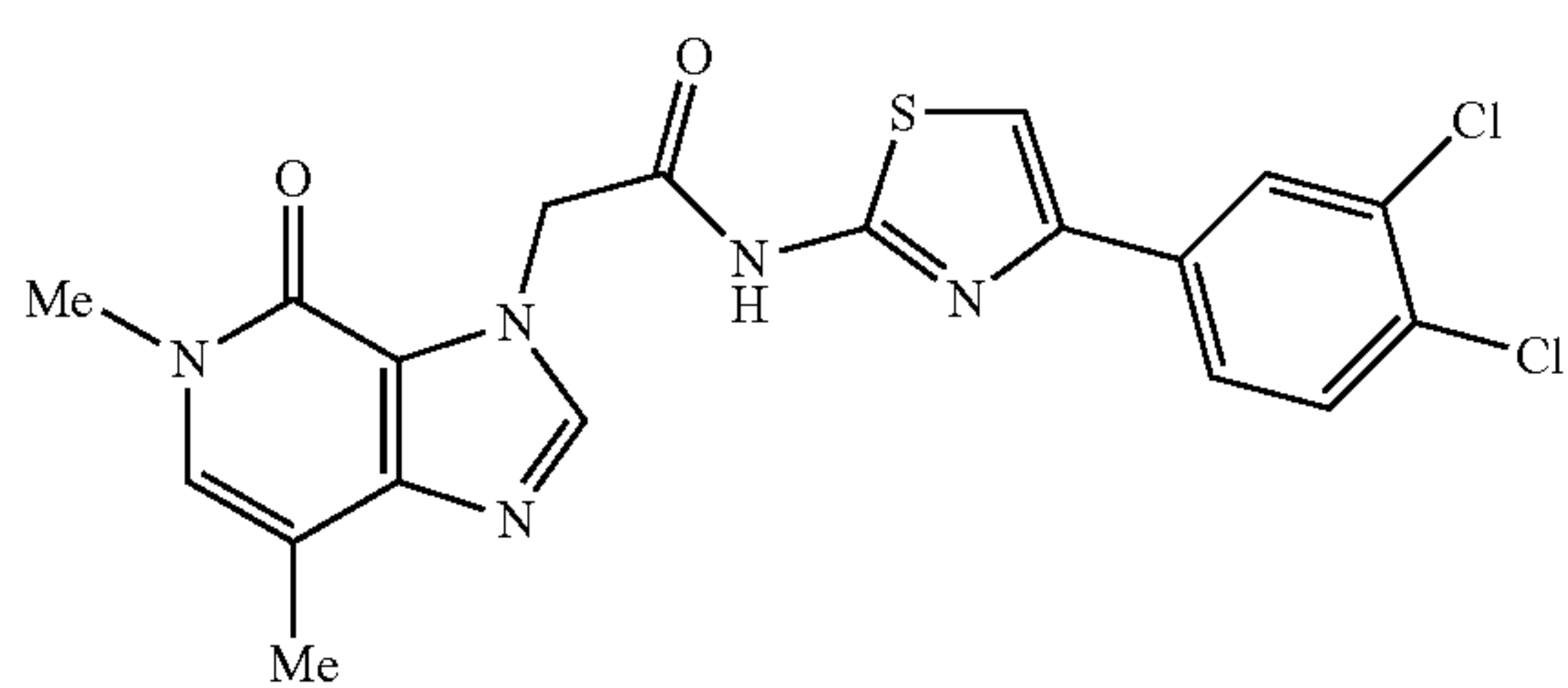
N-(4-(3,4-dichlorophenyl)thiazol-2-yl)-2-(5,7-dimethyl-4-oxo-4,5-dihydro-3H-imidazo[4,5-c]pyridin-3-yl)acetamide
