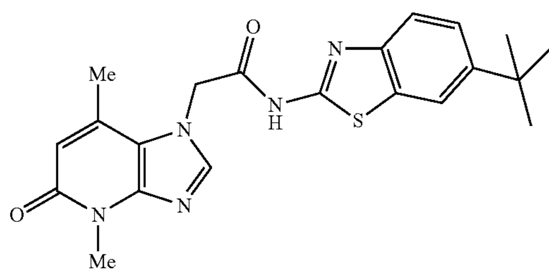
N-(6-tert-butylbenzo[d]thiazol-2-yl)-2-(4,7-dimethyl-5-oxo-4,5-dihydro-1H-imidazo[4,5-b]pyridin-1-yl)acetamide
