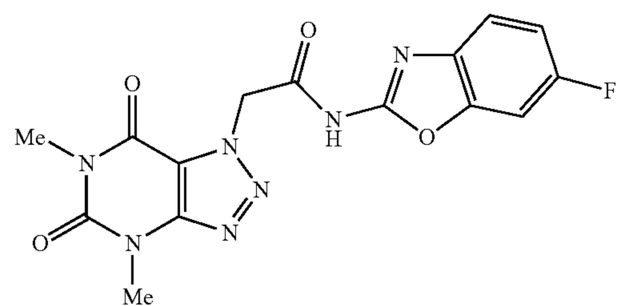
2-(4,6-dimethyl-5,7-dioxo-4,5,6,7-tetrahydro-1H-[1,2,3]triazolo[4,5-d]pyrimidin-1-yl)-N-(6-fluorobenzo[d]oxazol-2-yl)acetamide
