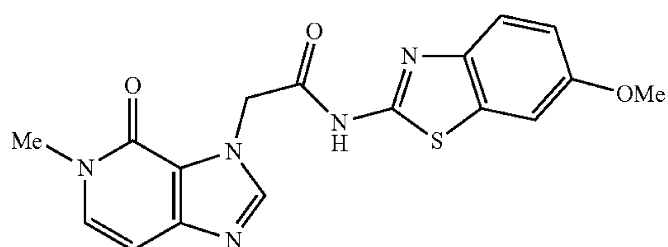
N-(6-methoxybenzo[d]thiazol-2-yl)-2-(5-methyl-4-oxo-4,5-dihydro-3H-imidazol[4,5-c]pyridin-3-yl)acetamide
