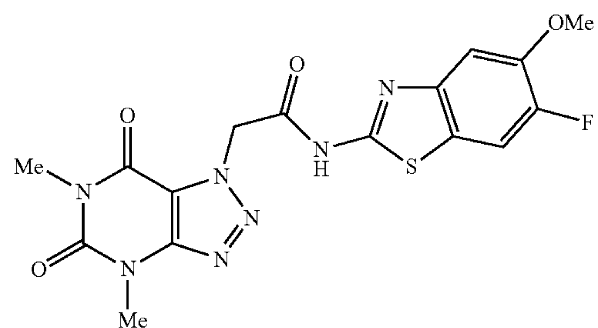
2-(4,6-dimethyl-5,7-dioxo-4,5,6,7-tetrahydro-1H-[1,2,3]triazolo[4,5-d]pyrimidin-1-yl)-N-(6-fluoro-5-methoxybenzo[d]thiazol-2-yl)acetamide
