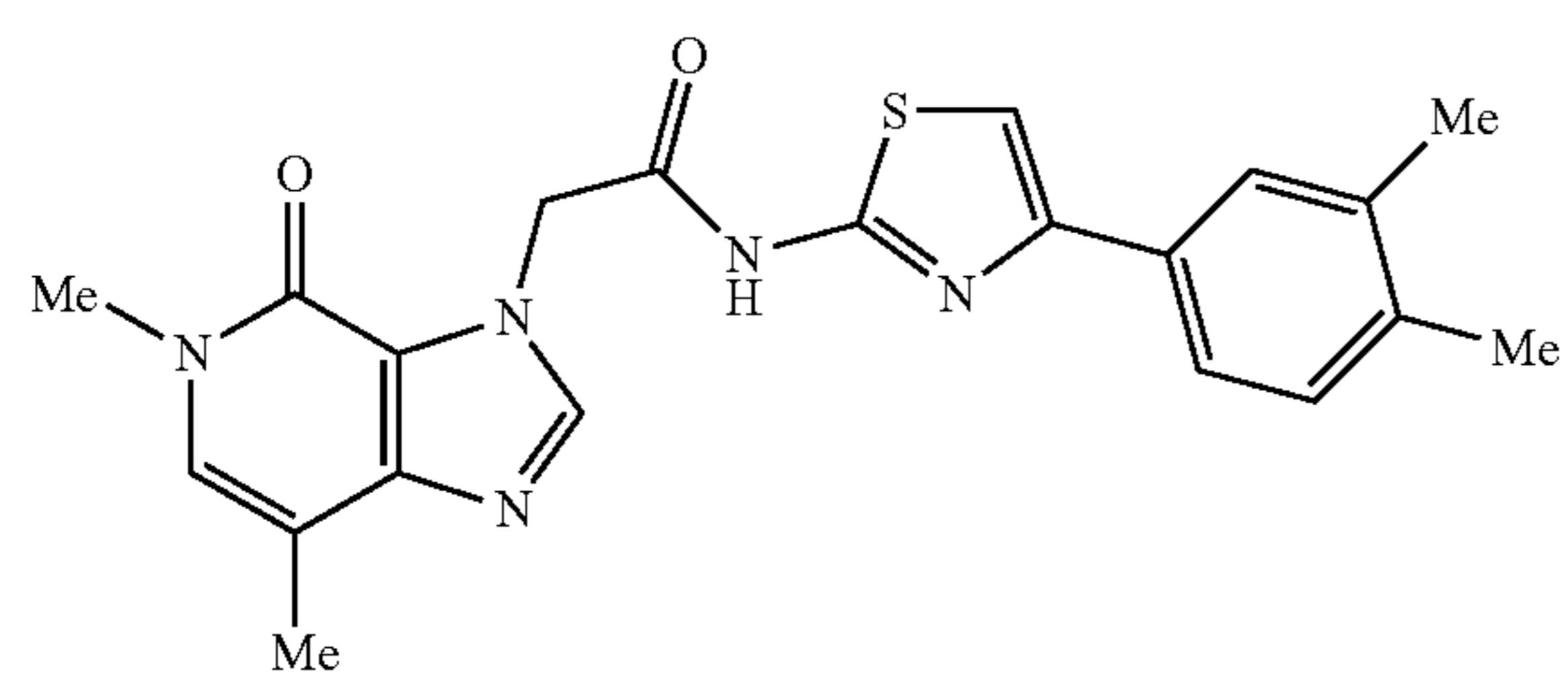
2-(5,7-dimethyl-4-oxo-4,5-dihydro-3H-imidazo[4,5-c]pyridin-3-yl)-N-(4-(3,4-dimethylphenyl)thiazol-2-yl)acetamide
