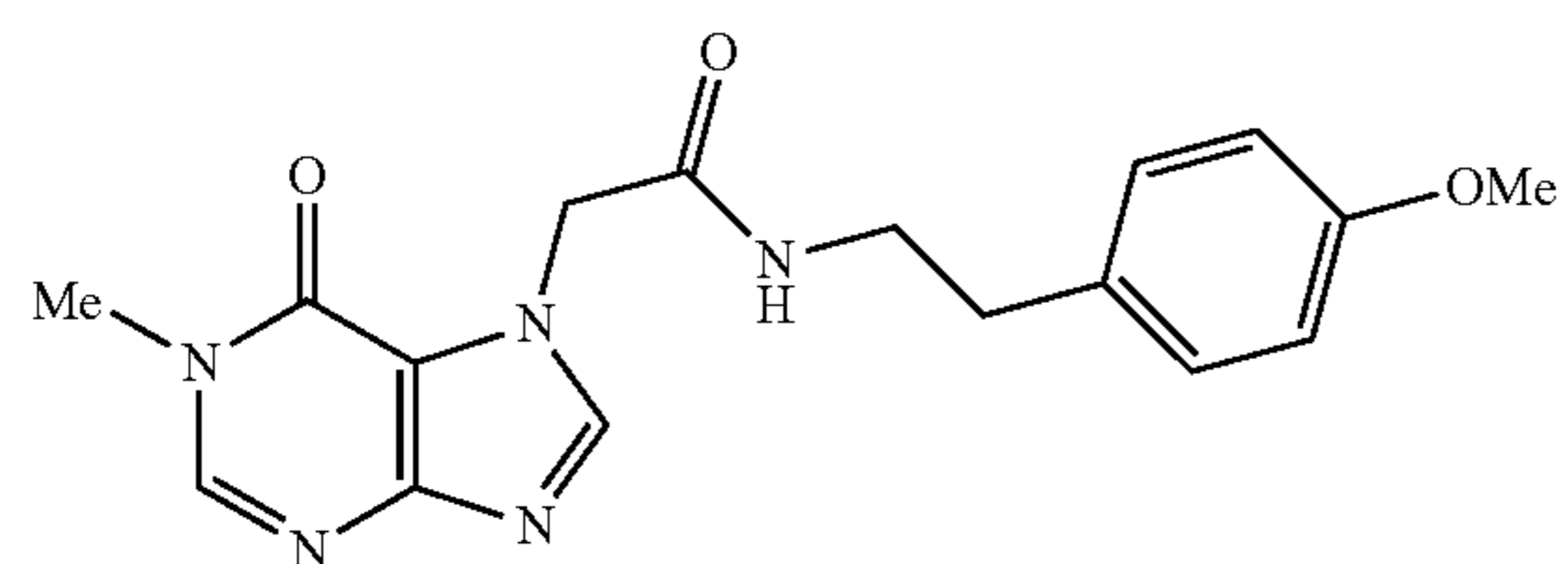
N-(4-methoxyphenethyl)-2-(1-methyl-6-oxo-1H-purin-7(6H)-yl)acetamide
