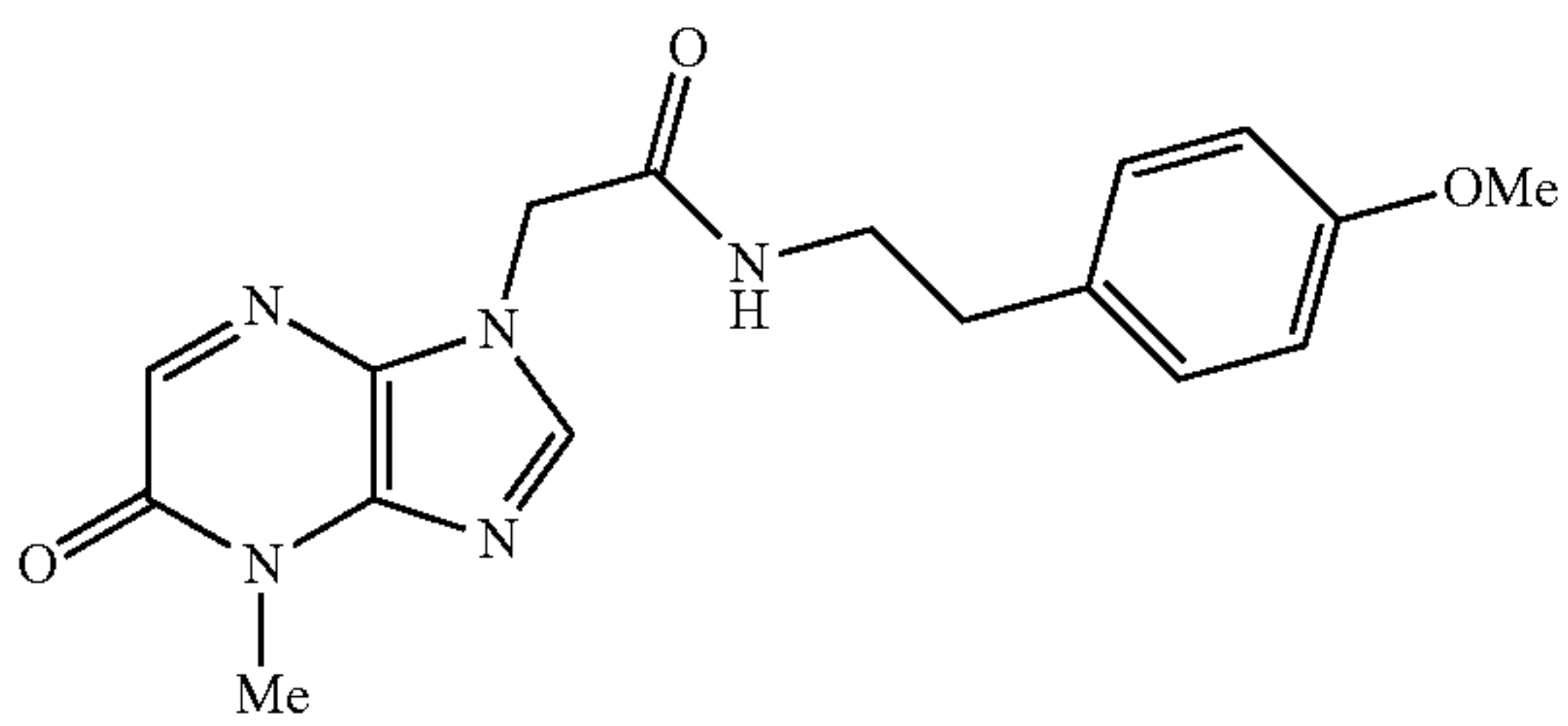
N-(4-methoxyphenethyl)-2-(4-methyl-5-oxo-4,5-dihydro-1H-imidazo[4,5-b]pyrazin-1-yl)acetamide
