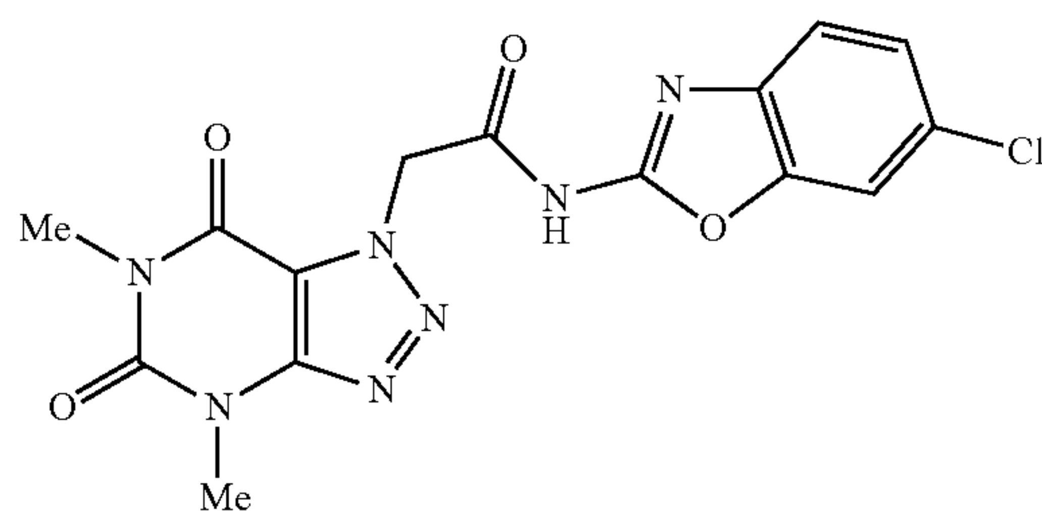
N-(6-chlorobenzo[d]oxazol-2-yl)-2-(4,6-dimethyl-5,7-dioxo-4,5,6,7-tetrahydro-1H-[1,2,3]triazolo[4,5-d]pyrimidin-1-yl)acetamide
