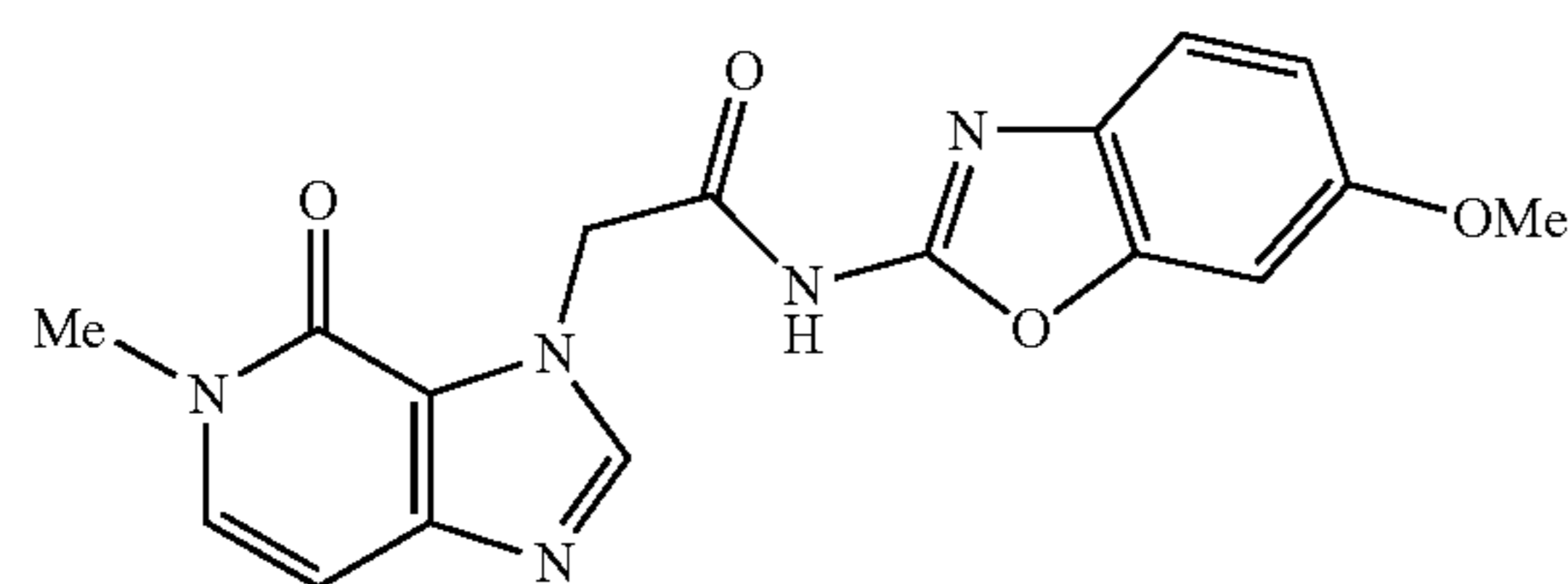
N-(6-methoxybenzo[d]oxazol-2-yl)-2-(5-methyl-4-oxo-4,5-dihydro-3H-imidazo[4,5-c]pyridin-3-yl)acetamide
