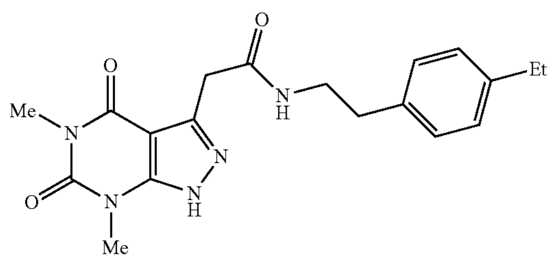
2-(5,7-dimethyl-4,6-dioxo-4,5,6,7-tetrahydro-1H-pyrazolo[3,4-d]pyrimidin-3-yl)-N-(4-ethylphenethyl)acetamide
