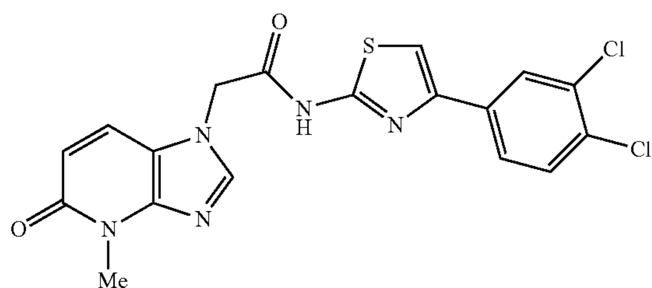
N-(4-(3,4-dichlorophenyl)thiazol-2-yl)-2-(4-methyl-5-oxo-4,5-dihydro-1H-imidazo[4,5-b]pyridin-1-yl)acetamide
