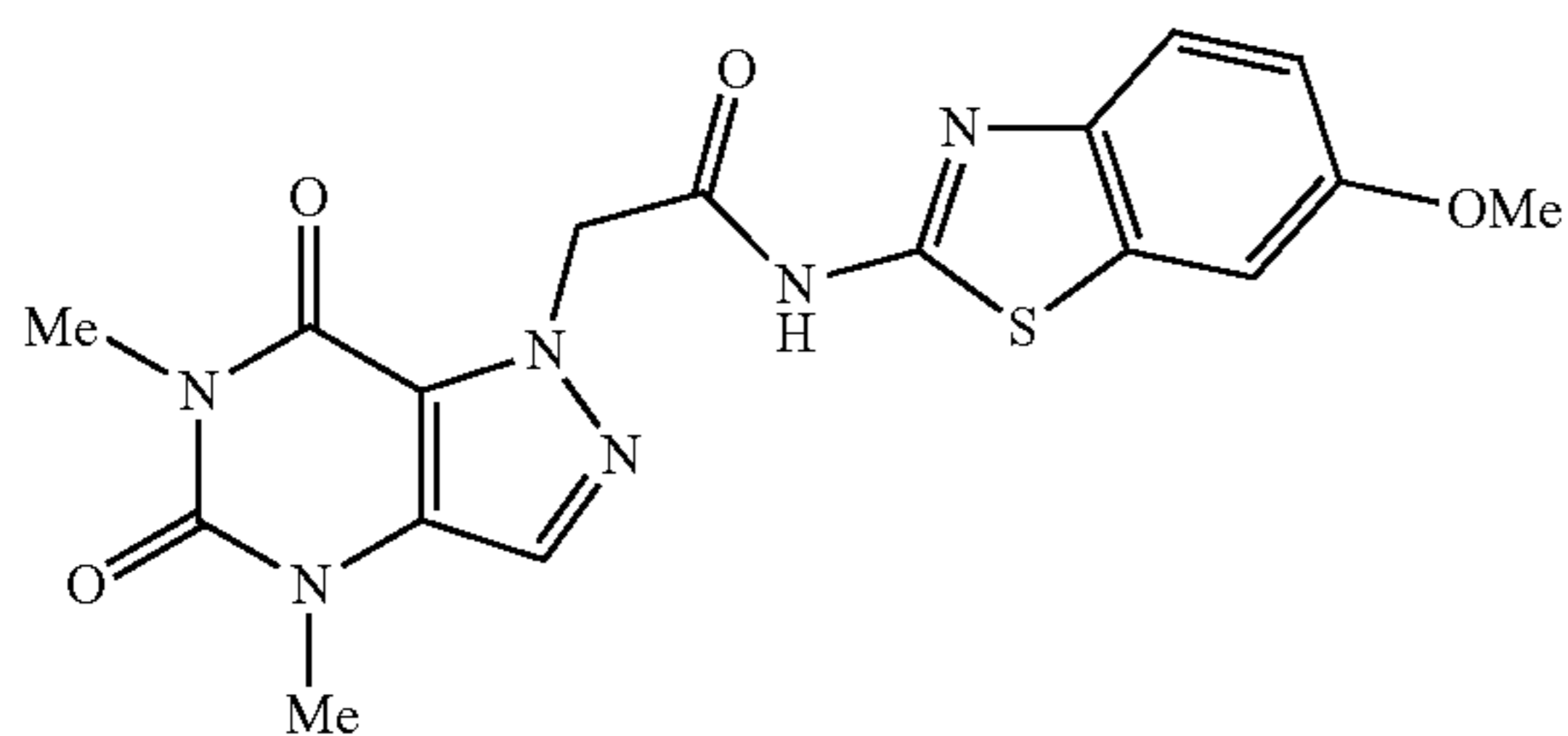
2-(4,6-dimethyl-5,7-dioxo-4,5,6,7-tetrahydro-1H-pyrazolo[4,3-d]pyrimidin-1-yl)-N-(6-methoxybenzo[d]thiazol-2-yl)acetamide
