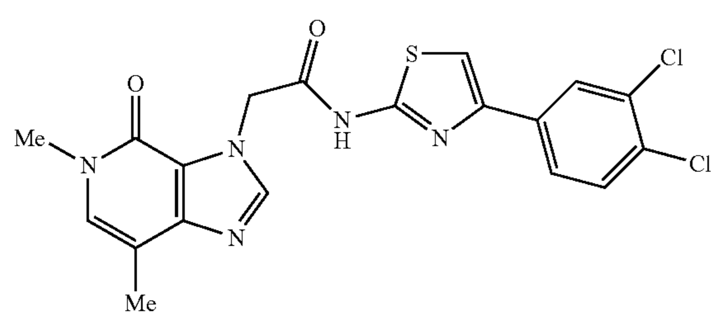
N-(4-(3,4-dichlorophenyl)thiazol-2-yl)-2-(5,7-dimethyl-4-oxo-4,5-dihydro-3H-imidazo[4,5-c]pyridin-3-yl)acetamide
