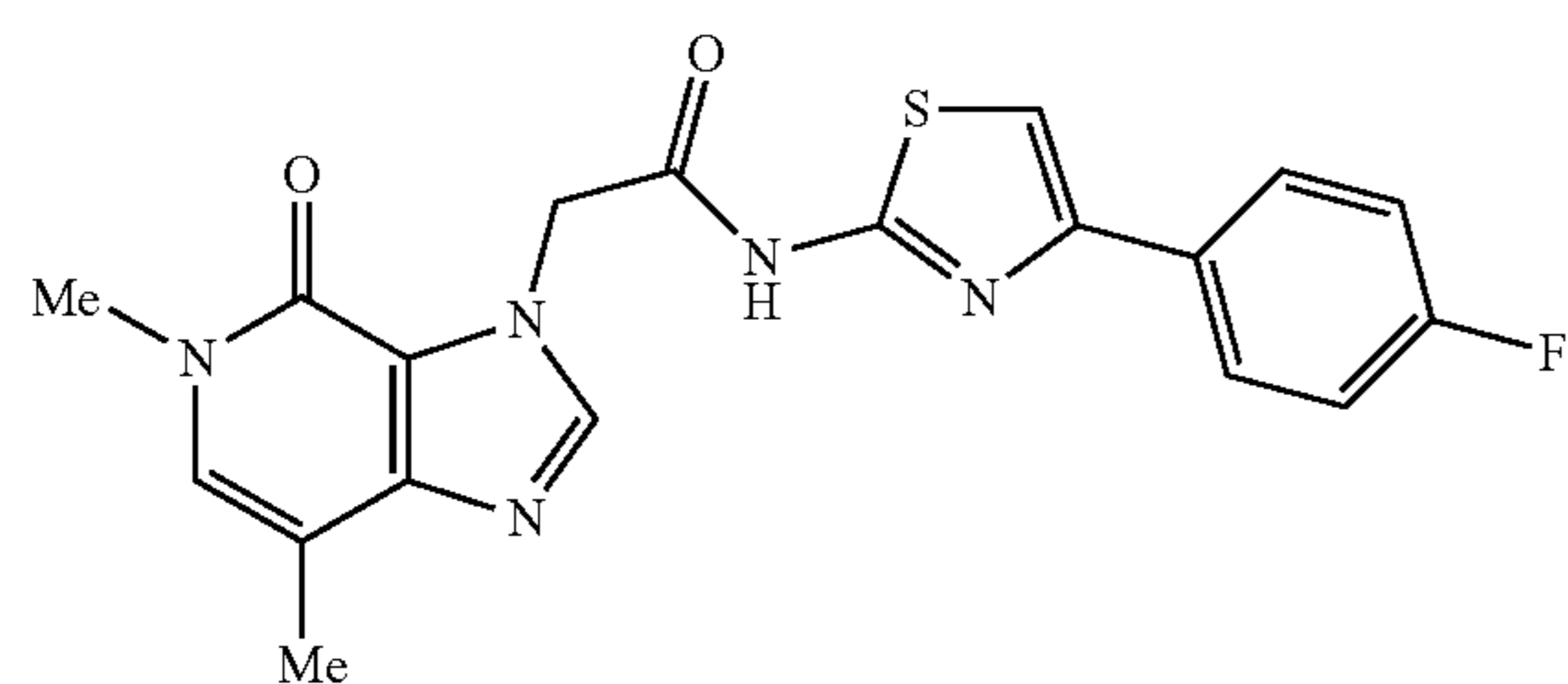
2-(5,7-dimethyl-4-oxo-4,5-dihydro-3H-imidazo[4,5-c]pyridin-3-yl)-N-(4-(4-fluorophenyl)thiazol-2-yl)acetamide
