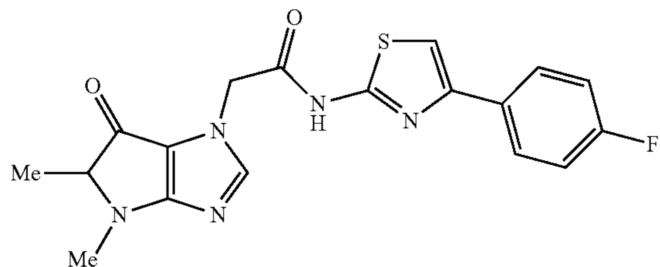
2-(4,5-dimethyl-6-oxo-5,6-dihydropyrrolo[3,2-d]imidazol-1(4H)-yl)-N-(4-(4-fluorophenyl)thiazol-2-yl)acetamide
