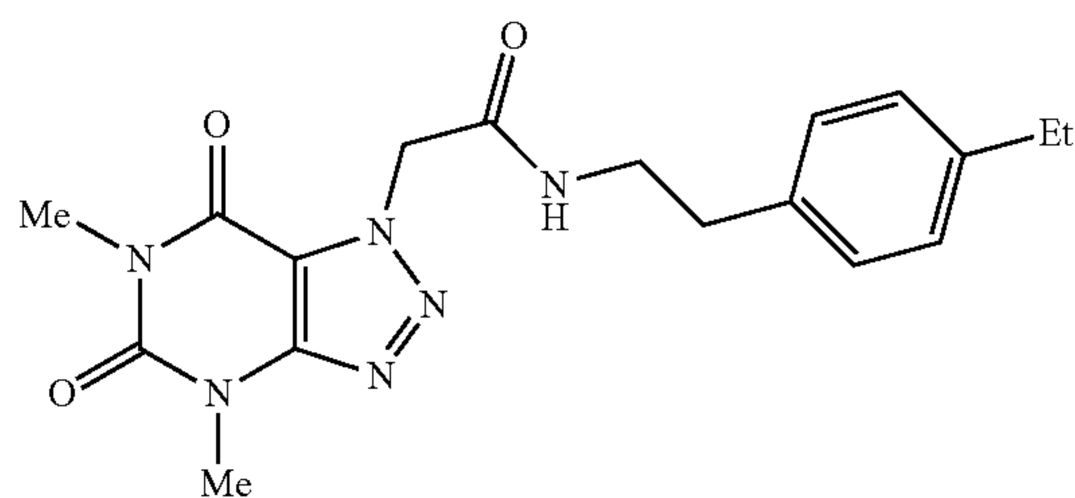
2-(4,6-dimethyl-5,7-dioxo-4,5,6,7-tetrahydro-1H-[1,2,3]triazolo[4,5-d]pyrimidin-1-yl)-N-(4-ethylphenethyl)acetamide
