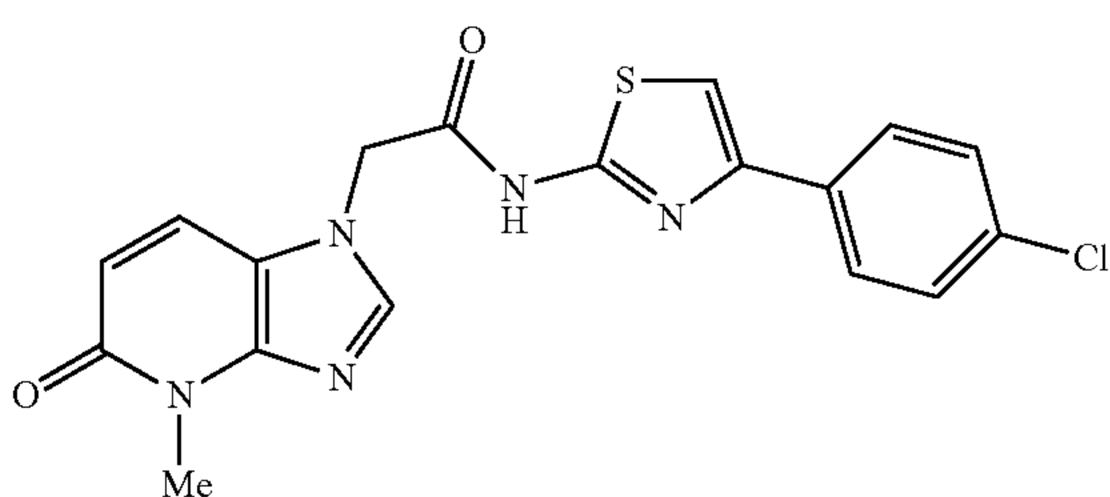
N-(4-(4-chlorophenyl)thiazol-2-yl)-2-(4-methyl-5-oxo-4,5-dihydro-1H-imidazo[4,5-b]pyridin-1-yl)acetamide
