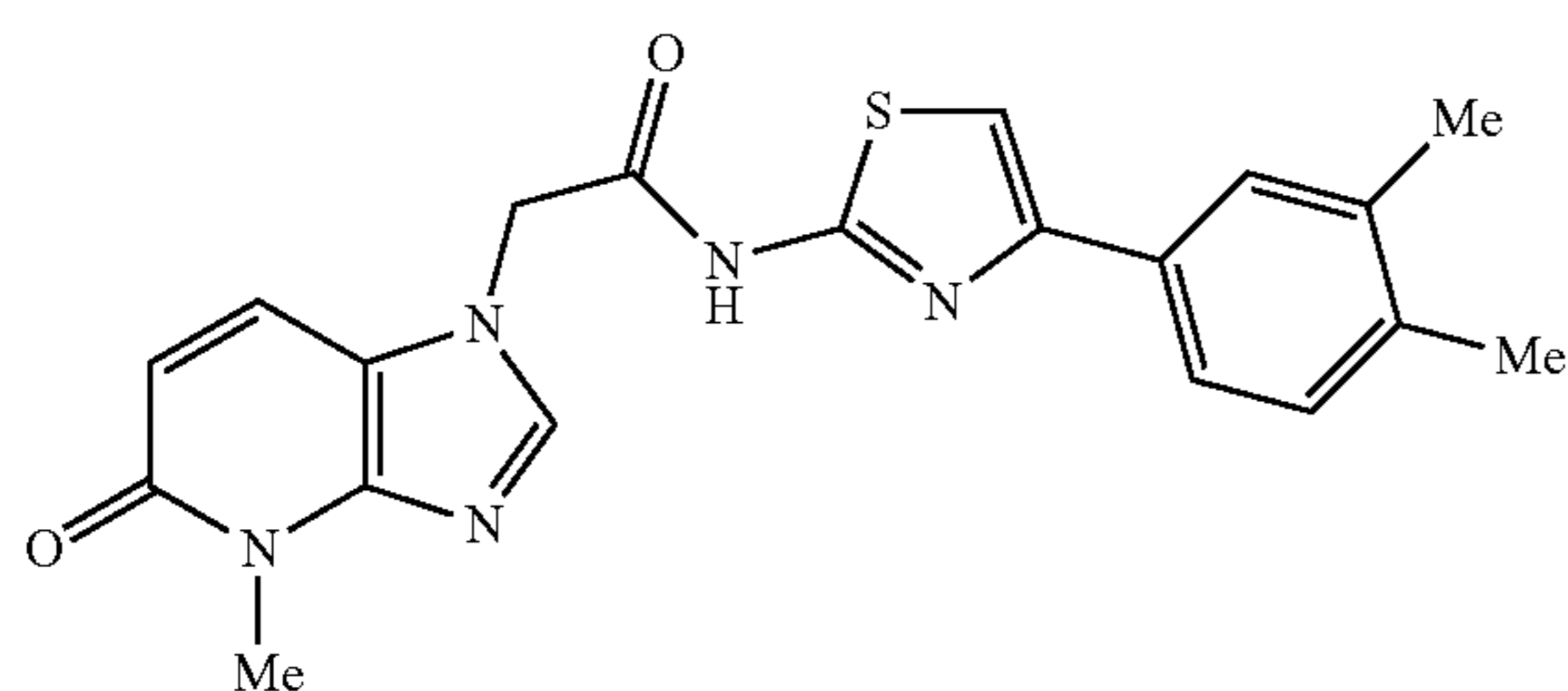
N-(4-(3,4-dimethylphenyl)thiazol-2-yl)-2-(4-methyl-5-oxo-4,5-dihydro-1H-imidazo[4,5-b]pyridin-1-yl)acetamide
