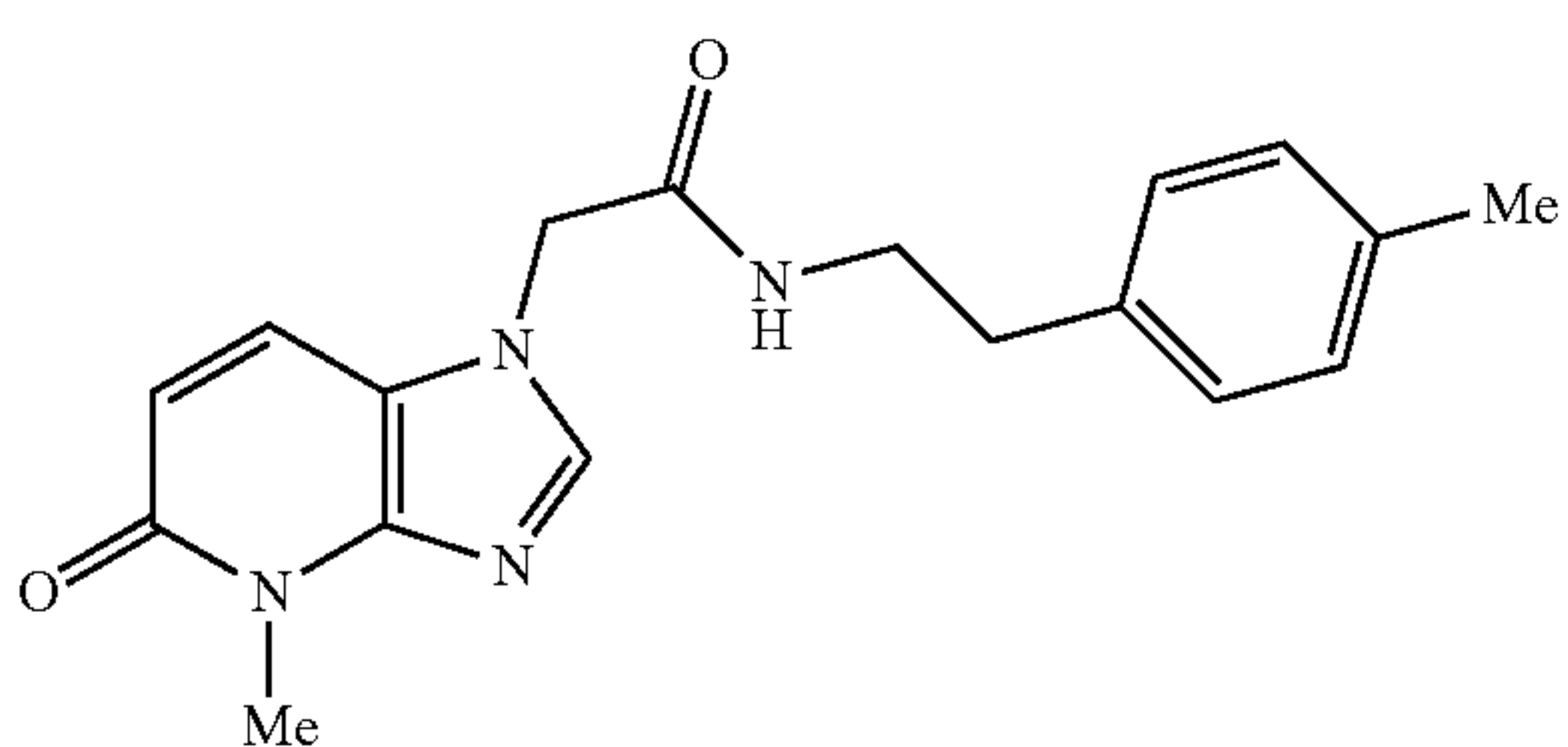
2-(4-methyl-5-oxo-4,5-dihydro-1H-imidazo[4,5-b]pyridin-1-yl)-N-(4-methylphenethyl)acetamide
