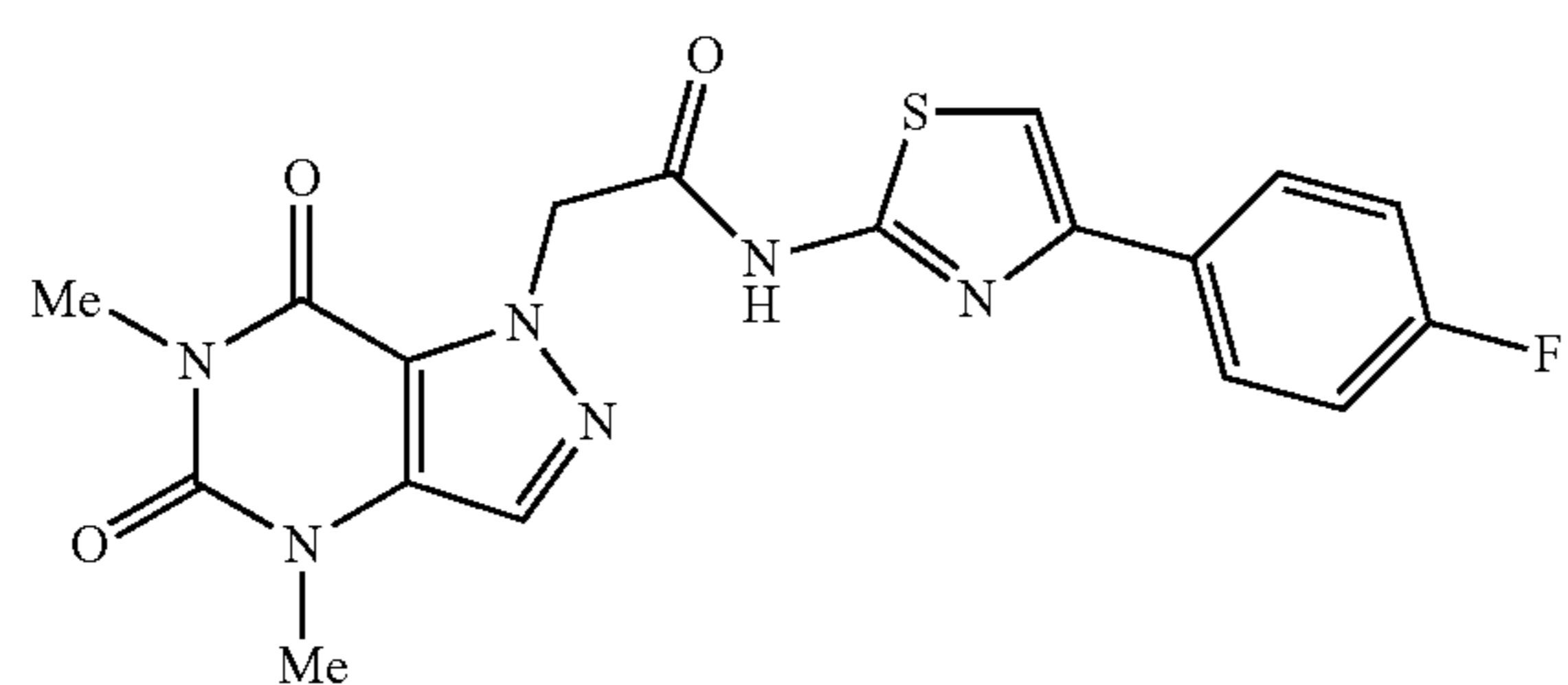
2-(4,6-dimethyl-5,7-dioxo-4,5,6,7-tetrahydro-1H-pyrazolo[4,3-d]pyrimidin-1-yl)-N-(4-(4-fluorophenyl)thiazol-2-yl)acetamide
