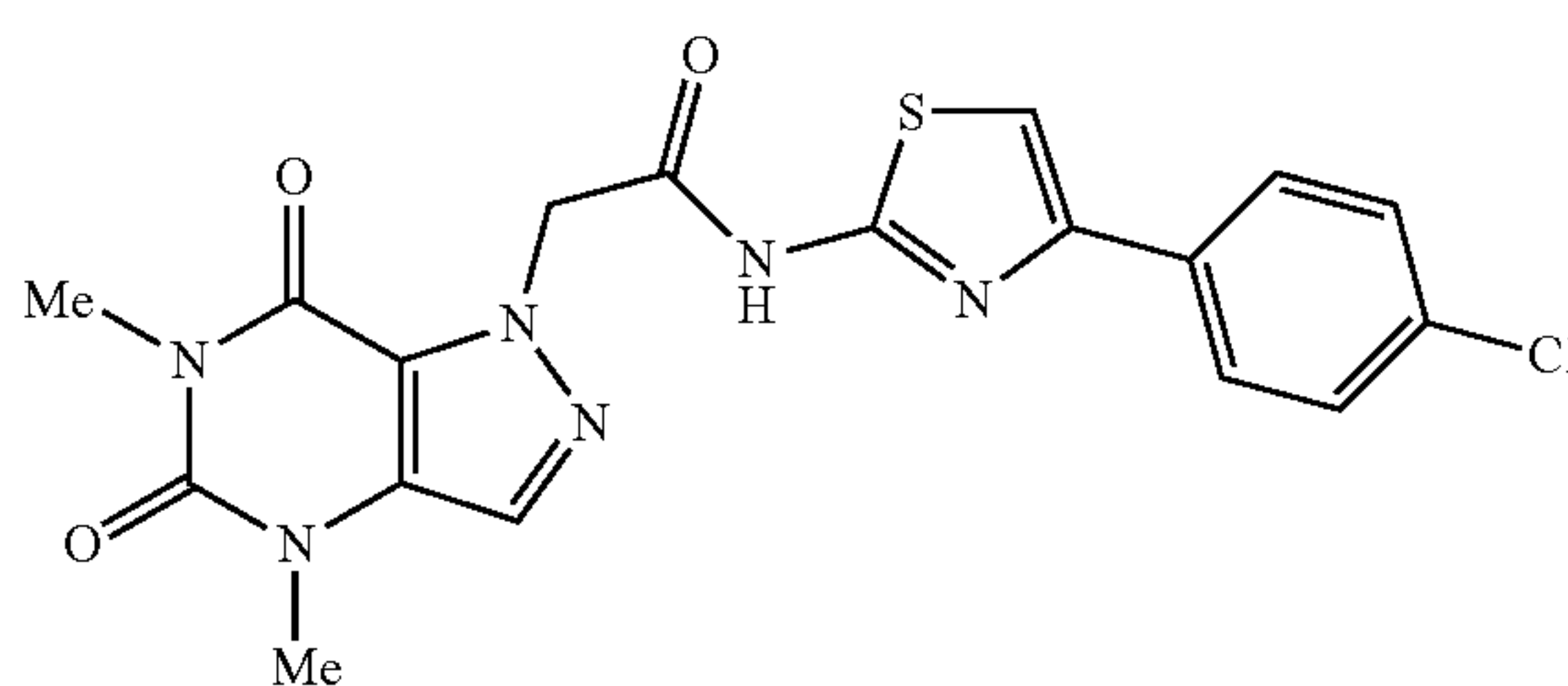
N-(4-(4-chlorophenyl)thiazol-2-yl)-2-(4,6-dimethyl-5,7-dioxo-4,5,6,7-tetrahydro-1H-pyrazolo[4,3-d]pyrimidin-1-yl)acetamide
