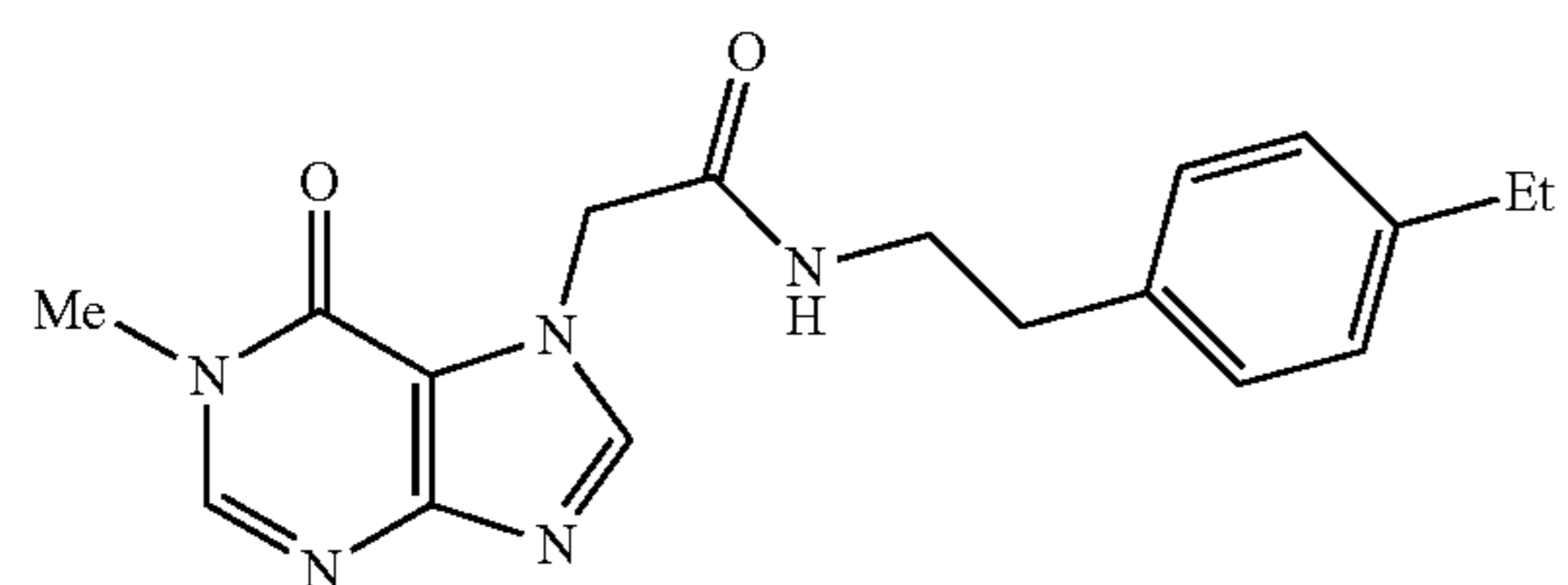
N-(4-ethylphenethyl)-2-(1-methyl-6-oxo-1H-purin-7(6H)-yl)acetamide
