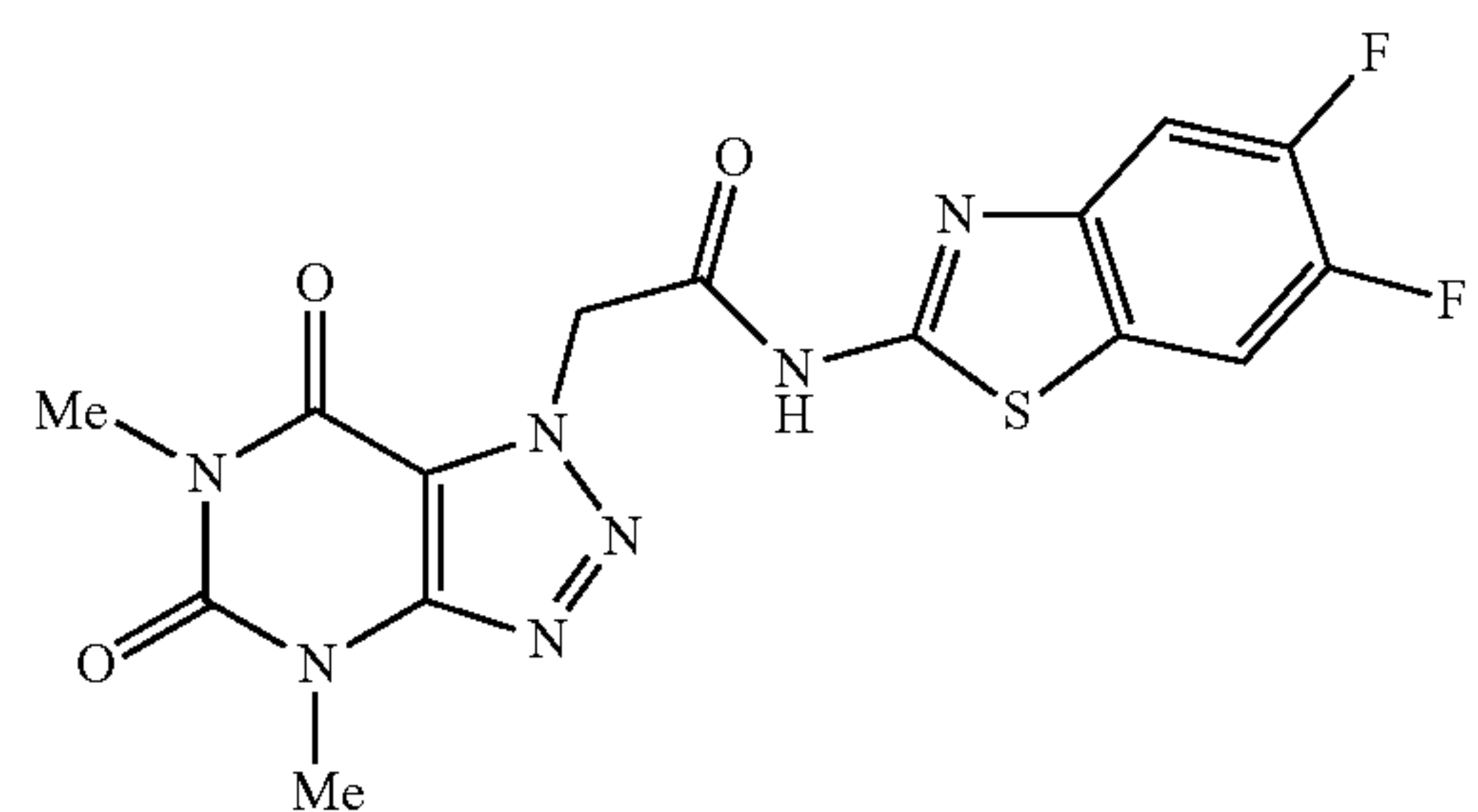
N-(5,6-difluorobenzo[d]thiazol-2-yl)-2-(4,6-dimethyl-5,7-dioxo-4,5,6,7-tetrahydro-1H-[1,2,3]triazolo[4,5-d]pyrimidin-1-yl)acetamide
