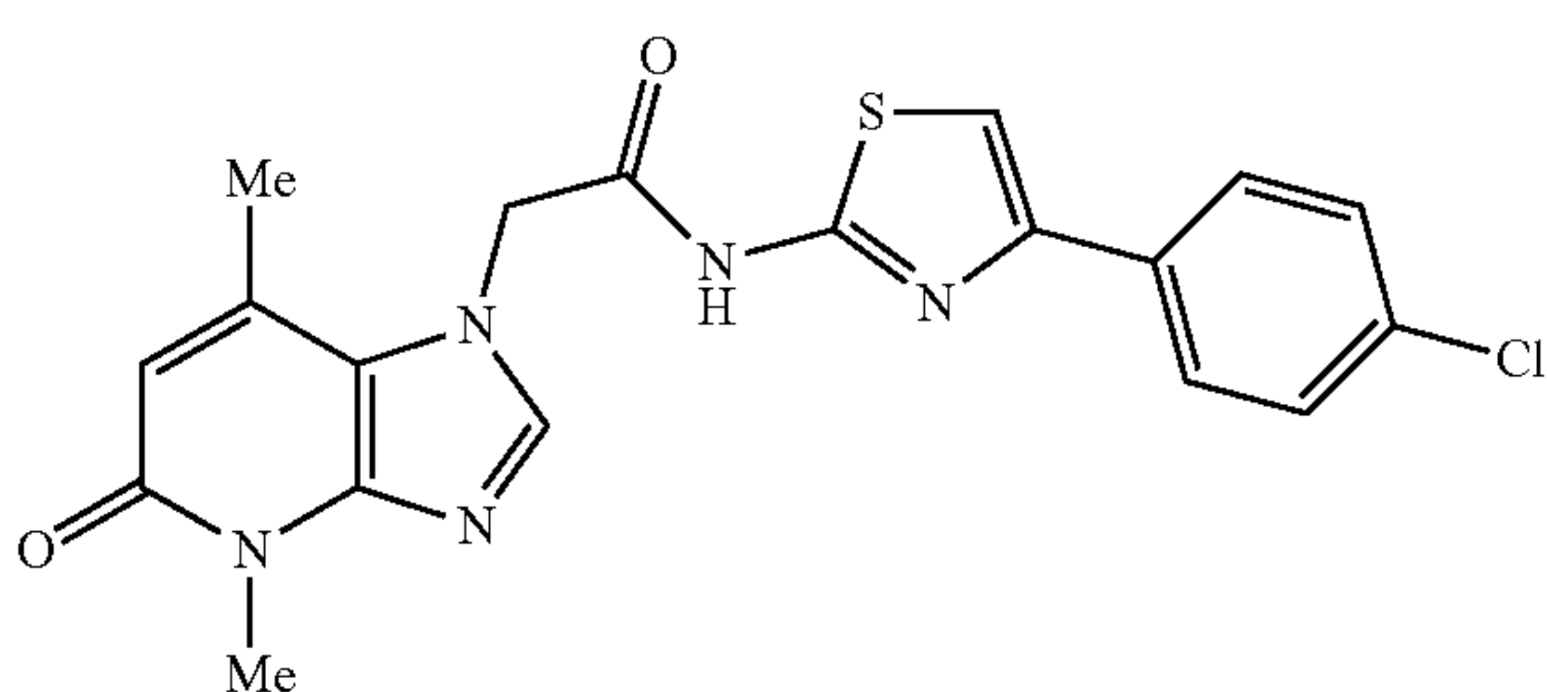
N-(4-(4-chlorophenyl)thiazol-2-yl)-2-(4,7-dimethyl-5-oxo-4,5-dihydro-1H-imidazo[4,5-b]pyridin-1-yl)acetamide
