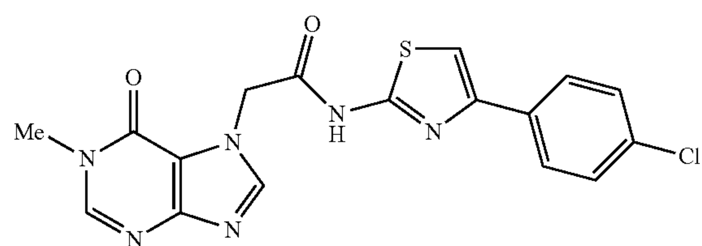
N-(4-(4-chlorophenyl)thiazol-2-yl)-2-(1-methyl-6-oxo-1H-purin-7(6H)-yl)acetamide
