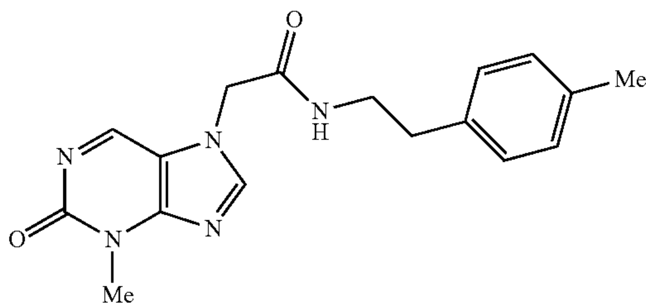
N-(4-methylphenethyl)-2-(3-methyl-2-oxo-2,3-dihydropurin-7-yl)acetamide
