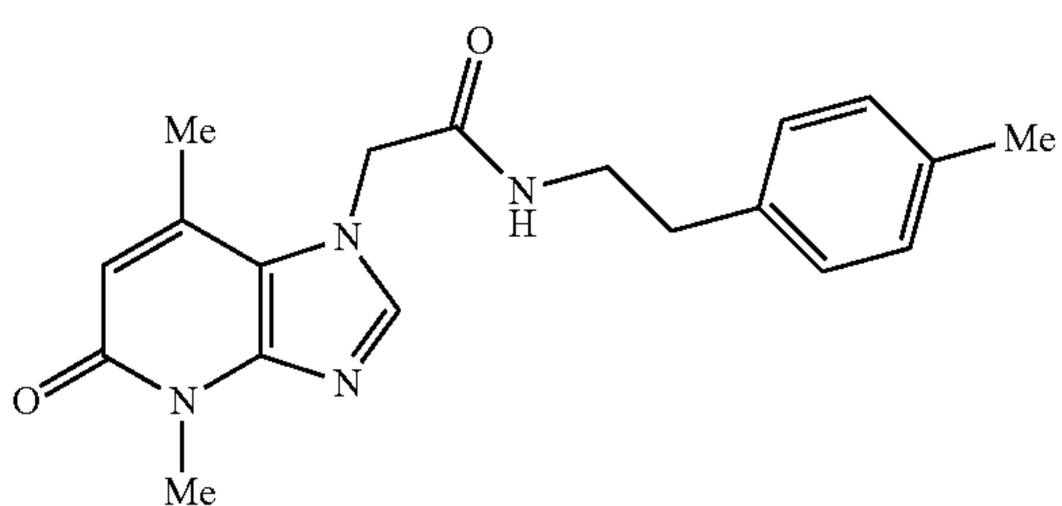
2-(4,7-dimethyl-5-oxo-4,5-dihydro-1H-imidazo[4,5-b]pyridin-1-yl)-N-(4-methylphenethyl)acetamide
