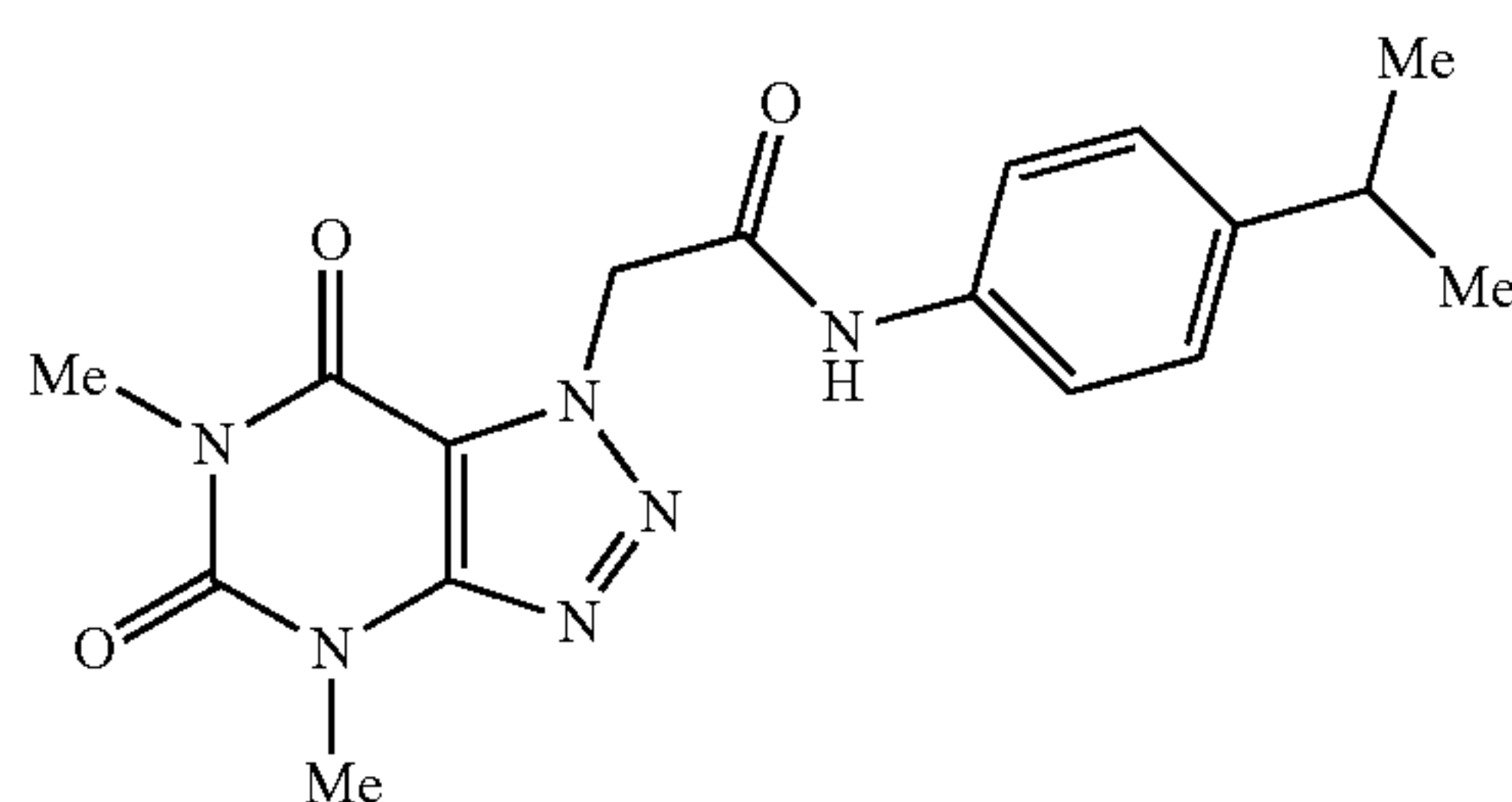
2-(4,6-dimethyl-5,7-dioxo-4,5,6,7-tetrahydro-1H-[1,2,3]triazolo[4,5-d]pyrimidin-1-yl)-N-(4-isopropylphenyl)acetamide
