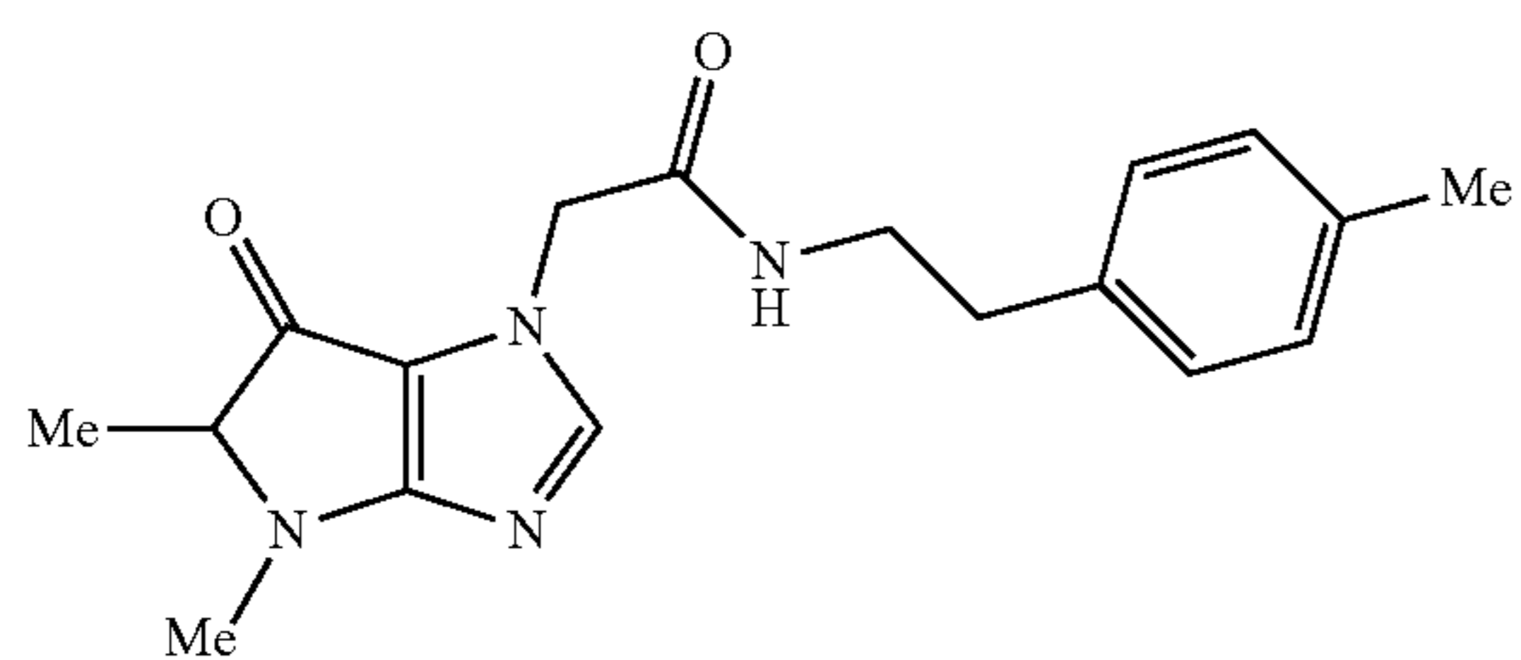
2-(4,5-dimethyl-6-oxo-5,6-dihydropyrrolo[3,2-d]imidazol-1(4H)-yl)-N-(4-methylphenethyl)acetamide
