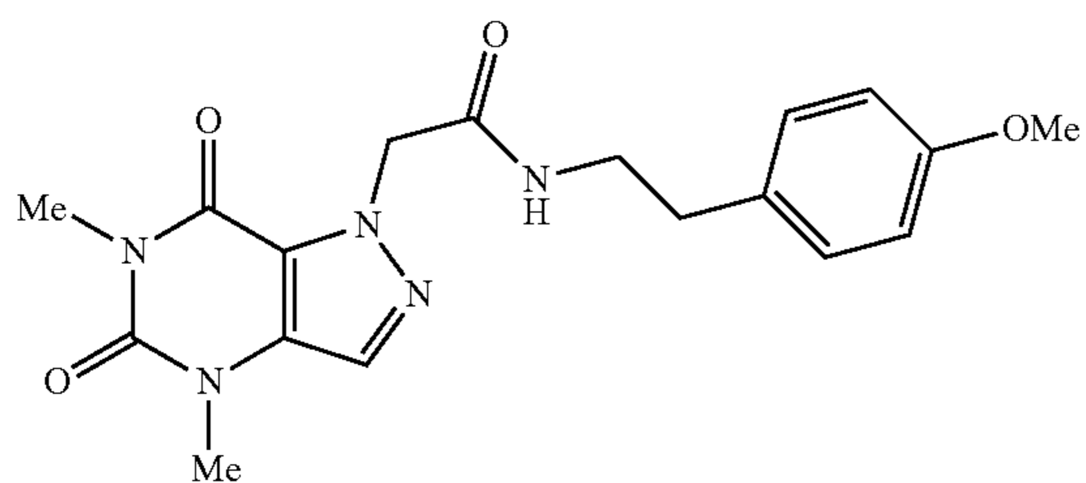
2-(4,6-dimethyl-5,7-dioxo-4,5,6,7-tetrahydro-1H-pyrazolo[4,3-d]pyrimidin-1-yl)-N-(4-methoxyphenethyl)acetamide
