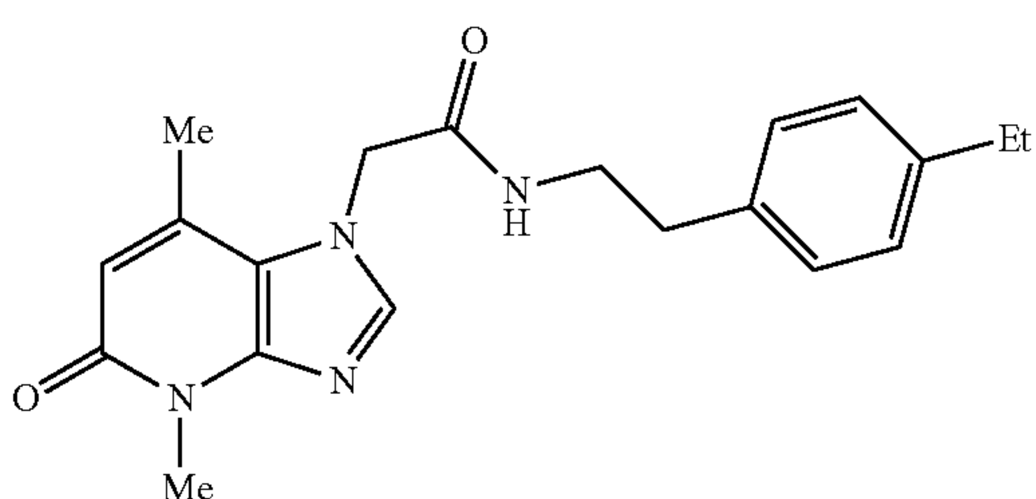
2-(4,7-dimethyl-5-oxo-4,5-dihydro-1H-imidazo[4,5-b]pyridin-1-yl)-N-(4-ethylphenethyl)acetamide
