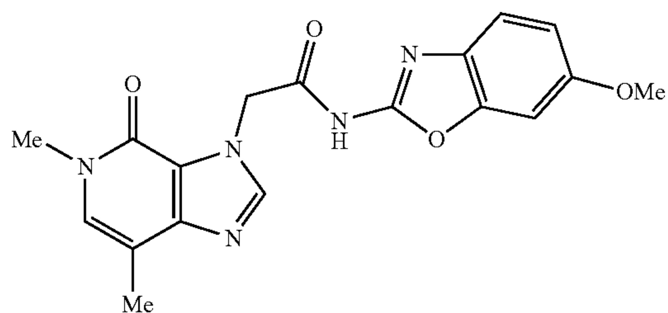
2-(5,7-dimethyl-4-oxo-4,5-dihydro-3H-imidazo[4,5-c]pyridin-3-yl)-N-(6-methoxybenzo[d]oxazol-2-yl)acetamide
