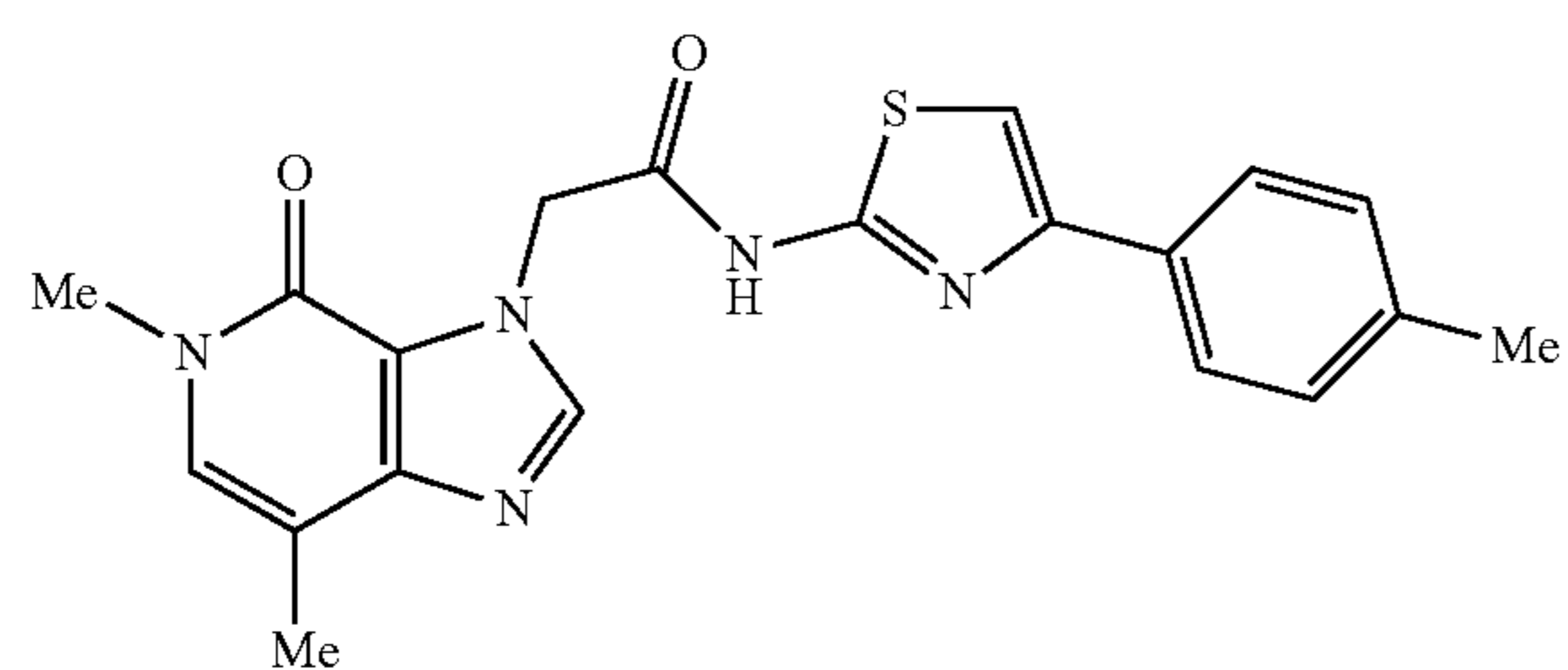
2-(5,7-dimethyl-4-oxo-4,5-dihydro-3H-imidazo[4,5-c]pyridin-3-yl)-N-(4-p-tolylthiazol-2-yl)acetamide
