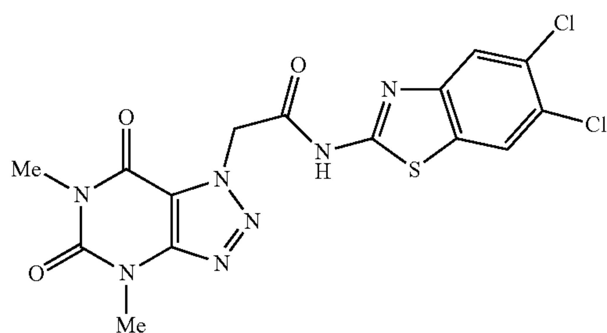
N-(5,6-dichlorobenzo[d]thiazol-2-yl)-2-(4,6-dimethyl-5,7-dioxo-4,5,6,7-tetrahydro-1H-[1,2,3]triazolo[4,5-d]pyrimidin-1-yl)acetamide
