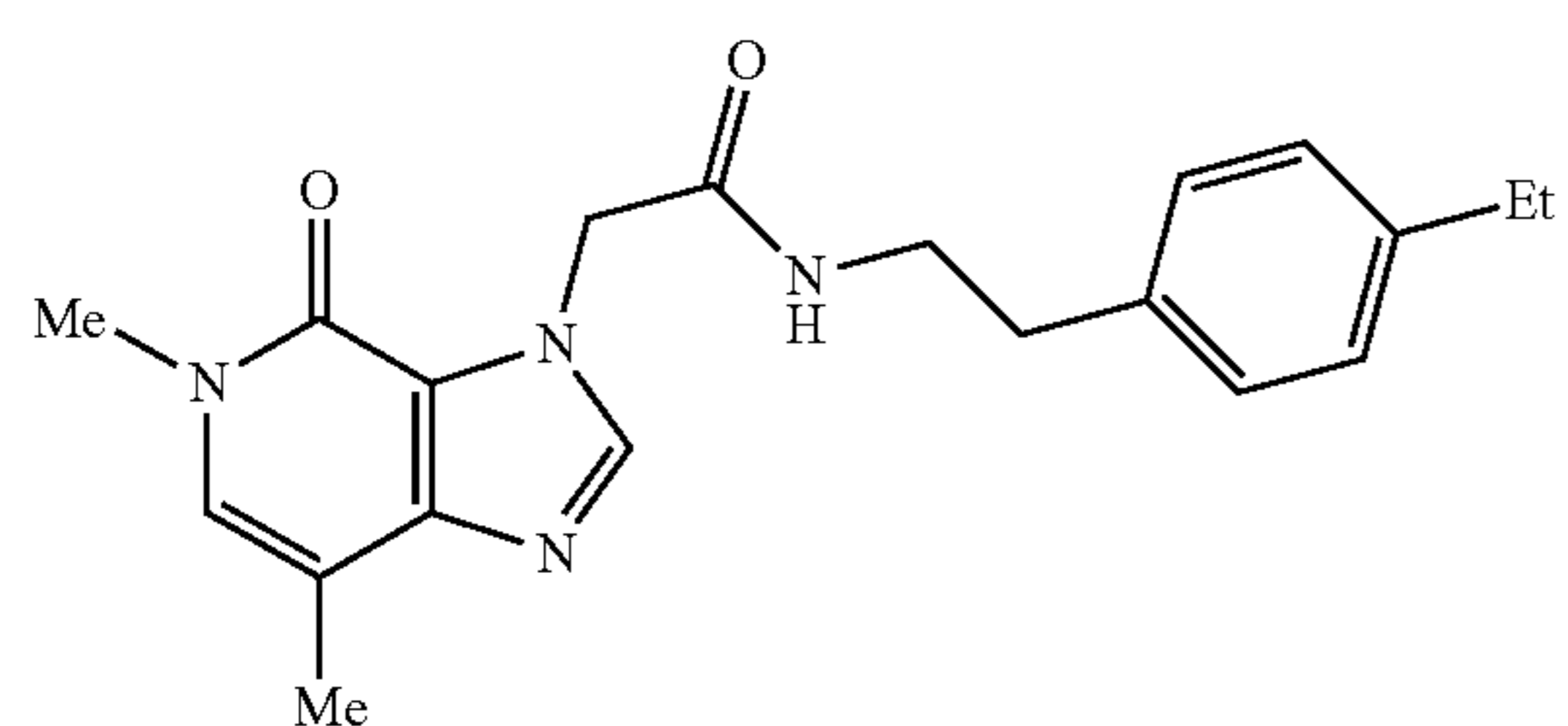
2-(5,7-dimethyl-4-oxo-4,5-dihydro-3H-imidazo[4,5-c]pyridin-3-yl)-N-(4-ethylphenethyl)acetamide
