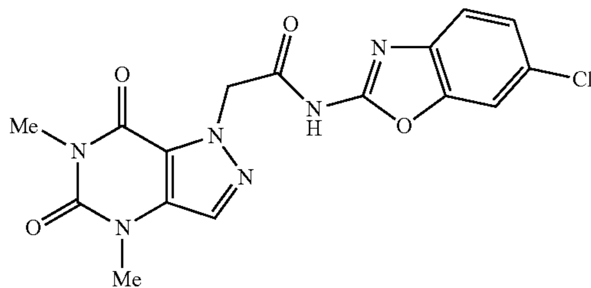
N-(6-chlorobenzo[d]oxazol-2-yl)-2-(4,6-dimethyl-5,7-dioxo-4,5,6,7-tetrahydro-1H-pyrazolo[4,3-d]pyrimidin-1-yl)acetamide
