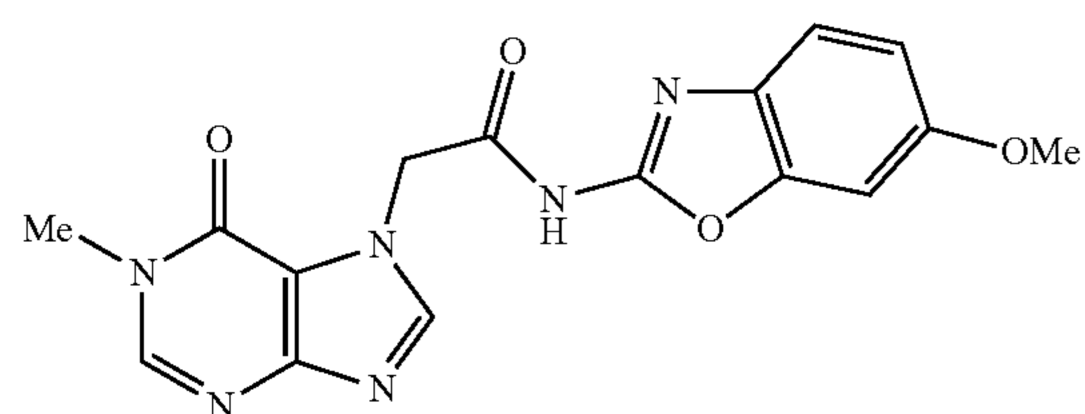
N-(6-methoxybenzo[d]oxazol-2-yl)-2-(1-methyl-6-oxo-1H-purin-7(6H)-yl)acetamide
