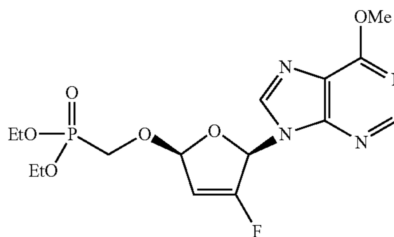
(2'R,5'R)-6-Methoxy-9-[3-fluoro-2,5-dihydro-5-(diethoxyphosphinyl)methoxy-2-furanyl]purine (7)
