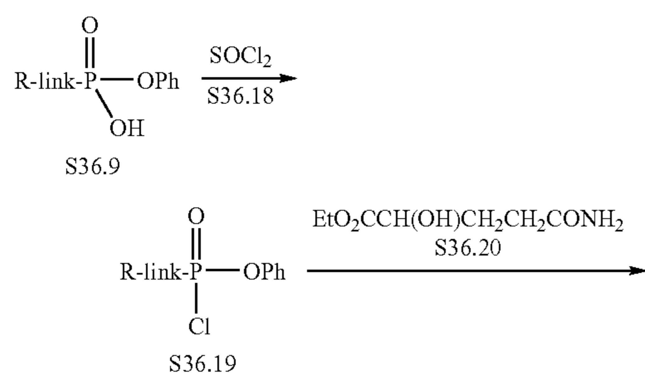
Scheme 36 Example 3
