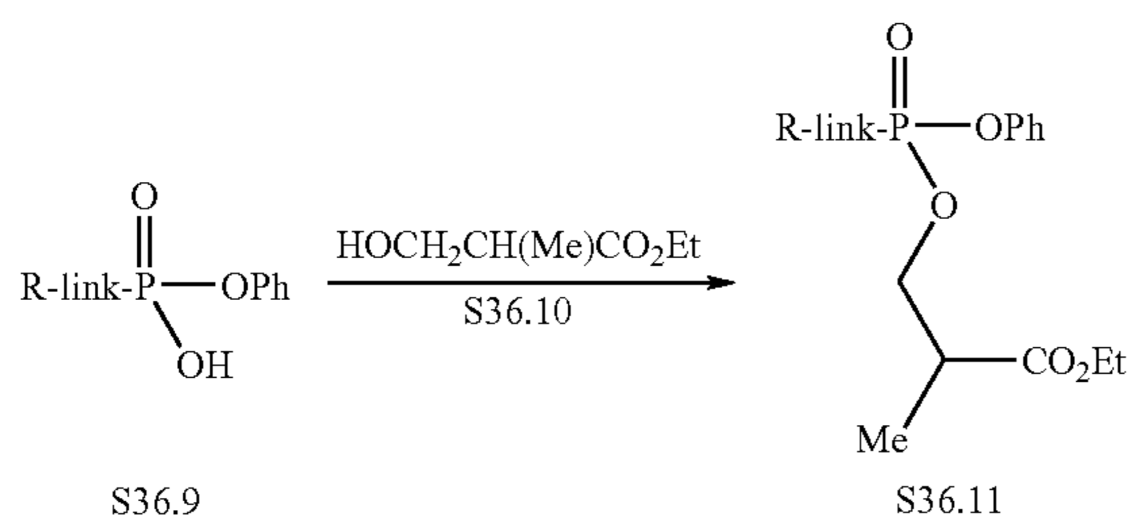
Scheme 36 Example 1
