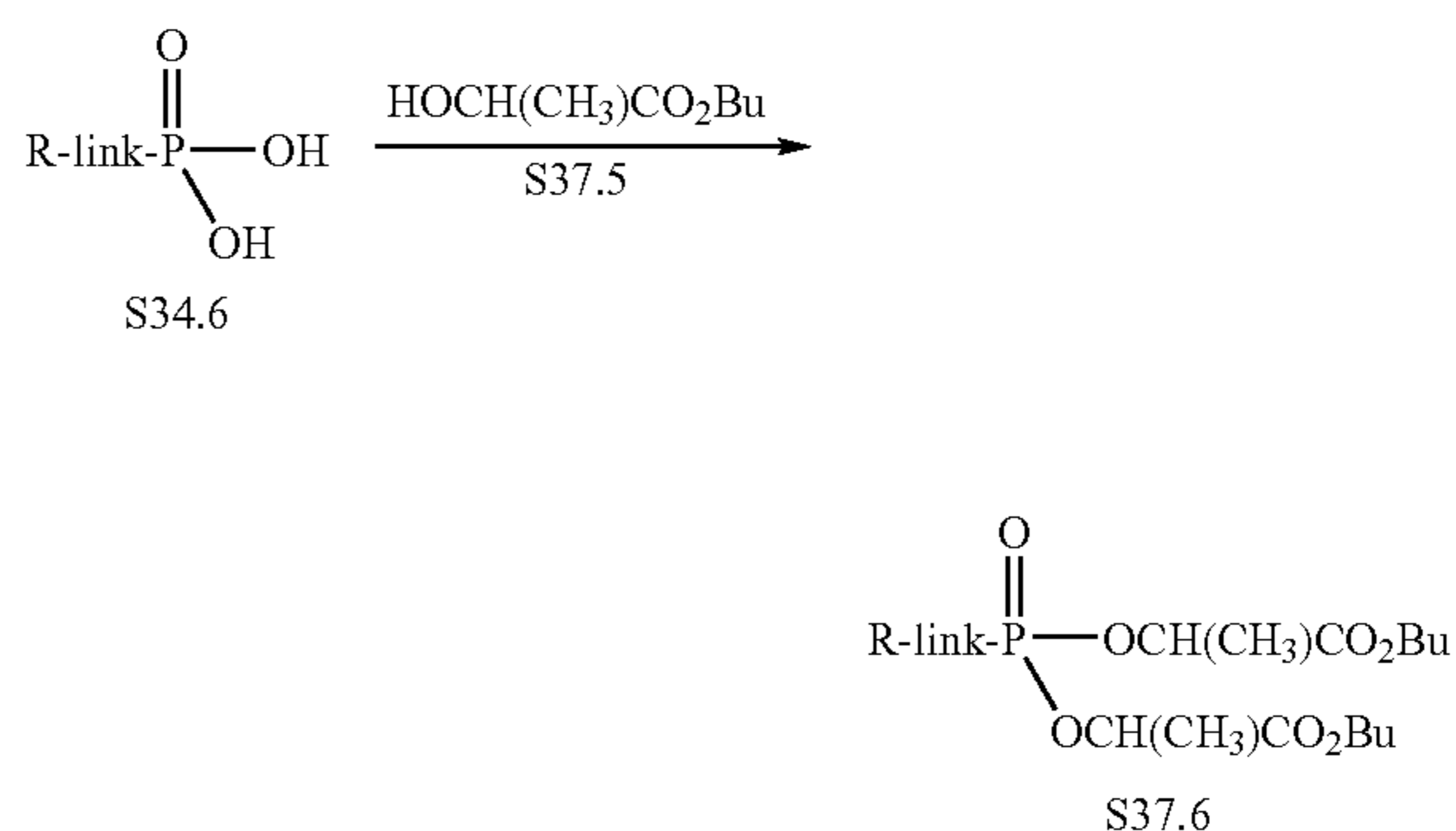
Scheme 37 Example 1
