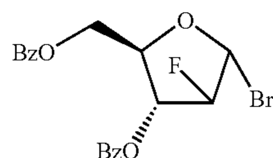
2-deoxy-2-fluoro-3,5-di-O-benzoyl- \beta -D-arabinofuranosylbromide (2)
