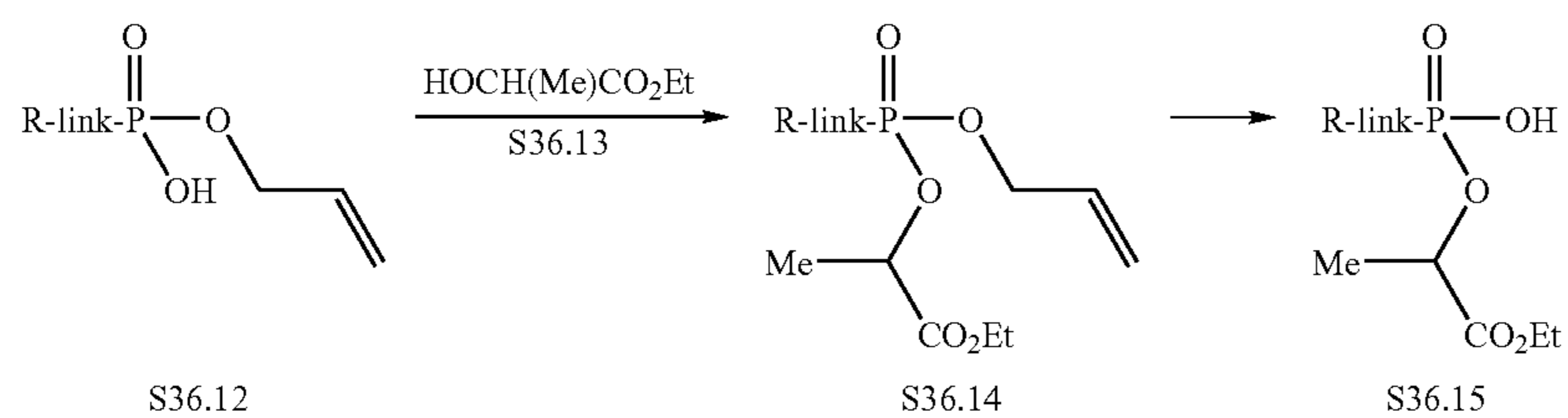
Scheme 36 Example 2
