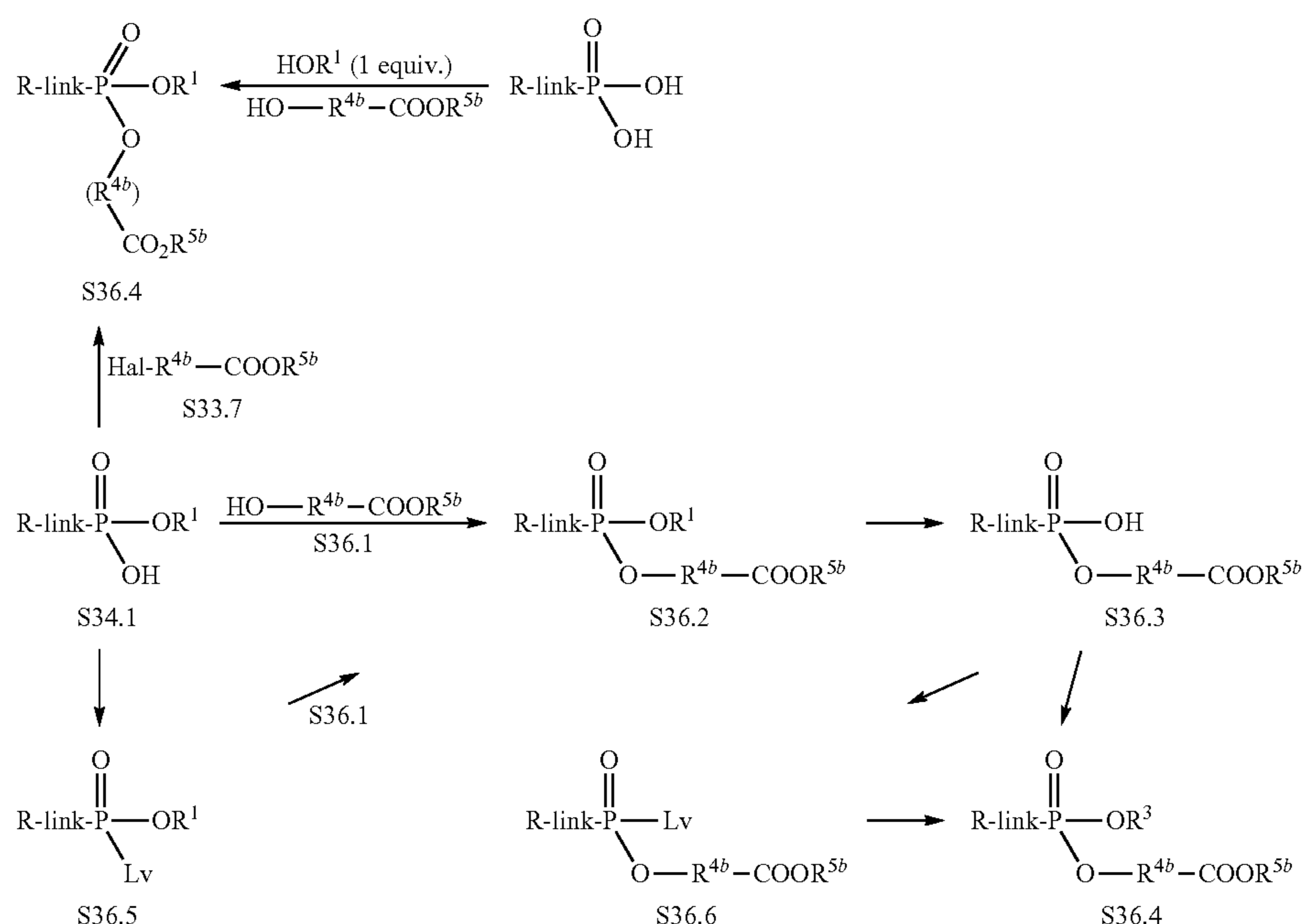
Scheme 36
