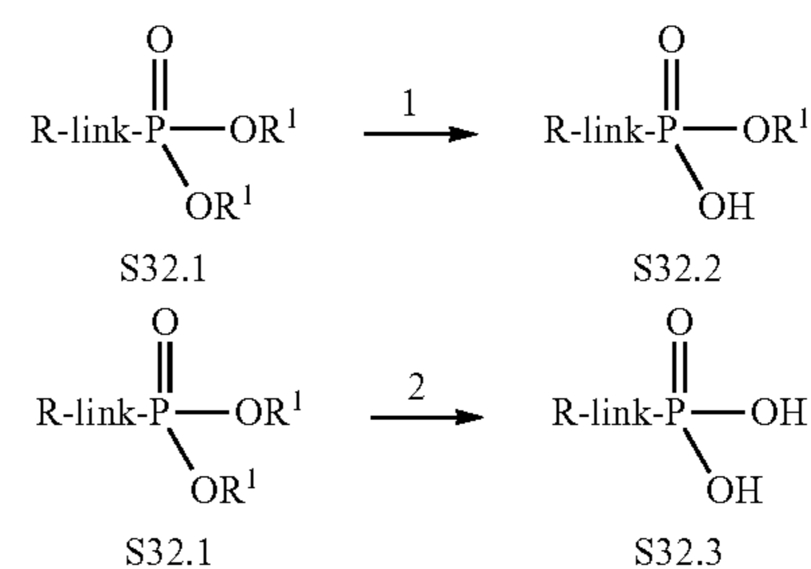
Scheme 32
