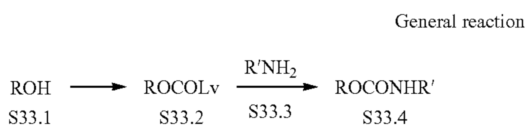
Scheme 33. Preparation of carbamates.
