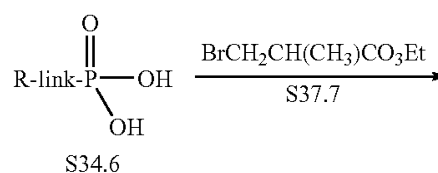
Scheme 37 Example 2
