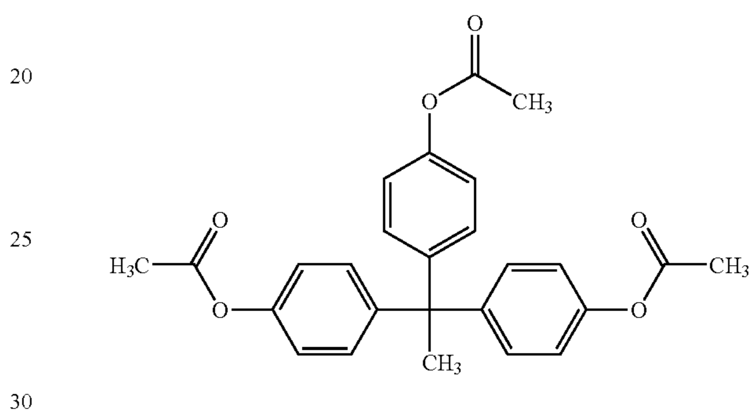
1,1,1-Tris-(4-acetoxyphenyl)ethane (I-9)
