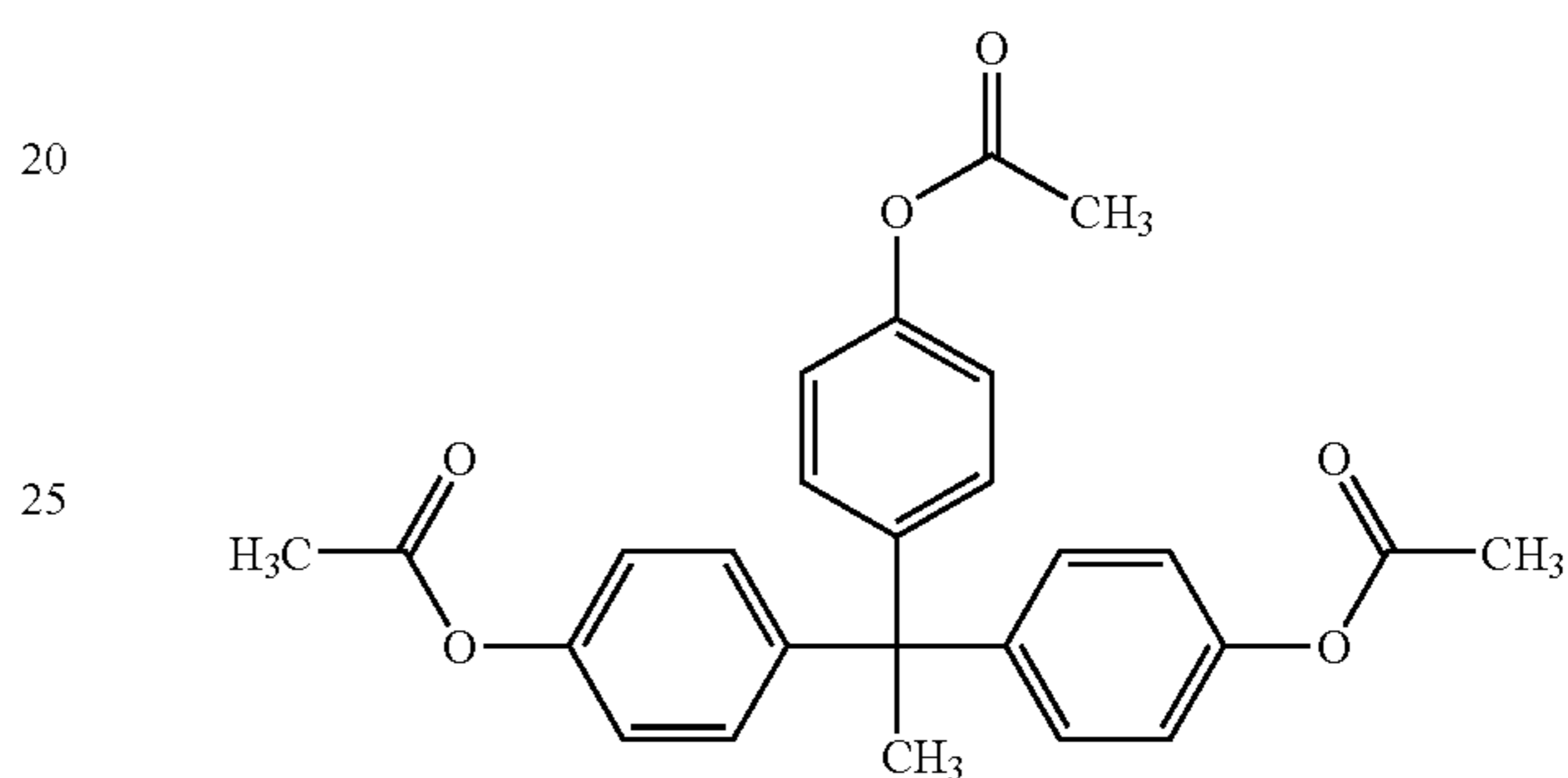
1,1,1-Tris-(4-acetoxyphenyl)ethane (I-9)
