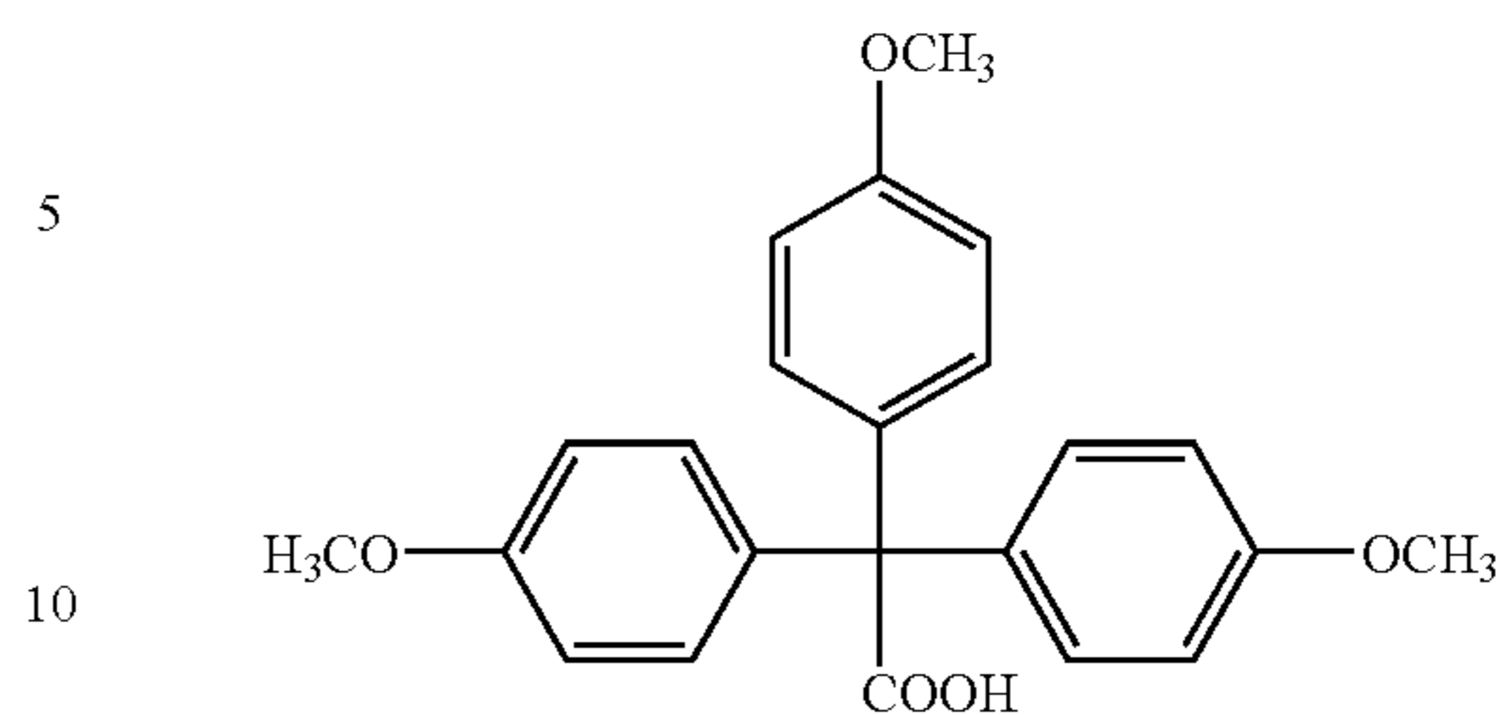
1,1,1-Tris-(4-methoxyphenyl)acetic acid (I-8)
