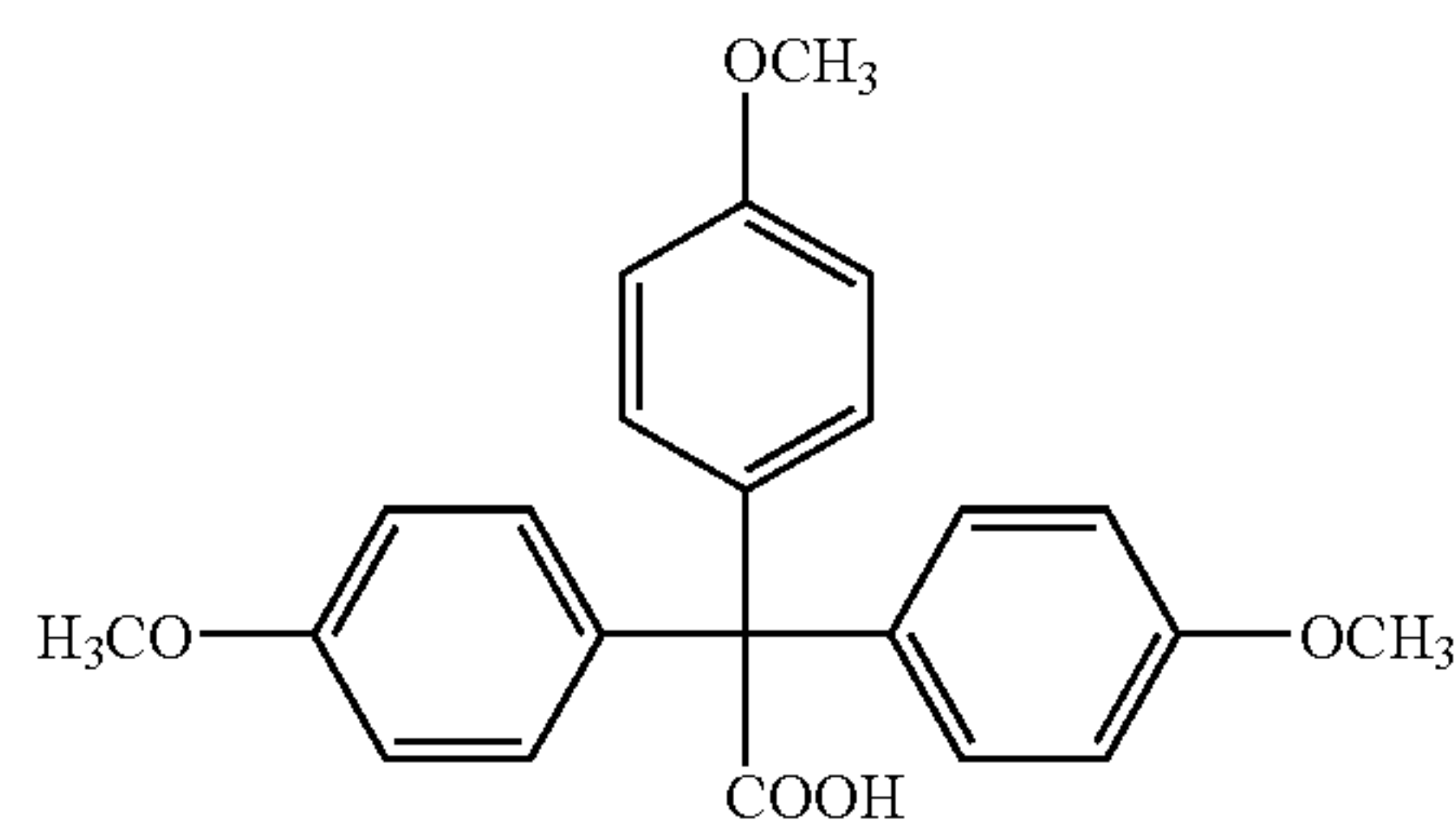
1,1,1-Tris-(4-methoxyphenyl)acetic acid (I-8)
