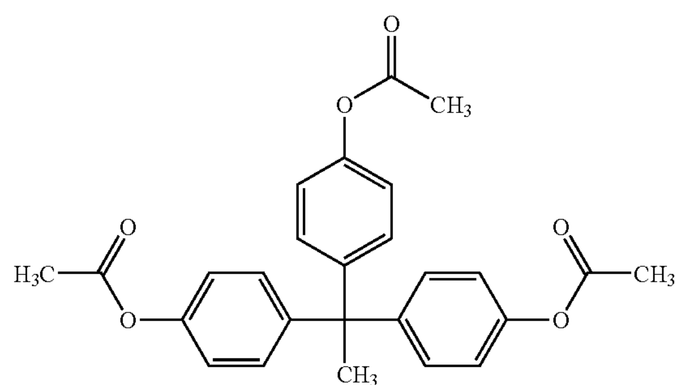
1,1,1-Tris-(4-acetoxyphenyl)ethane (I-9)
