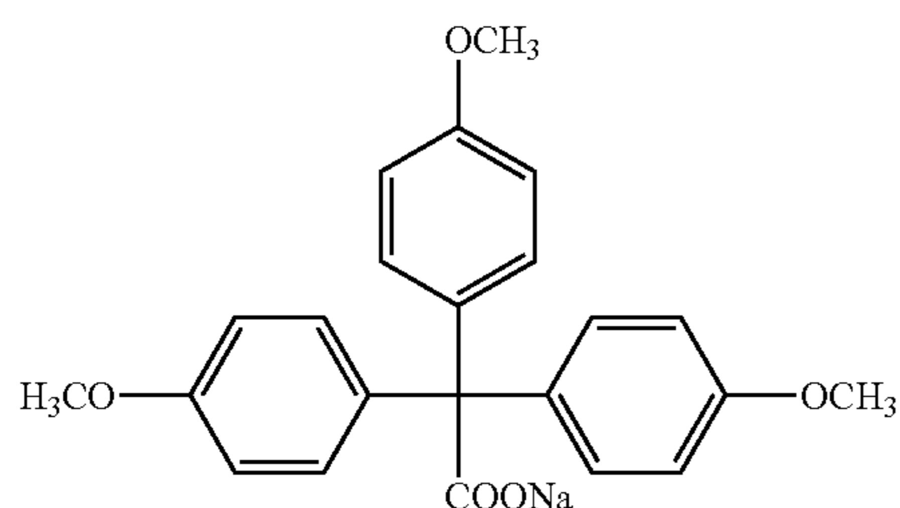
Sodium 1,1,1-tris-(4-methoxyphenyl)acetate (I-5)
