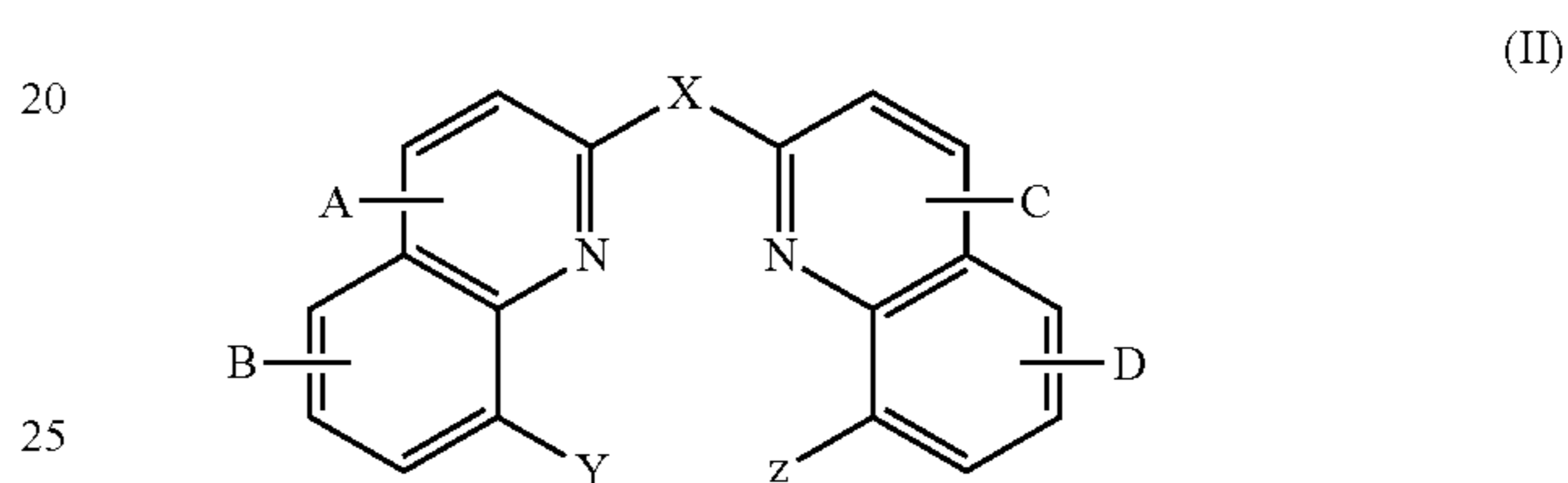
Ligands of the general formula (II)
