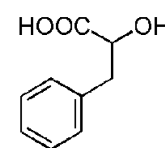
phenyl lactic acid
