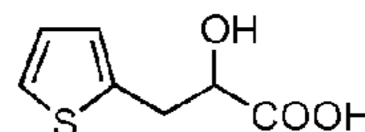
thienyl acetic acid
