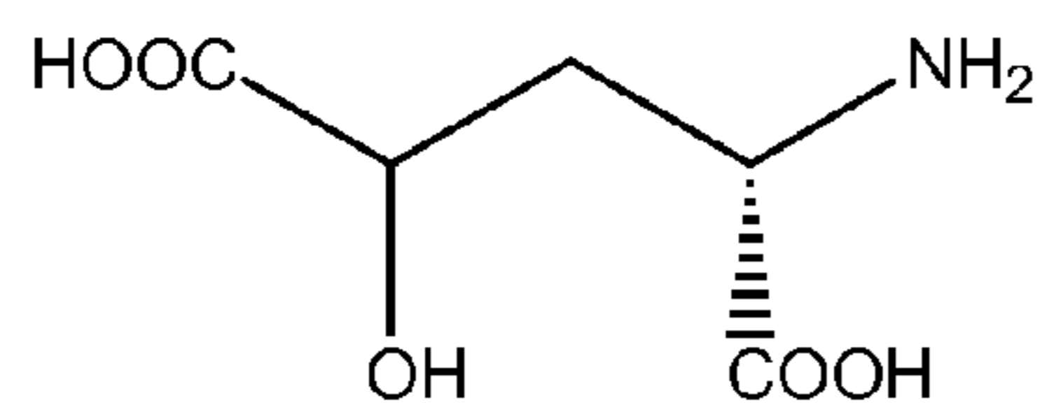
L-gamma-hydroxy glutamate
