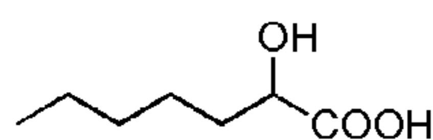
2-hydroxy heptanoic acid
