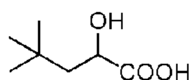
2-hydroxy-4-di-methyl-pentanoic acid
