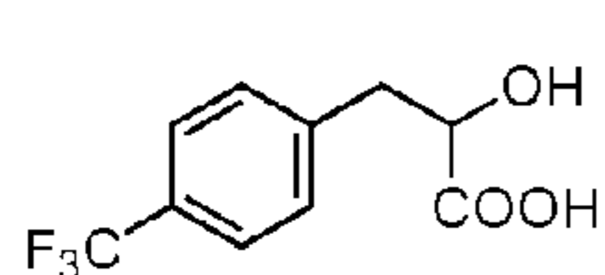
trifluoromethylphenyl lactic acid
