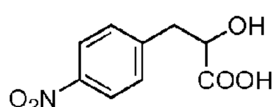
nitro phenyl lactic acid
