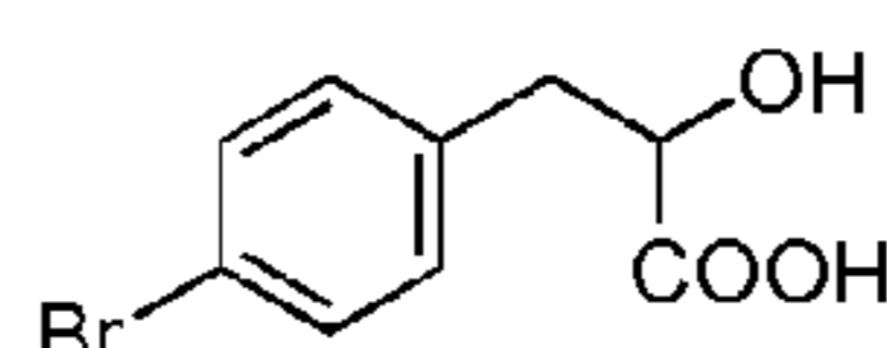
bromophenyl lactic acid
