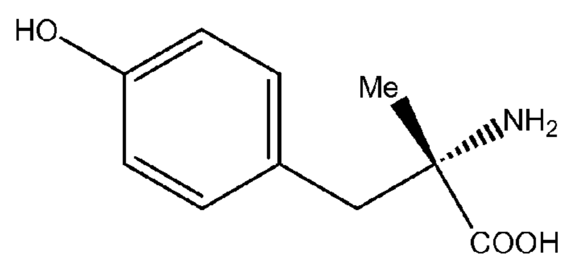
alpha-methyl-L-tyrosine
