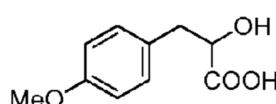
methoxy phenyl lactic acid
