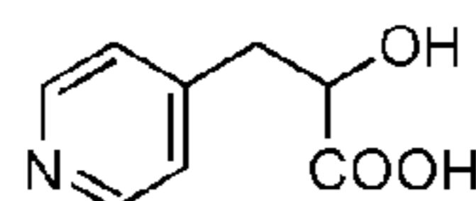
pyridyl acetic acid
