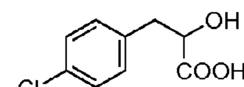
chlorophenyl lactic acid
