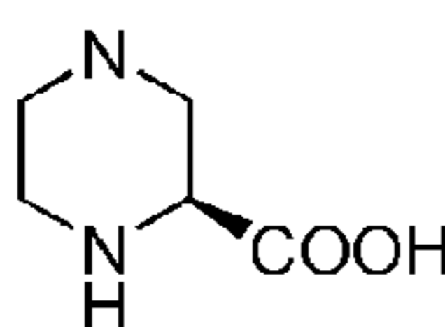
2-carboxy-piperazine
