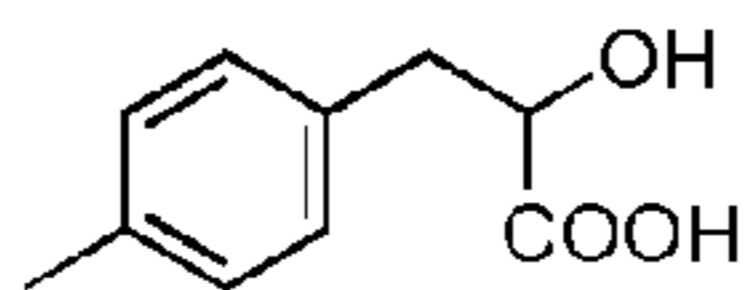
methyl phenyl lactic acid
