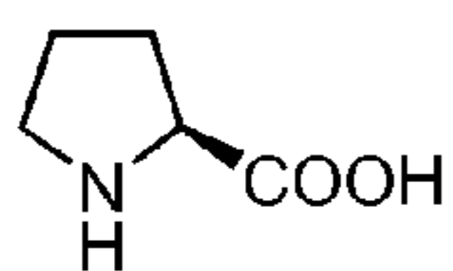
2-carboxy-cyclobutyl amine
