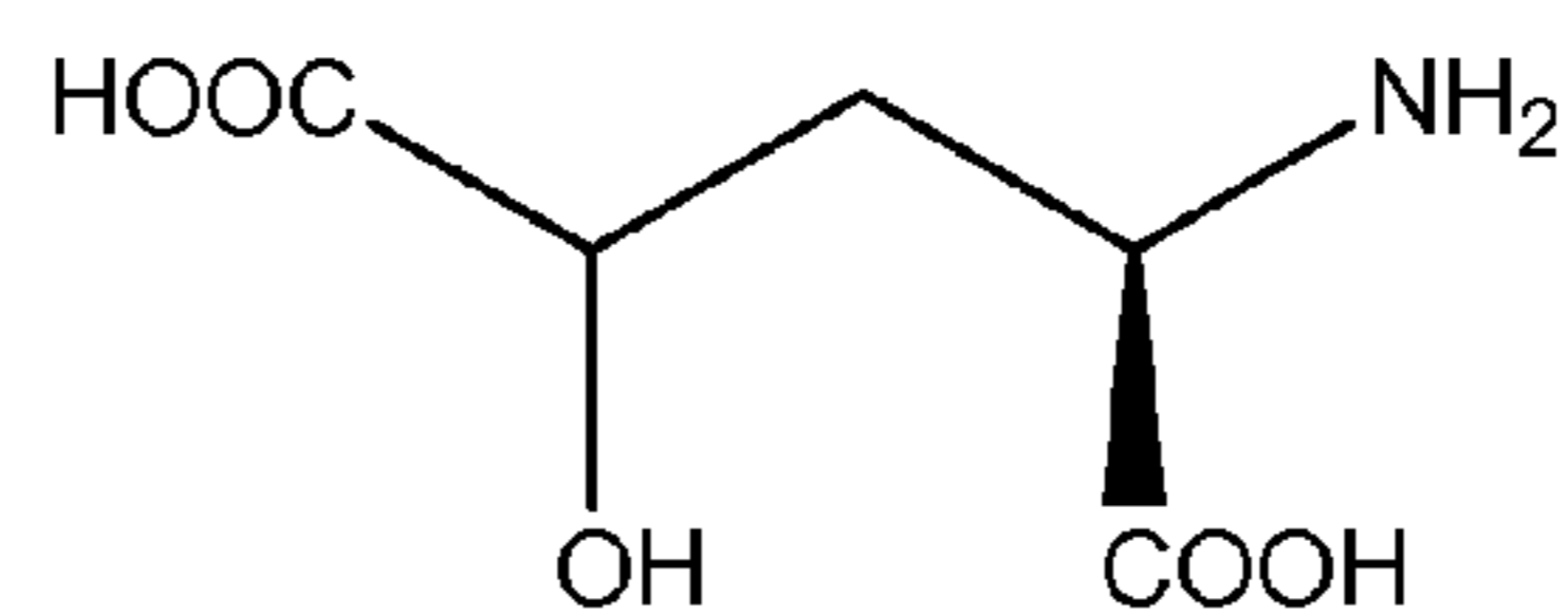
D-gamma-hydroxy glutamate
