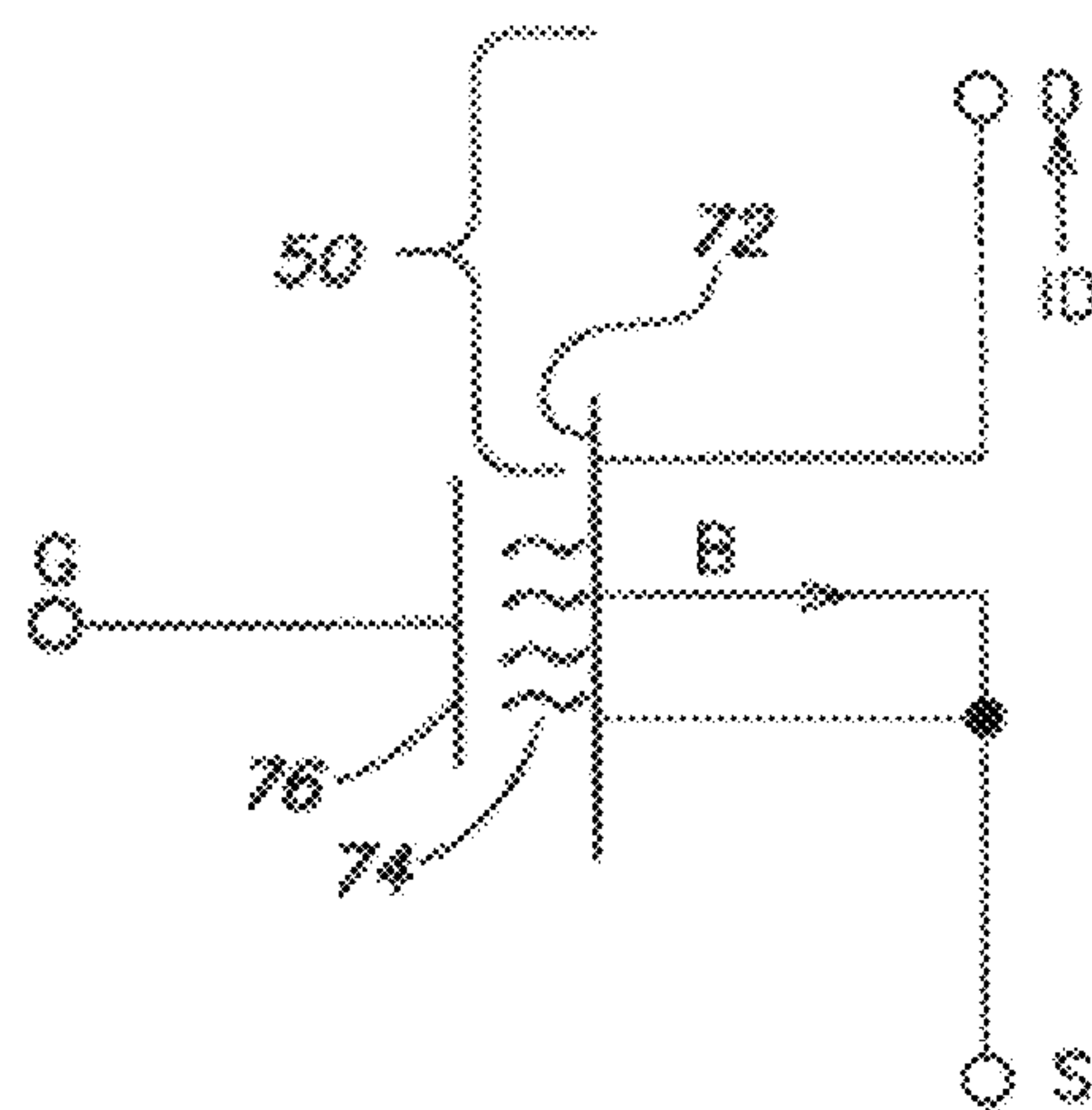
FIG. 2 (Prior Art)
