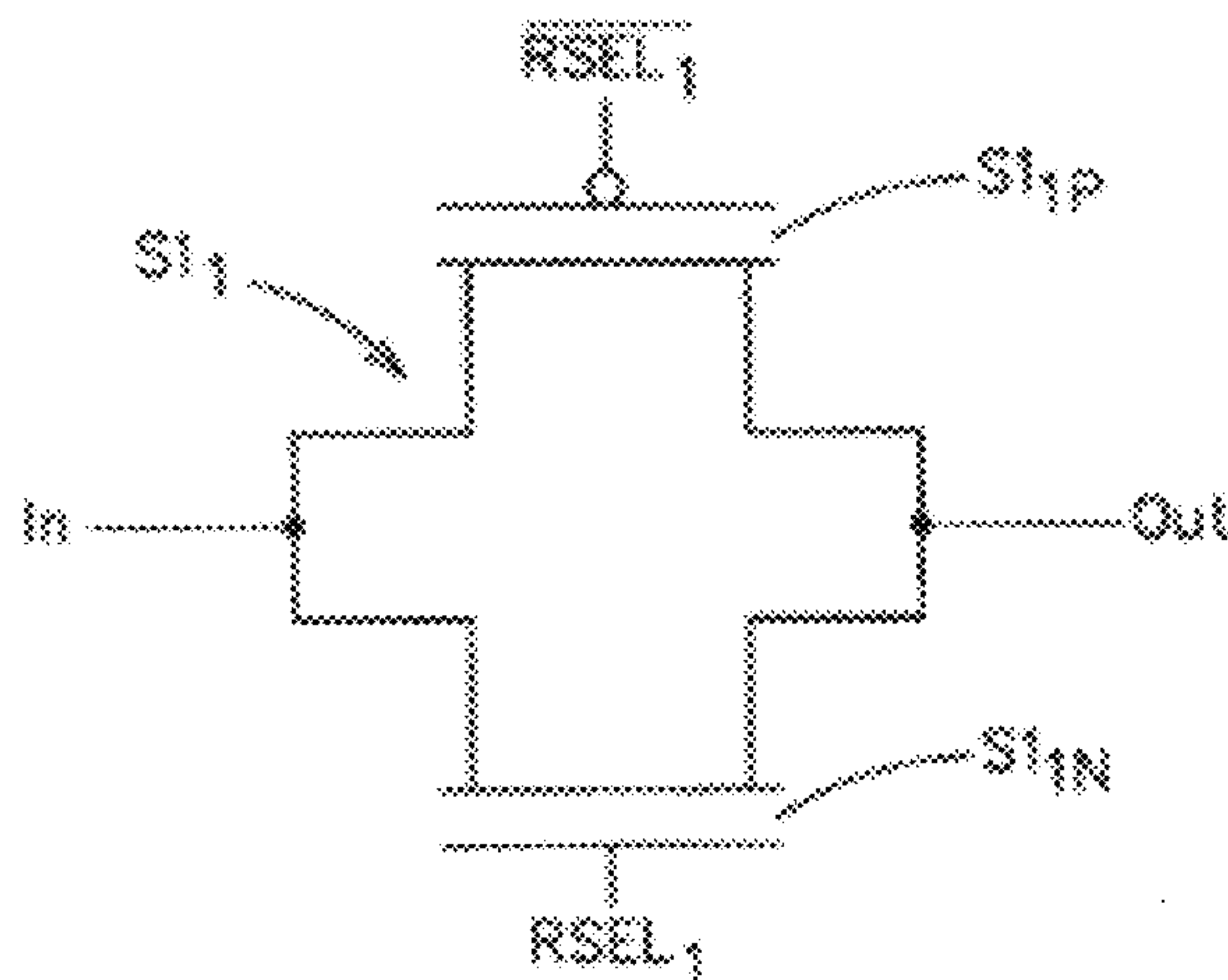
FIG. 4 (Prior Art)
