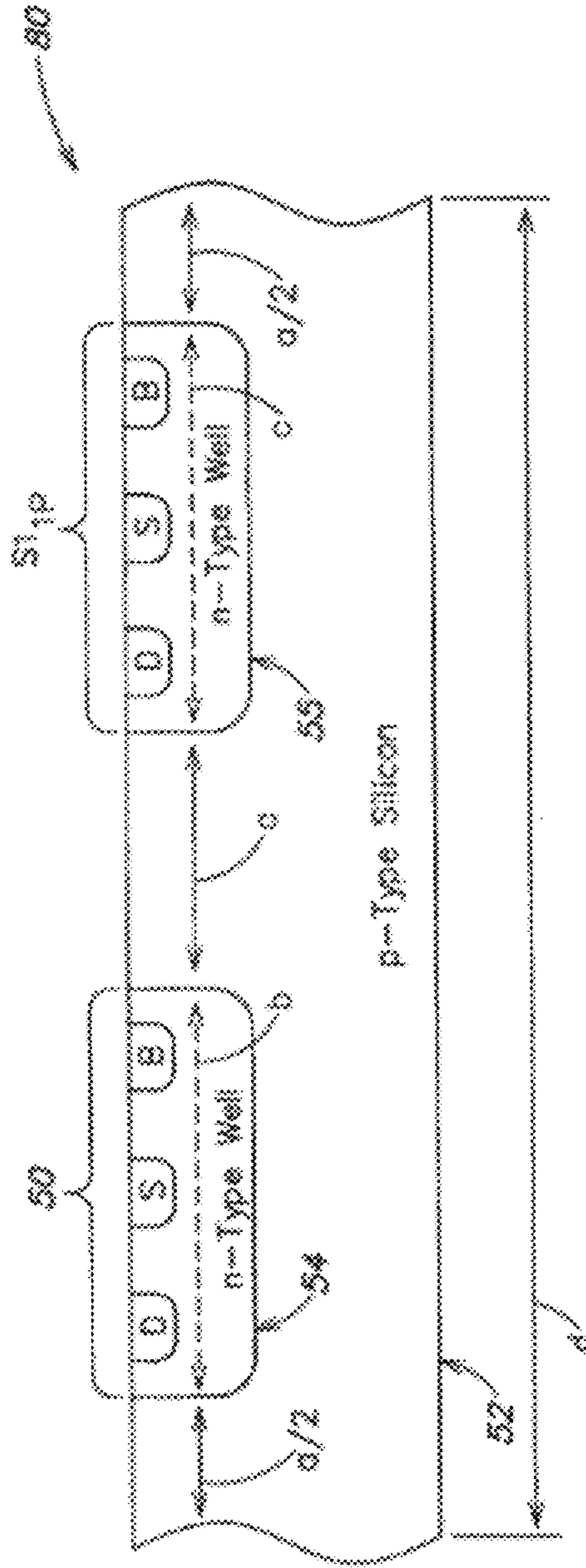
FIG. 5 (Prior Art)
