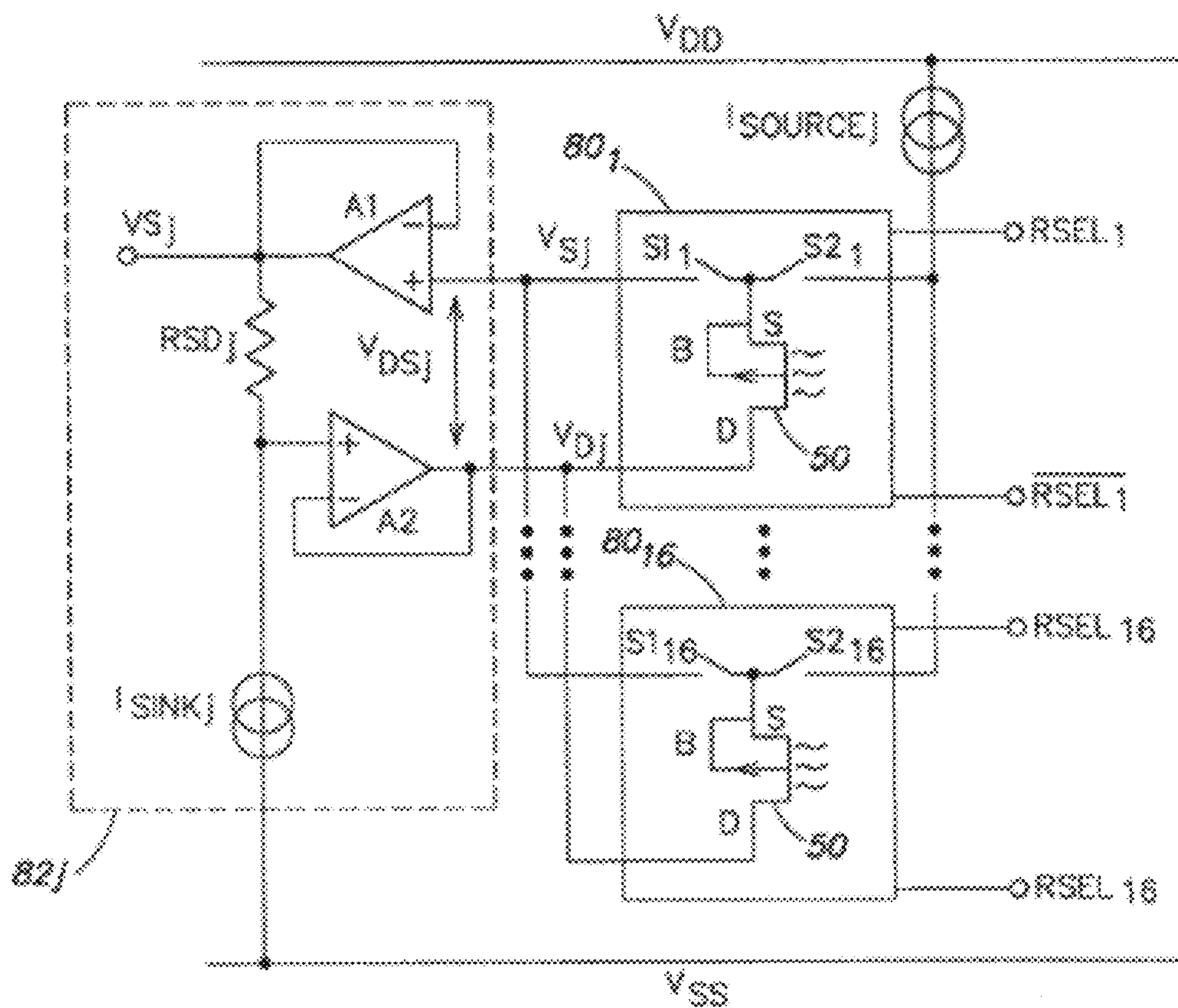
FIG. 3 (Prior Art)
