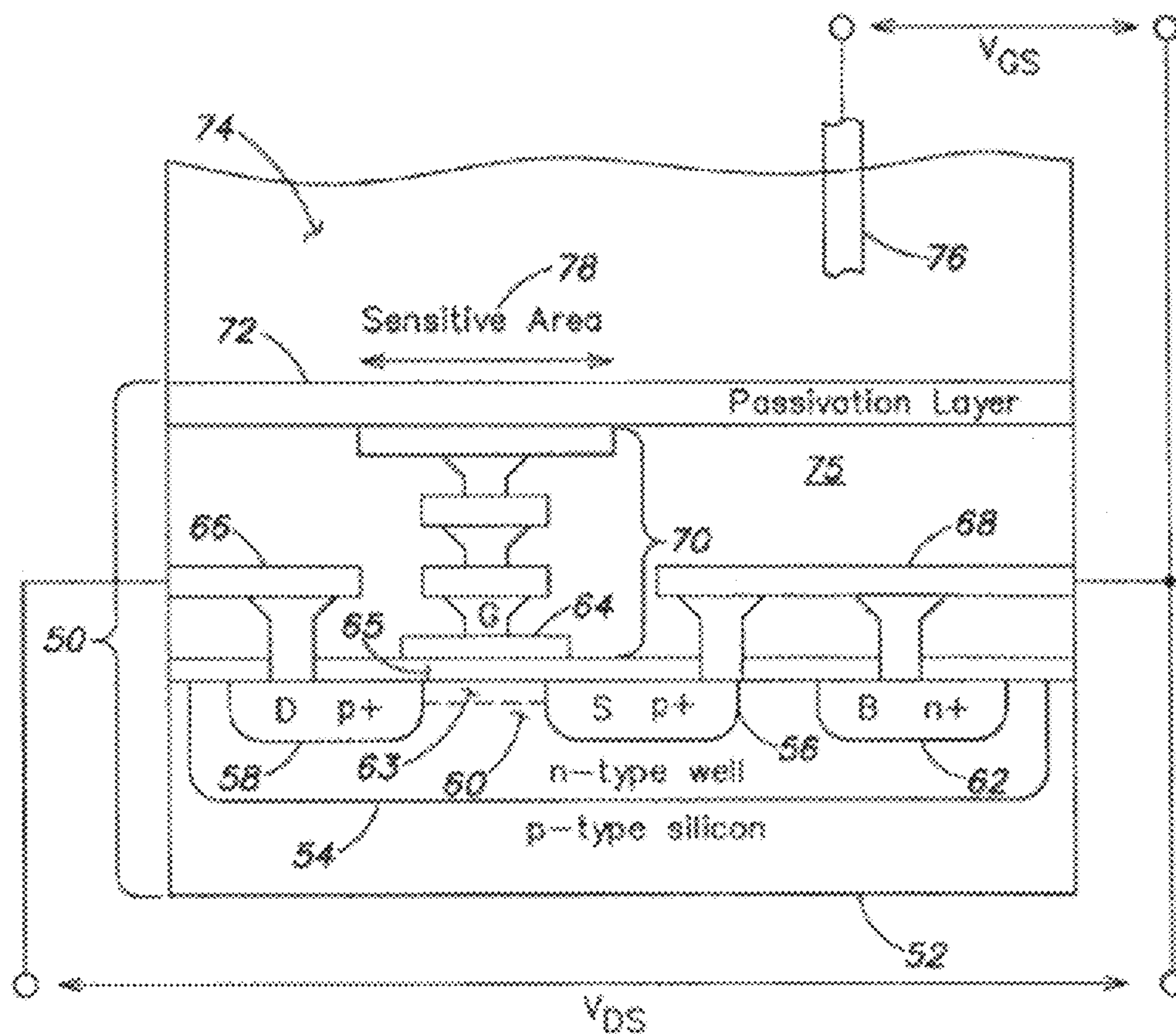
FIG. 1 (Prior Art)
