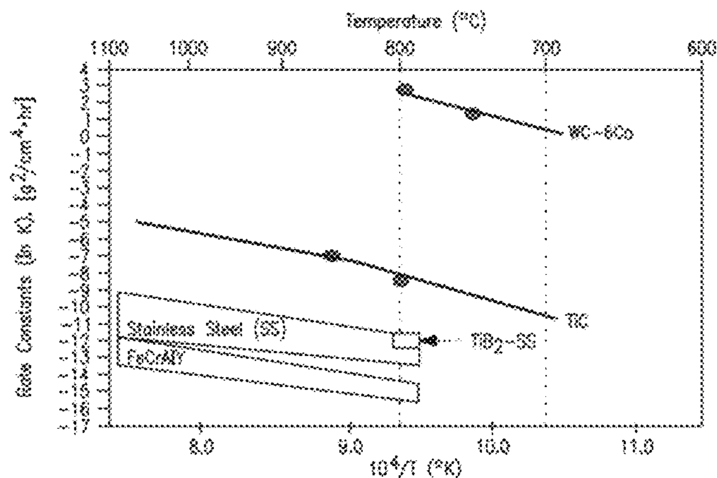
Corrosion Resistance Versus Temperature of Prior Art TiC, FeCrAlY, Stainless Steel (SS) and WC-6Co In Comparison to TiB 2 -SS Cermet of Present Invention: (a) and SEM Images of Corrosion Layer Formed on WC-Co Cermet and TiB 2 -SS Cermet (b)
