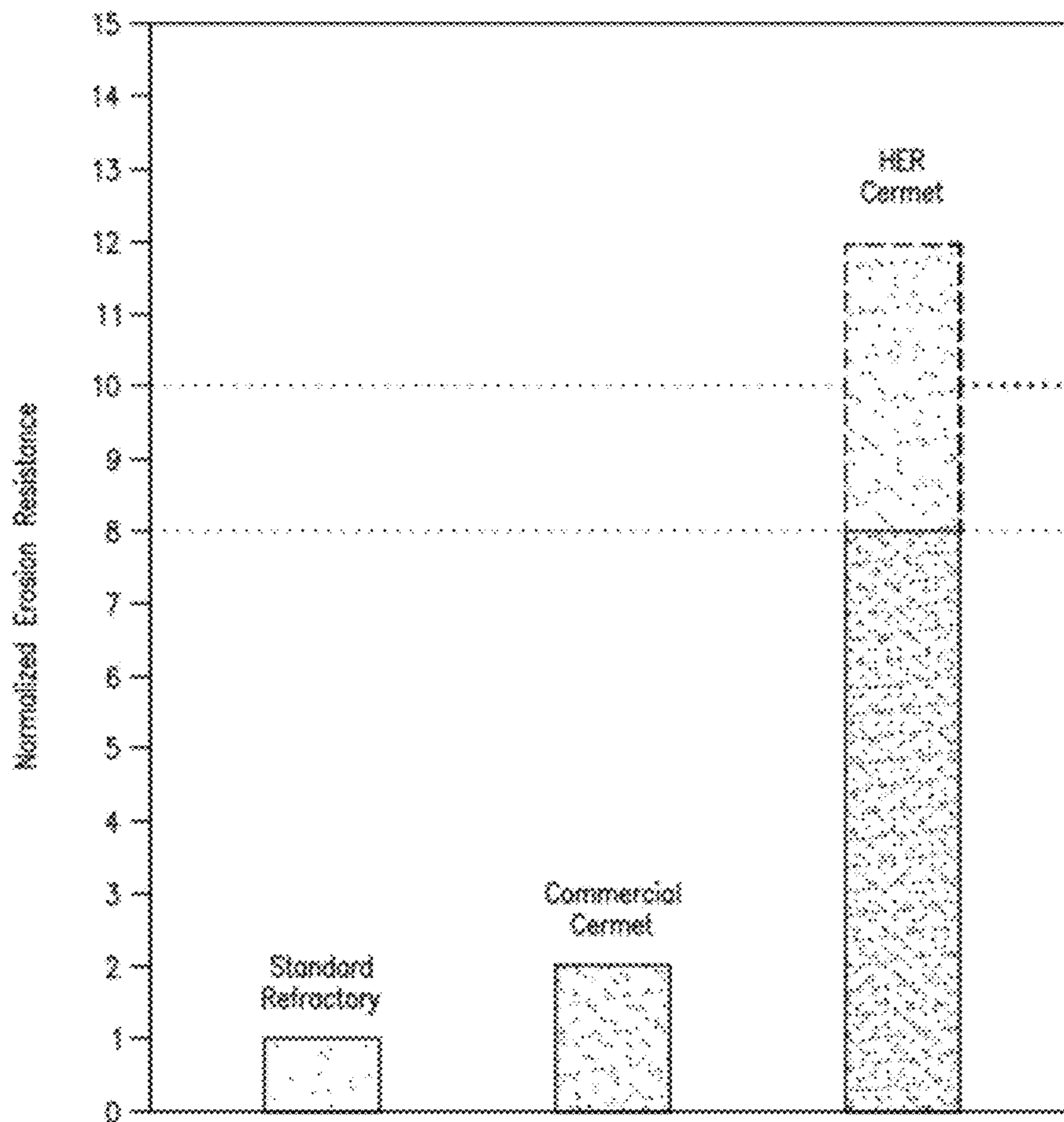
HEAT Erosion Index for Prior Art Materials and HER Cermet of the Present Invention
