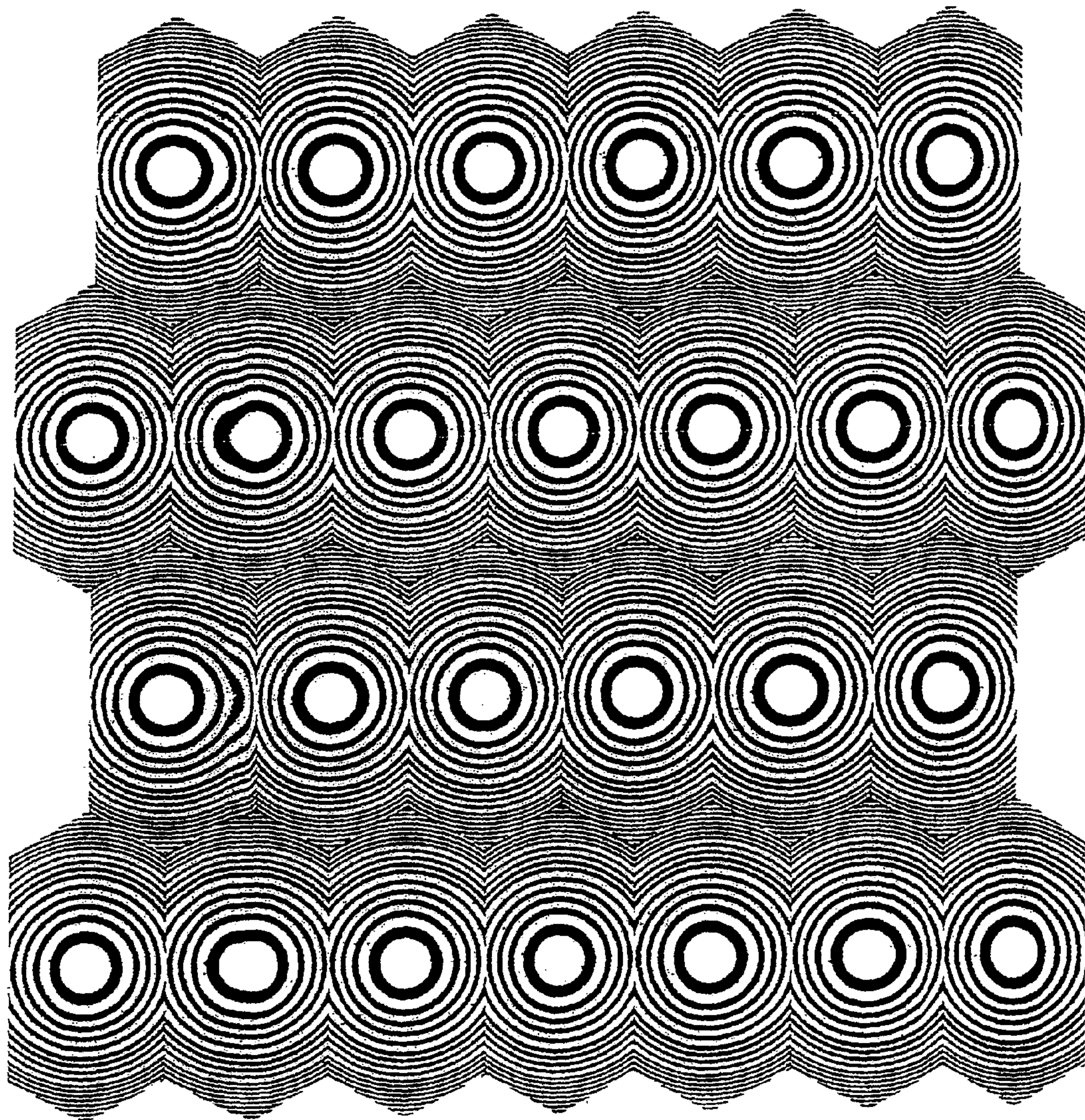
Diffraction Lens Arrays Arranged in Elongated Hexagonal Shapes
