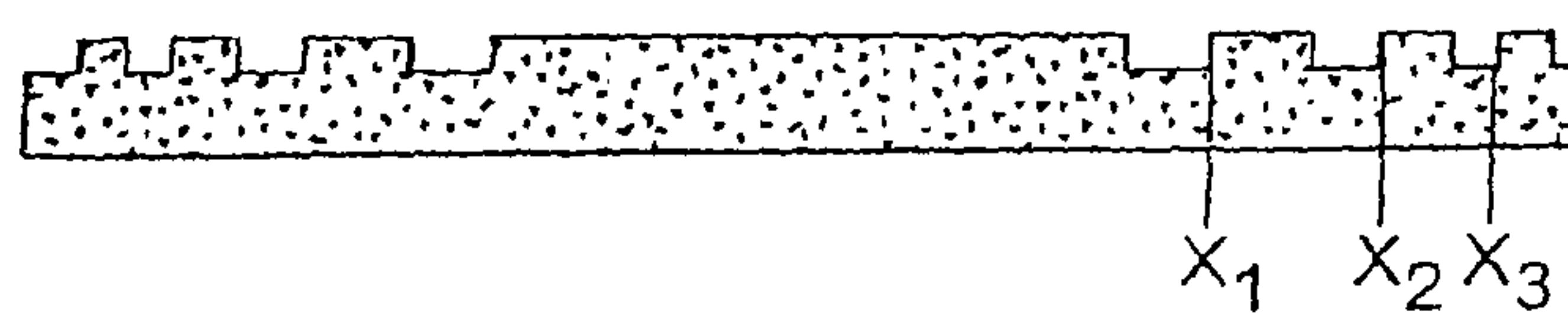
Diffractive Lens with Two Levels
