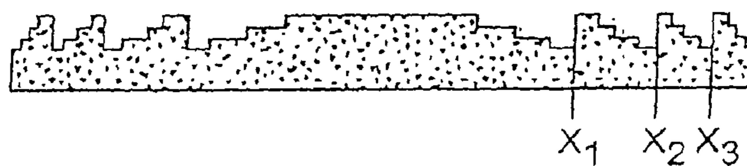
Diffractive Lens with Four Levels
