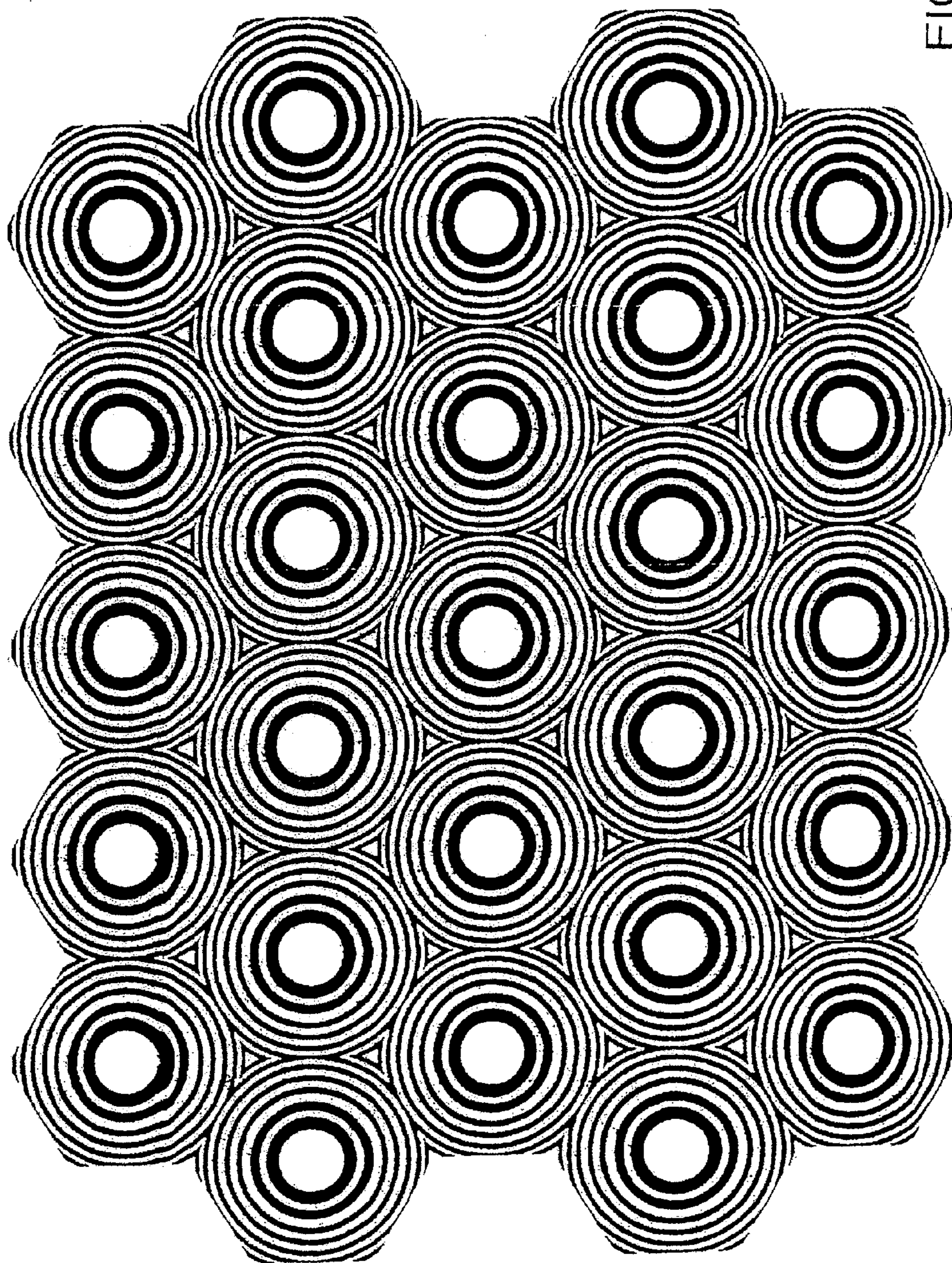
Diffraction Lens Arrays Arranged in Hexagonal Shapes
