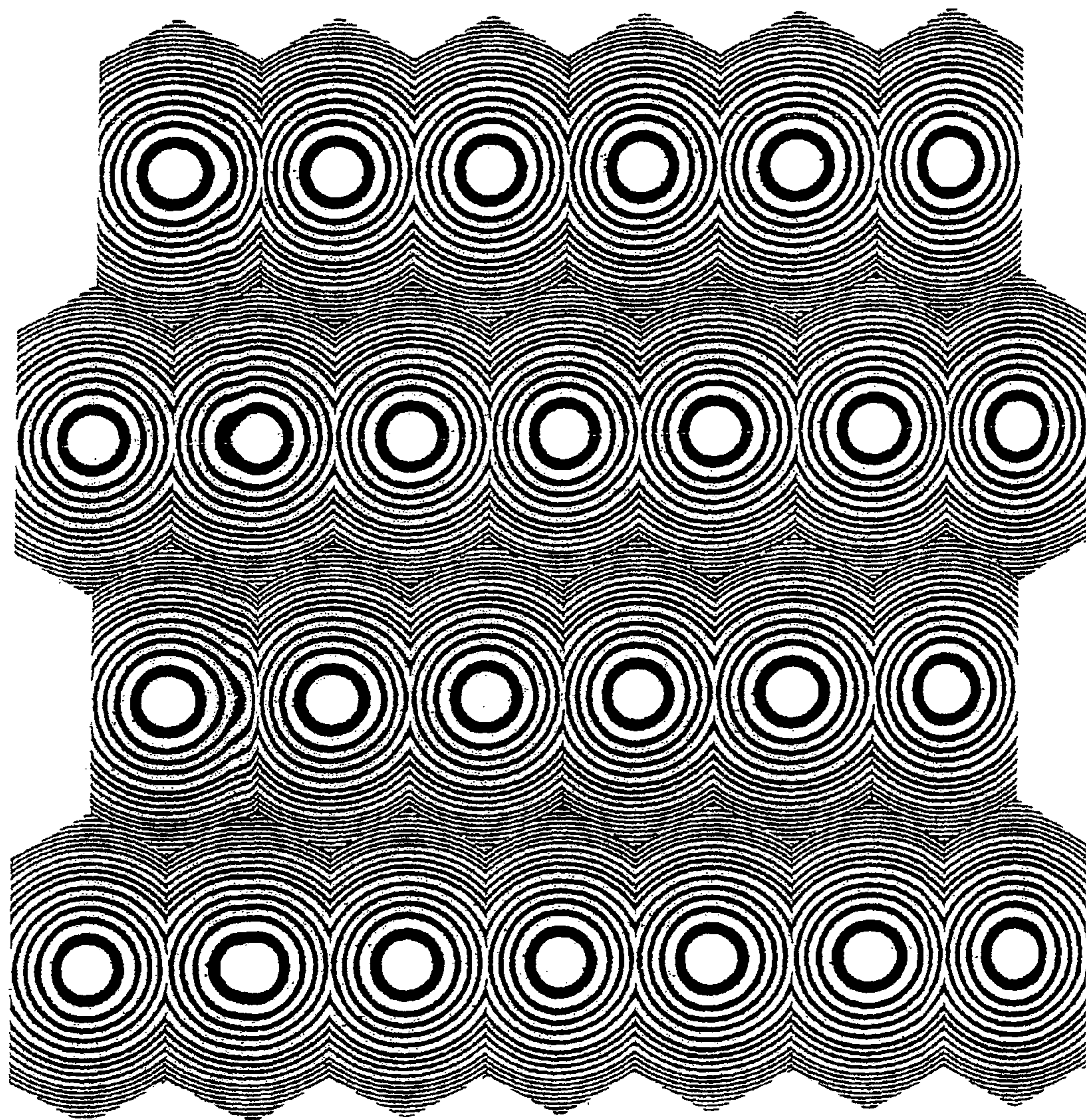
Diffractive Lens Arrays Arranged in Elongated Hexagonal Shapes
