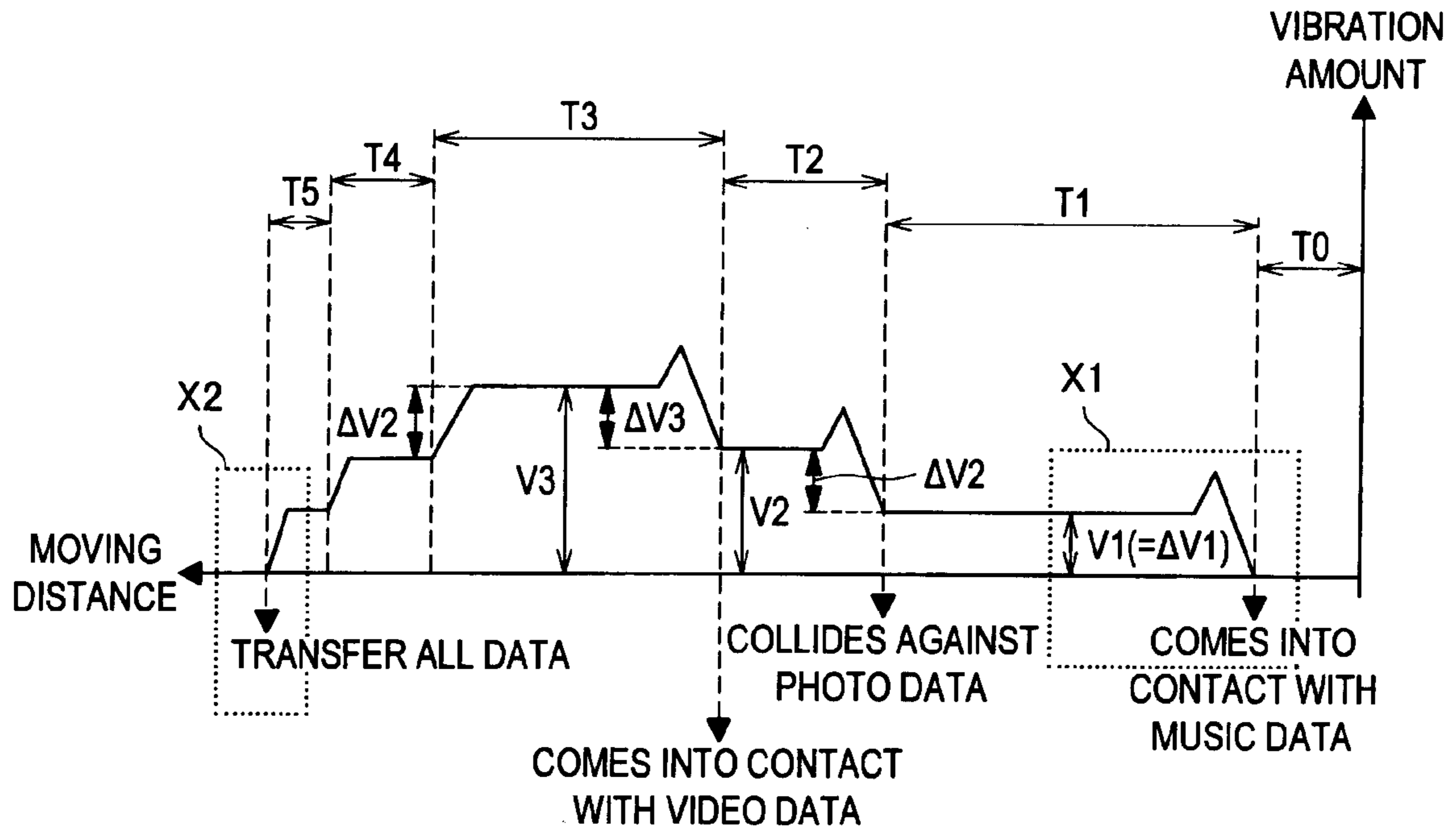
VIBRATION CONTROL EXAMPLE
