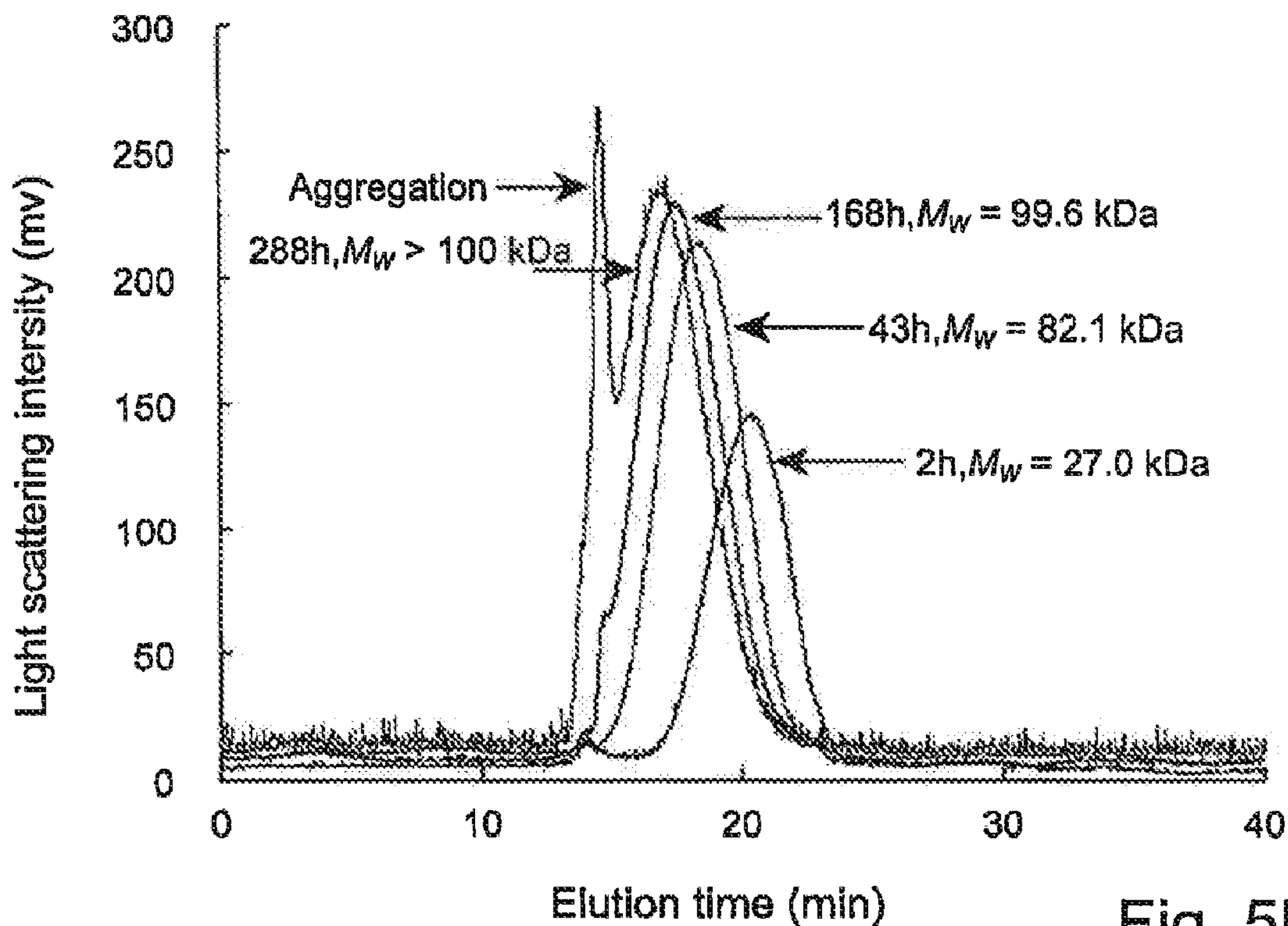
Polymerization control by adjusting polymerization time
