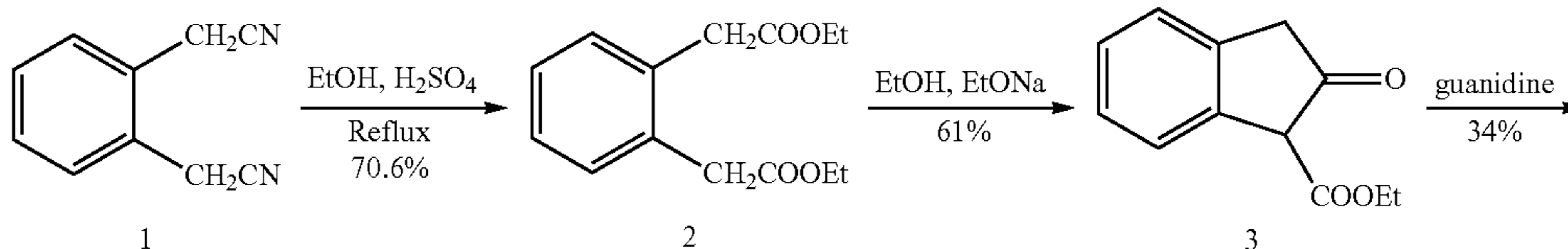
Scheme 3:
