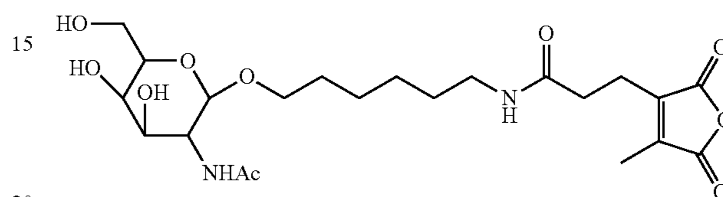
CDM-NAG with alkyl spacer
