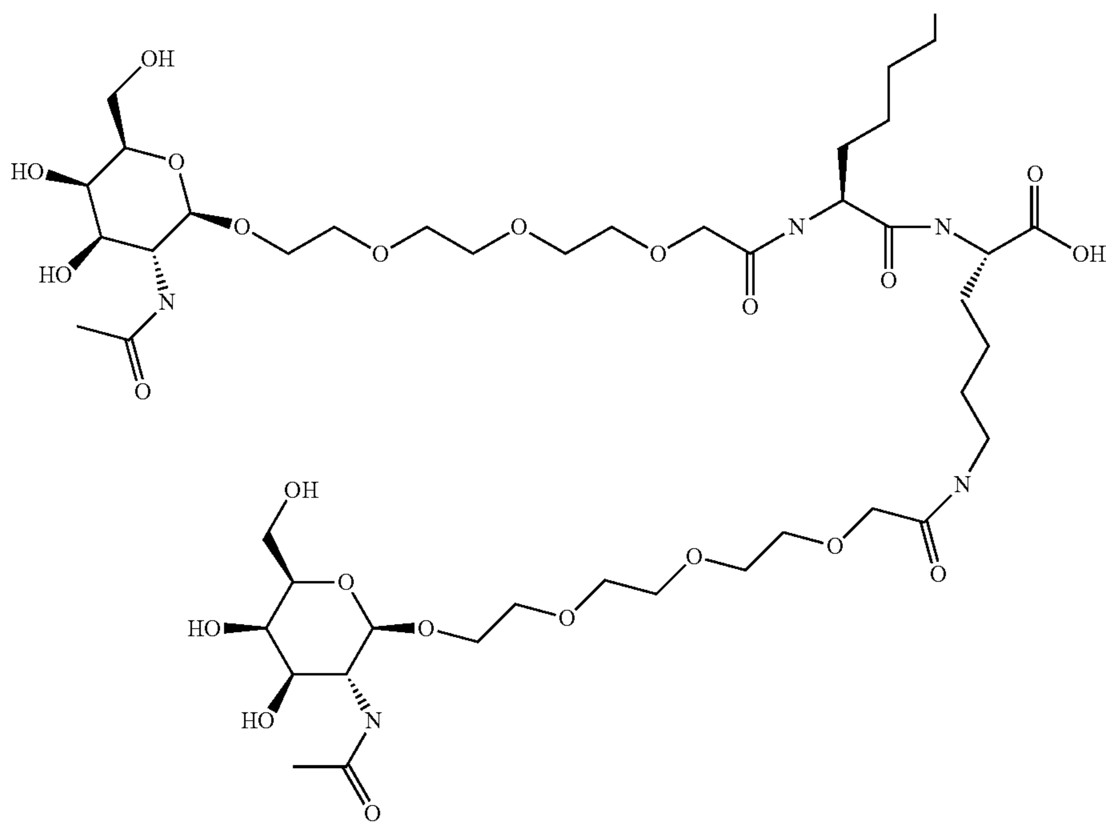
One embodiment of a Galactose cluster
