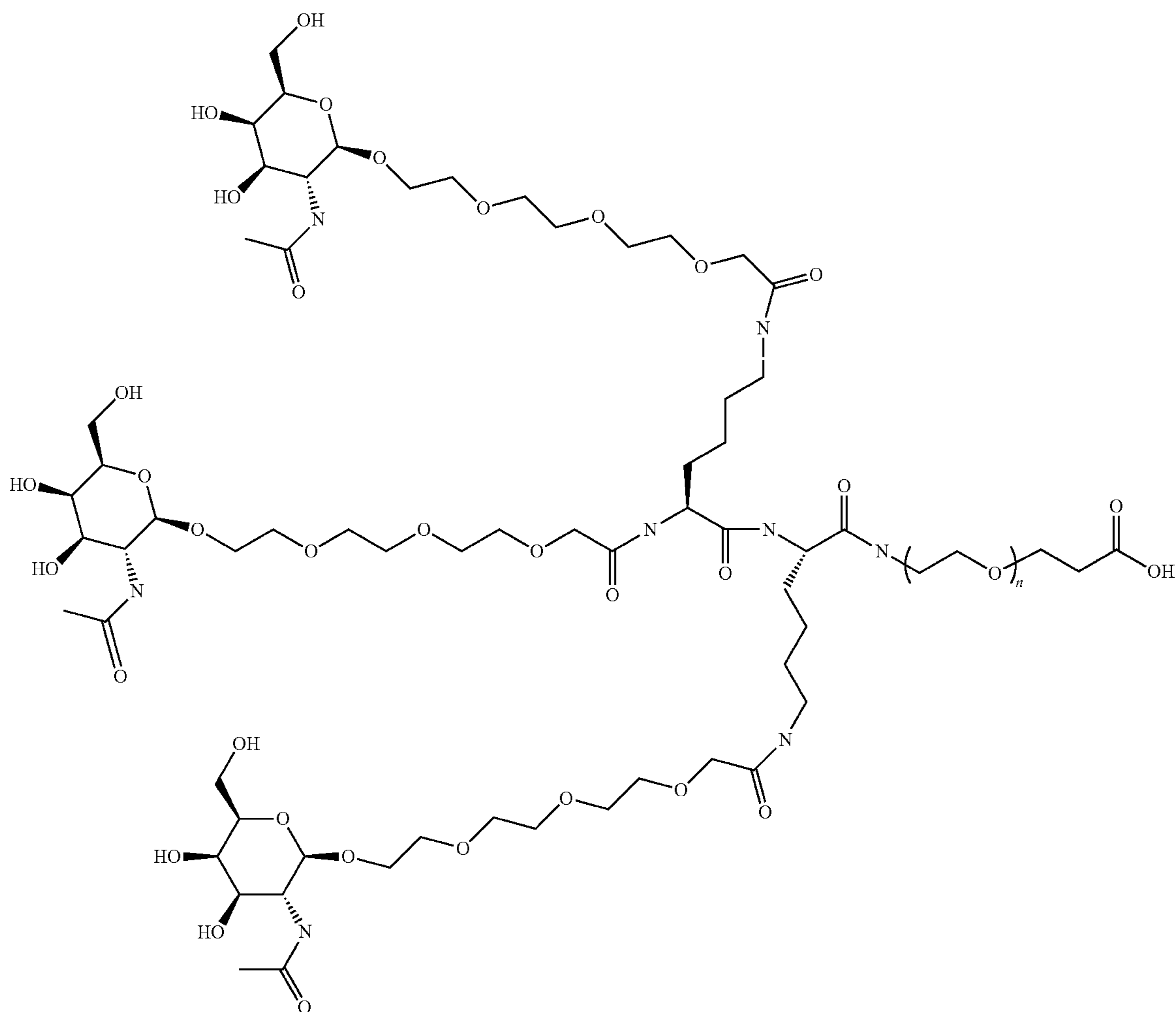
Galactose cluster with PEG spacer; targeting ligand attached to the siRNA through the carboxyl group.
