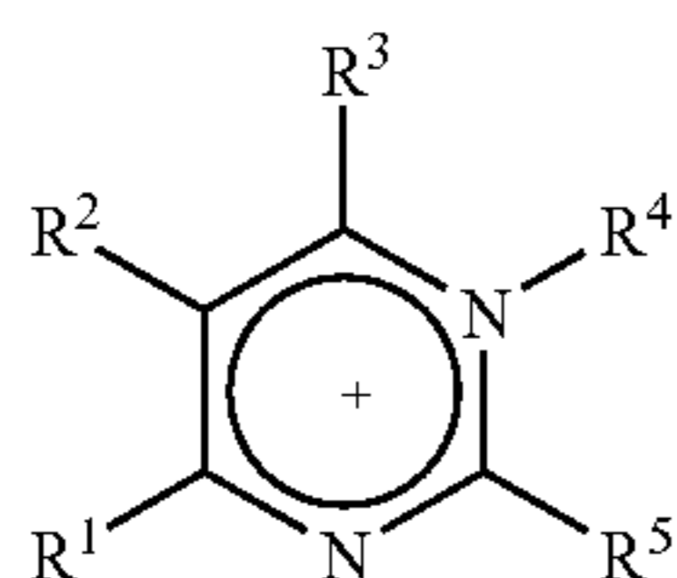
Pyrimidinium
