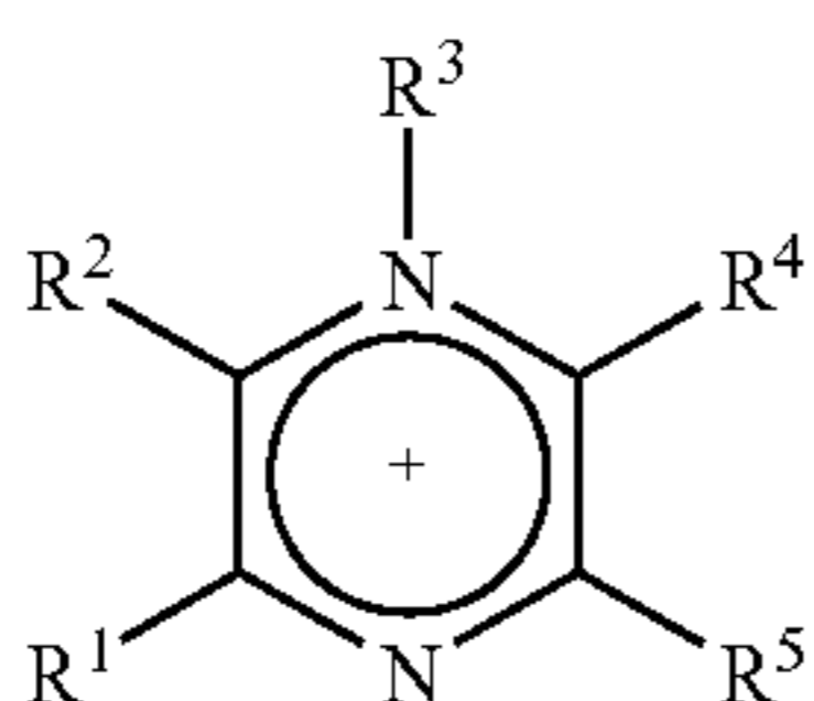
Pyrazinium
