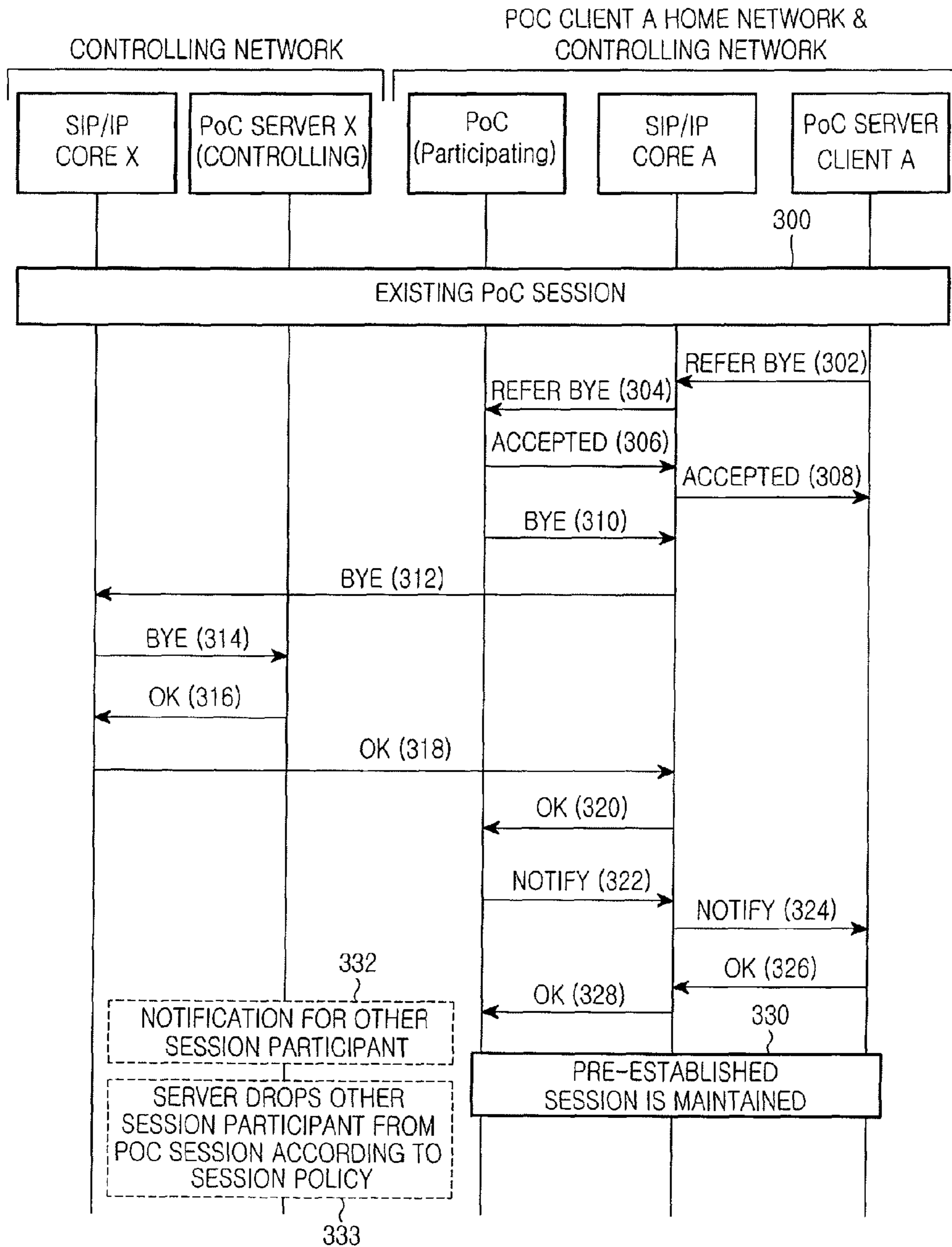
FIG.3 (CONVENTIONAL ART)
