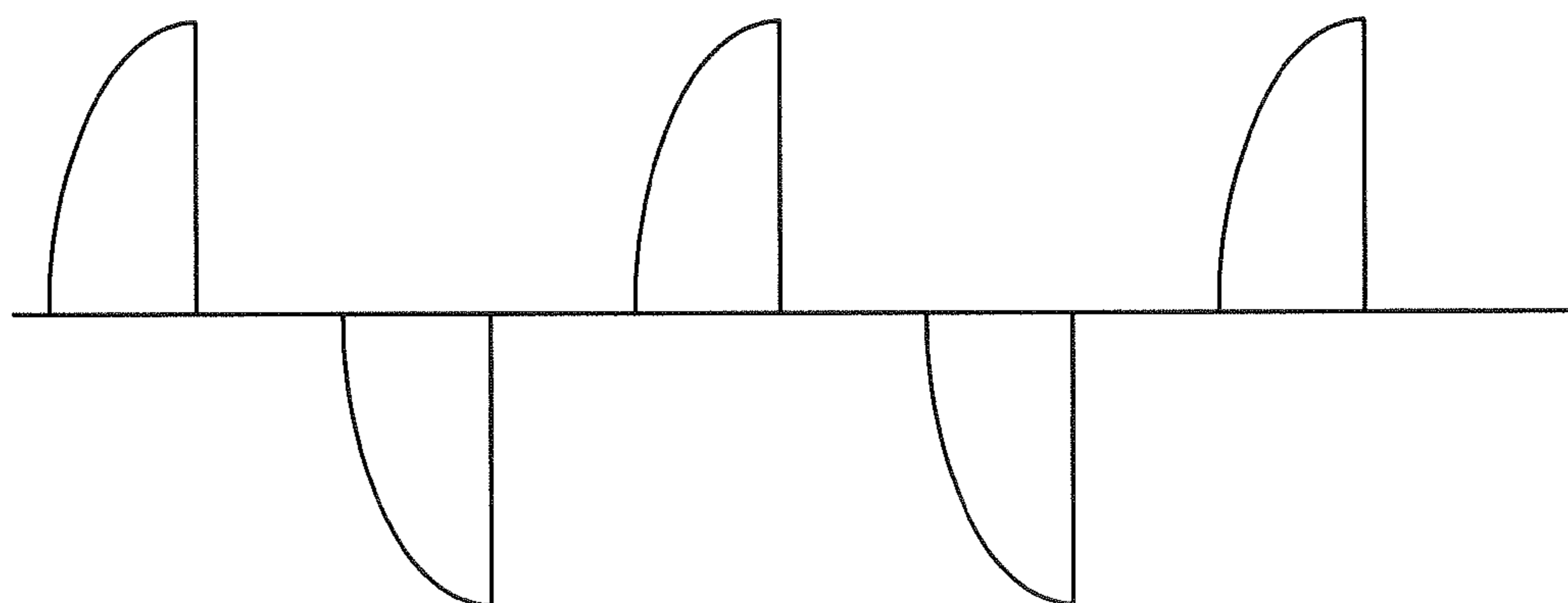
Trailing Edge Electronic Low Voltage Dimmer (~50%)
