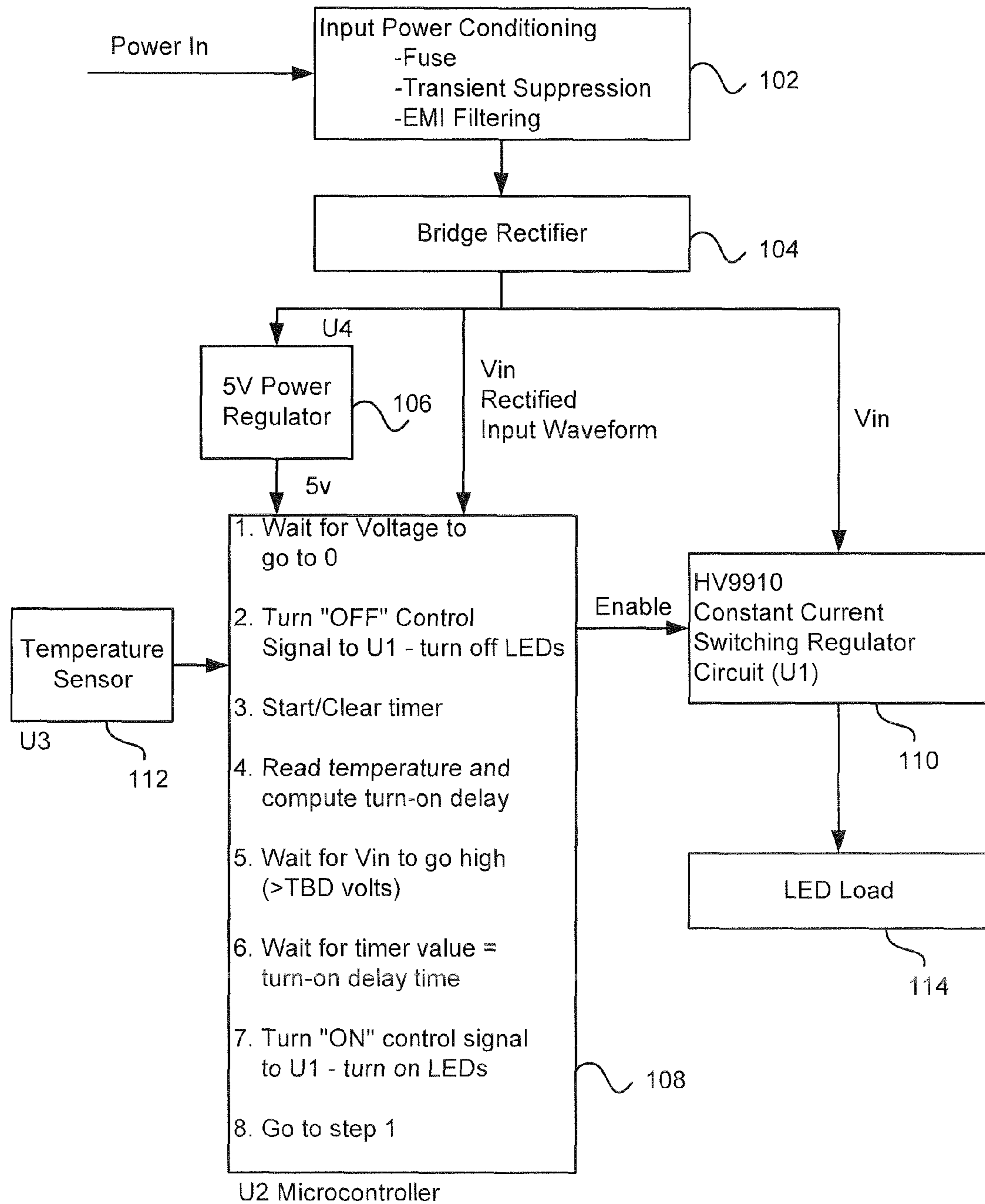
Functional Block Diagram
