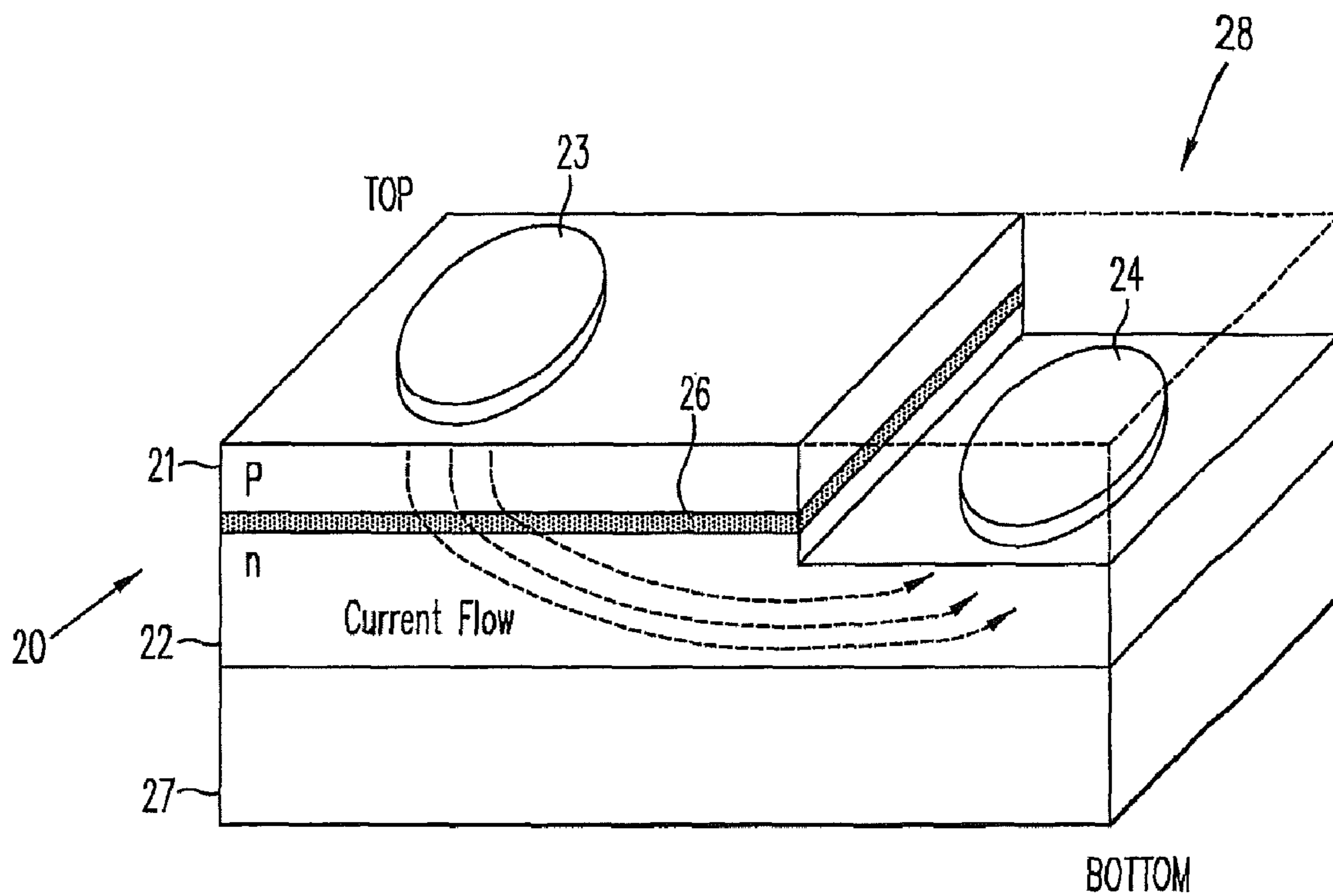
FIG. 2 (Prior Art)
