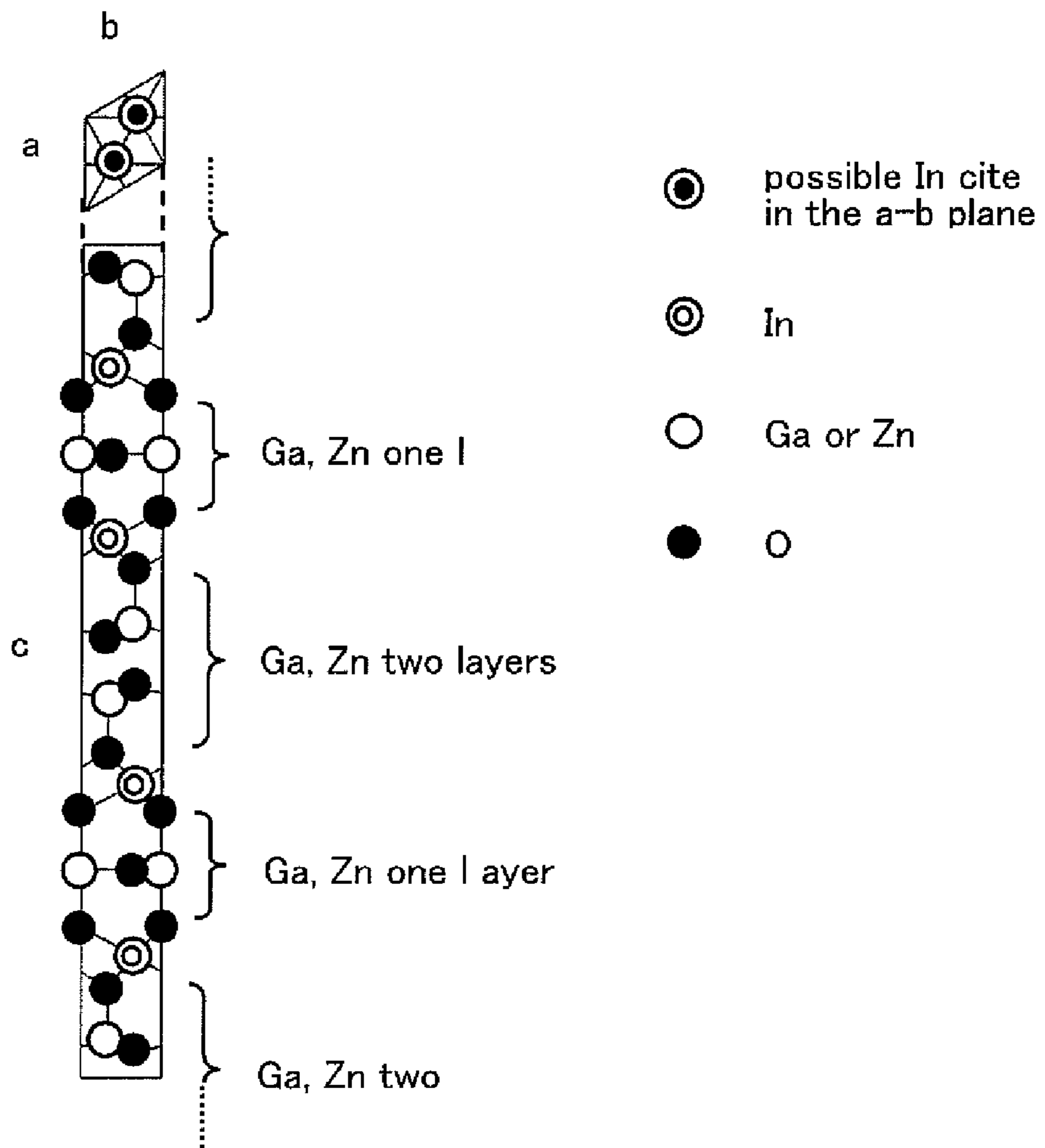
Crystal Structure of \text{In}_2\text{Ga}_2\text{ZnO}_7
