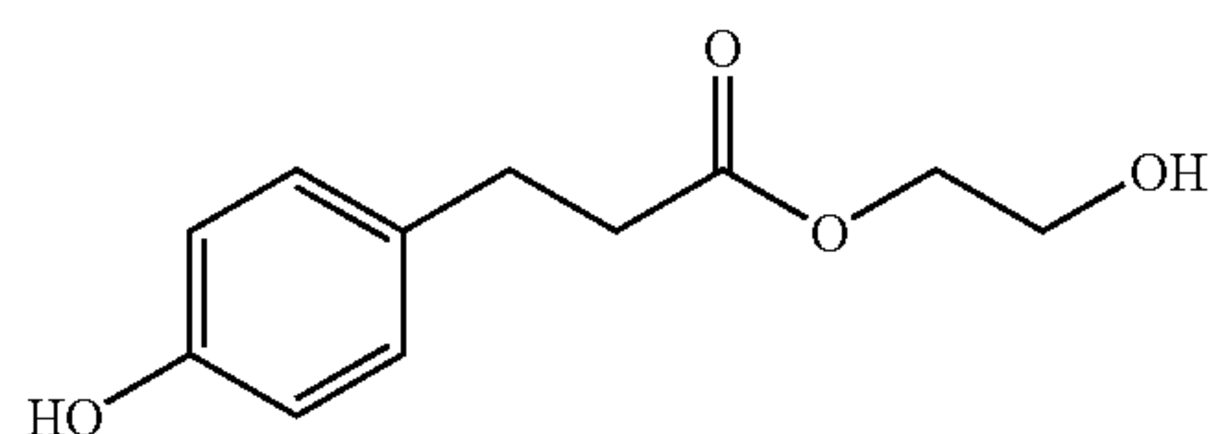
C_{11}H_{14}O_4 Mol. Wt.: 210.23
