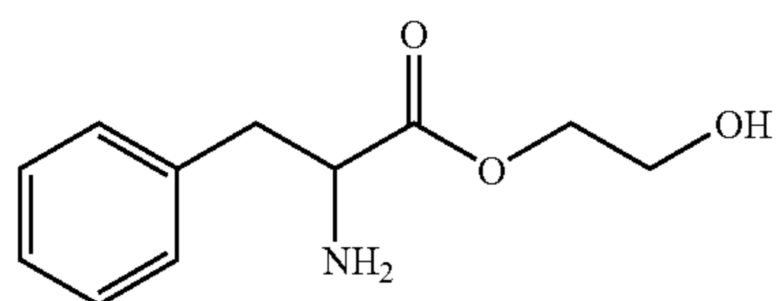
C_{11}H_{15}NO_3 Mol. Wt.: 209.24
