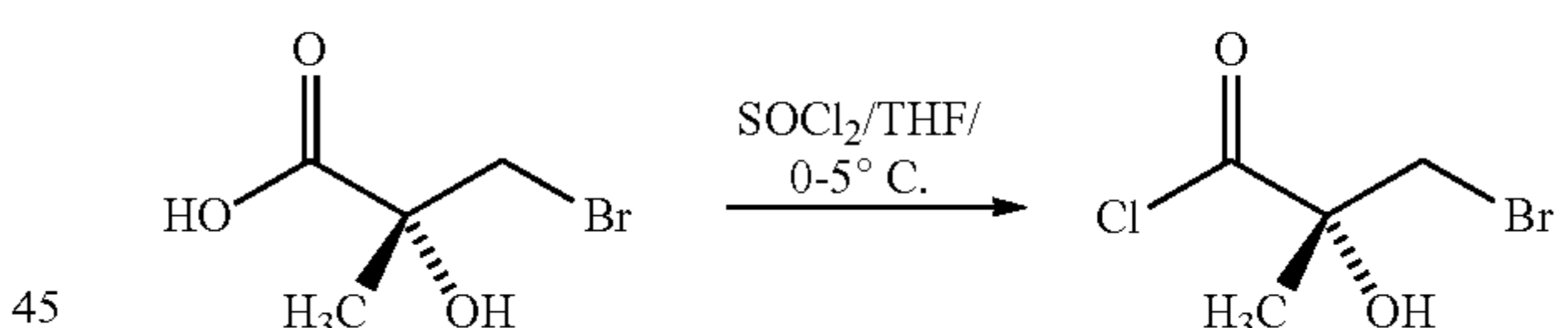
(R)-3-bromo-2-hydroxy-2-methylpropanoic acid R-18
