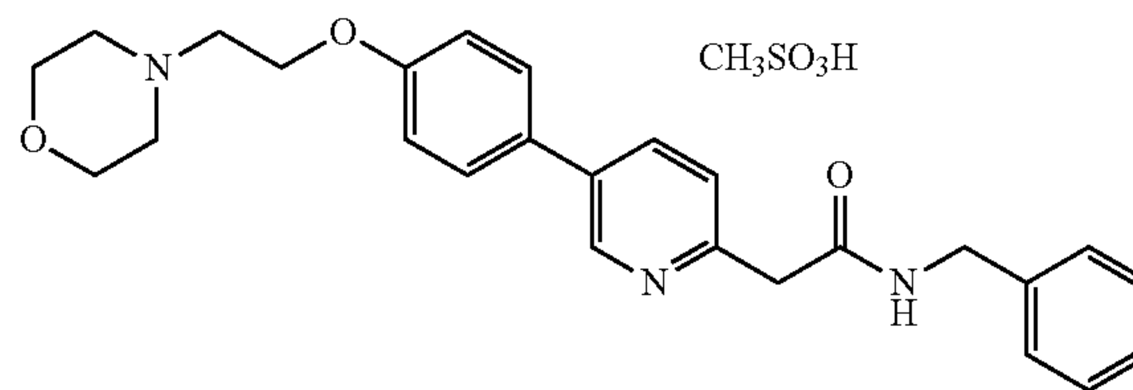
KX2-391 MSA
