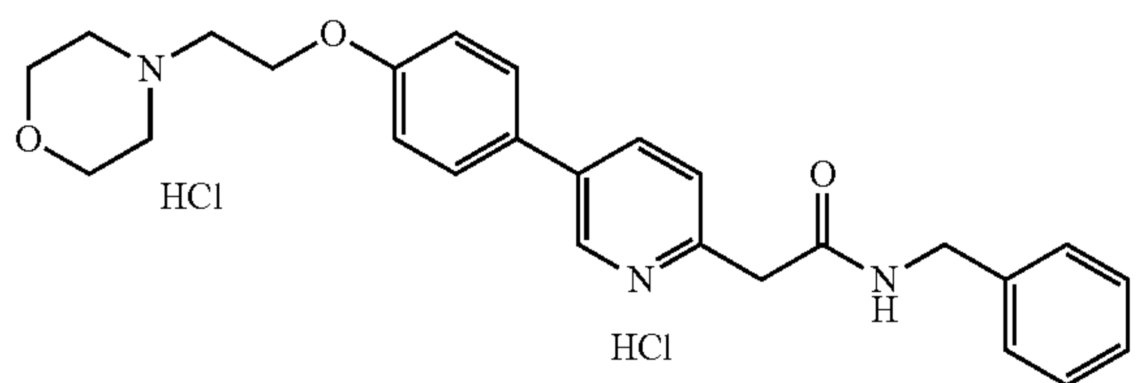
KX2-391 2HCl
