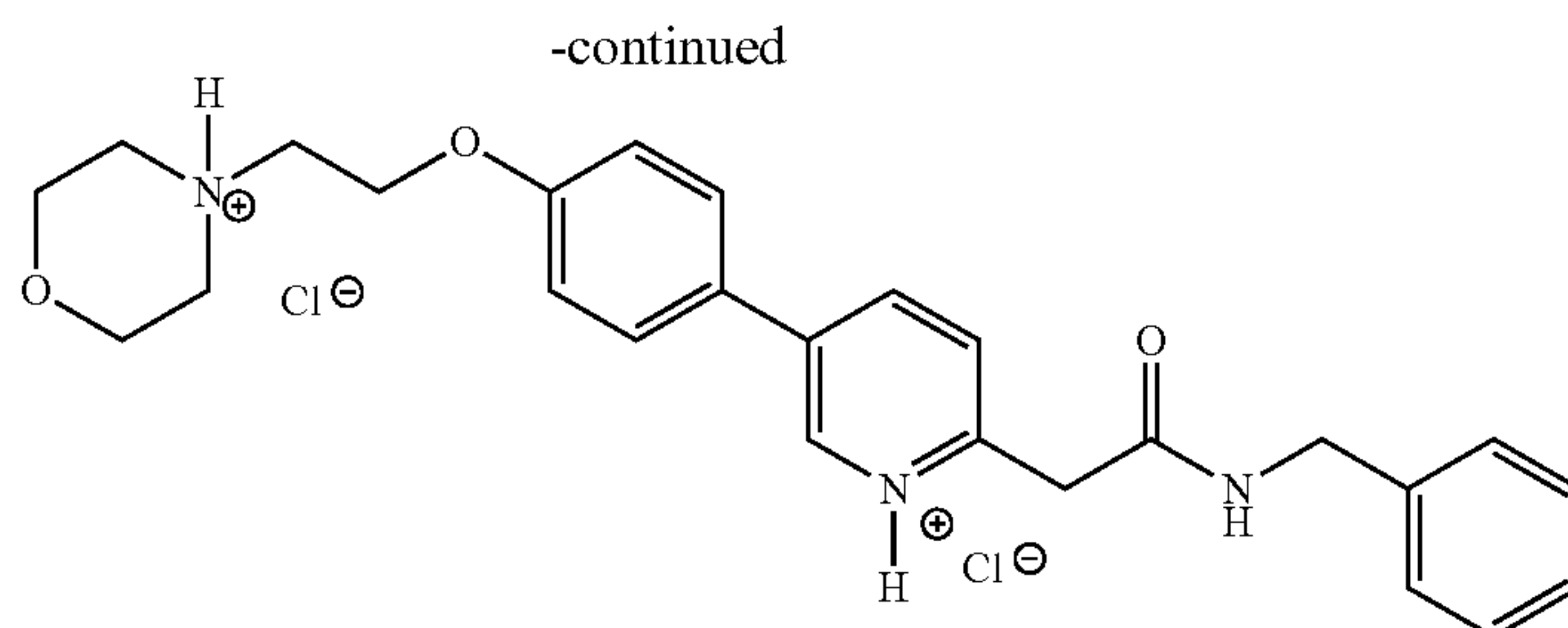
KX2-391 (diHCl salt)
