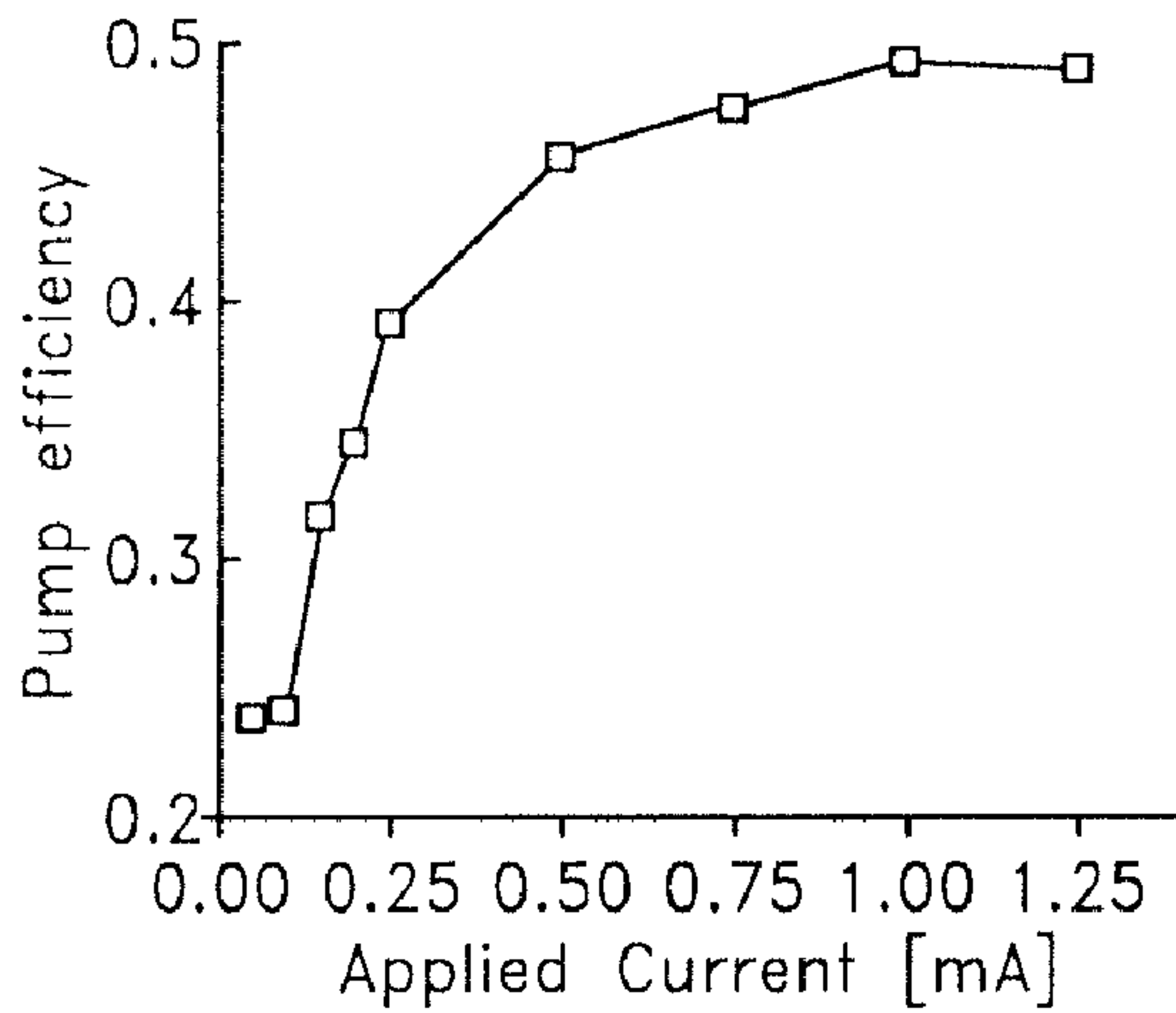
Pump efficiency FIG. 21C
