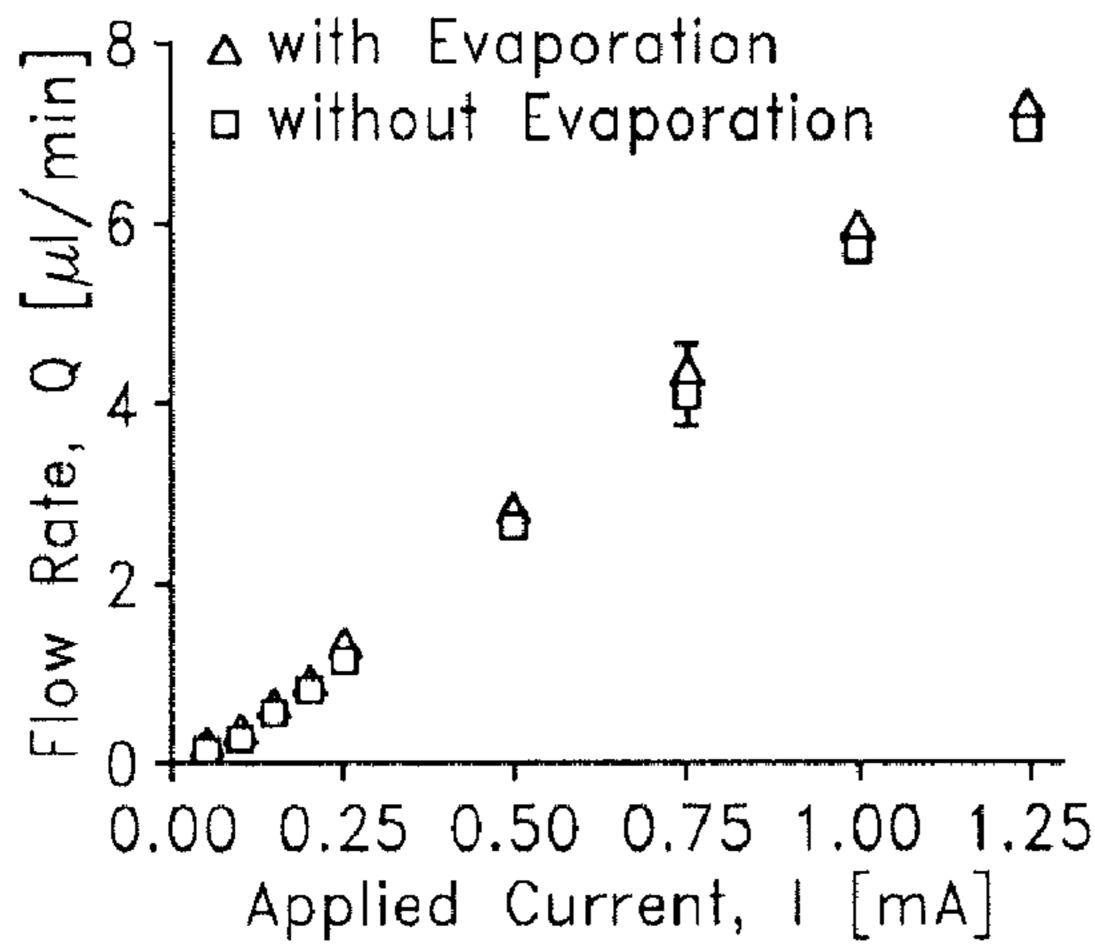
Flow rate testing
