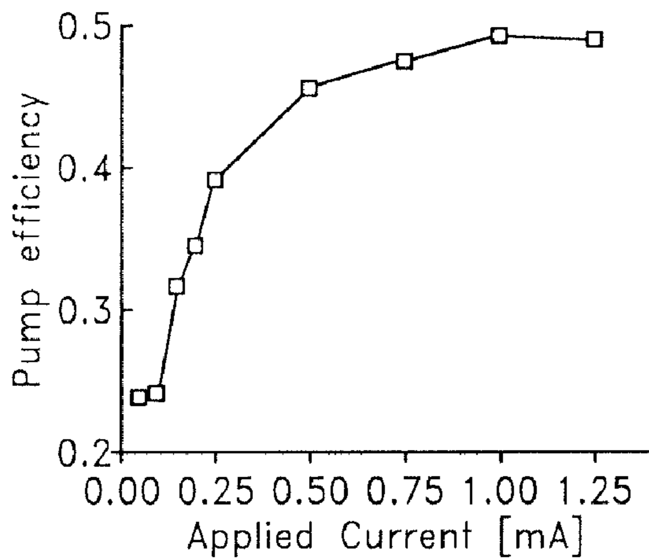
Pump efficiency
