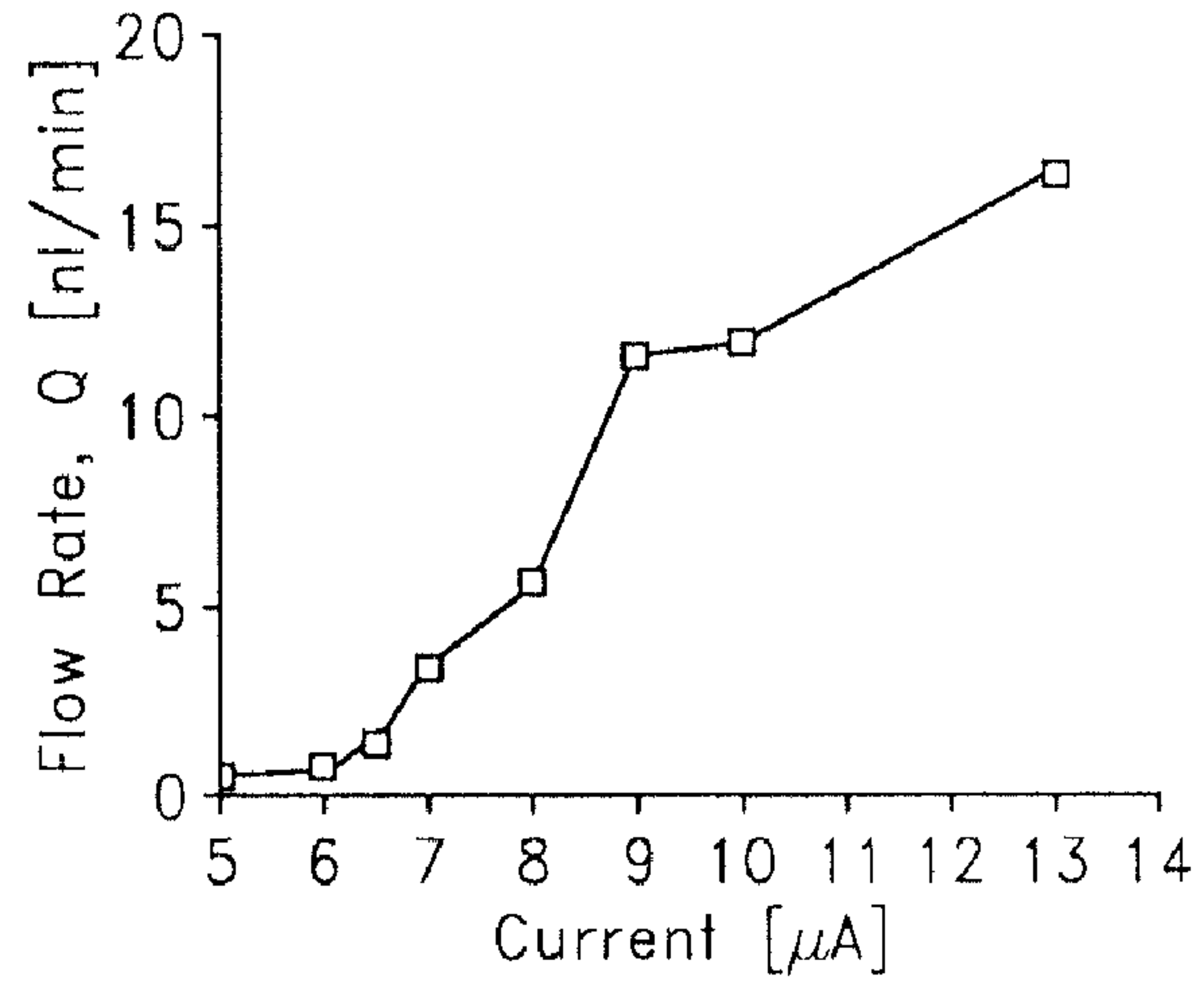
Ultra low flow rate FIG. 21B
