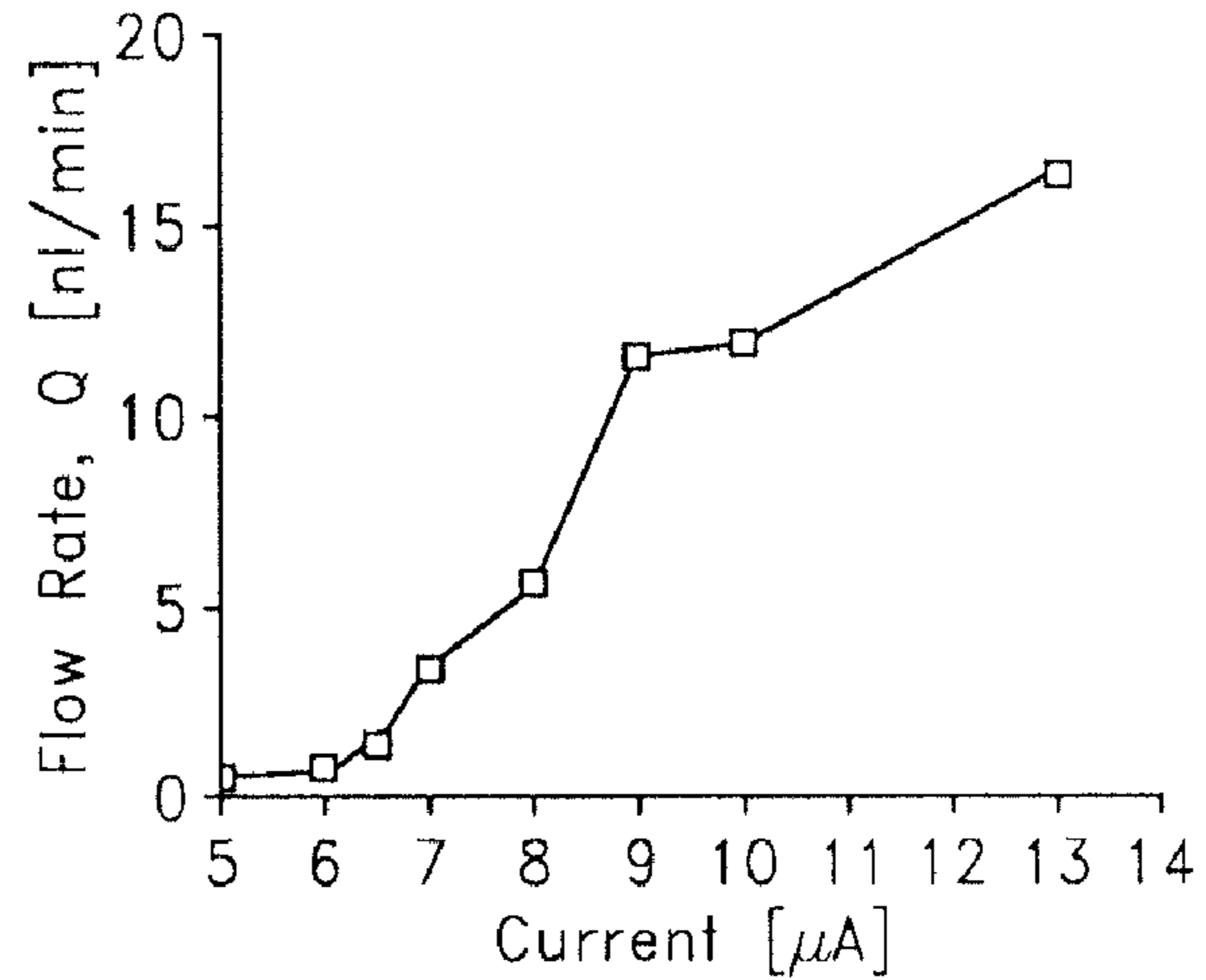
Ultra low flow rate
