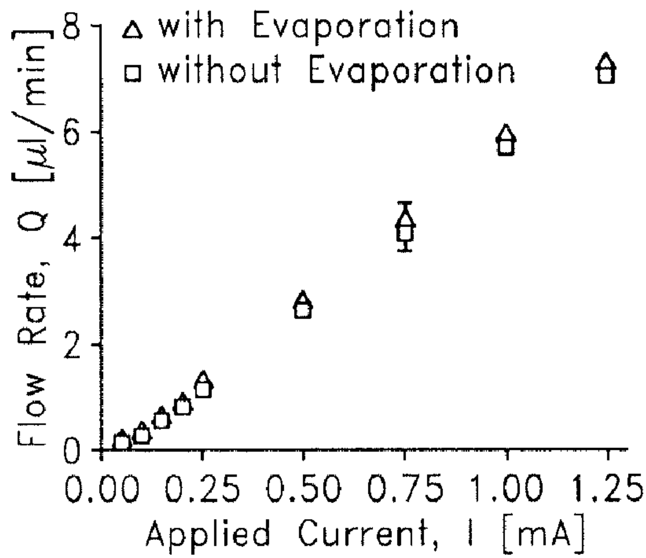
Flow rate testing FIG. 21A
