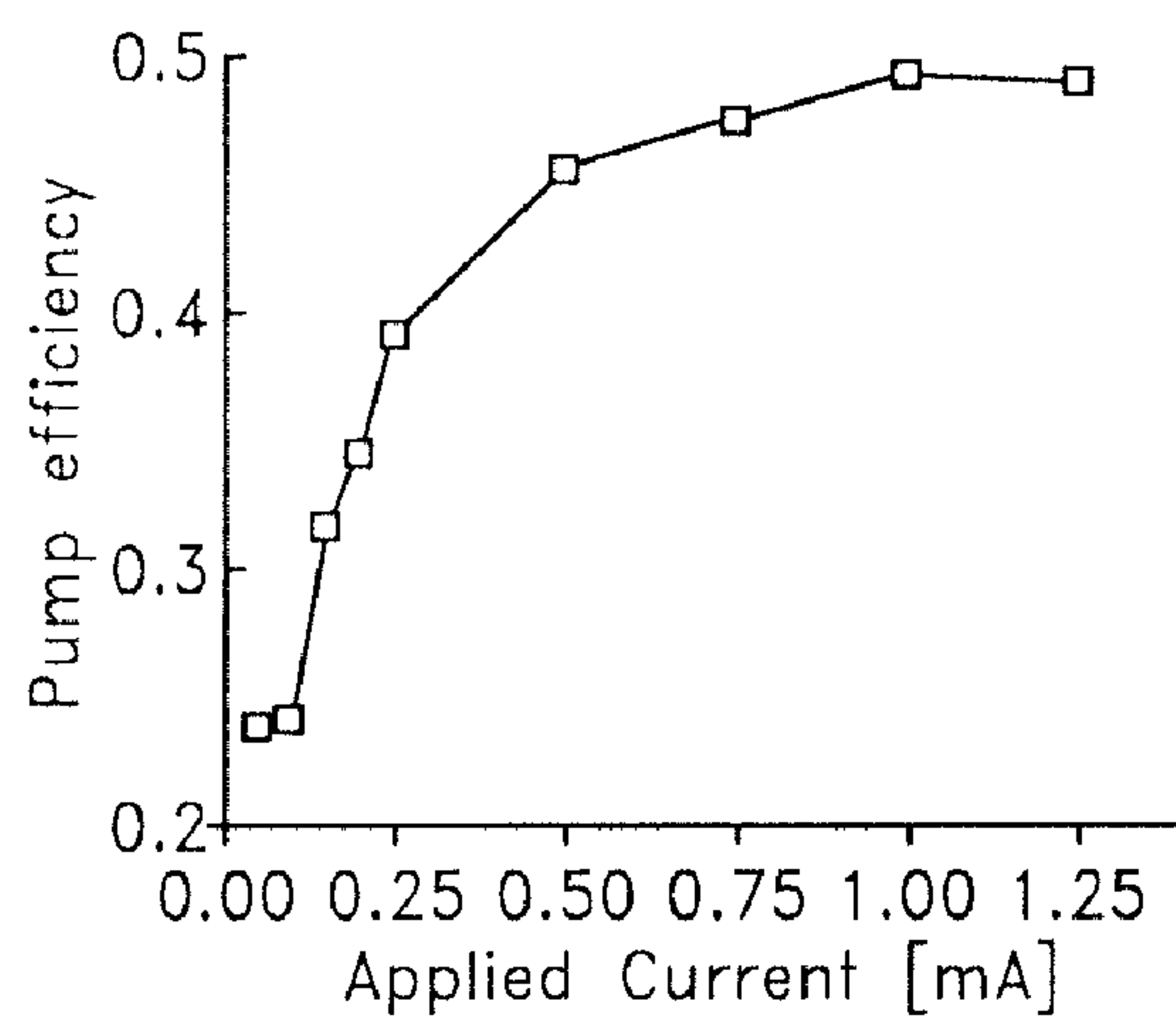
Pump efficiency
