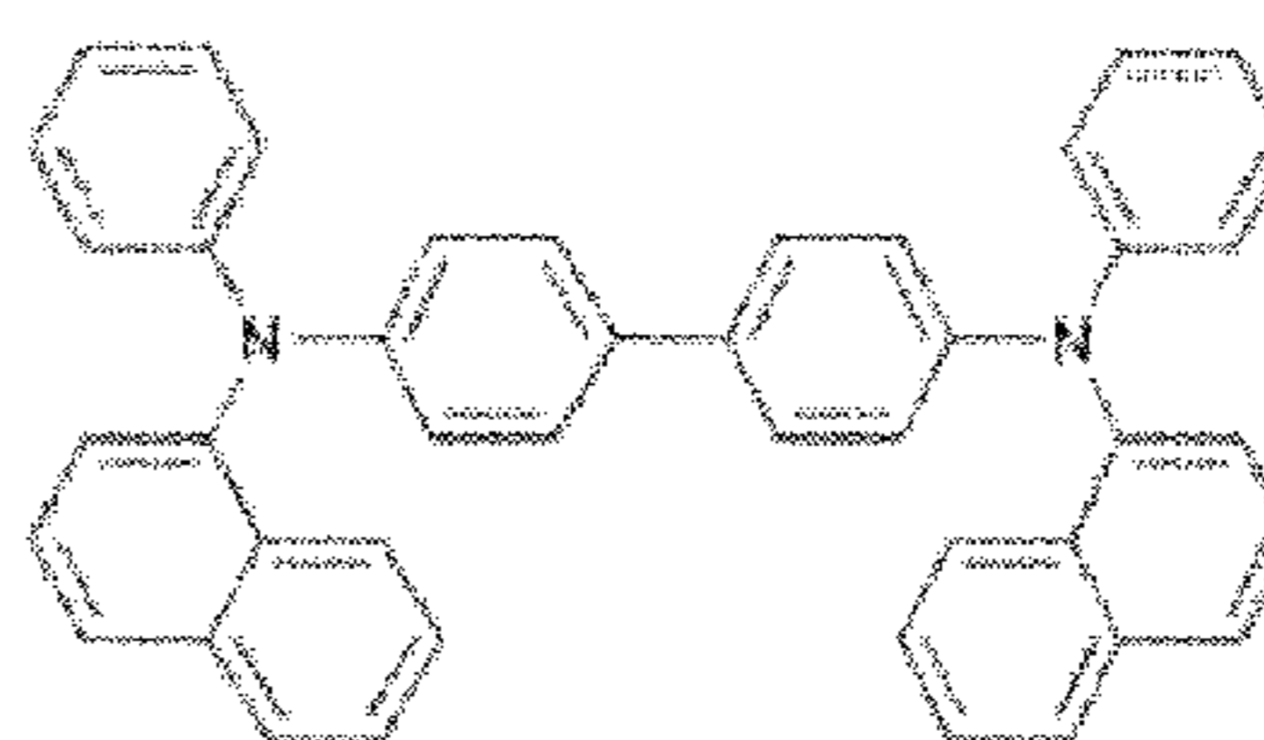
4-4'-bis[N-(1-naphthyl)-N-phenyl-amino]biphenyl (NPD)
