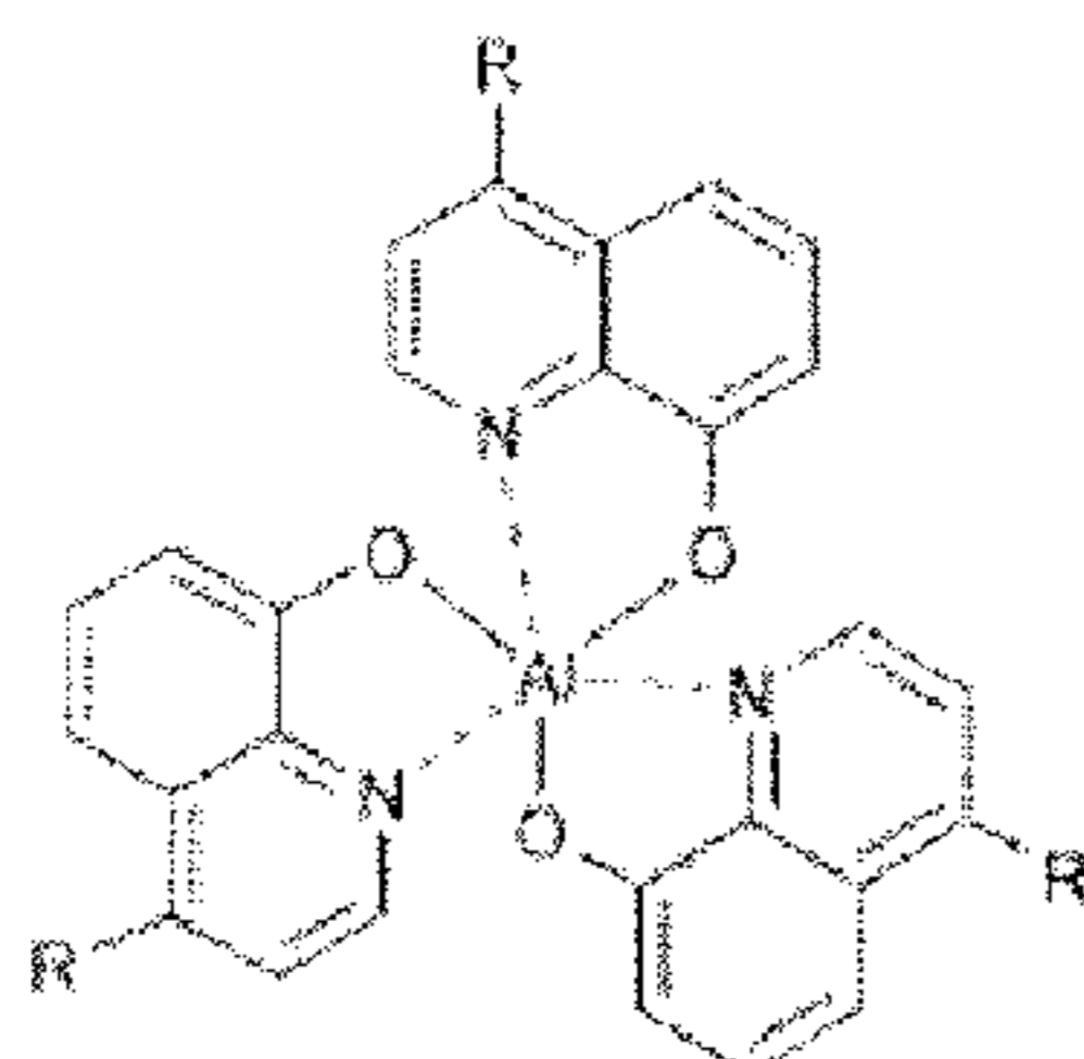
tris-(8-hydroxyquinoline) aluminum (Alq3)
