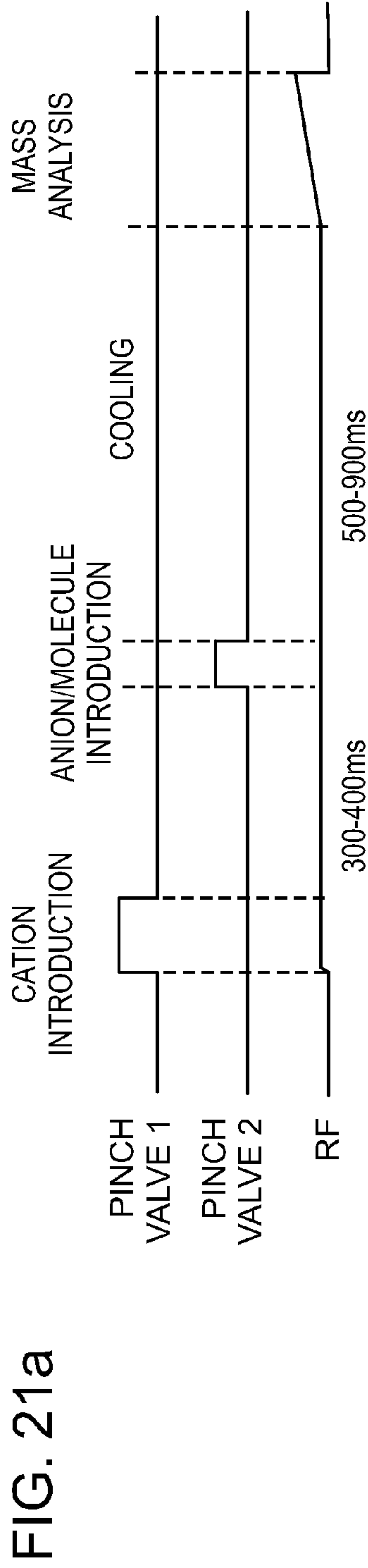
FIG. 21a Angiotensin 1 cation with azobenzene molecule
