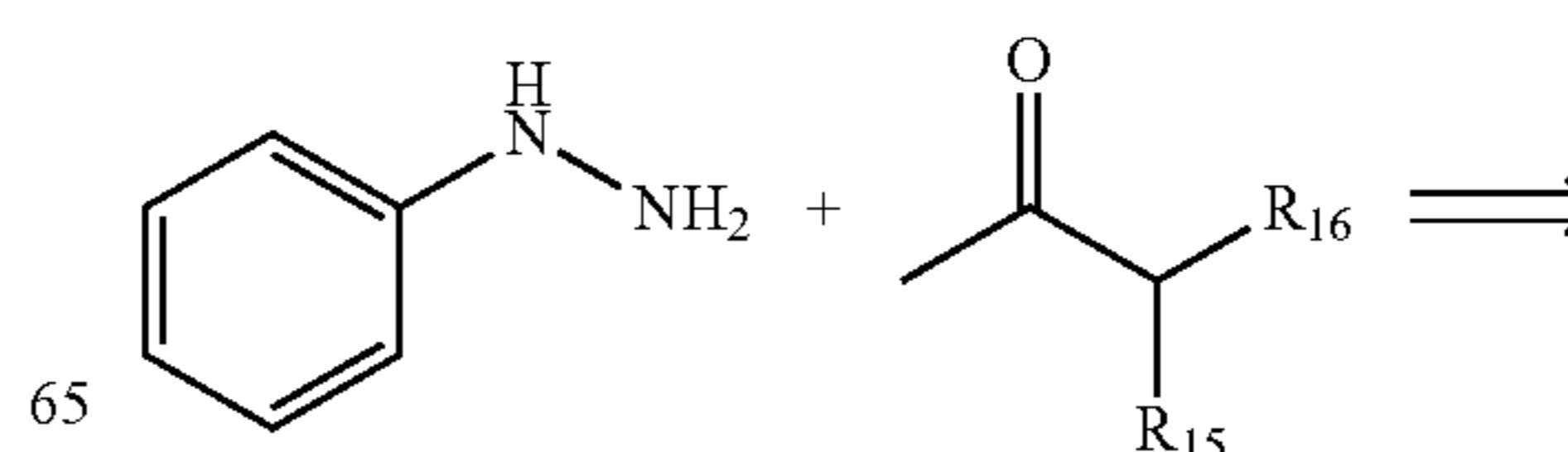
Scheme 3. Typical synthesis of indolium intermediate
