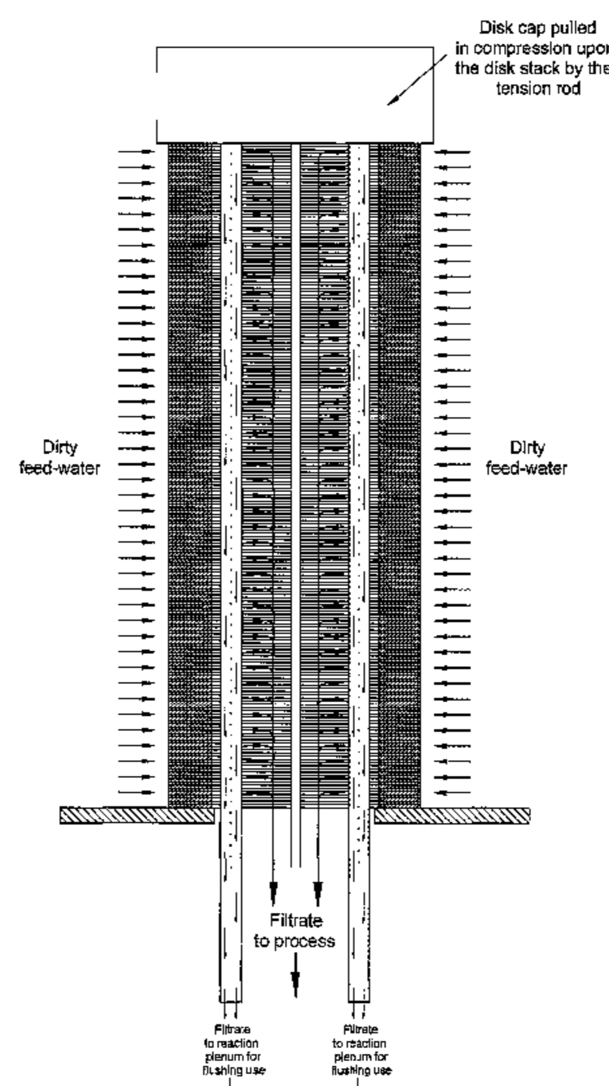
Stacked Disks in Filtration Mode
