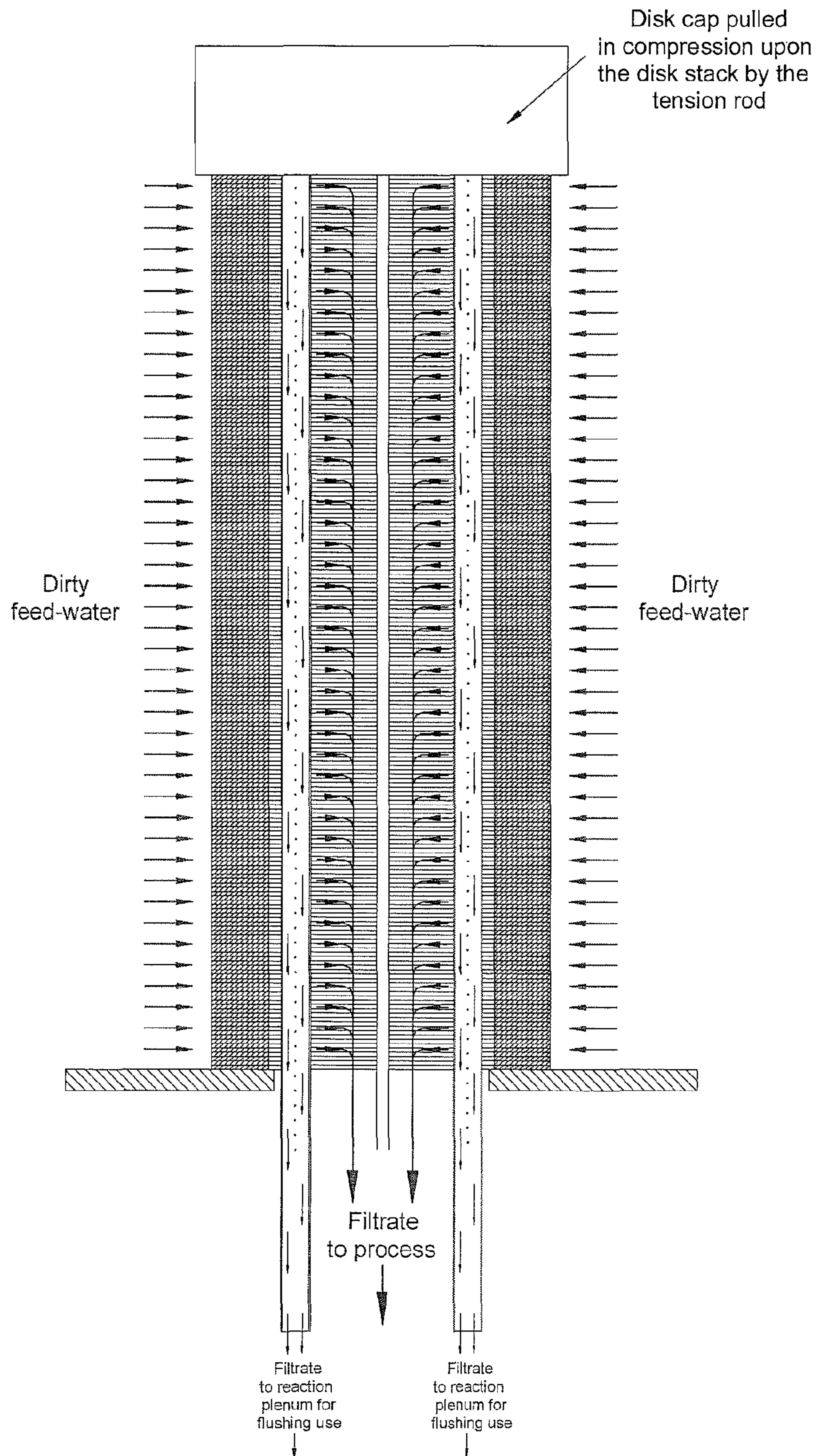
Figure 6 Stacked Disks in Filtration Mode
