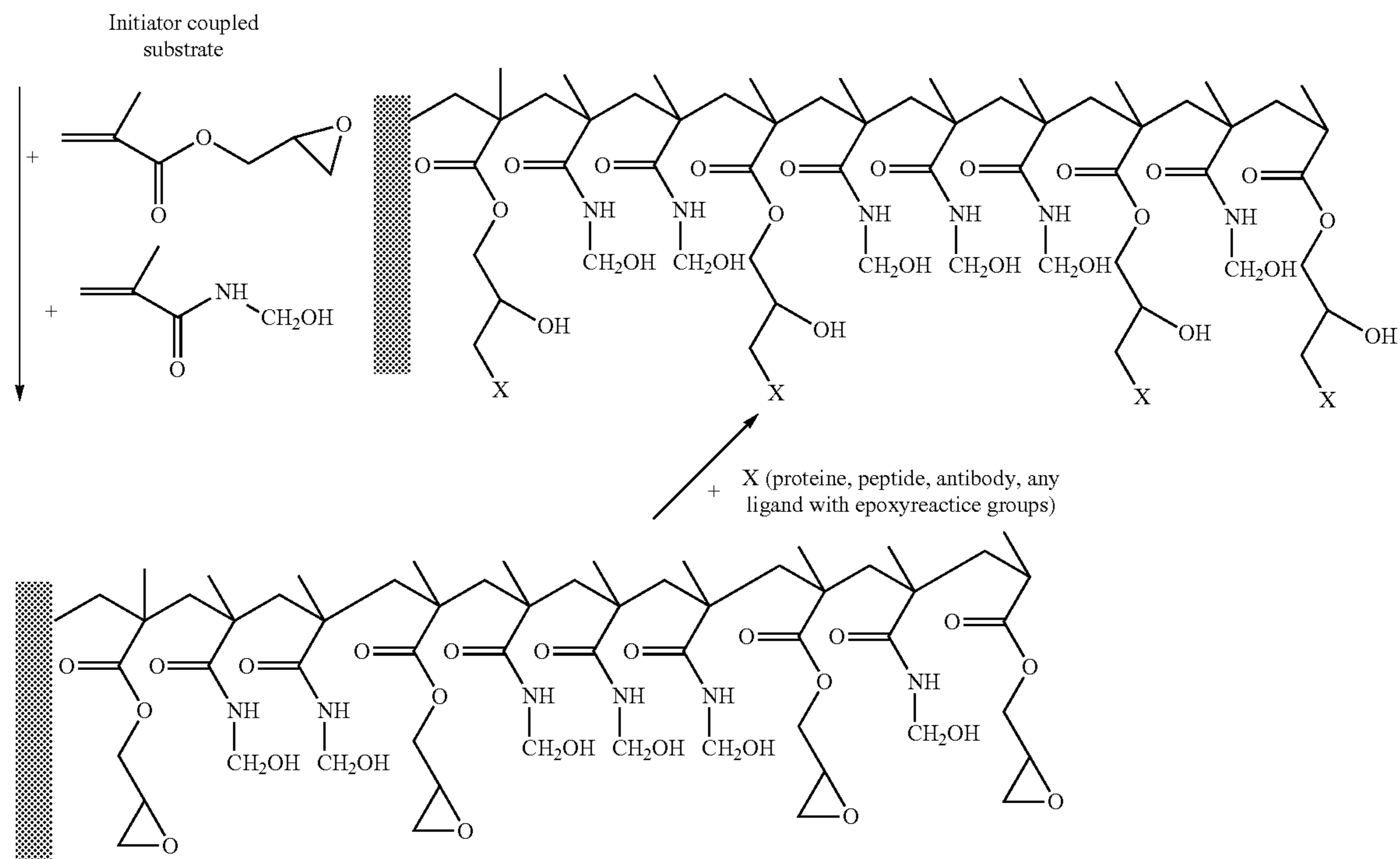
Reaction scheme 3
