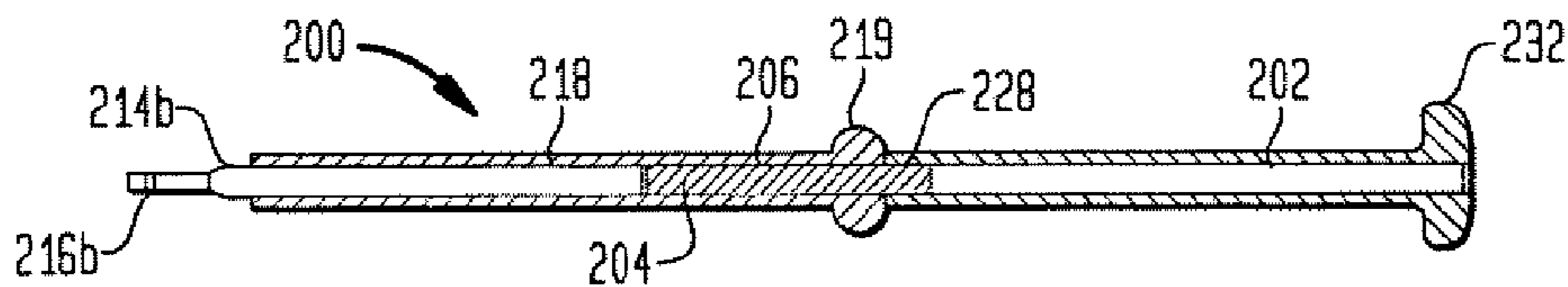
FIG. 31 (SECTION A-A OF FIG. 22)
