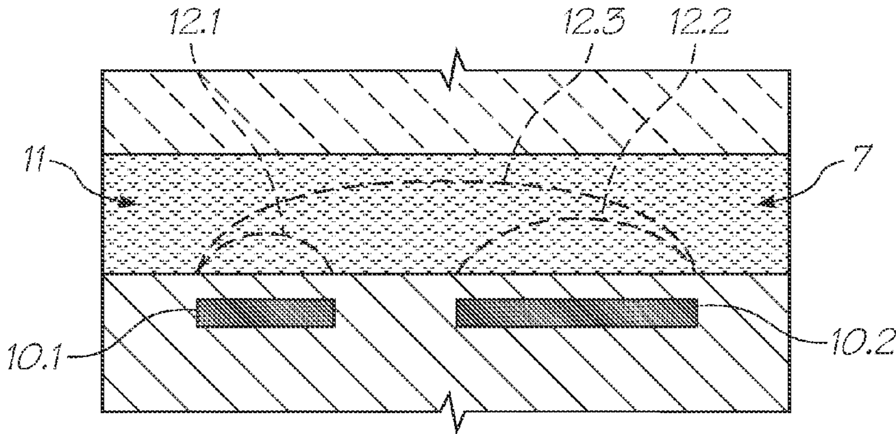
FIG. 52 (PRIOR ART)
