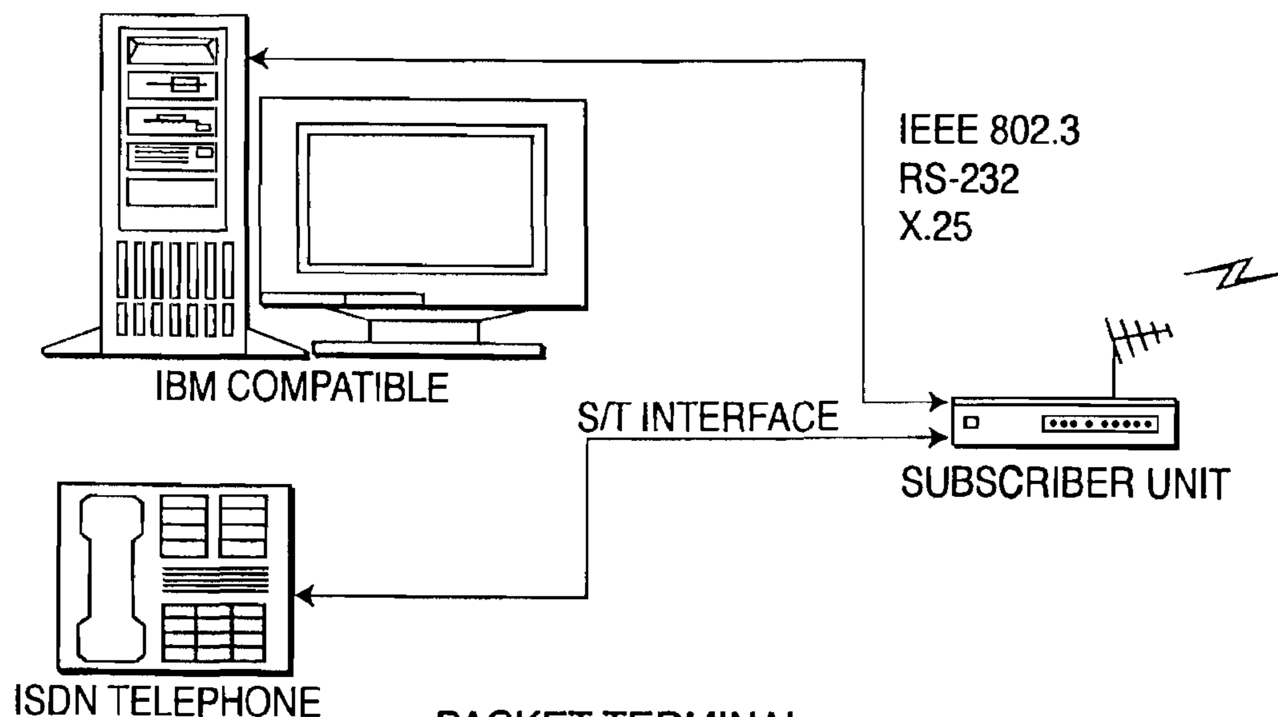
PACKET TERMINAL
