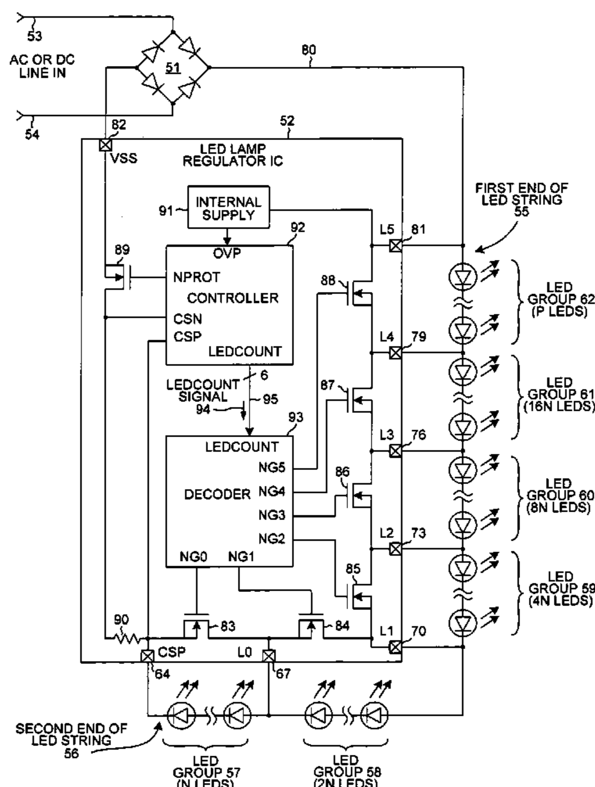
LED LAMP
