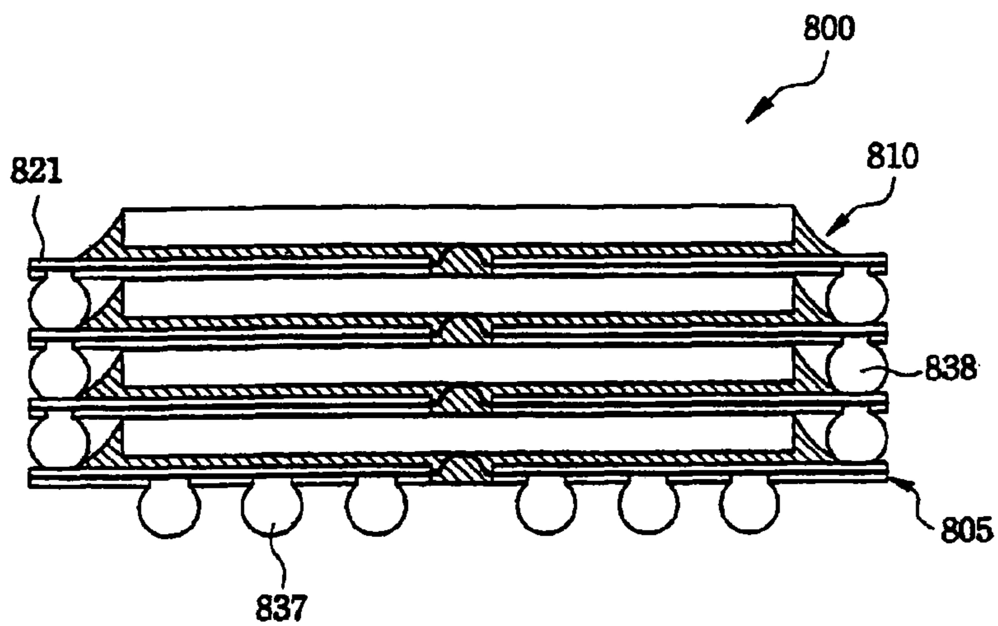
FIG. 3 (Prior Art)
