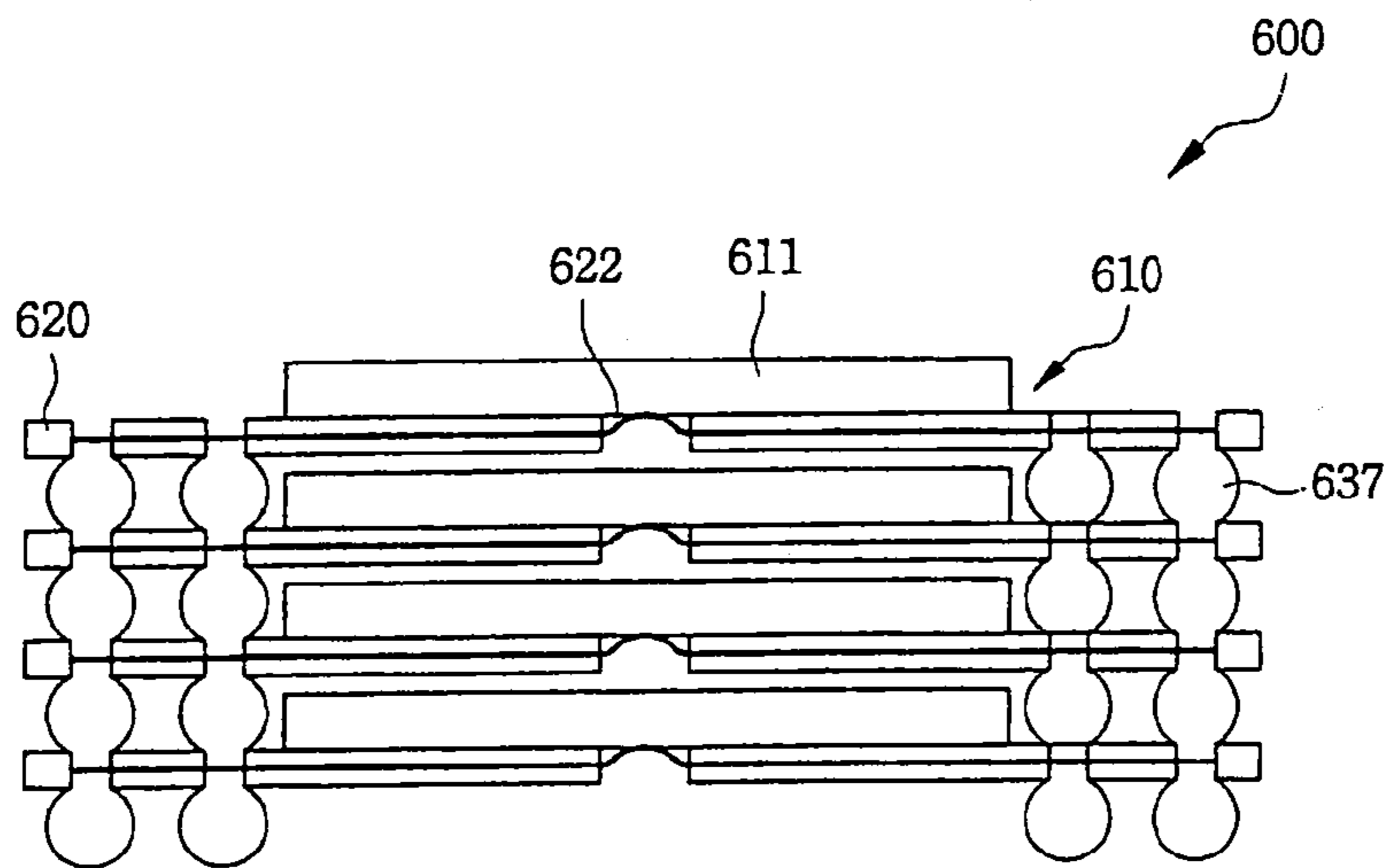
FIG. 1 (Prior Art)
