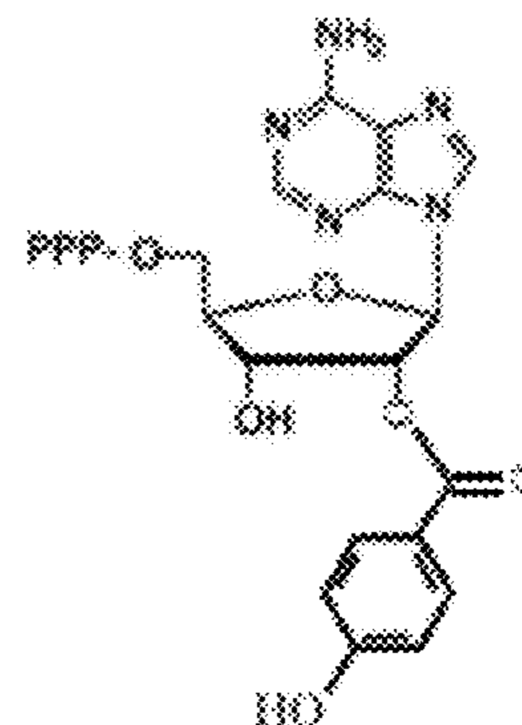
2'-p-hydroxyphenacyl-ATP
