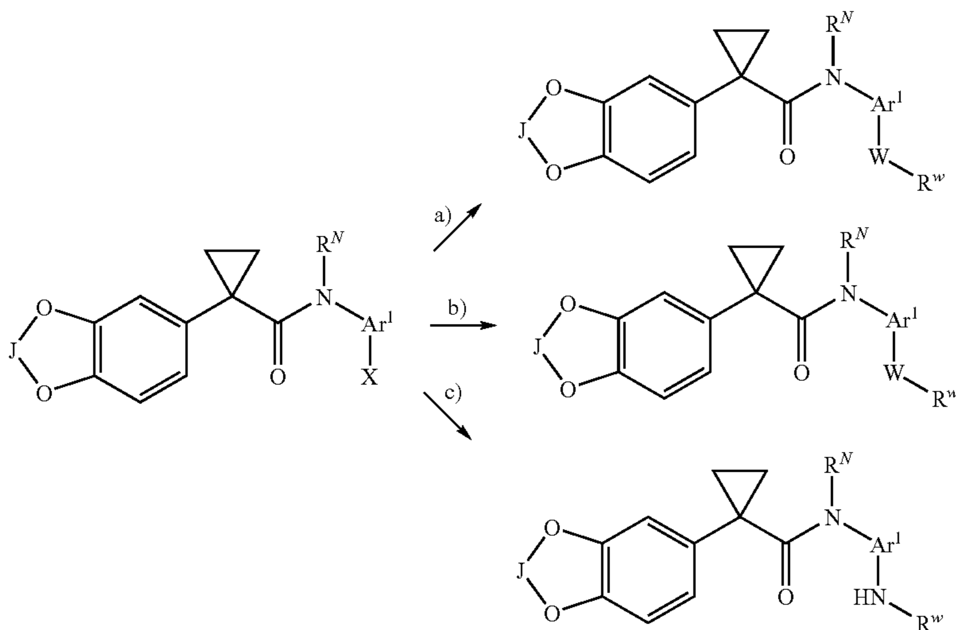
Scheme III-Derivatization of heteroarylhalides
