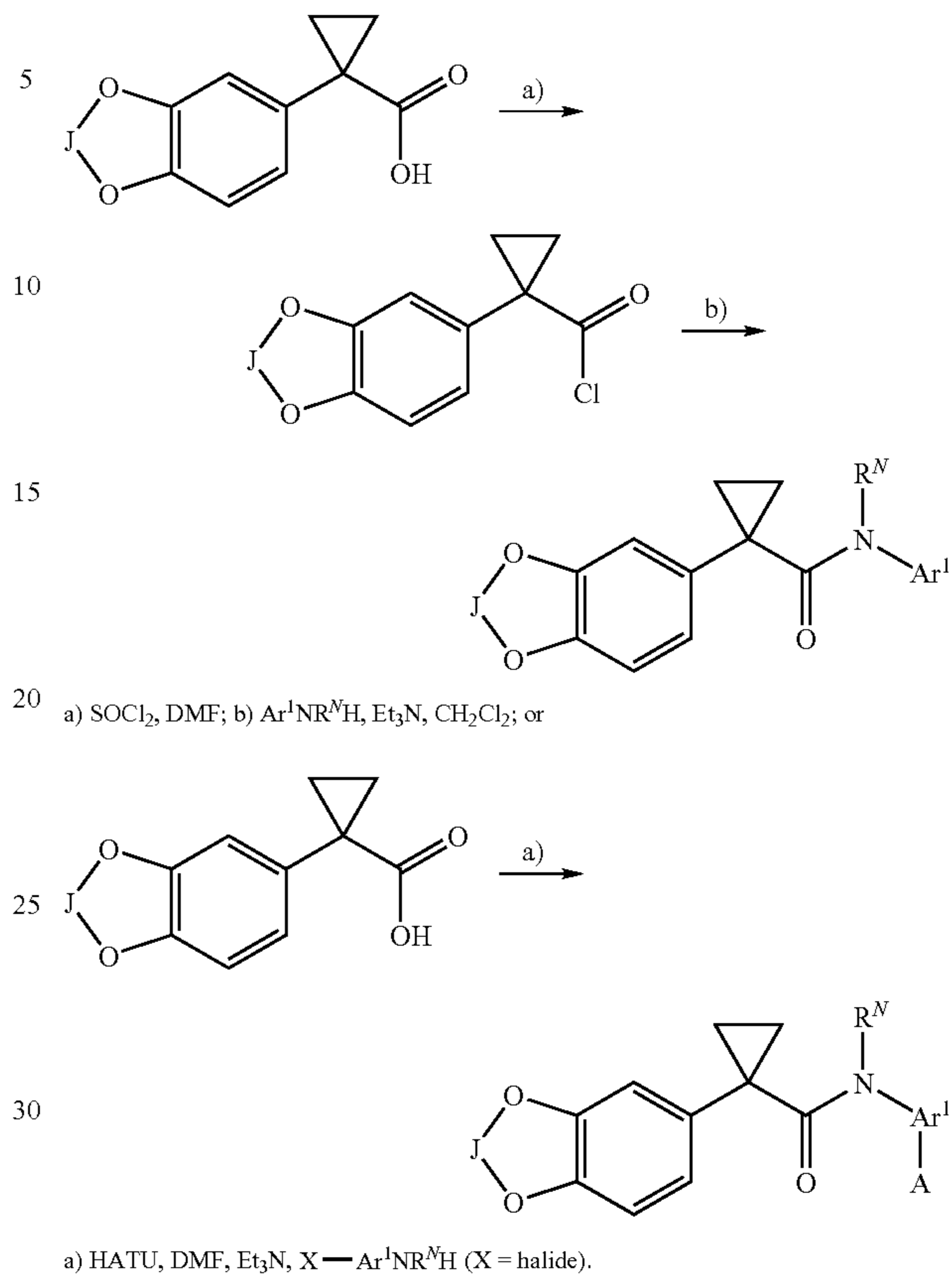
Scheme II-Amid coupling.
