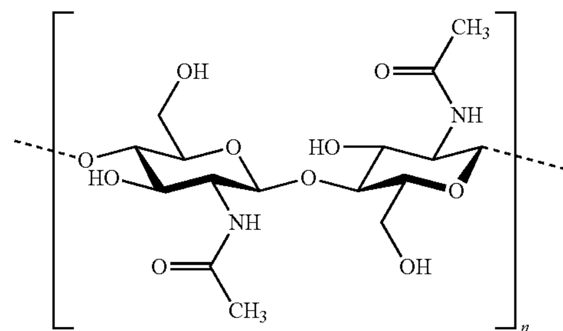
Chitin Chemical Structure
