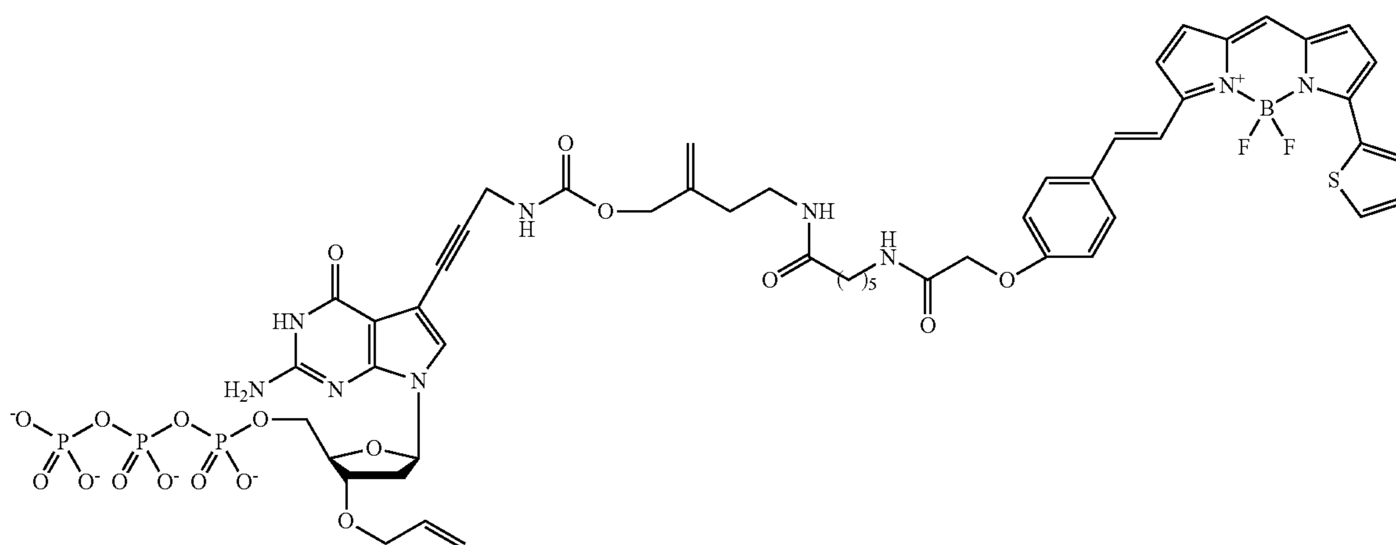
3'-O-allyl-dGTP-allyl-Bodipy-650 43
