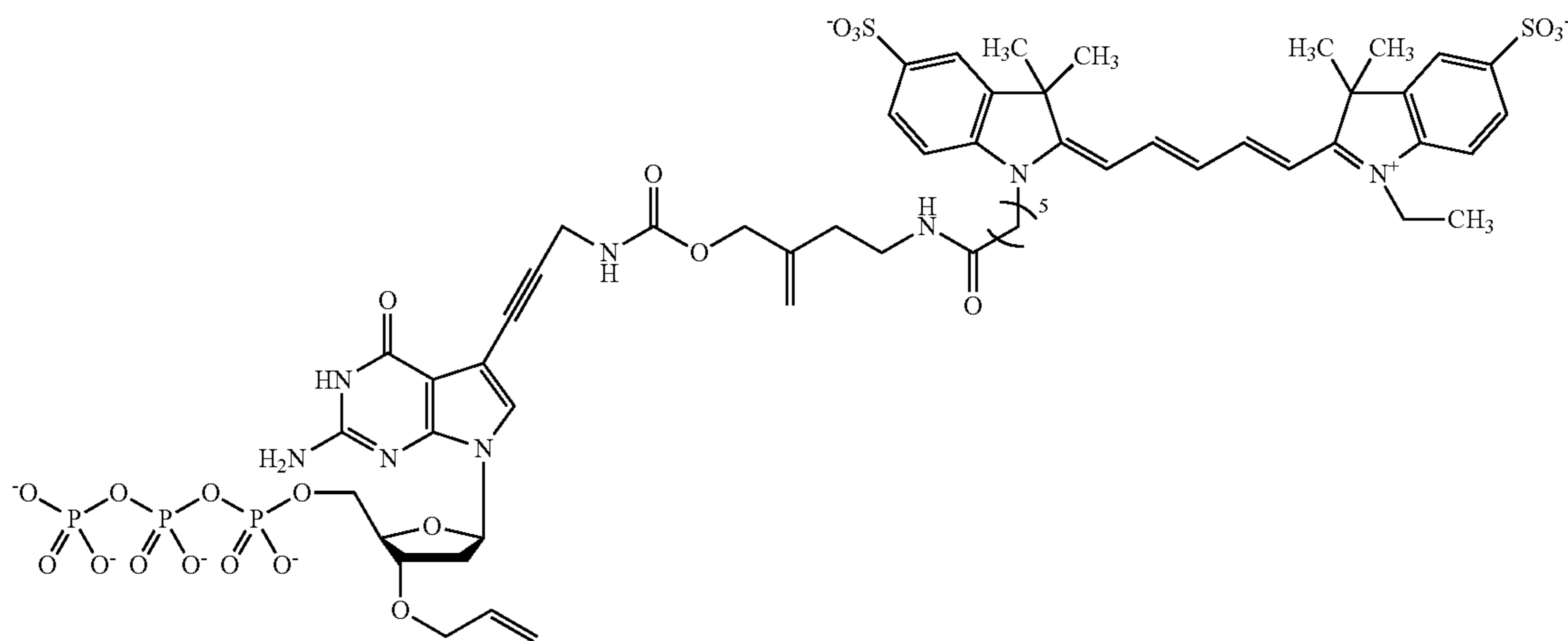
3'-O-allyl-dGTP-allyl-Cy5 44
