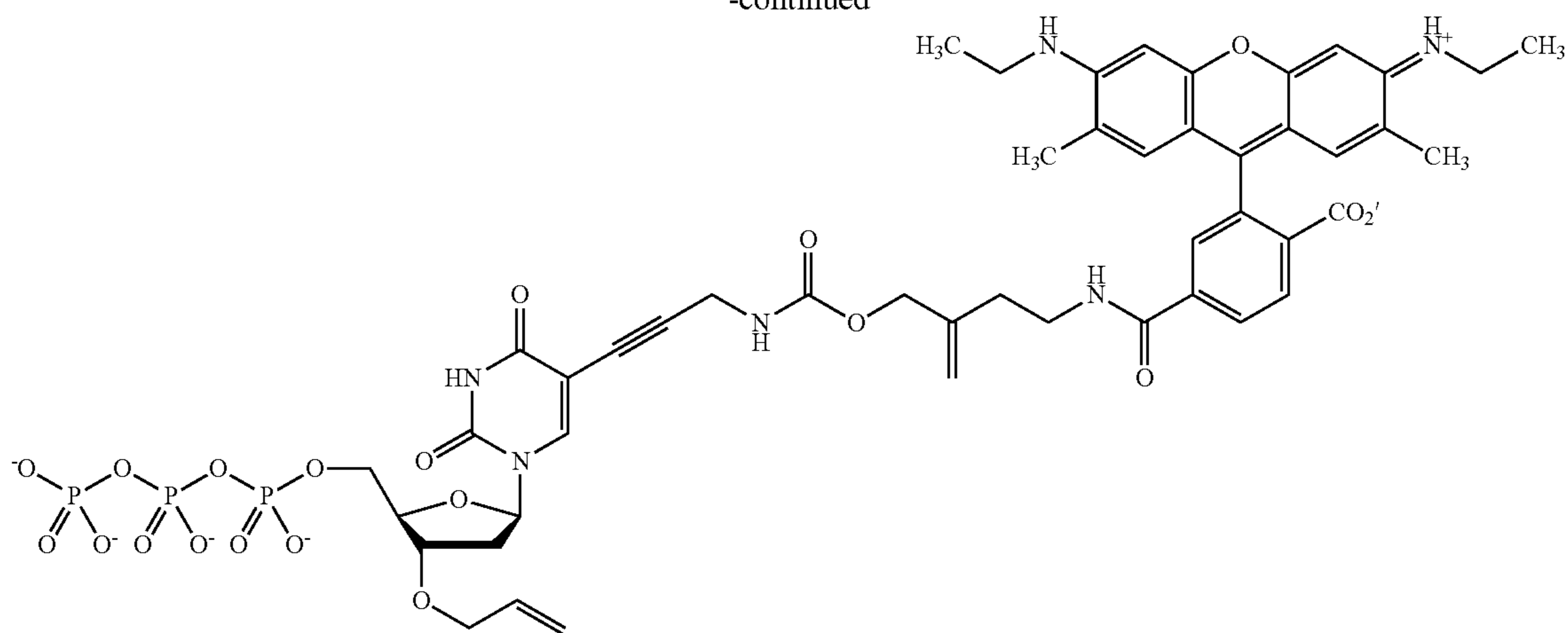
3'-O-allyl dUTP-allyl-R6G 27
