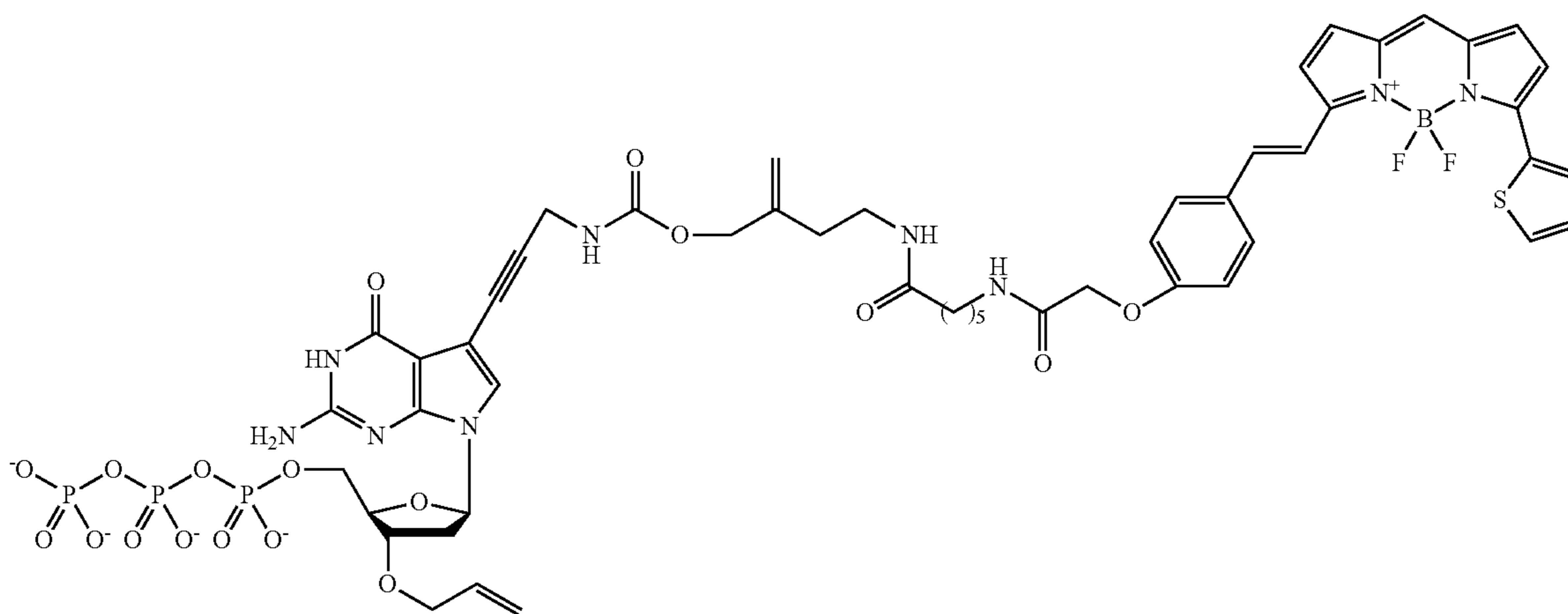
3'-O-allyl-dGTP-allyl-Bodipy-650 43
