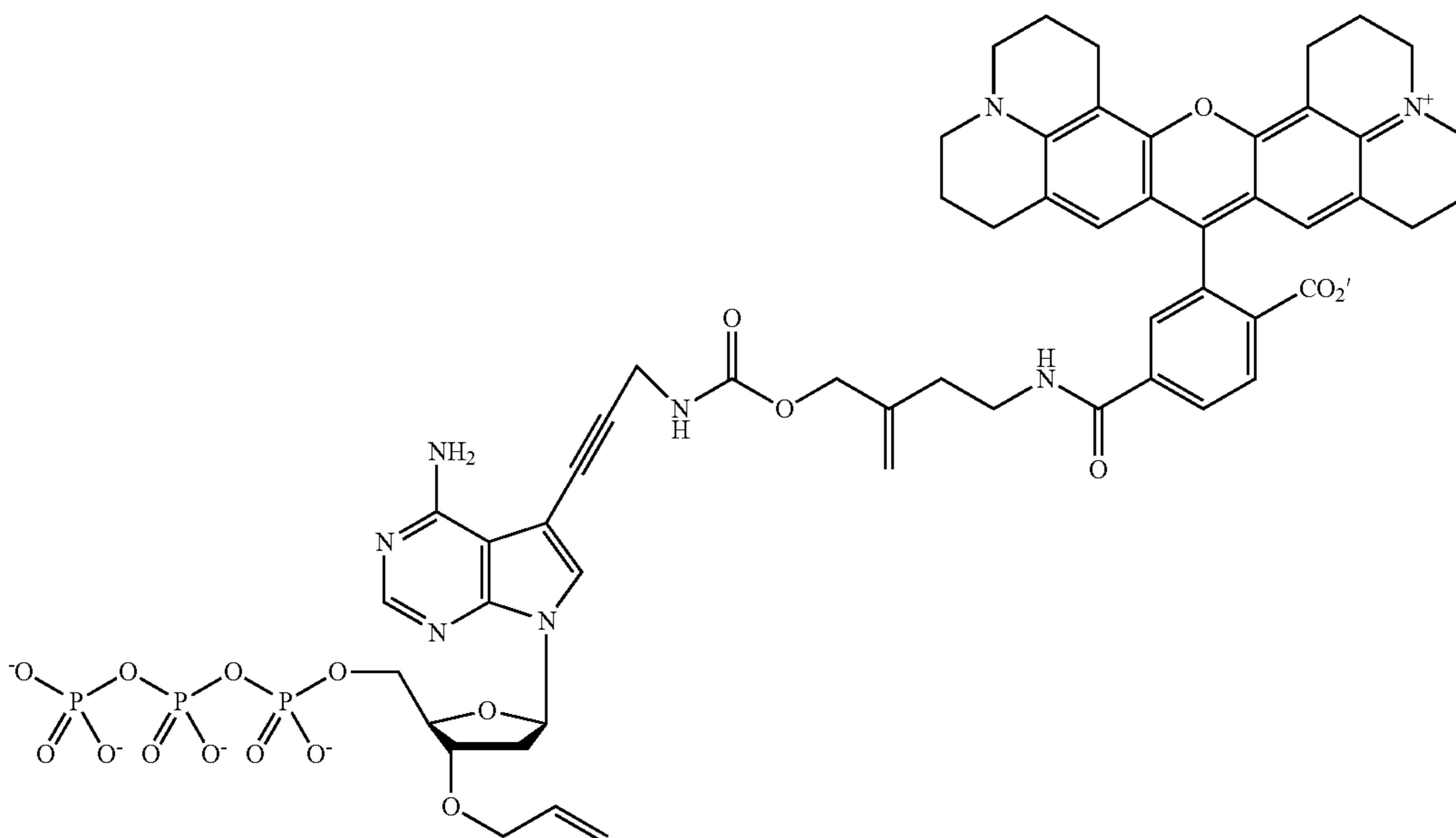
3'-O-allyl-dATP-allyl-ROX 39
