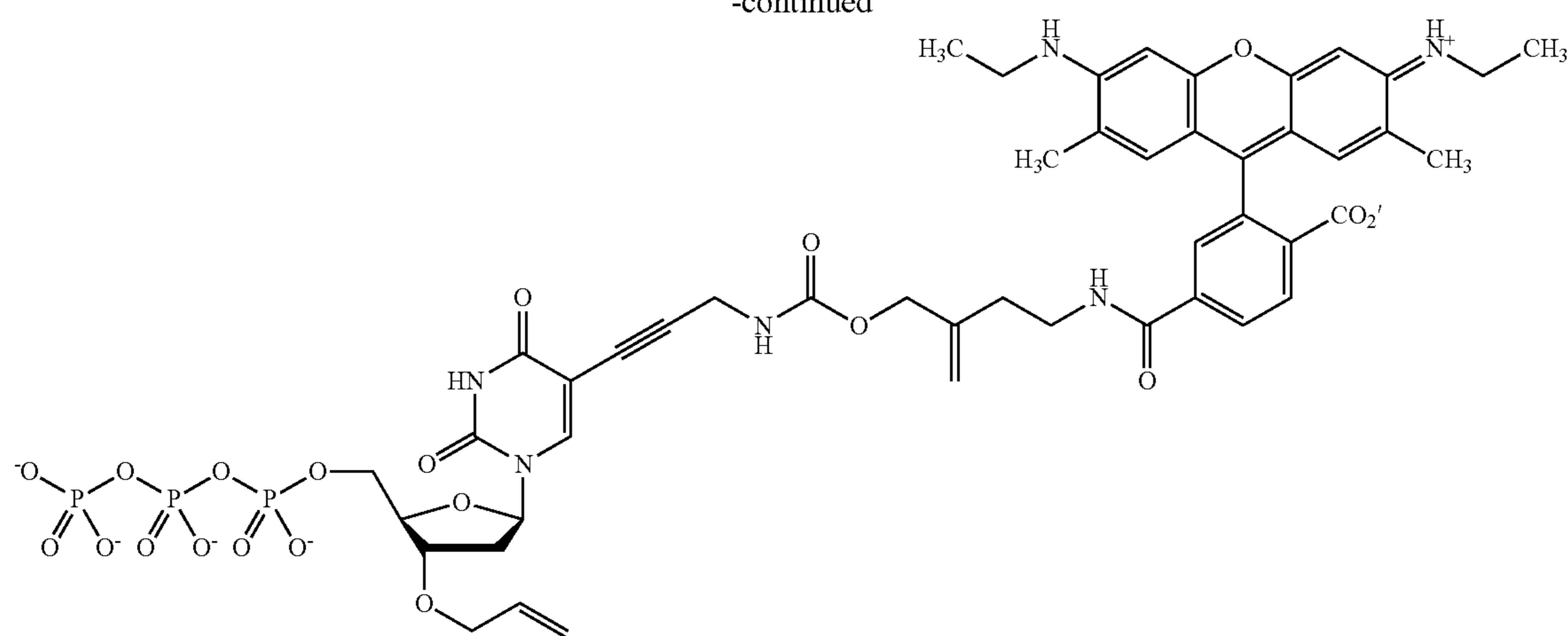
3'-O-allyl dUTP-allyl-R6G 27
