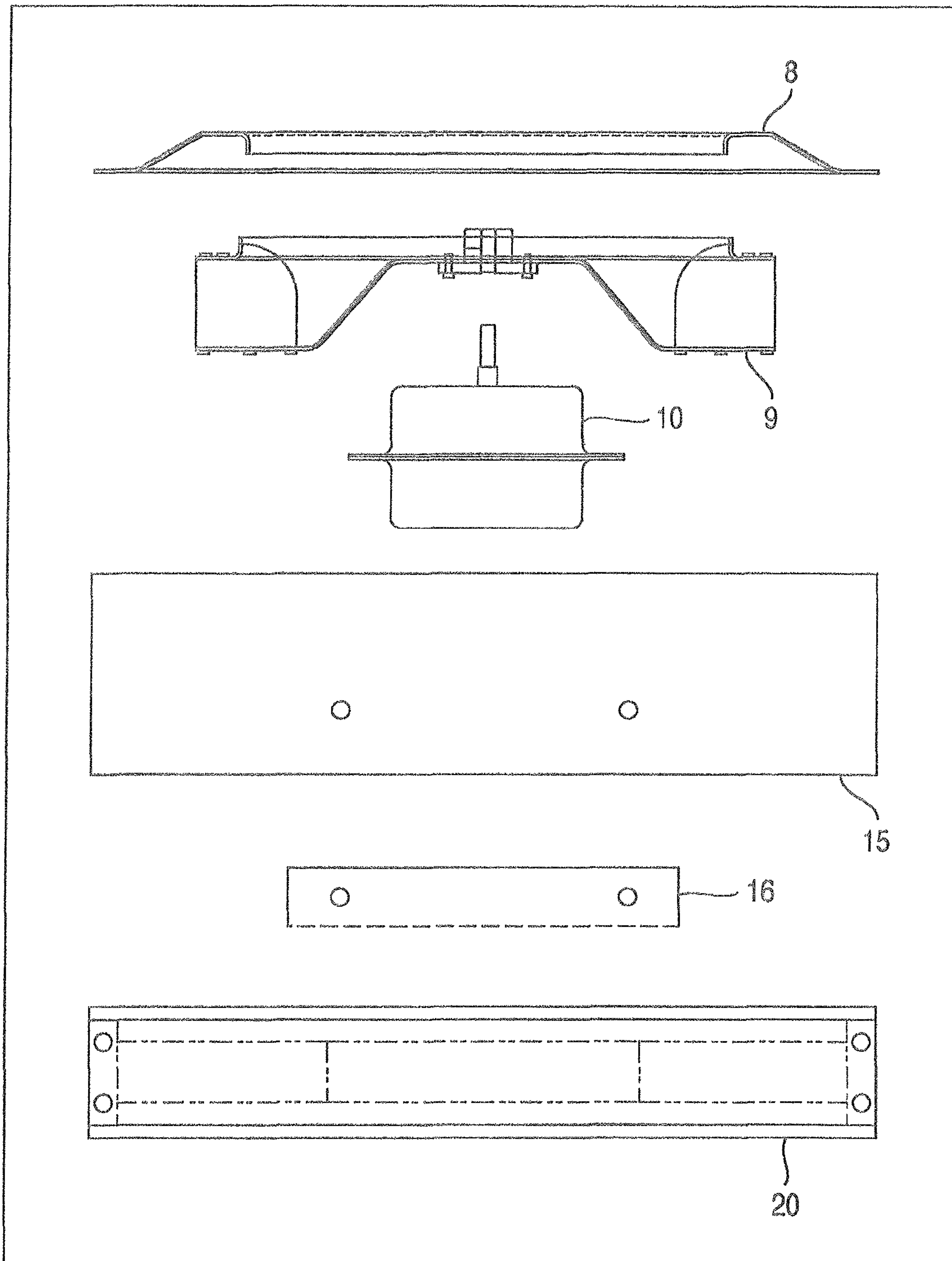
FIG. 11 PRIOR ART
