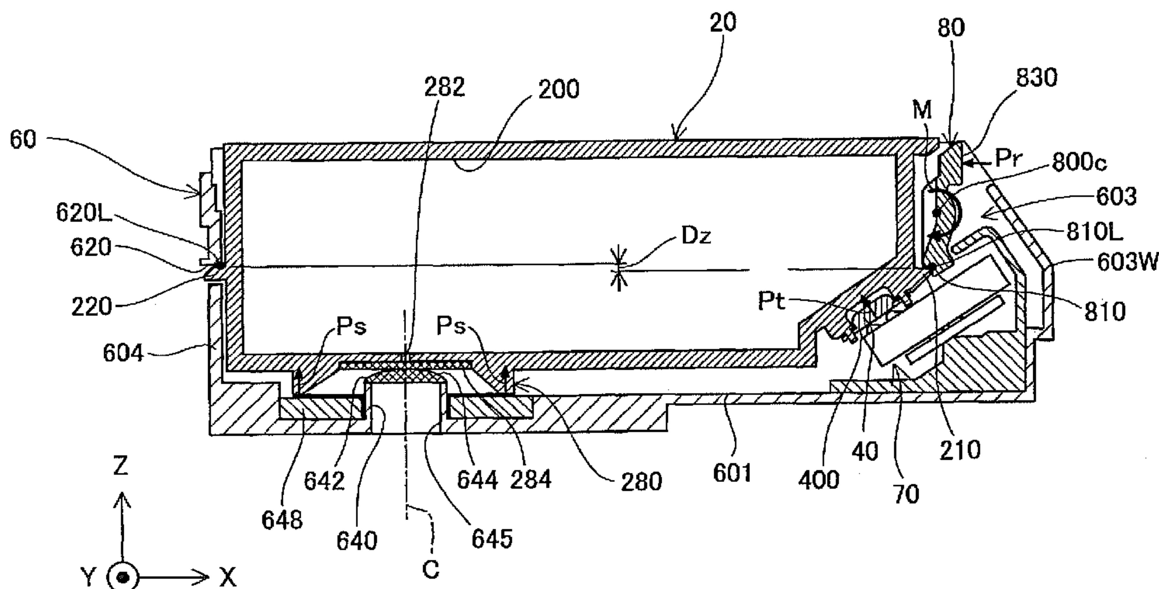
F4-F4 CROSS SECTION
