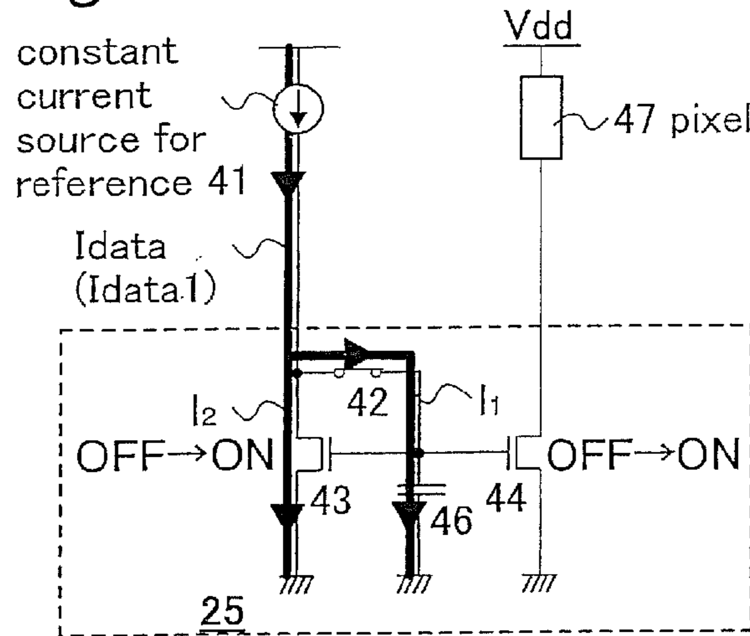
Fig. 20C signal input time to pixel
