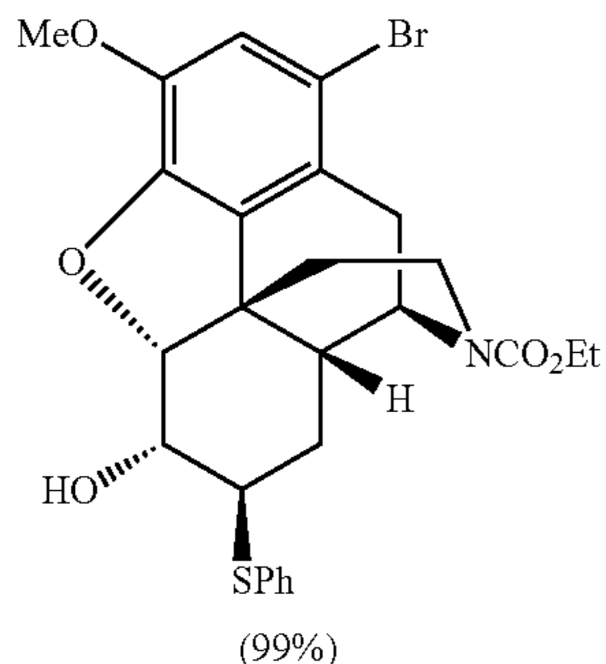
Phenyl Sulfide (22)
