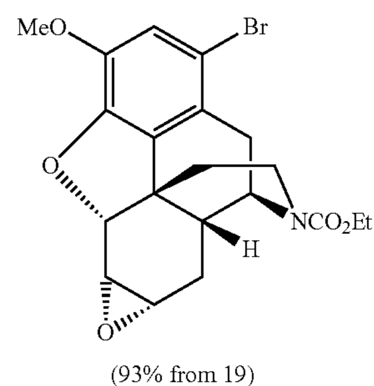
Epoxide (21)
