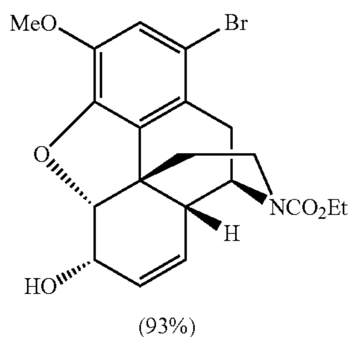
Allylic Alcohol (23)
