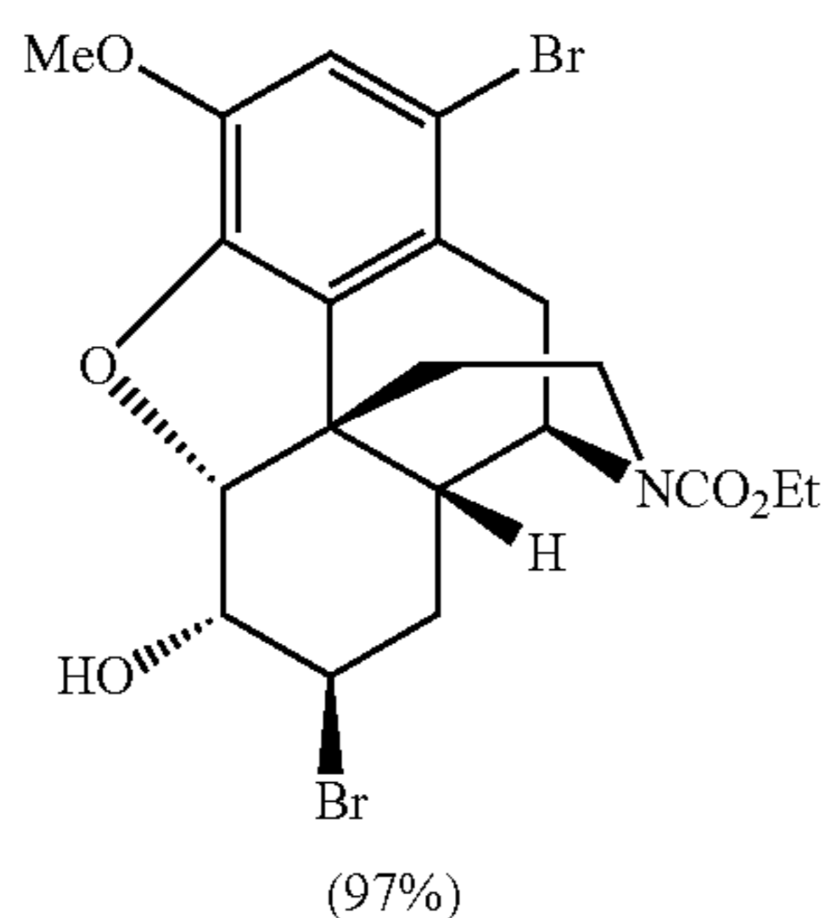
Bromohydrin (20)
