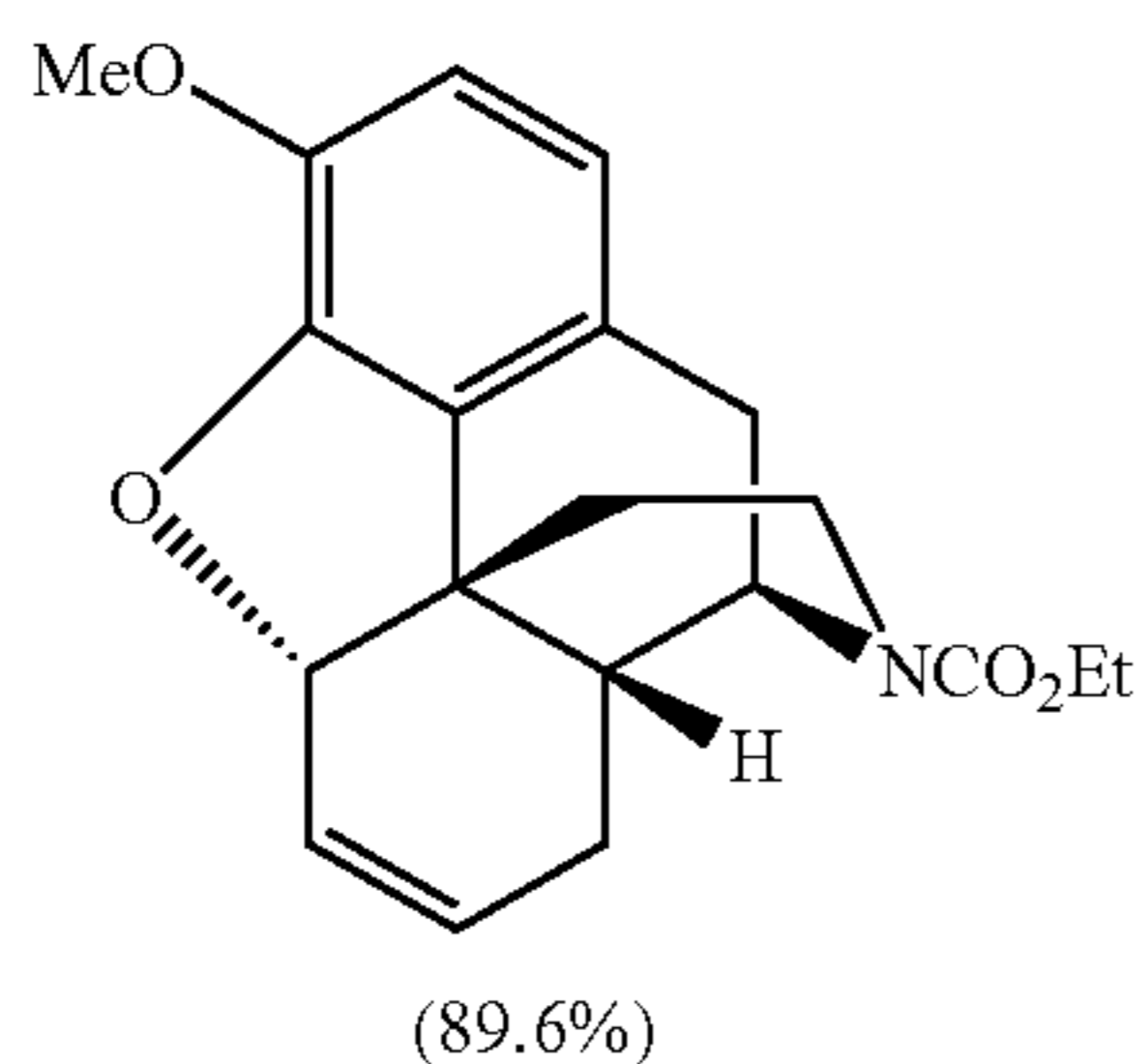
Ethyl Carbamate (19)
